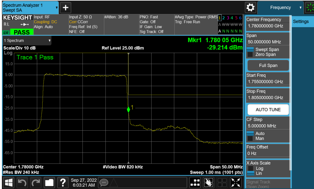
Plot 7-305. Upper Band Edge Plot (NR Band n66 – 20.0MHz - Full RB - ANT A)
