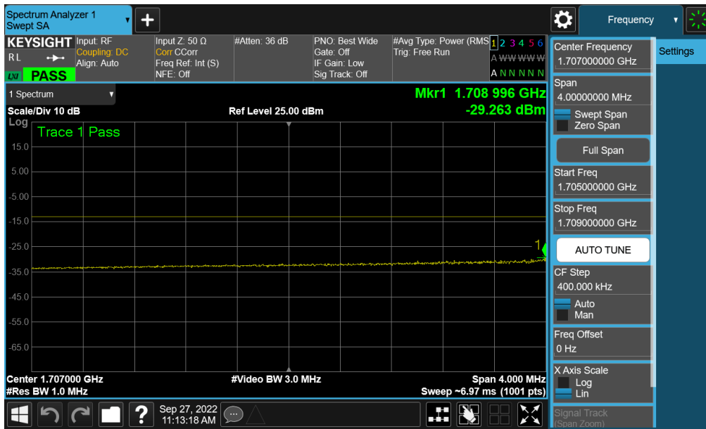
Plot 7-364. Lower Extended Band Edge Plot (NR Band n66 – 30.0MHz - Full RB - Ant F)
