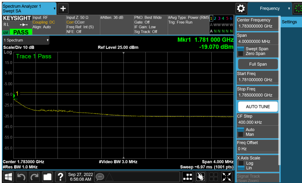
Plot 7-314. Upper Extended Band Edge Plot (NR Band n66 – 10.0MHz - Full RB - ANT A)
