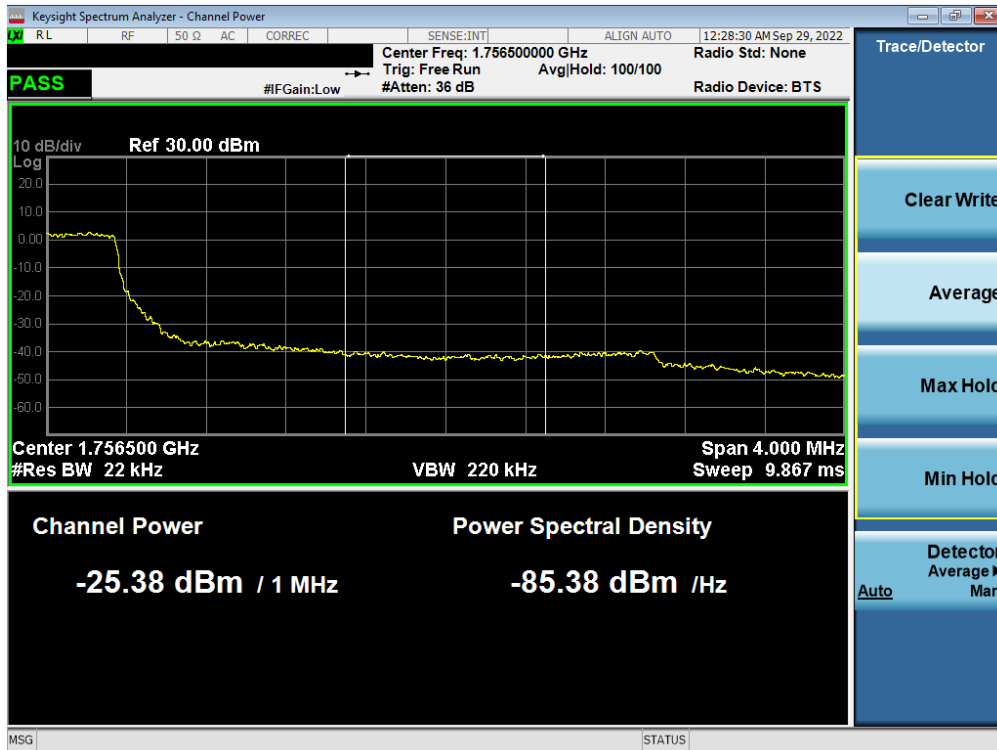
Plot 7-350. Upper Extended Band Edge Plot (LTE Band 4 - 3MHz QPSK – Full RB - Ant F)
