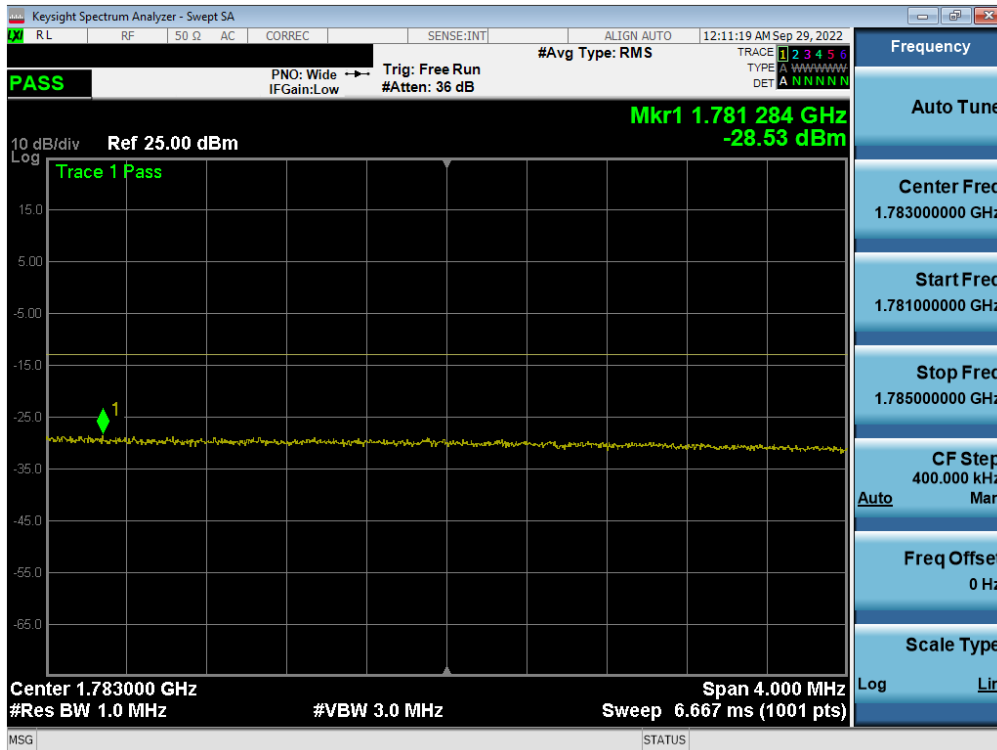
Plot 7-328. Channel Edge Plot (LTE Band 66 - 20MHz QPSK – Full RB - Ant F)
