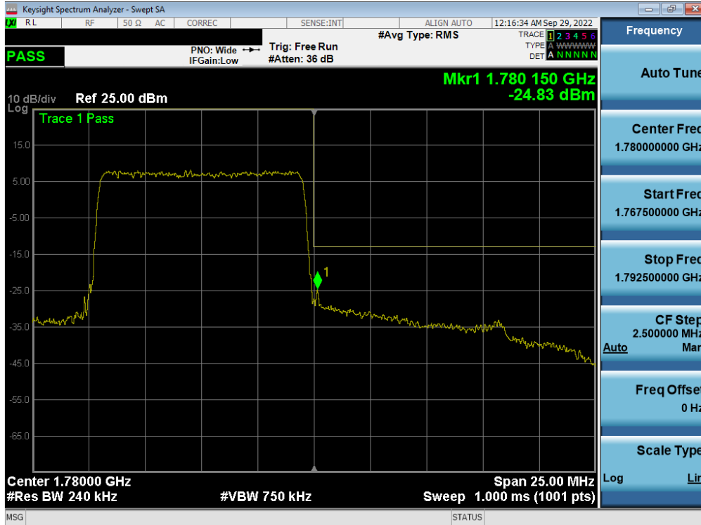
Plot 7-339. Upper Band Edge Plot (LTE Band 66 - 10MHz QPSK - Full RB - Ant F)
