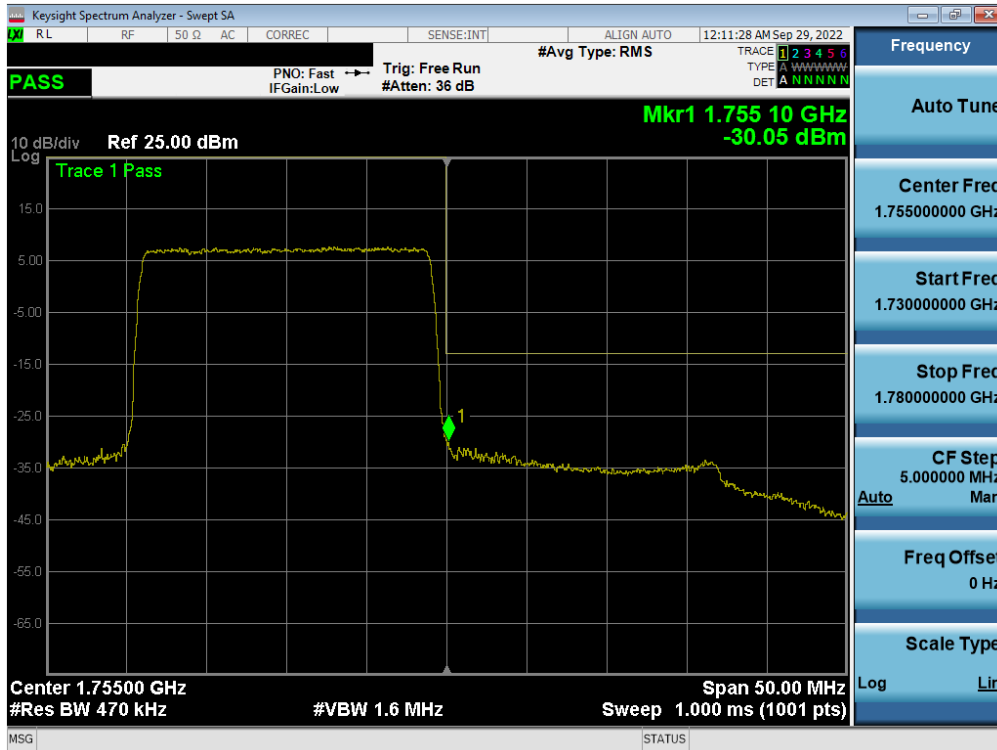
Plot 7-325. Upper Band Edge Plot (LTE Band 4 - 20MHz QPSK – Full RB - Ant F)
