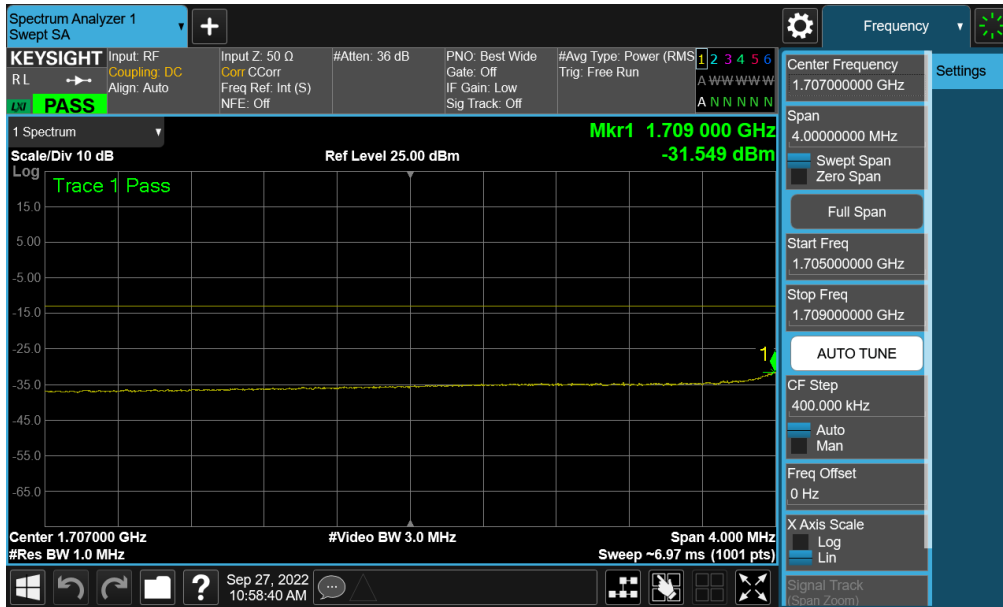
Plot 7-360. Lower Extended Band Edge Plot (NR Band n66 – 40.0MHz - Full RB - Ant F)
