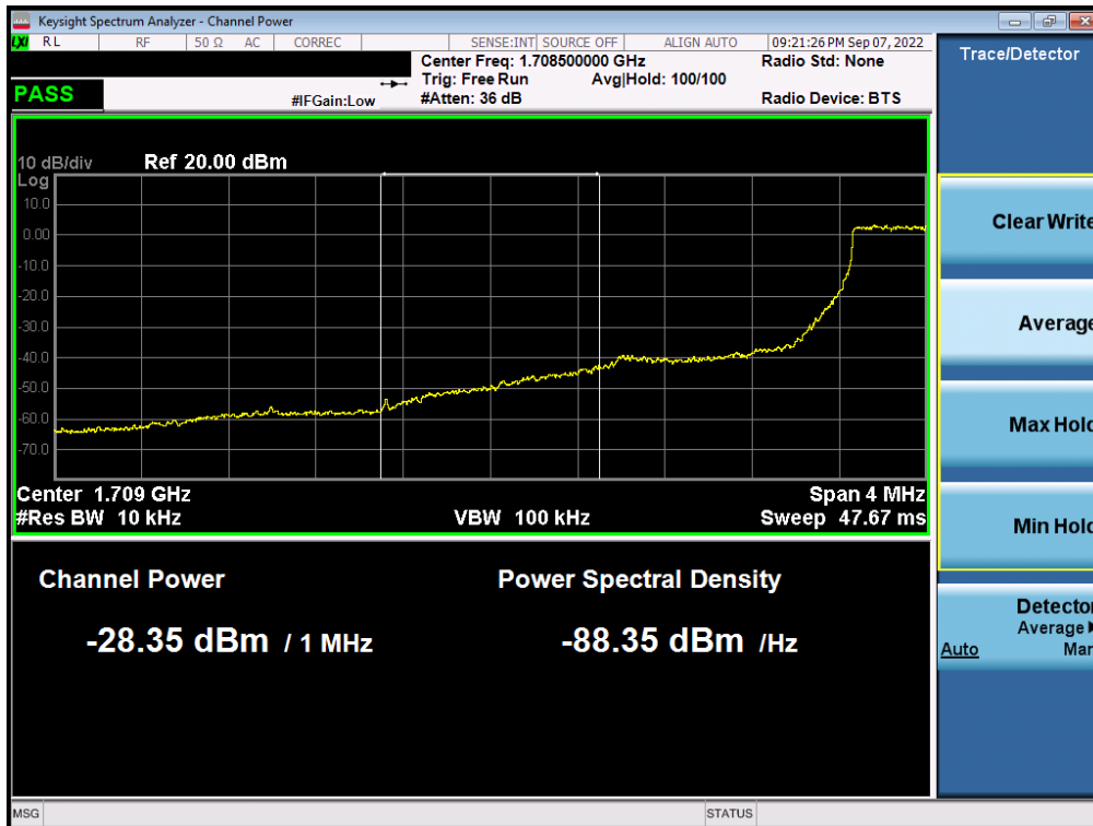
Plot 7-286. Lower Extended Band Edge Plot (LTE Band 66/4 – 1.4MHz QPSK – Full RB - ANT A)
