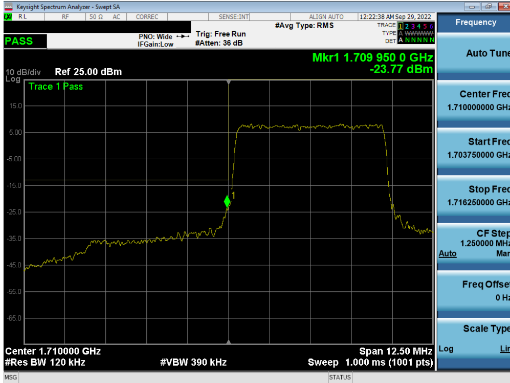
Plot 7-341. Lower Band Edge Plot (LTE Band 66/4 - 5MHz QPSK – Full RB - Ant F)
