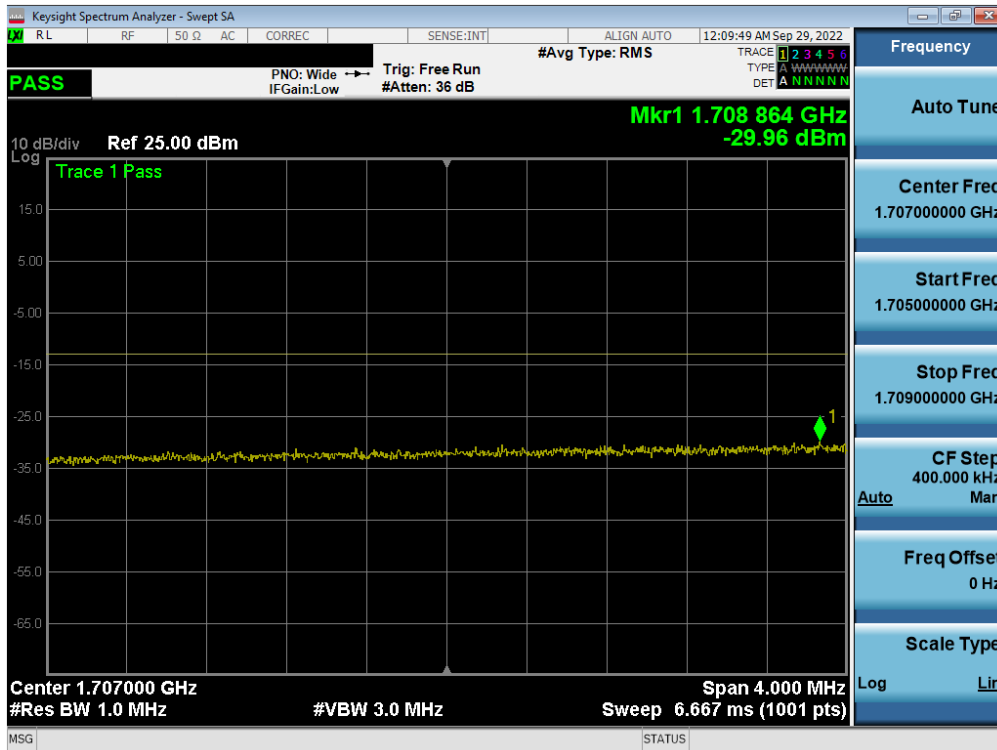
Plot 7-324. Lower Extended Band Edge Plot (LTE Band 66/4 - 20MHz QPSK – Full RB - Ant F)
