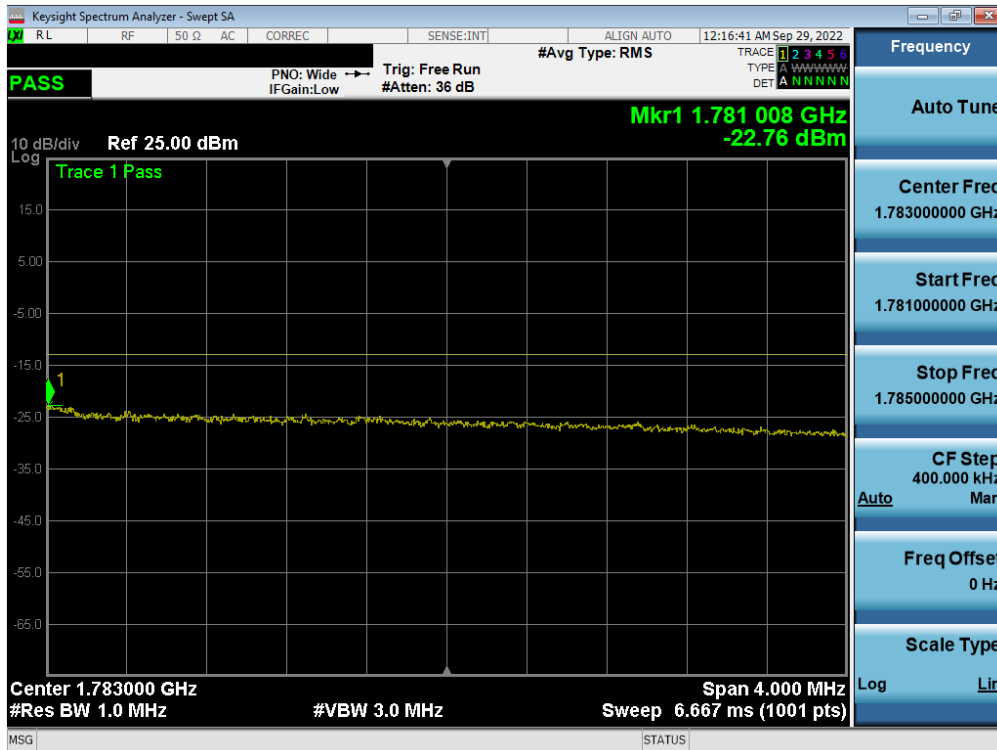
Plot 7-340. Upper Extended Band Edge Plot (LTE Band 66 - 10MHz QPSK - Full RB - Ant F)
