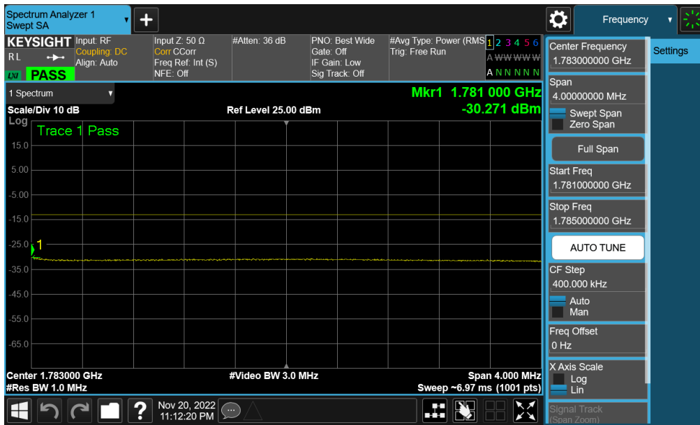
Plot 7-302. Upper Extended Band Edge Plot (NR Band n66 – 25.0MHz - Full RB - ANT A)
