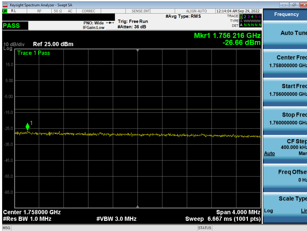
Plot 7-332. Upper Extended Band Edge Plot (LTE Band 4 - 15MHz QPSK – Full RB - Ant F)
