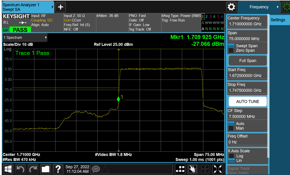
Plot 7-363. Lower Band Edge Plot (NR Band n66 – 30.0MHz - Full RB - Ant F)
