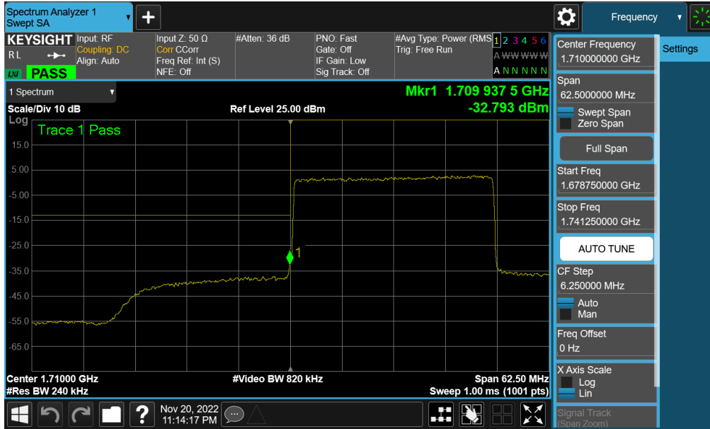
Plot 7-299. Lower Band Edge Plot (NR Band n66 – 25.0MHz - Full RB - ANT A)
