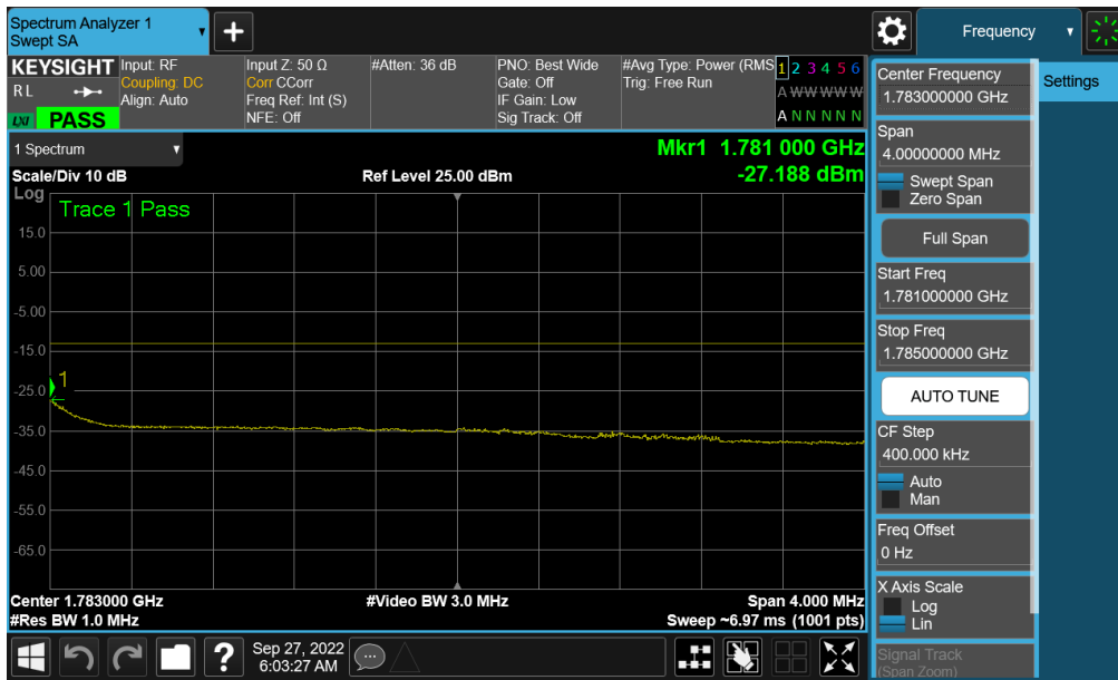
Plot 7-306. Upper Extended Band Edge Plot (NR Band n66 – 20.0MHz - Full RB - ANT A)
