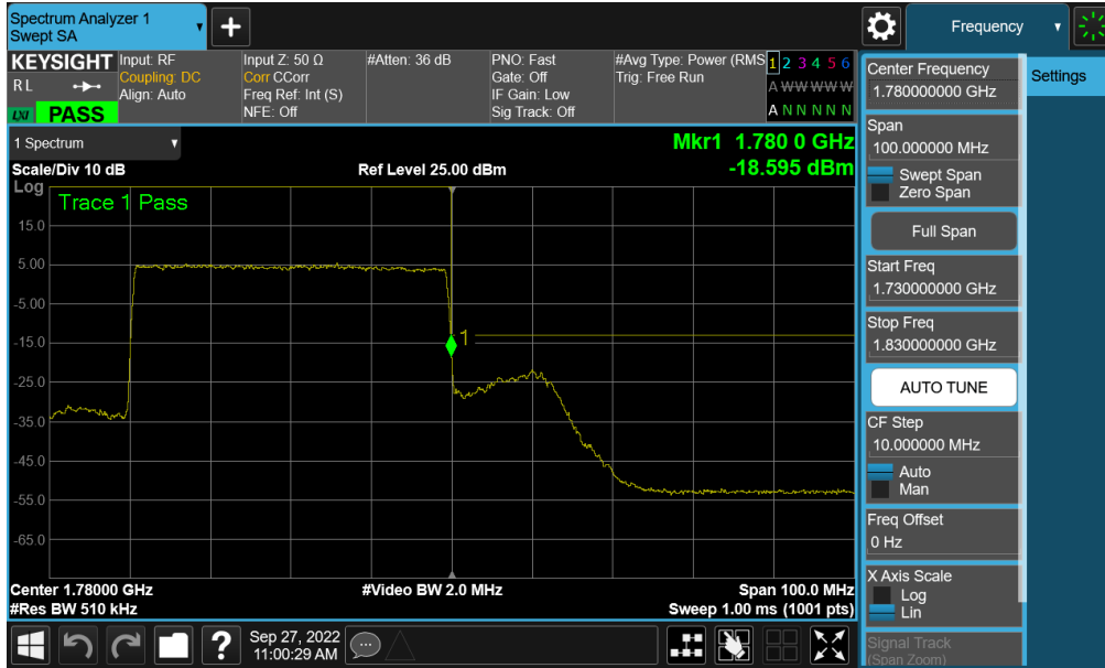
Plot 7-361. Upper Band Edge Plot (NR Band n66 – 40.0MHz - Full RB - Ant F)
