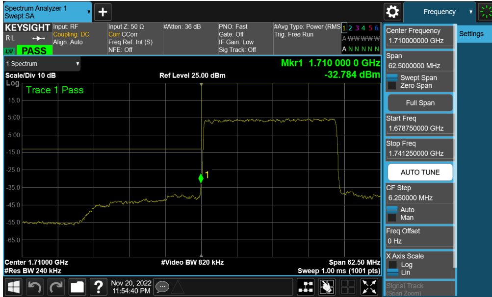
Plot 7-367. Lower Band Edge Plot (NR Band n66 – 30.0MHz - Full RB - Ant F)
