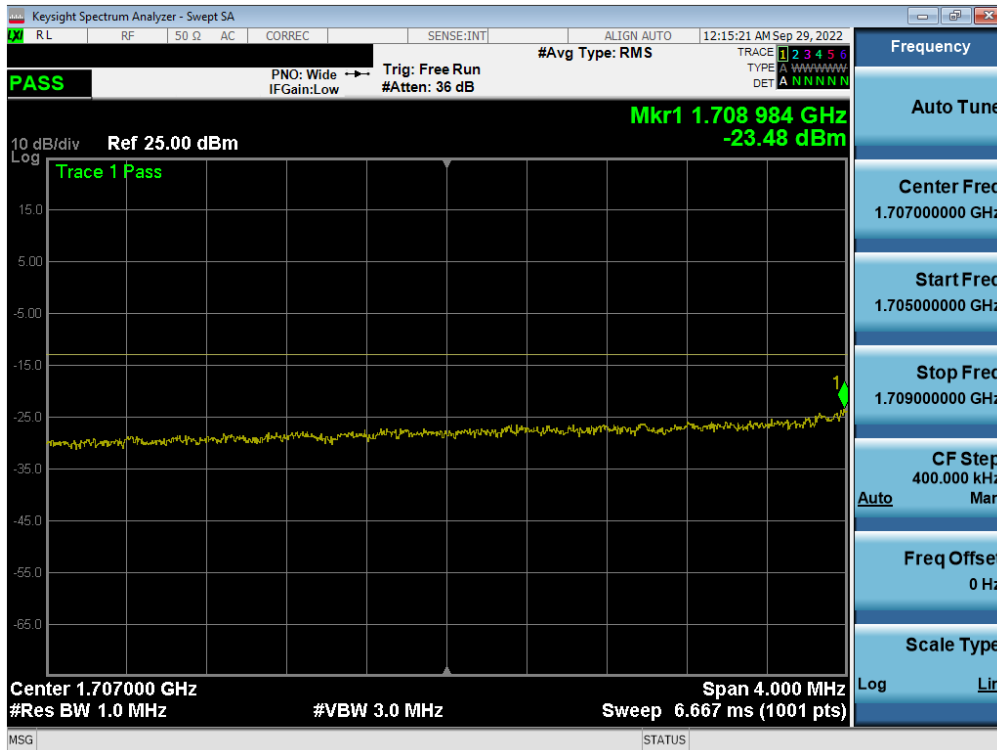
Plot 7-336. Lower Extended Band Edge Plot (LTE Band 66/4 - 10MHz QPSK – Full RB - Ant F)
