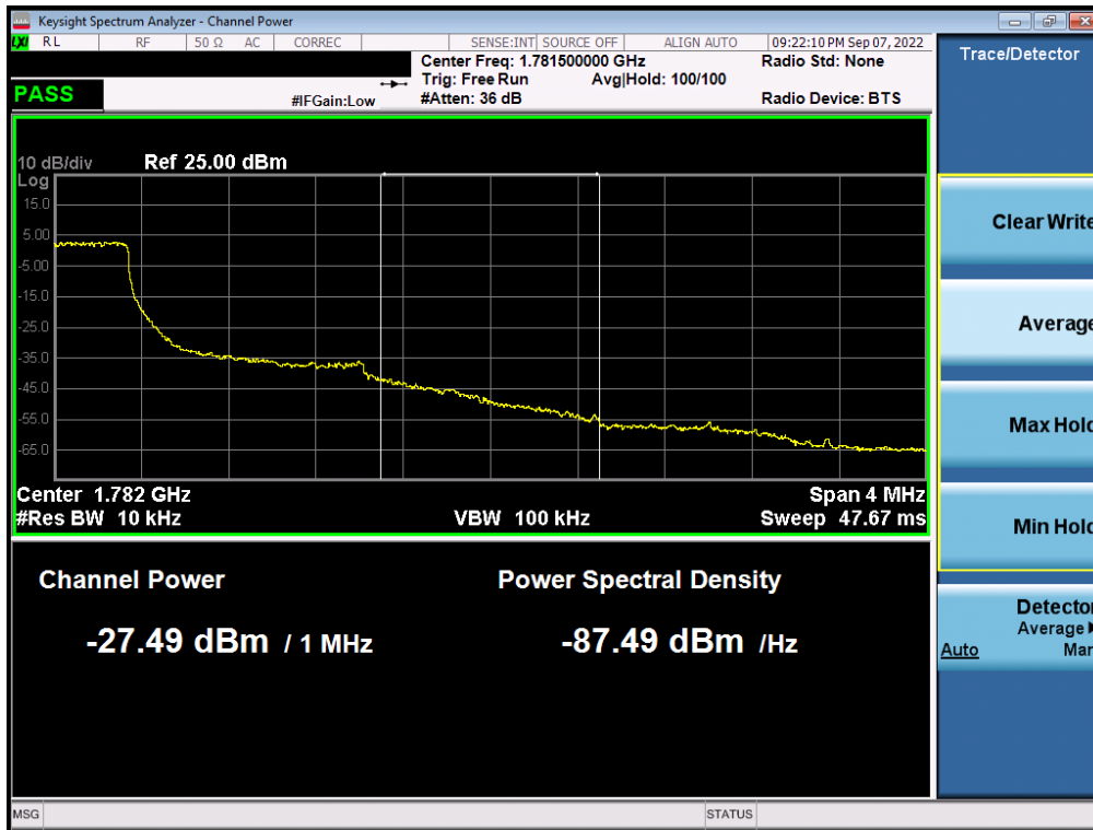
Plot 7-290. Upper Extended Band Edge Plot (LTE Band 66 – 1.4MHz QPSK – Full RB - ANT A)
