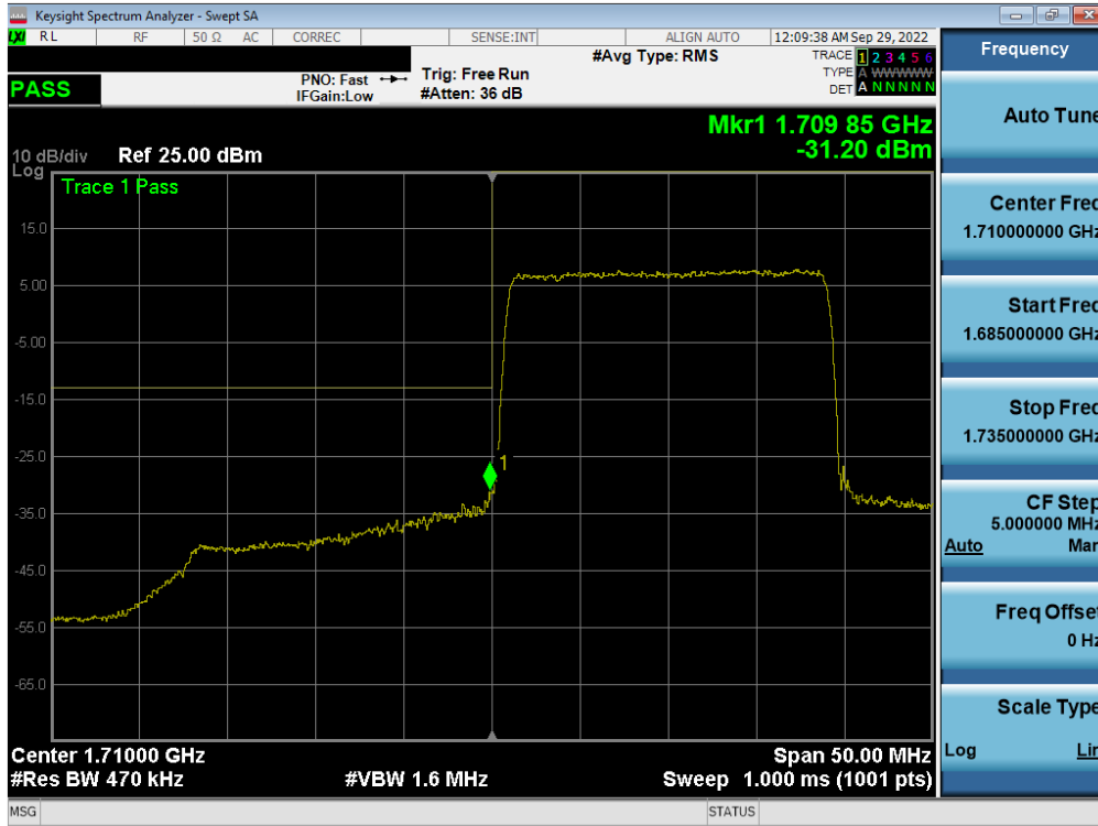
Plot 7-323. Lower Band Edge Plot (LTE Band 66/4 - 20MHz QPSK – Full RB - Ant F)
