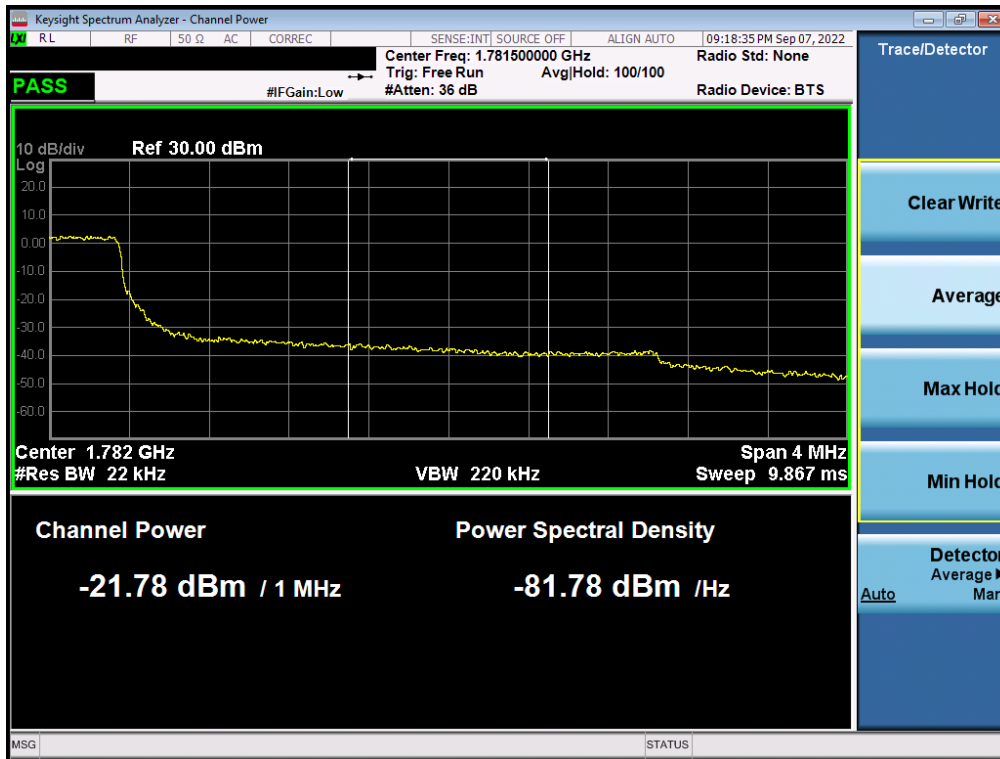
Plot 7-284. Upper Extended Band Edge Plot (LTE Band 66 - 3MHz QPSK – Full RB - ANT A)
