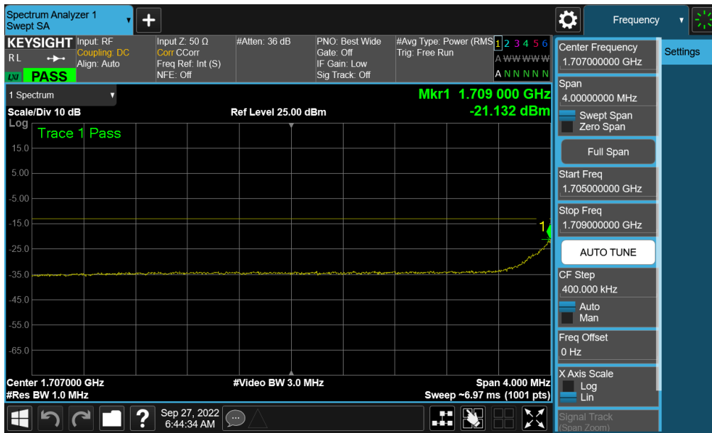
Plot 7-308. Lower Extended Band Edge Plot (NR Band n66 – 15.0MHz - Full RB - ANT A)
