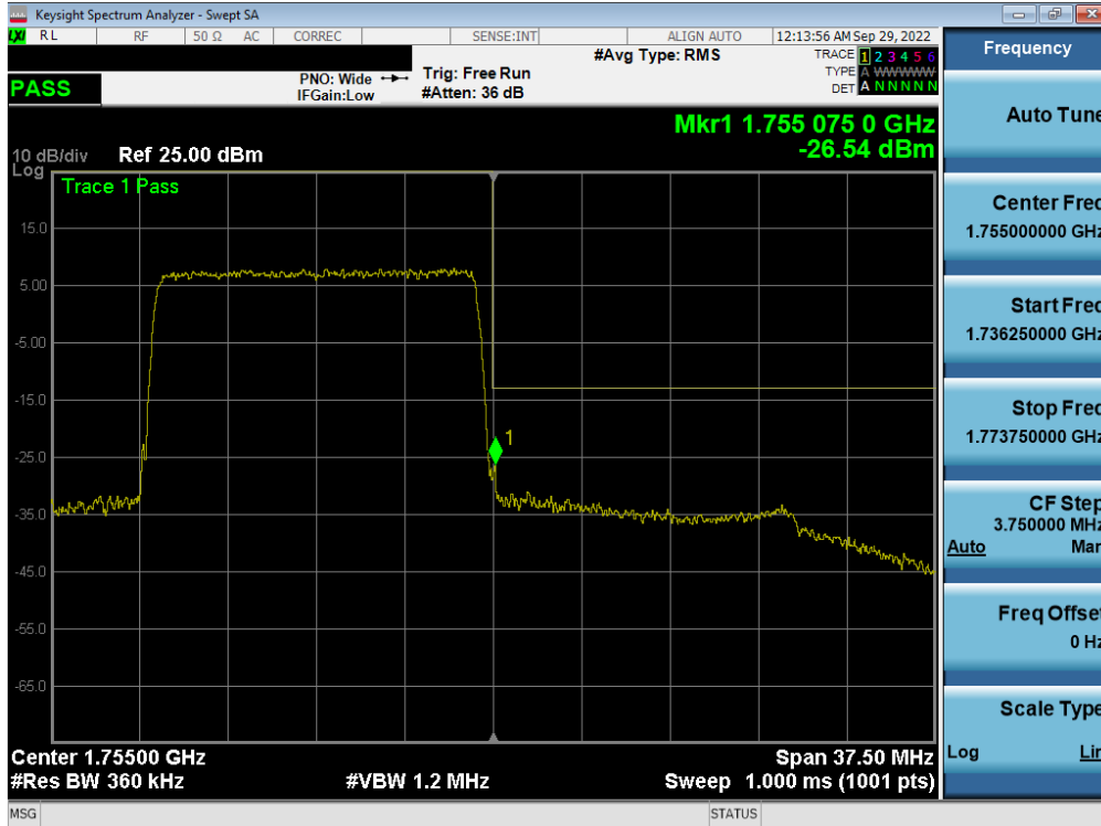
Plot 7-331. Upper Band Edge Plot (LTE Band 4 - 15MHz QPSK – Full RB - Ant F)
