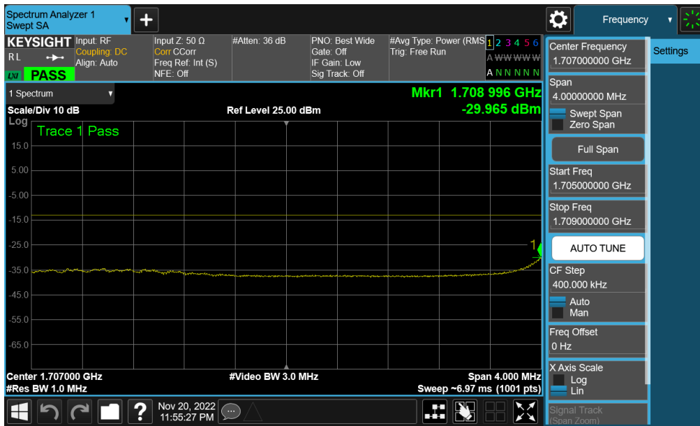
Plot 7-368. Lower Extended Band Edge Plot (NR Band n66 – 30.0MHz - Full RB - Ant F)
