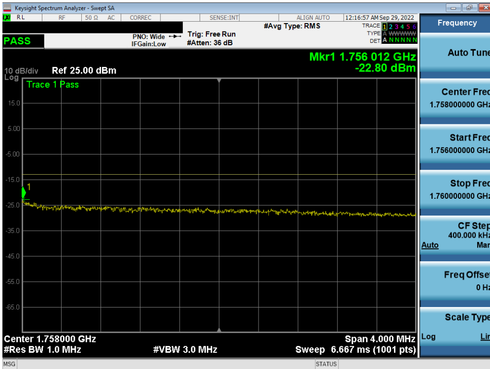
Plot 7-338. Upper Extended Band Edge Plot (LTE Band 4 - 10MHz QPSK – Full RB - Ant F)
