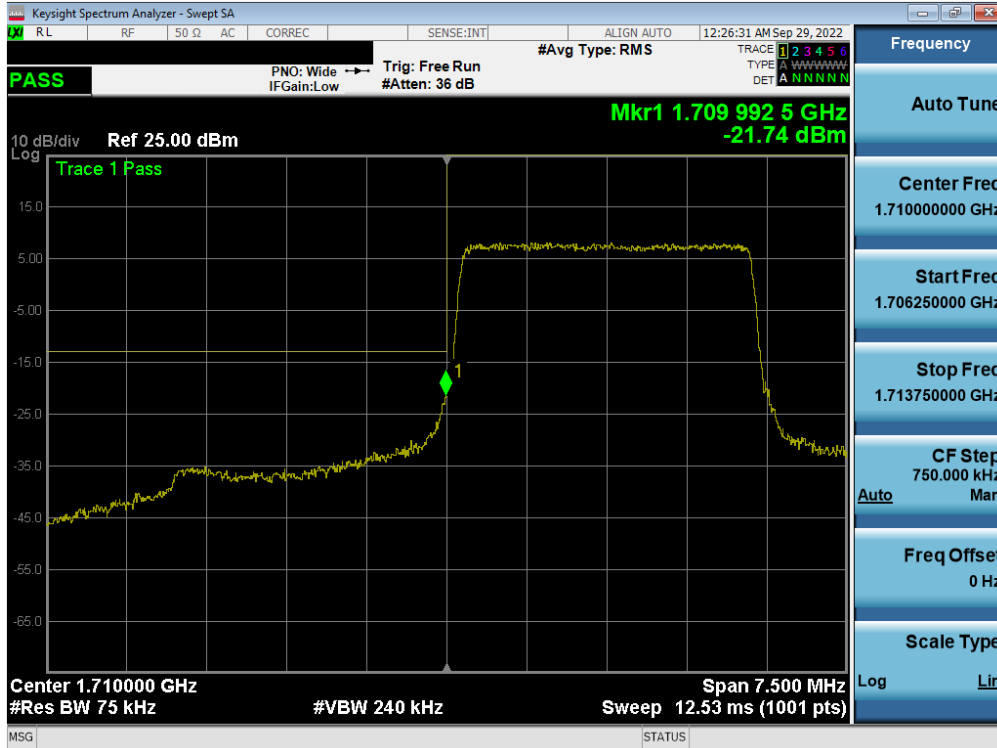
Plot 7-347. Lower Band Edge Plot (LTE Band 66/4 - 3MHz QPSK – Full RB - Ant F)
