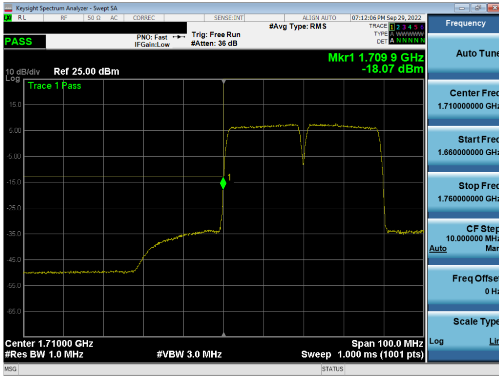
Plot 7-319. Lower Band Edge Plot (ULCA LTE Band 66 - ANT A)
