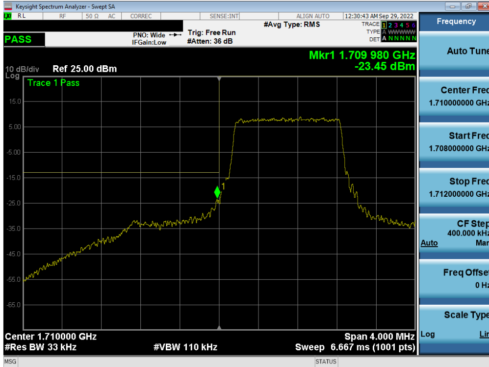
Plot 7-353. Lower Band Edge Plot (LTE Band 66/4 – 1.4MHz QPSK – Full RB - Ant F)
