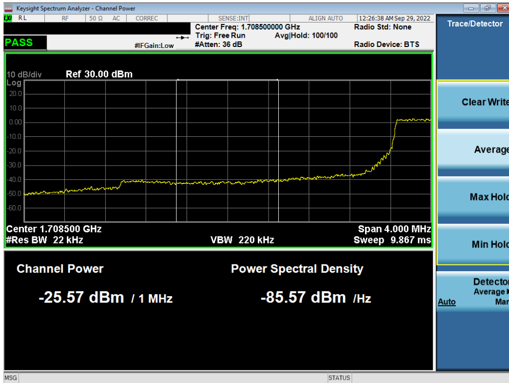
Plot 7-348. Lower Extended Band Edge Plot (LTE Band 66/4 - 3MHz QPSK – Full RB - Ant F)
