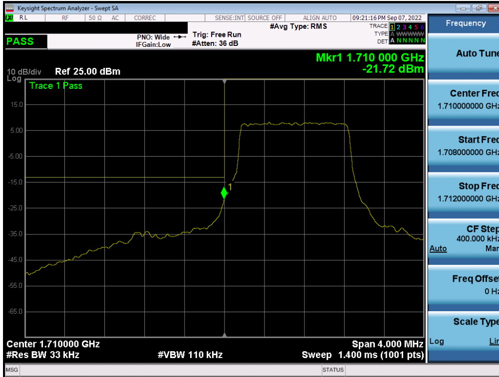
Plot 7-285. Lower Band Edge Plot (LTE Band 66/4 – 1.4MHz QPSK – Full RB - ANT A)
