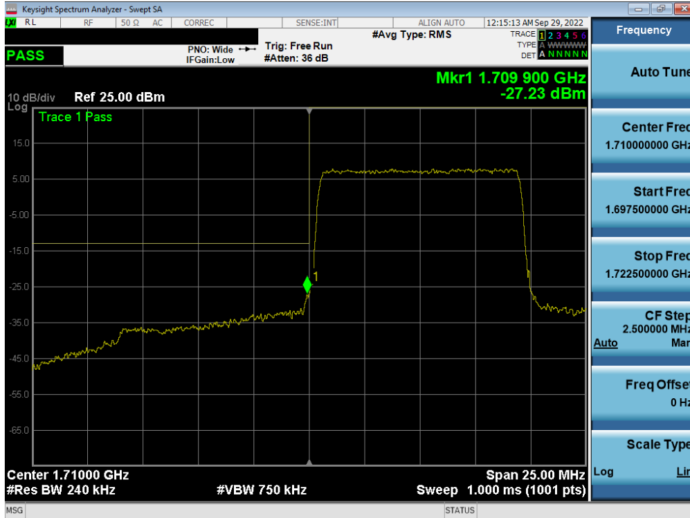
Plot 7-335. Lower Band Edge Plot (LTE Band 66/4 - 10MHz QPSK – Full RB - Ant F)
