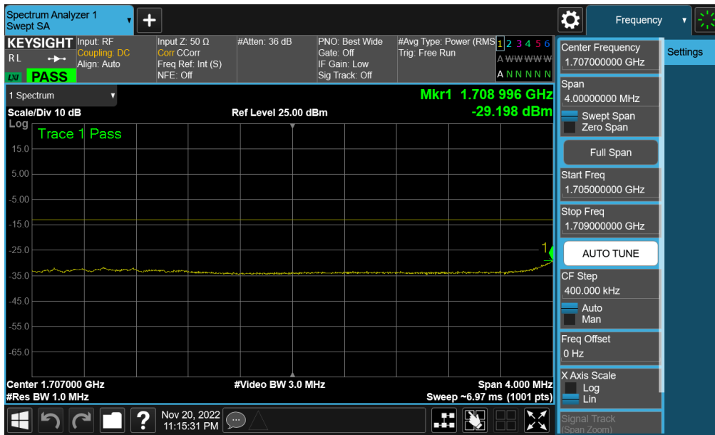
Plot 7-300. Lower Extended Band Edge Plot (NR Band n66 – 25.0MHz - Full RB - ANT A)
