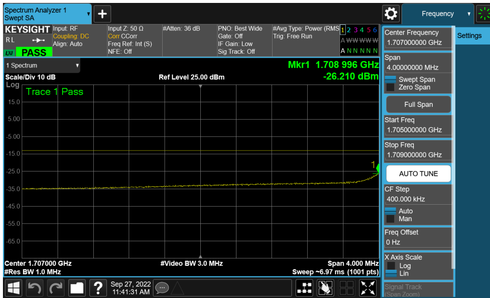
Plot 7-372. Lower Extended Band Edge Plot (NR Band n66 – 20.0MHz - Full RB - Ant F)
