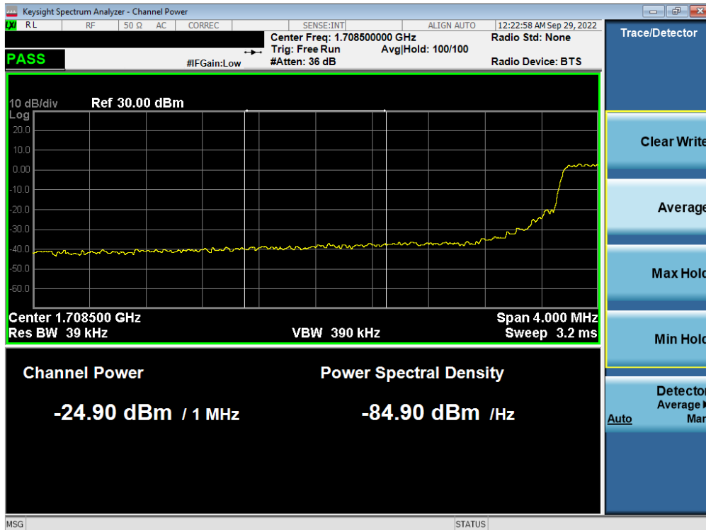
Plot 7-342. Lower Extended Band Edge Plot (LTE Band 66/4 - 5MHz QPSK – Full RB - Ant F)
