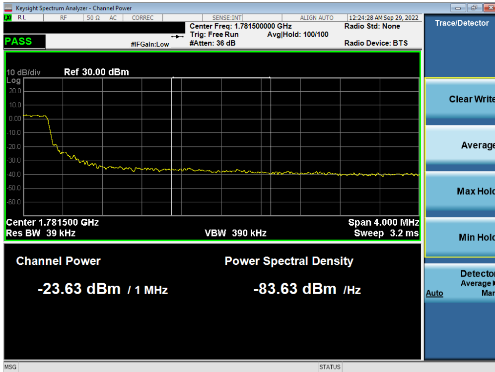
Plot 7-346. Upper Extended Band Edge Plot (LTE Band 66 - 5MHz QPSK – Full RB - Ant F)
