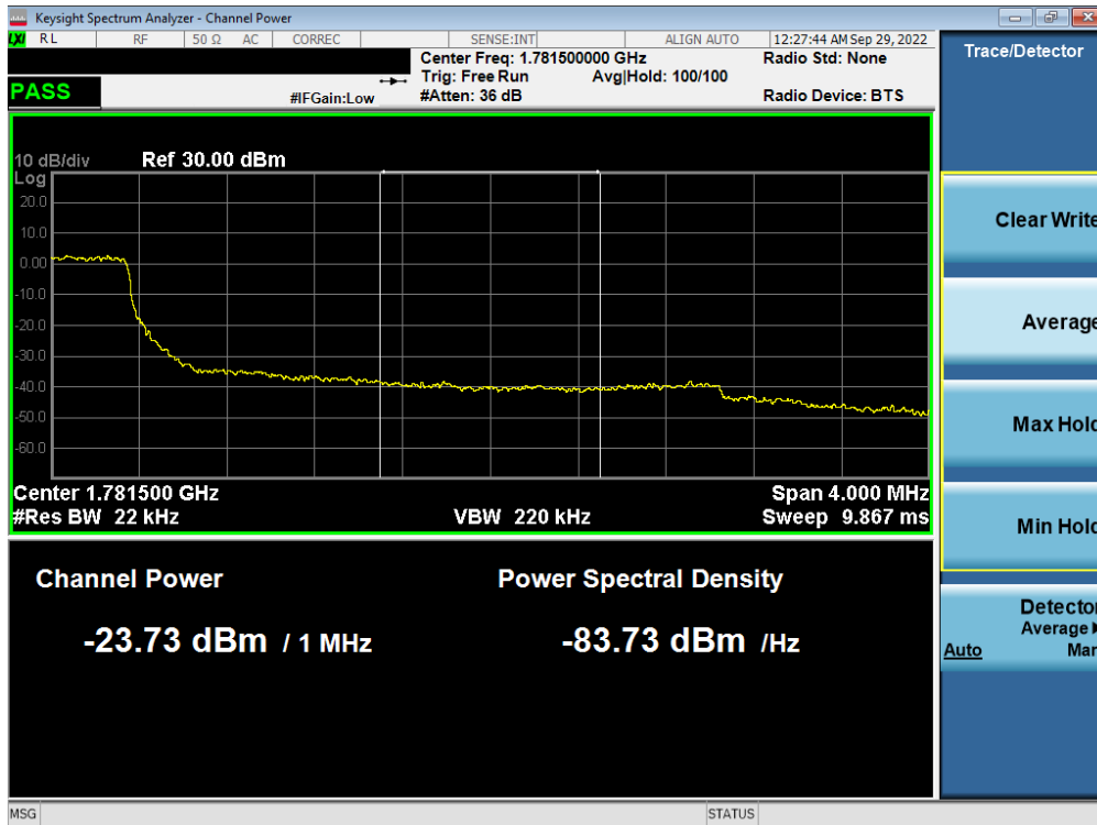
Plot 7-352. Upper Extended Band Edge Plot (LTE Band 66 - 3MHz QPSK – Full RB - Ant F)
