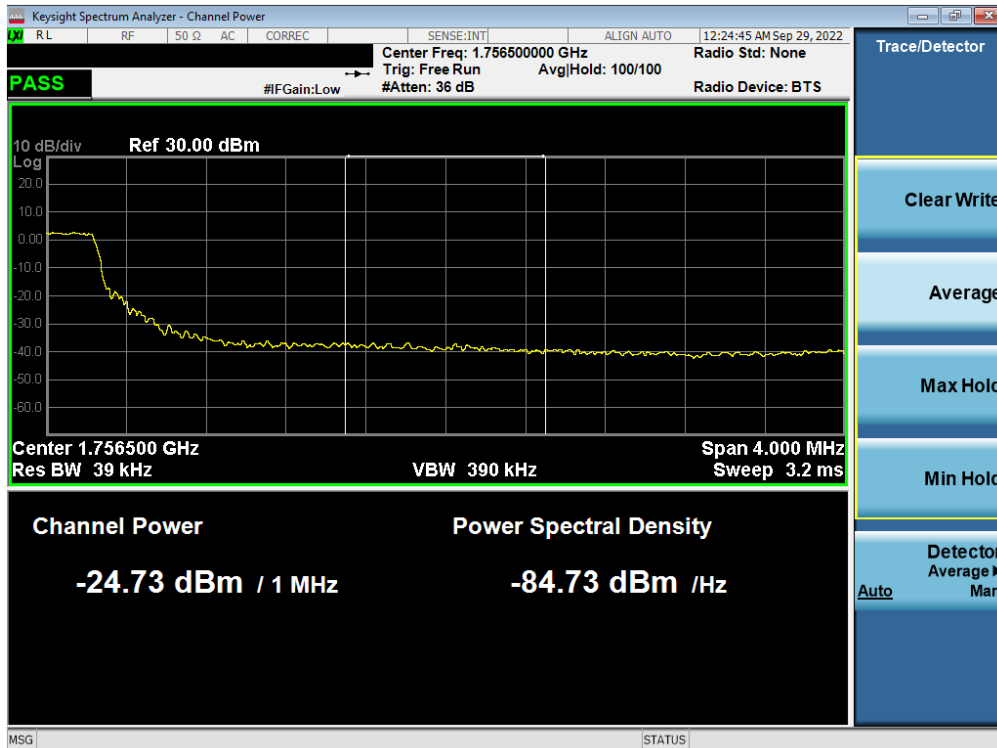
Plot 7-344. Upper Extended Band Edge Plot (LTE Band 4 - 5MHz QPSK – Full RB - Ant F)
