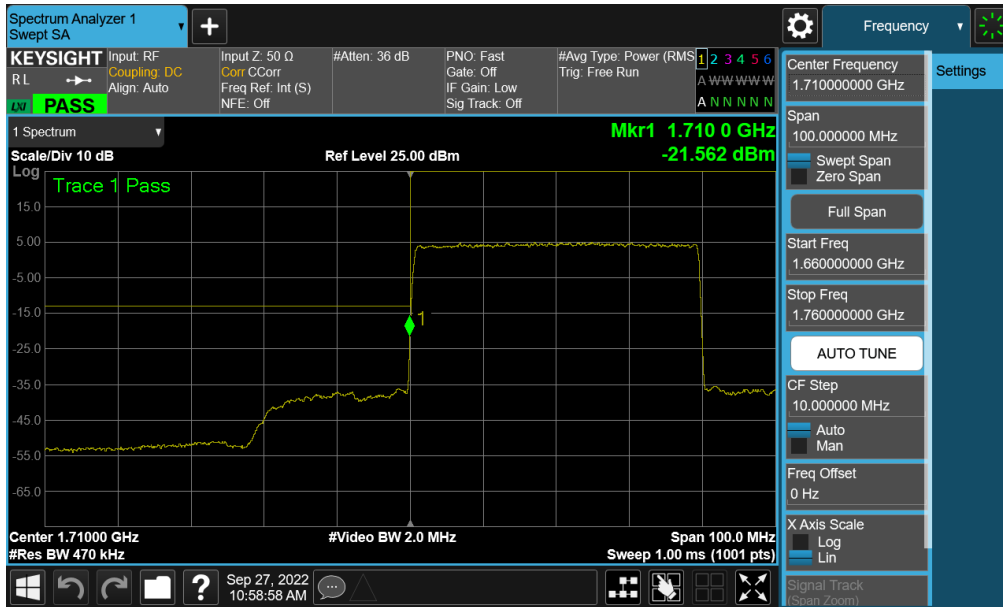
Plot 7-359. Lower Band Edge Plot (NR Band n66 – 40.0MHz - Full RB - Ant F)
