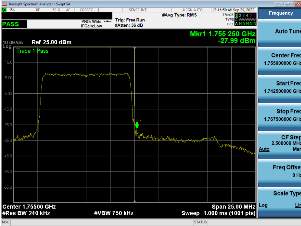
Plot 7-337. Upper Band Edge Plot (LTE Band 4 - 10MHz QPSK – Full RB - Ant F)
