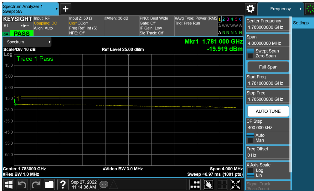
Plot 7-366. Upper Extended Band Edge Plot (NR Band n66 – 30.0MHz - Full RB - Ant F)
