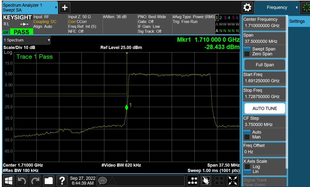
Plot 7-307. Lower Band Edge Plot (NR Band n66 – 15.0MHz - Full RB - ANT A)
