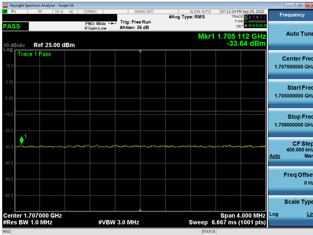
Plot 7-320. Lower Extended Band Edge Plot (ULCA LTE Band 66 - ANT A)
