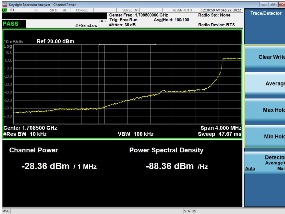
Plot 7-354. Lower Extended Band Edge Plot (LTE Band 66/4 – 1.4MHz QPSK – Full RB - Ant F)
