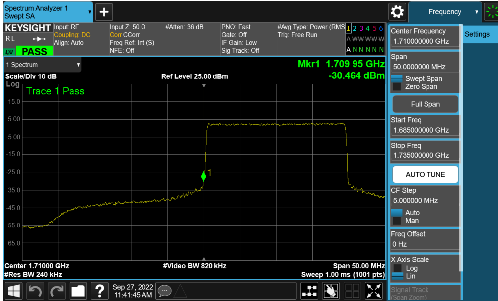
Plot 7-371. Lower Band Edge Plot (NR Band n66 – 20.0MHz - Full RB - Ant F)
