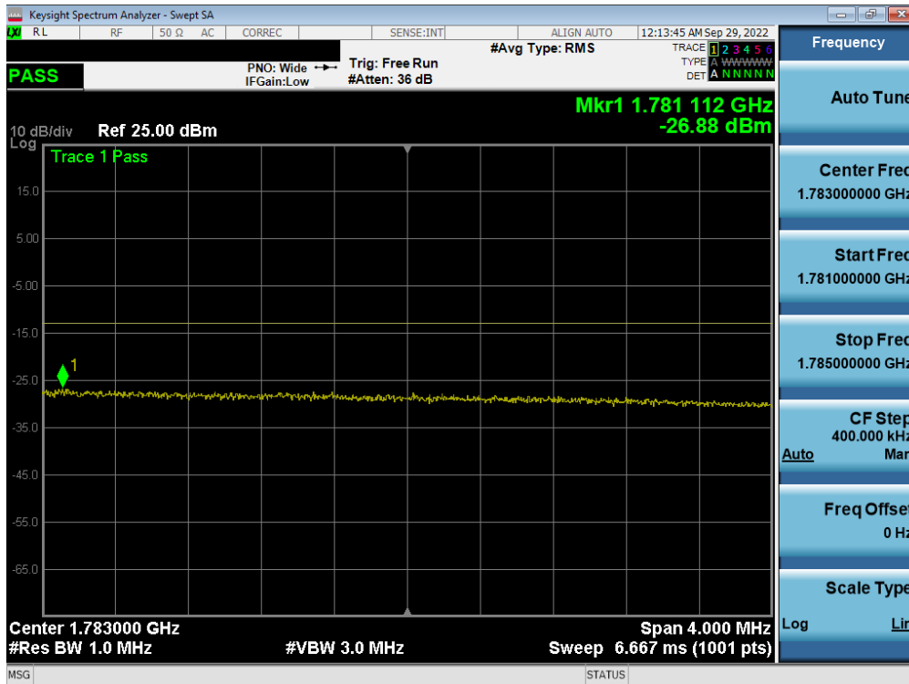
Plot 7-334. Upper Extended Band Edge Plot (LTE Band 66 - 15MHz QPSK – Full RB - Ant F)
