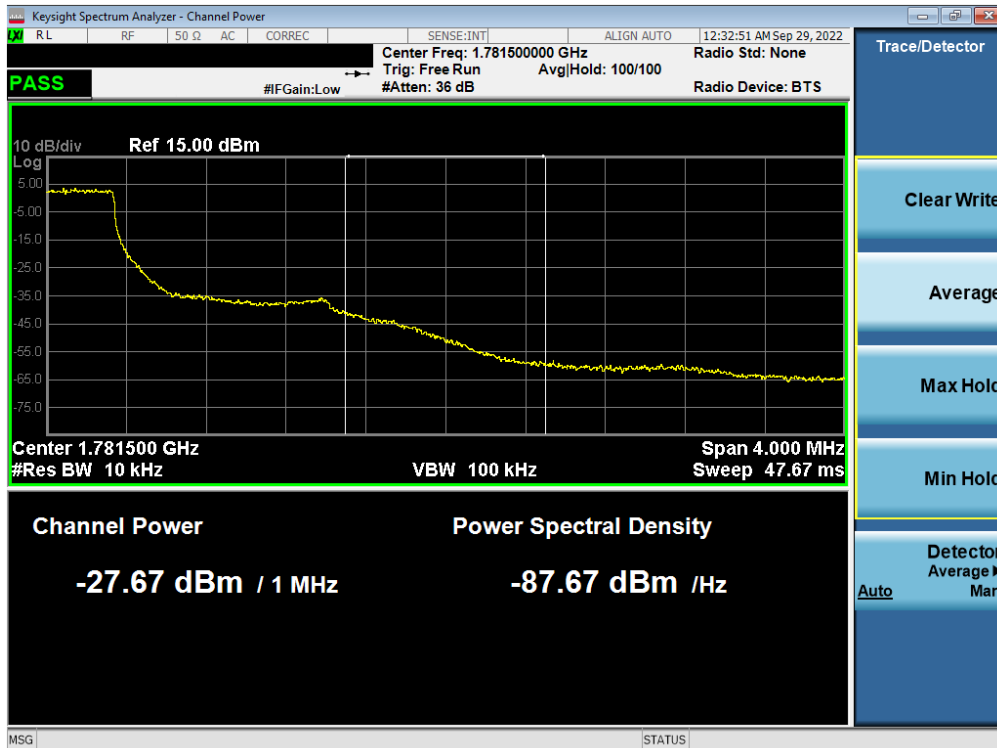
Plot 7-358. Upper Extended Band Edge Plot (LTE Band 66 – 1.4MHz QPSK – Full RB - Ant F)
