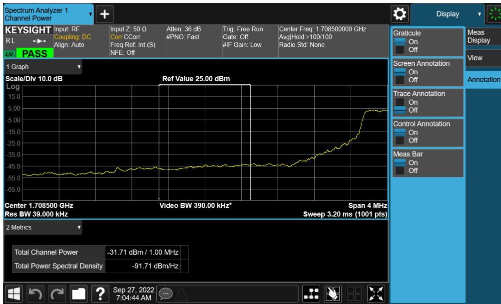
Plot 7-316. Lower Extended Band Edge Plot (NR Band n66 – 5.0MHz - Full RB - ANT A)
