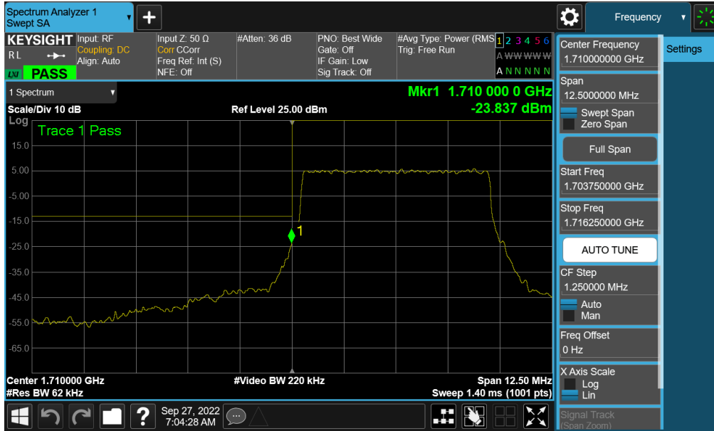
Plot 7-315. Lower Band Edge Plot (NR Band n66 – 5.0MHz - Full RB - ANT A)
