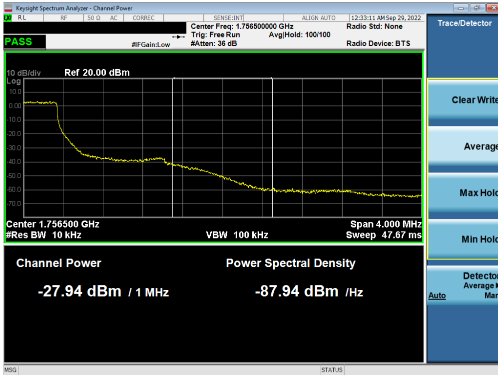
Plot 7-356. Upper Extended Band Edge Plot (LTE Band 4 – 1.4MHz QPSK – Full RB - Ant F)
