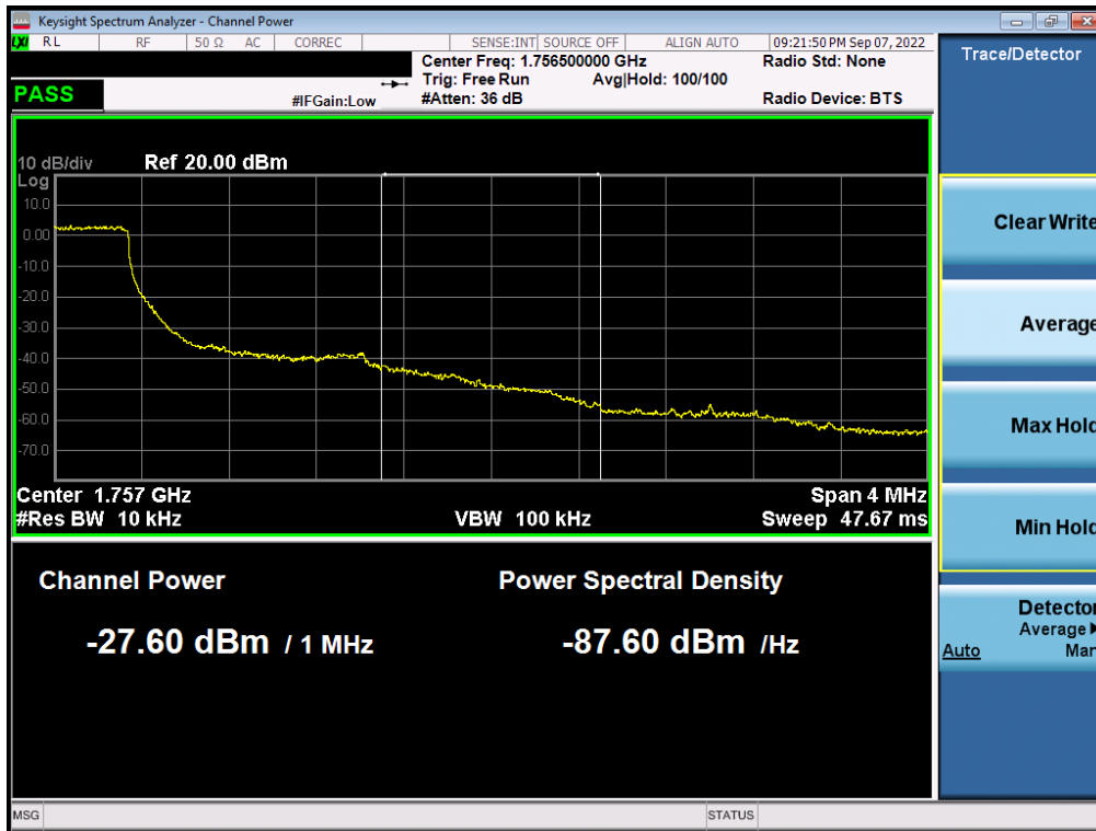
Plot 7-288. Upper Extended Band Edge Plot (LTE Band 4 – 1.4MHz QPSK – Full RB - ANT A)
