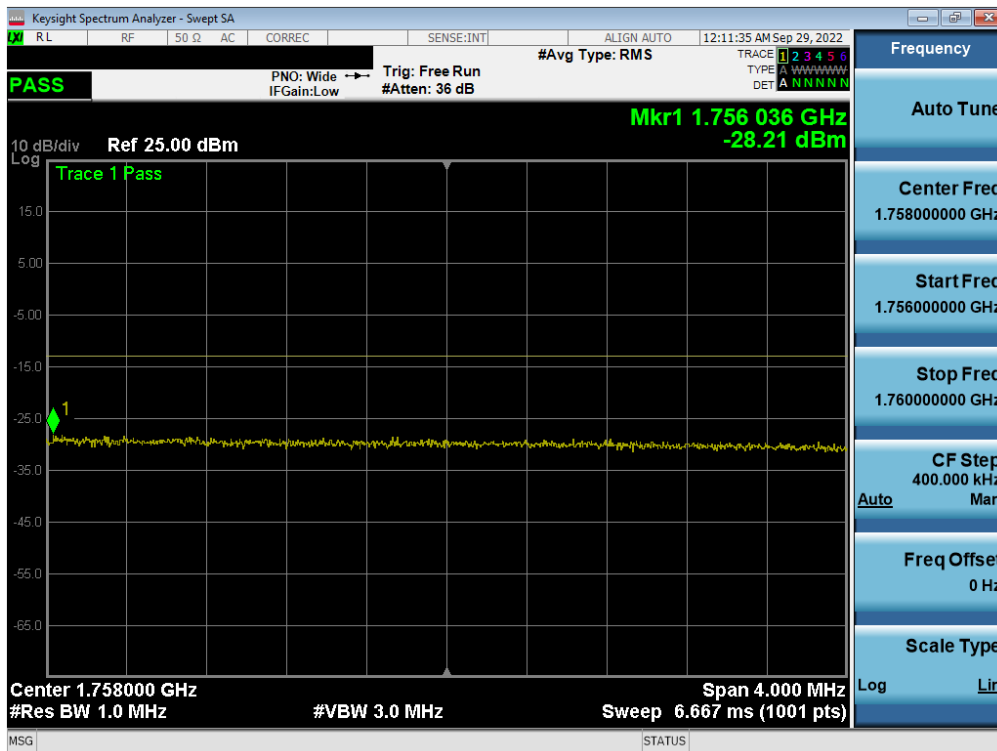
Plot 7-326. Upper Extended Band Edge Plot (LTE Band 4 - 20MHz QPSK – Full RB - Ant F)
