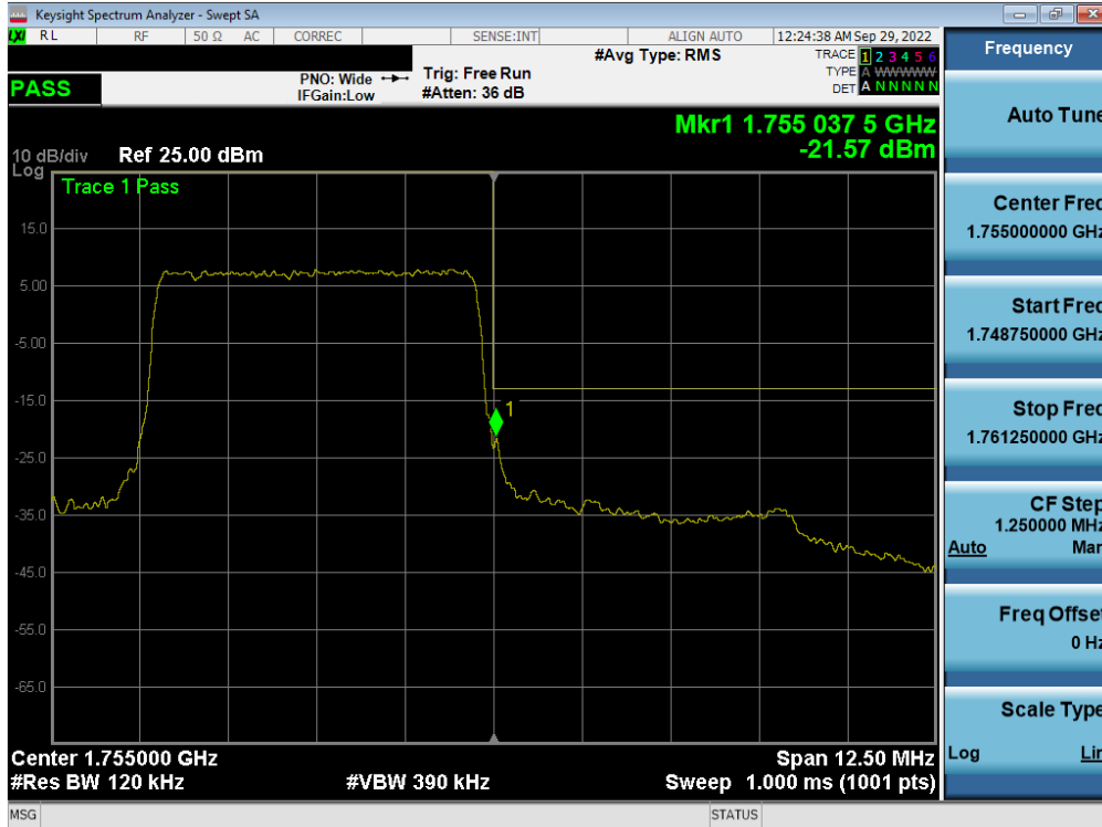
Plot 7-343. Upper Band Edge Plot (LTE Band 4 - 5MHz QPSK – Full RB - Ant F)
