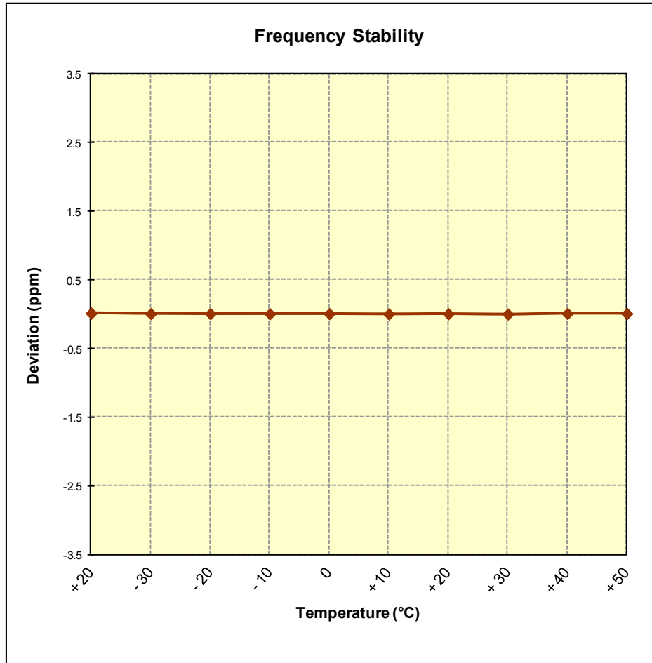
Figure 6-9. Frequency Stability Graph (PCS GSM Mode – Ch. 661)
