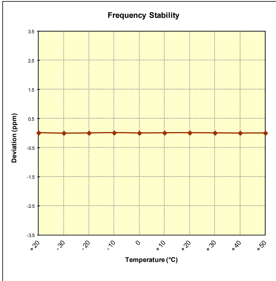
Figure 6-10. Frequency Stability Graph (PCS WCDMA Mode – Ch. 9400)
