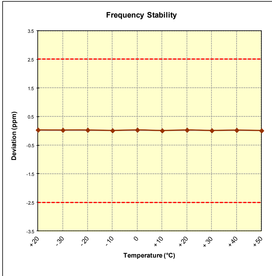
Figure 6-7. Frequency Stability Graph (Cellular GSM Mode – Ch. 190)
