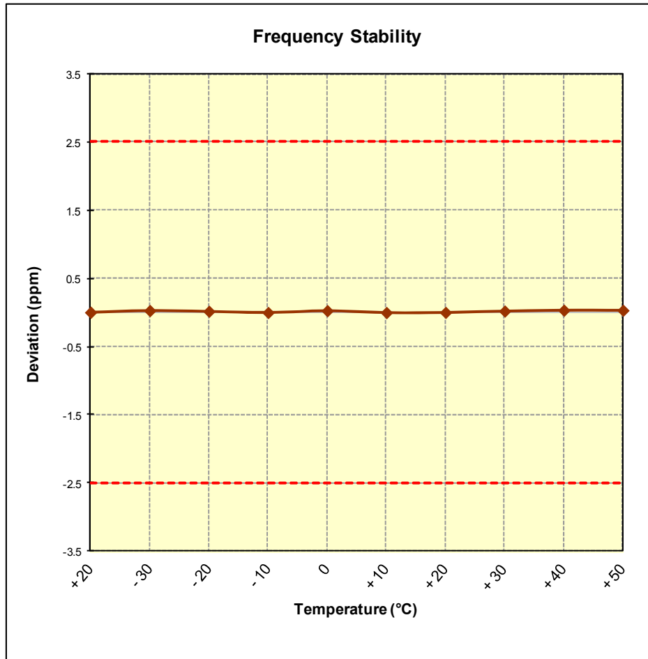
Figure 6-8. Frequency Stability Graph (Cellular WCDMA Mode – Ch. 4183)
