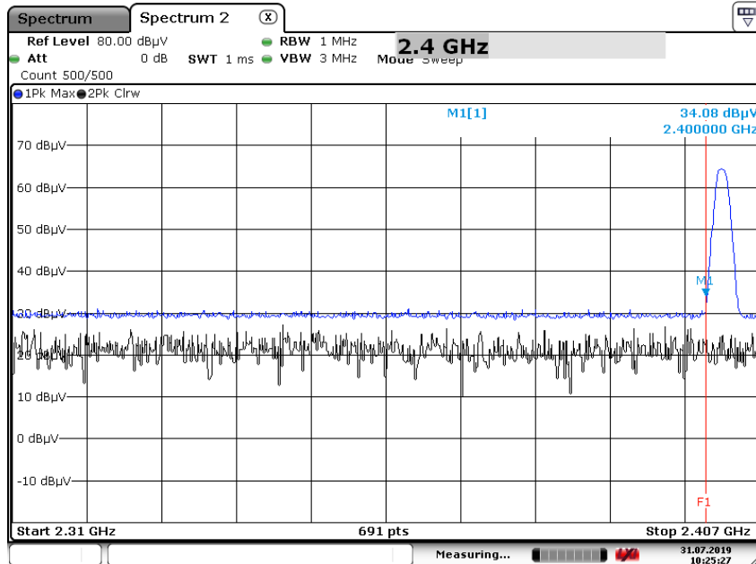
Radiated Band Edges plot – Peak Reading (Ch.0)
