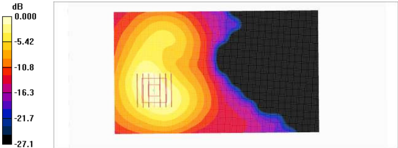
0 dB = 0.521mW/g
