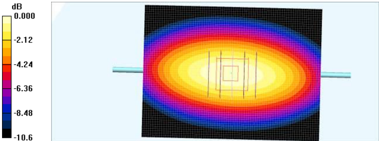
0 dB = 0.995mW/g
