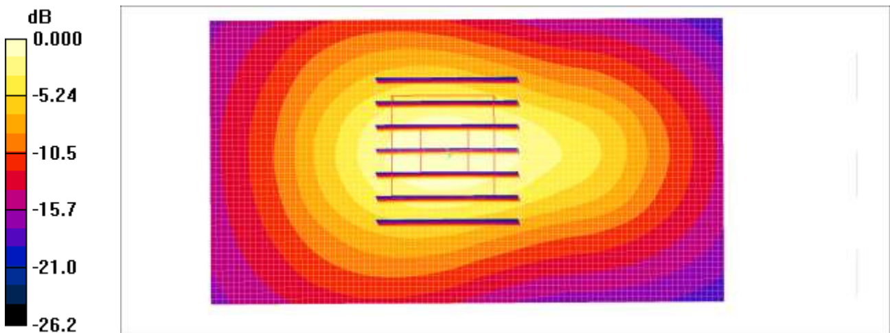
0 dB = 1.63mW/g
