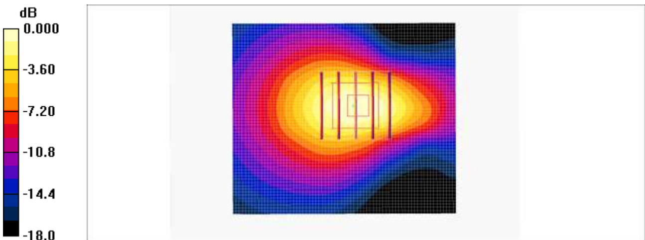
0 dB = 0.679mW/g
