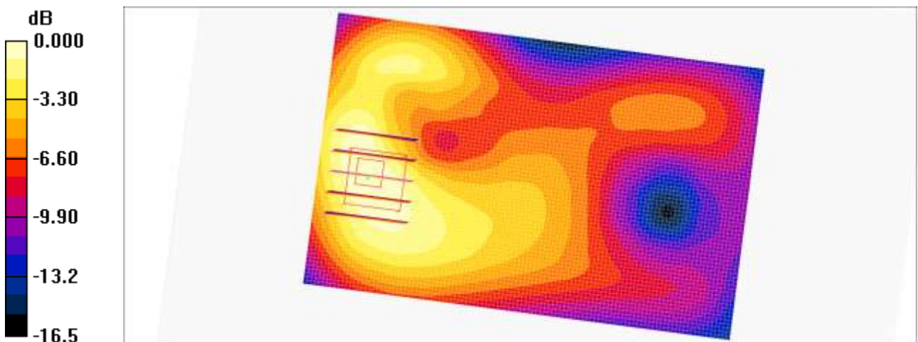
0 dB = 0.376mW/g
