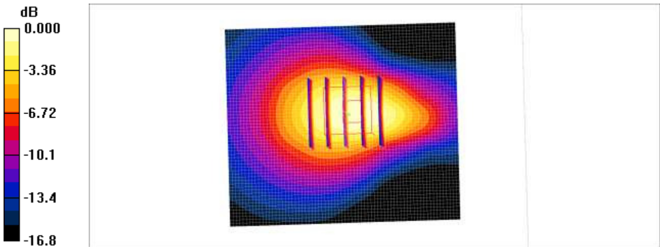
0 dB = 1.08mW/g
