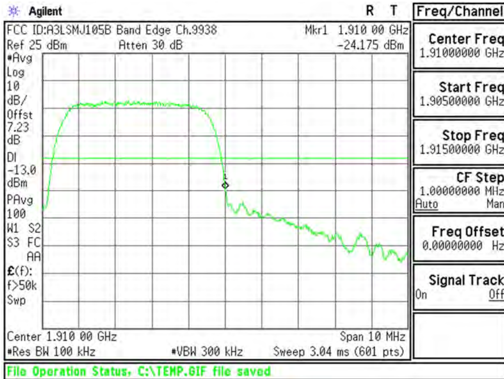
Plot 6-33. Upper Band Edge Plot (PCS WCDMA Mode - Ch.9538(DL9938))
