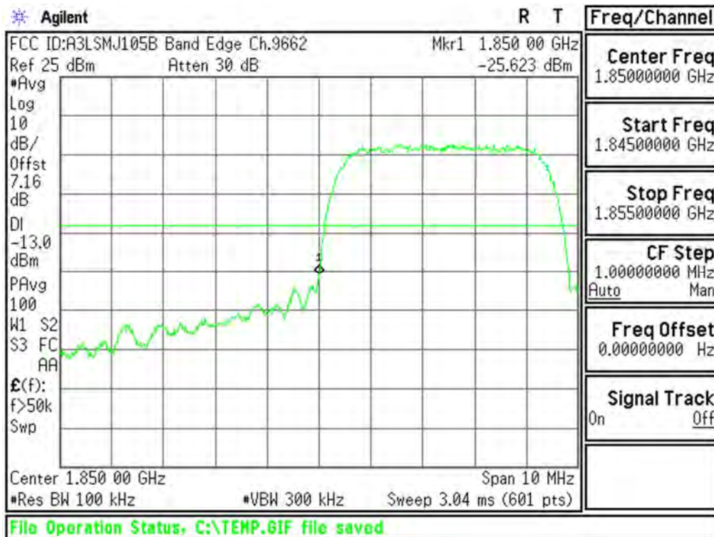
Plot 6-31. Lower Band Edge Plot (PCS WCDMA Mode - Ch.9262(DL9662))
