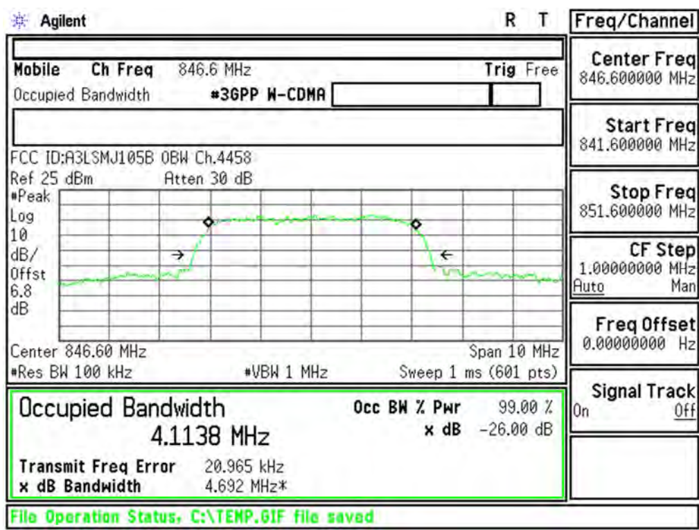
Plot 6-1. Occupied Bandwidth Plot (Cellular WCDMA Mode - Ch.4233(DL4458))
