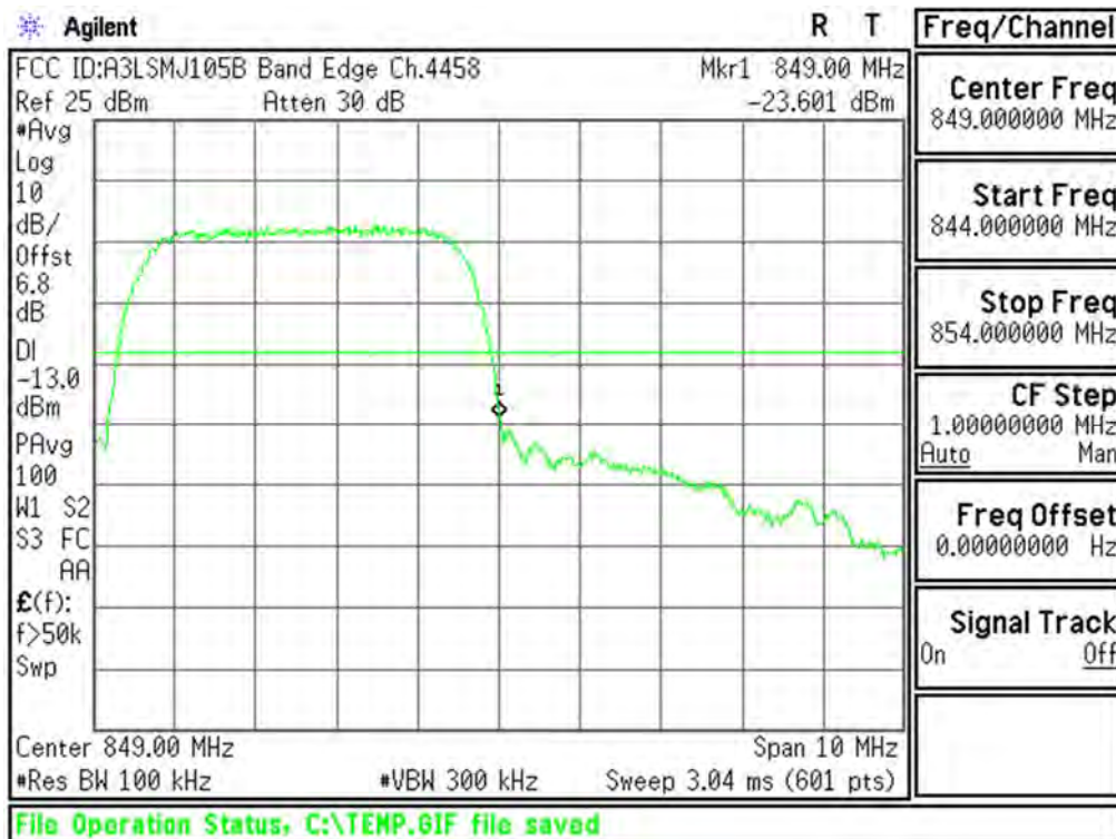
Plot 6-29. Upper Band Edge Plot (Cellular WCDMA Mode - Ch.4233(DL4458))
