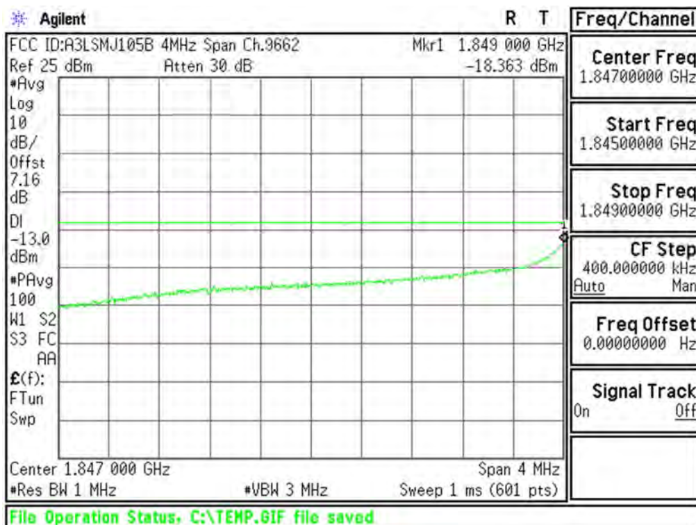
Plot 6-32. Extended Lower Band Edge Plot (PCS WCDMA Mode - Ch.9262(DL9662))
