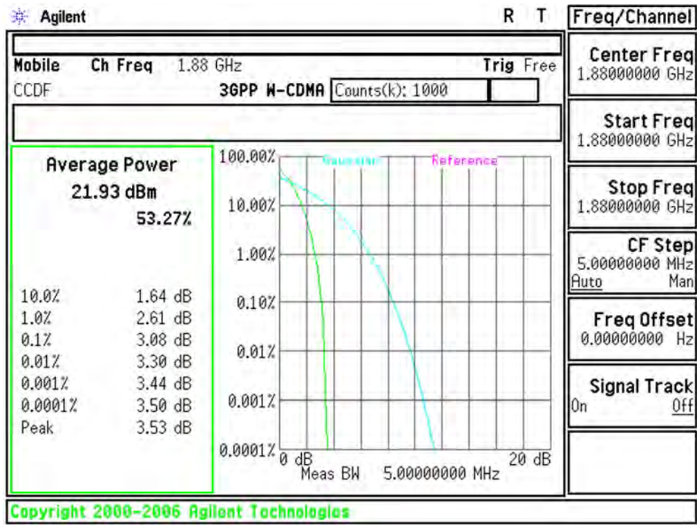
Plot 6-35. Peak-Average Ratio Plot (PCS WCDMA Mode - Ch.9400(DL9800))
