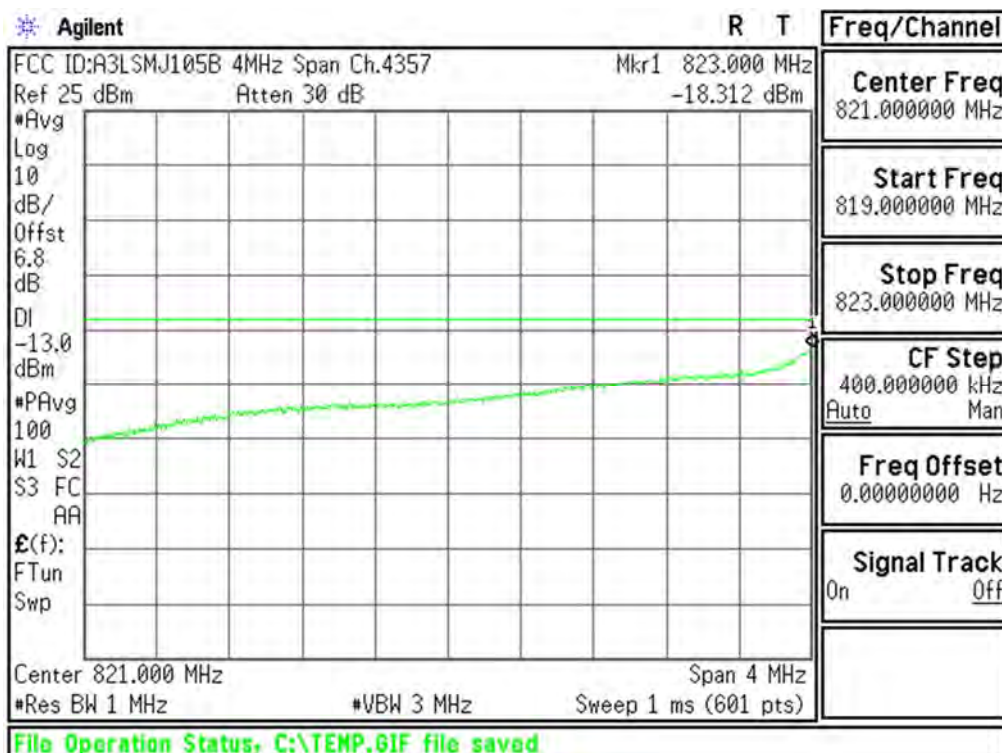
Plot 6-28. Extended Lower Band Edge Plot (Cellular WCDMA Mode - Ch.4132(DL4357))
