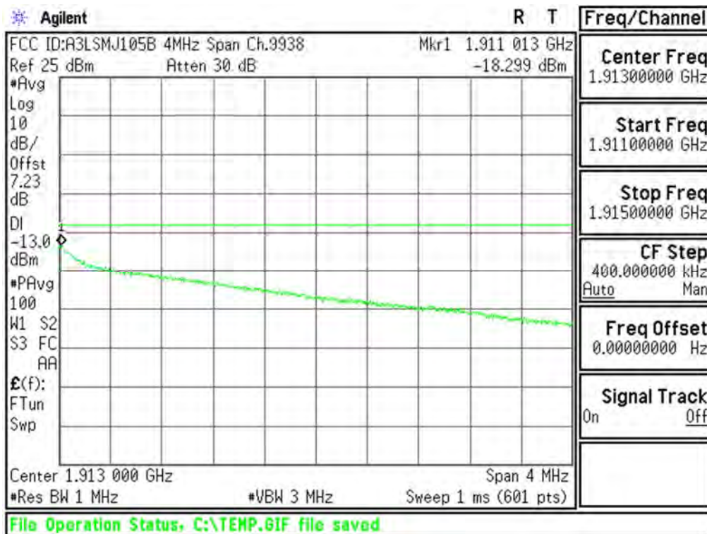
Plot 6-34. Extended Upper Band Edge Plot (PCS WCDMA Mode - Ch.9538(DL9938))
