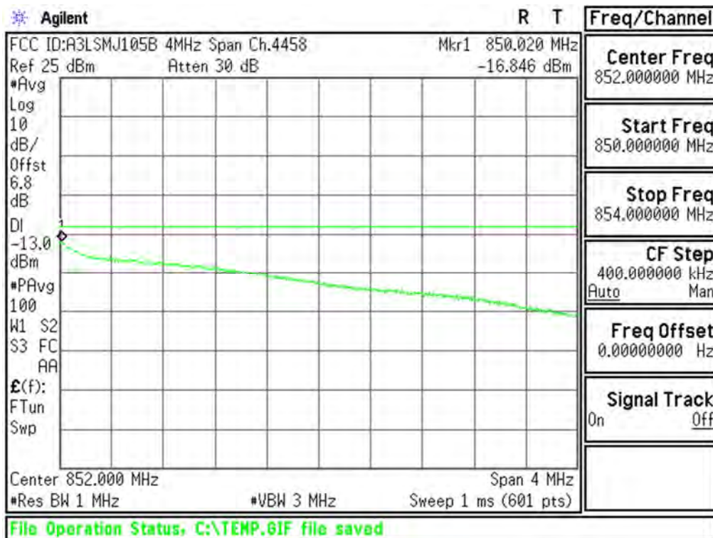
Plot 6-30. Extended Upper Band Edge Plot (Cellular WCDMA Mode - Ch.4233(DL4458))
