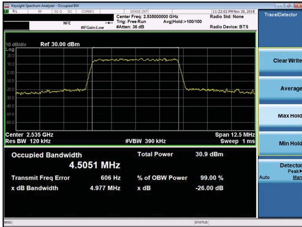
Plot 7-117. Occupied Bandwidth Plot (Band 7 ANT B – 5.0MHz QPSK - Full RB Configuration)
