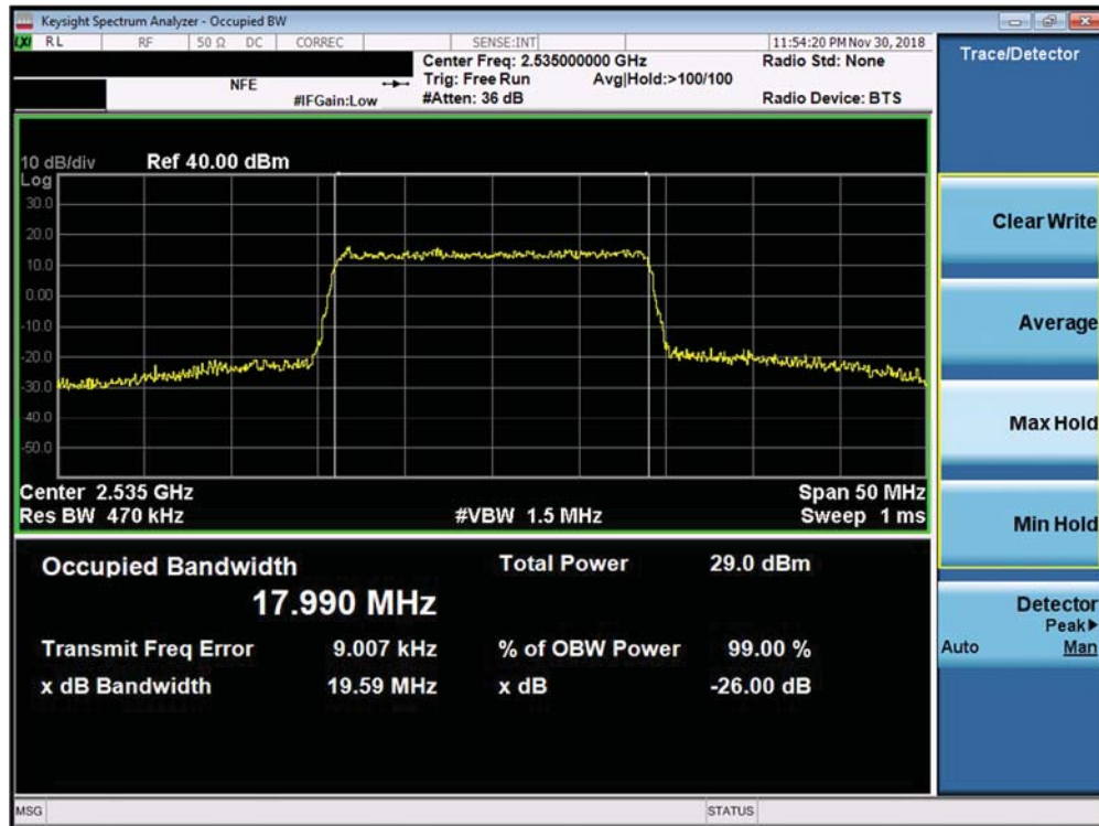
Plot 7-131. Occupied Bandwidth Plot (Band 7 ANT B - 20.0MHz 64-QAM - Full RB Configuration)
