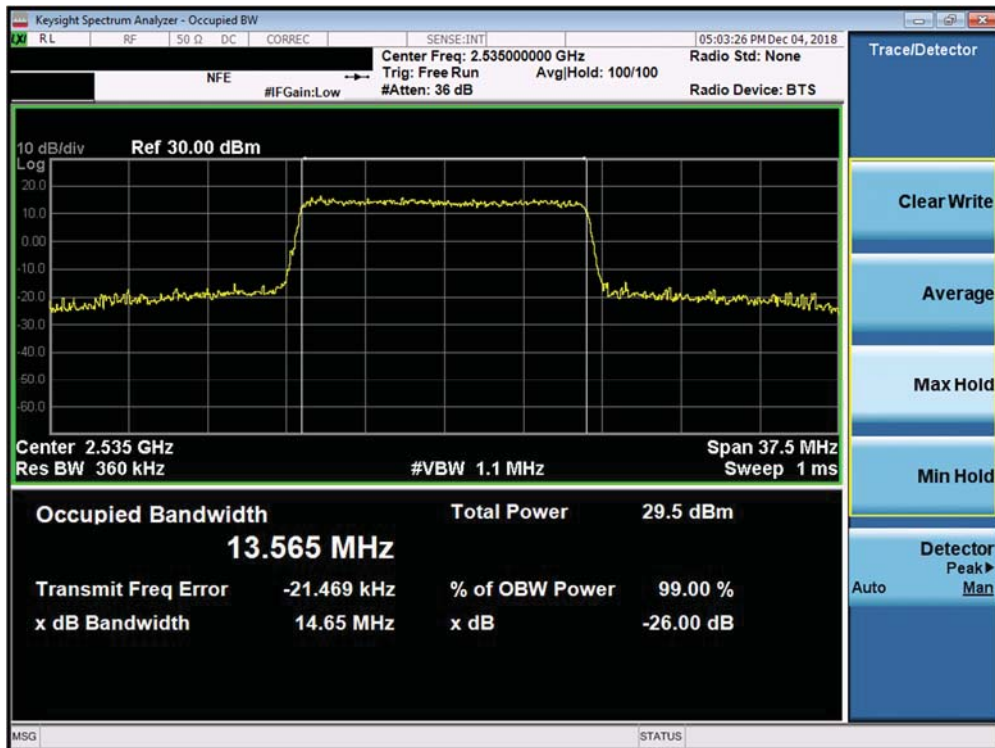
Plot 7-142. Occupied Bandwidth Plot (Band 7 Ant A - 15.0MHz 16-QAM - Full RB Configuration)
