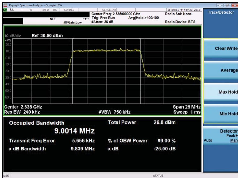
Plot 7-124. Occupied Bandwidth Plot (Band 7 ANT B - 10.0MHz 256-QAM - Full RB Configuration)
