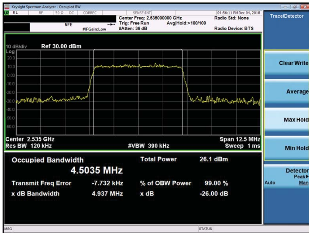
Plot 7-136. Occupied Bandwidth Plot (Band 7 Ant A – 5.0MHz 256-QAM - Full RB Configuration)
