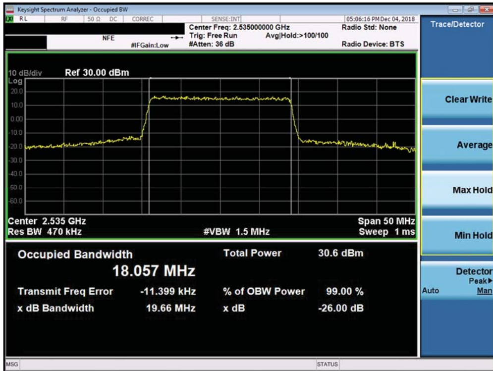
Plot 7-145. Occupied Bandwidth Plot (Band 7 Ant A - 20.0MHz QPSK - Full RB Configuration)
