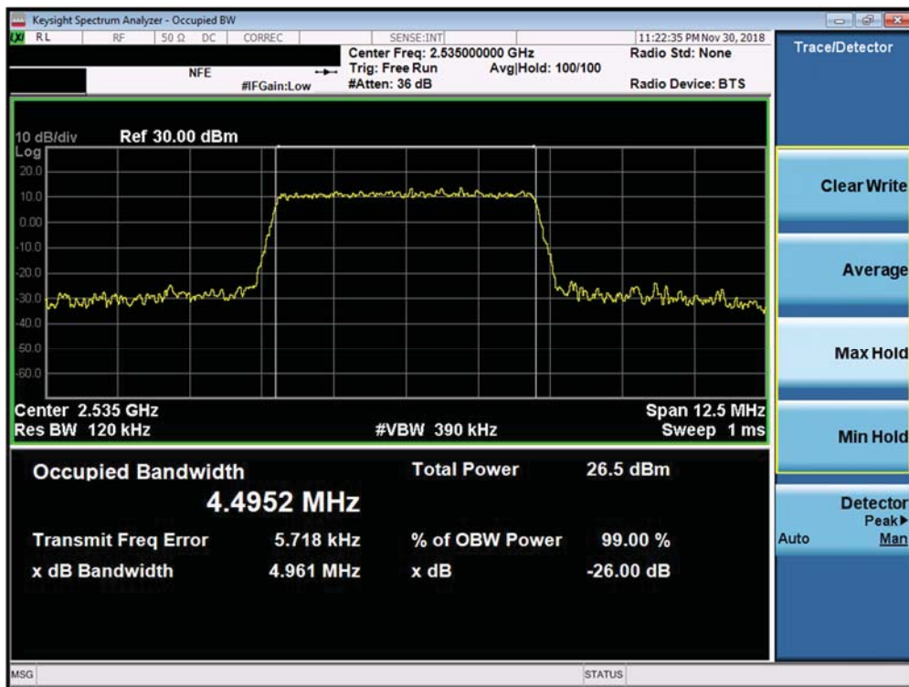
Plot 7-120. Occupied Bandwidth Plot (Band 7 ANT B – 5.0MHz 256-QAM - Full RB Configuration)
