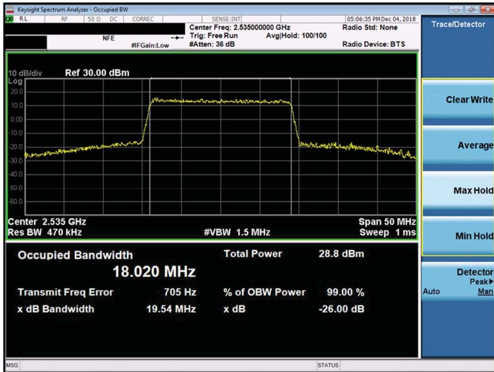
Plot 7-147. Occupied Bandwidth Plot (Band 7 Ant A - 20.0MHz 64-QAM - Full RB Configuration)
