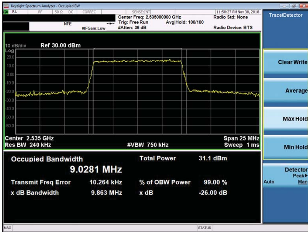
Plot 7-121. Occupied Bandwidth Plot (Band 7 ANT B - 10.0MHz QPSK - Full RB Configuration)
