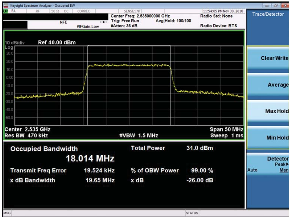
Plot 7-129. Occupied Bandwidth Plot (Band 7 ANT B - 20.0MHz QPSK - Full RB Configuration)
