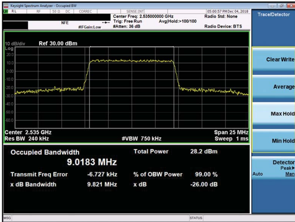
Plot 7-139. Occupied Bandwidth Plot (Band 7 Ant A - 10.0MHz 64-QAM - Full RB Configuration)
