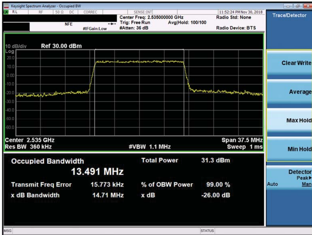
Plot 7-125. Occupied Bandwidth Plot (Band 7 ANT B - 15.0MHz QPSK - Full RB Configuration)
