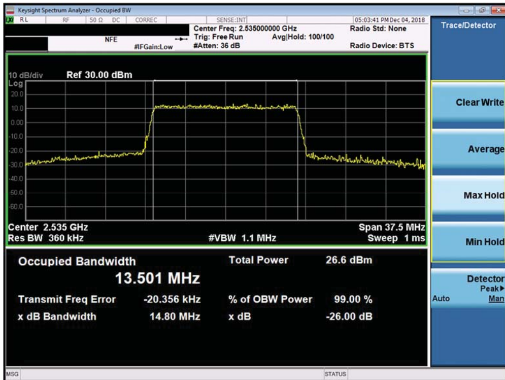
Plot 7-144. Occupied Bandwidth Plot (Band 7 Ant A - 15.0MHz 256-QAM - Full RB Configuration)
