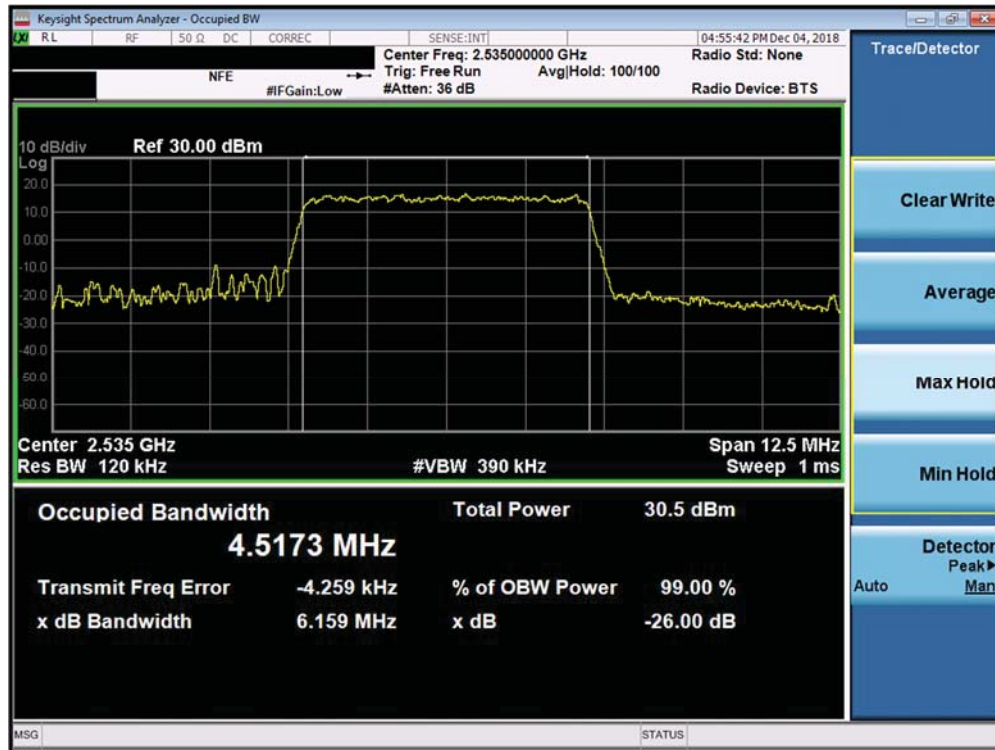
Plot 7-133. Occupied Bandwidth Plot (Band 7 Ant A – 5.0MHz QPSK - Full RB Configuration)
