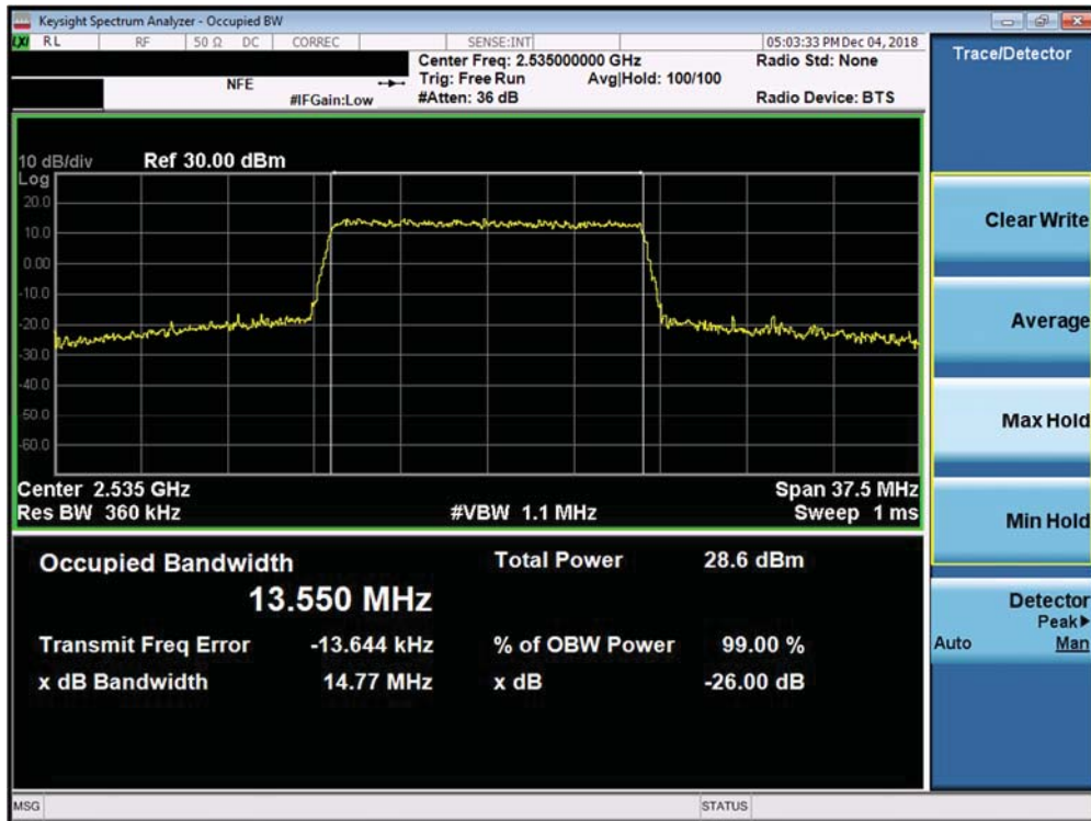
Plot 7-143. Occupied Bandwidth Plot (Band 7 Ant A - 15.0MHz 64-QAM - Full RB Configuration)
