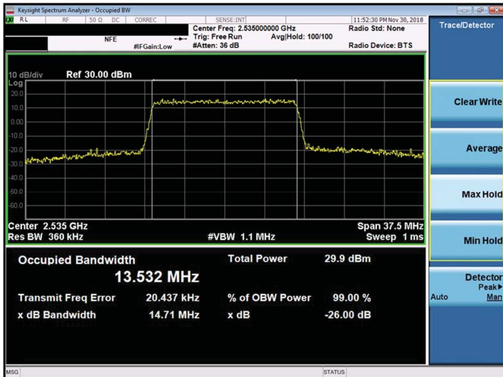
Plot 7-126. Occupied Bandwidth Plot (Band 7 ANT B - 15.0MHz 16-QAM - Full RB Configuration)
