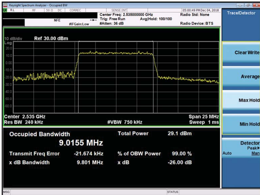
Plot 7-138. Occupied Bandwidth Plot (Band 7 Ant A - 10.0MHz 16-QAM - Full RB Configuration)
