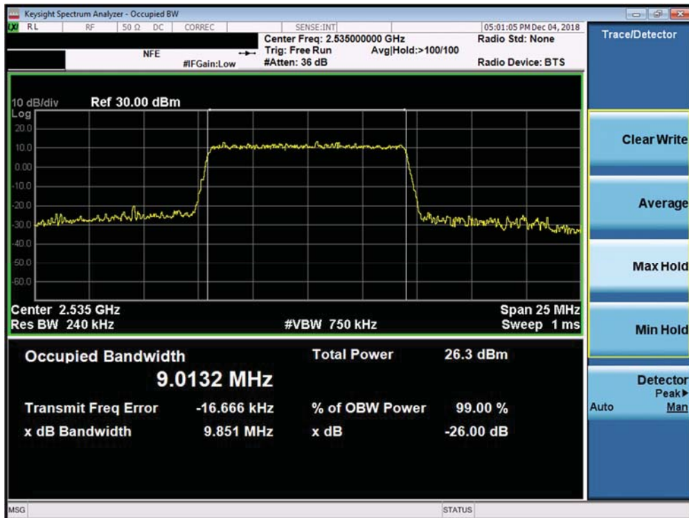
Plot 7-140. Occupied Bandwidth Plot (Band 7 Ant A - 10.0MHz 256-QAM - Full RB Configuration)
