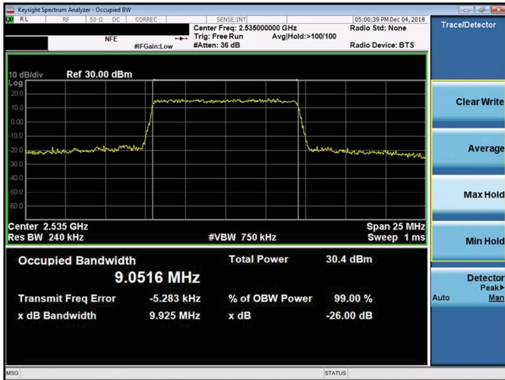
Plot 7-137. Occupied Bandwidth Plot (Band 7 Ant A - 10.0MHz QPSK - Full RB Configuration)
