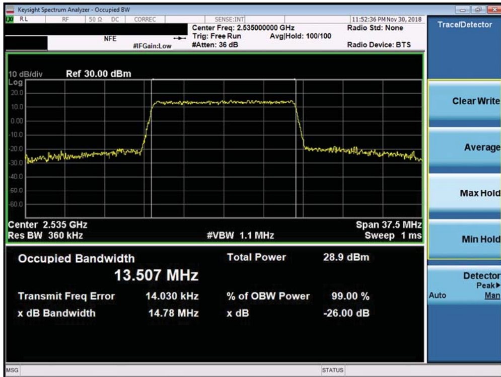
Plot 7-127. Occupied Bandwidth Plot (Band 7 ANT B - 15.0MHz 64-QAM - Full RB Configuration)
