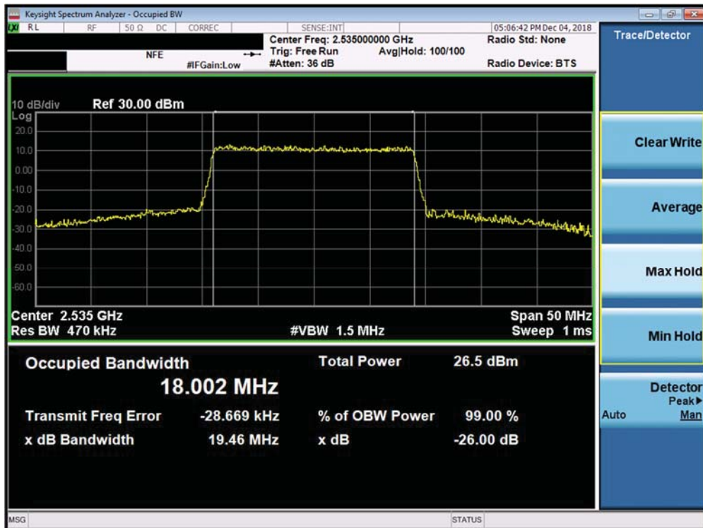
Plot 7-148. Occupied Bandwidth Plot (Band 7 Ant A - 20.0MHz 256-QAM - Full RB Configuration)
