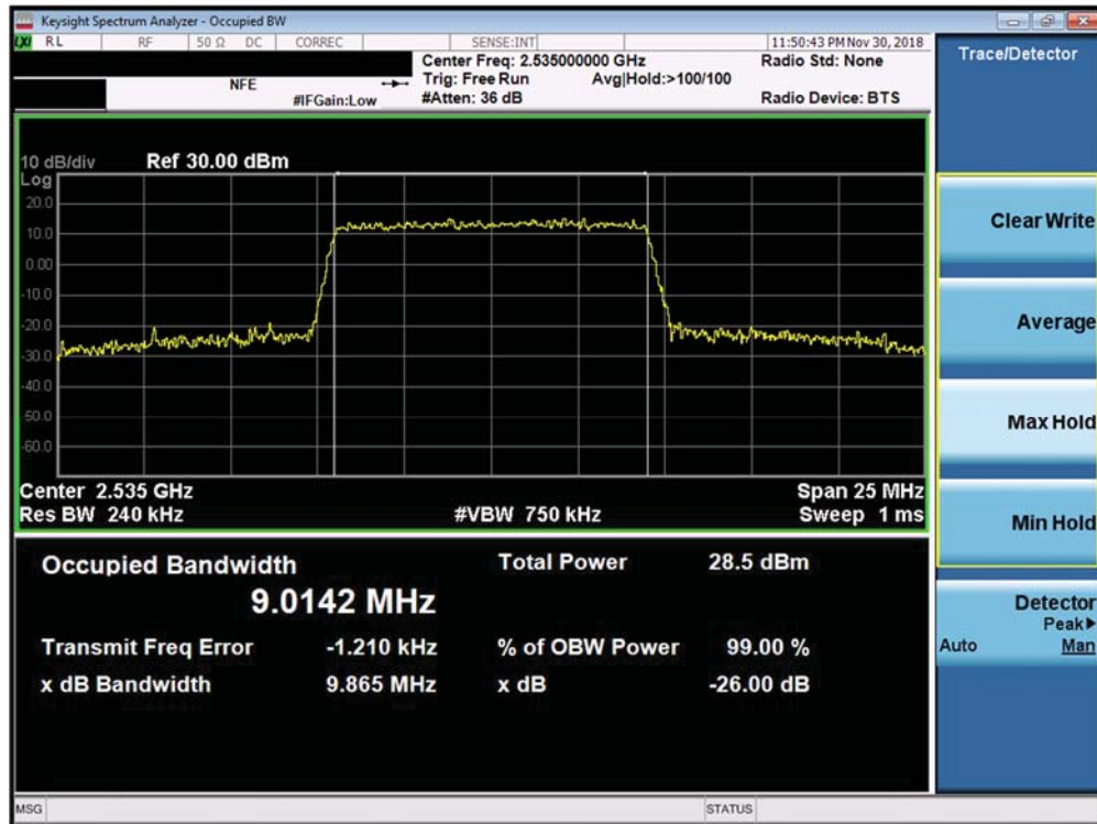
Plot 7-123. Occupied Bandwidth Plot (Band 7 ANT B - 10.0MHz 64-QAM - Full RB Configuration)
