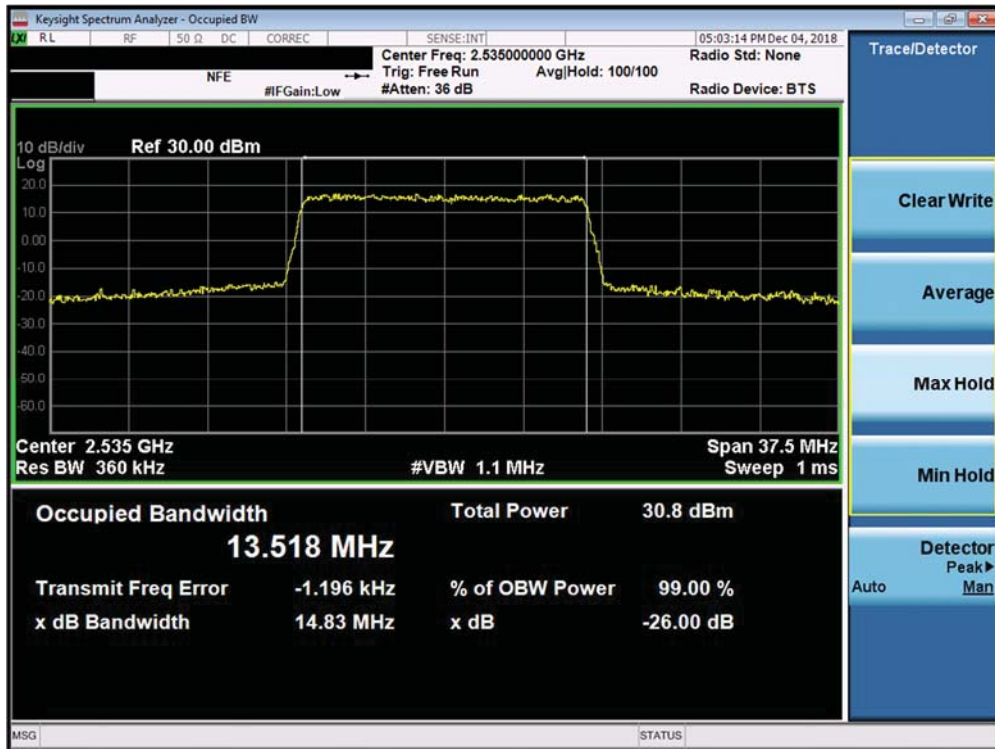
Plot 7-141. Occupied Bandwidth Plot (Band 7 Ant A - 15.0MHz QPSK - Full RB Configuration)
