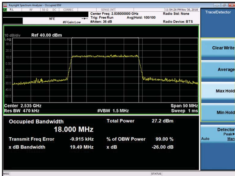
Plot 7-132. Occupied Bandwidth Plot (Band 7 ANT B - 20.0MHz 256-QAM - Full RB Configuration)
