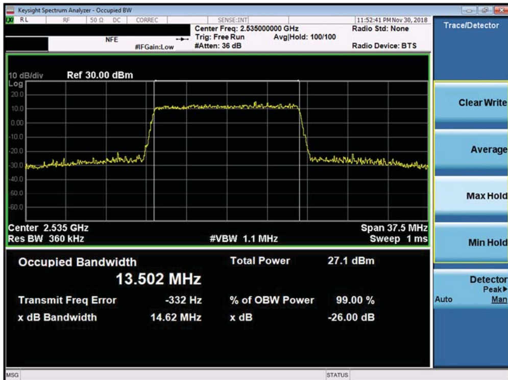
Plot 7-128. Occupied Bandwidth Plot (Band 7 ANT B - 15.0MHz 256-QAM - Full RB Configuration)
