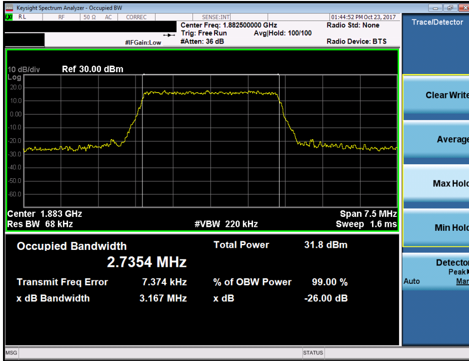
Plot 7-37. Occupied Bandwidth Plot (Band 25/2 - 3.0MHz QPSK - Full RB Configuration)
