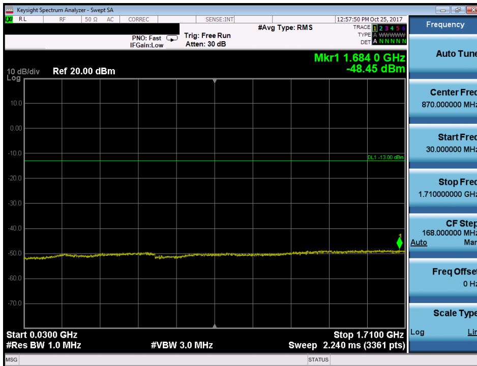
Plot 7-79. Conducted Spurious Plot (Band 66/4 - 5.0MHz QPSK - RB Size 1, RB Offset 0 - Mid Channel)
