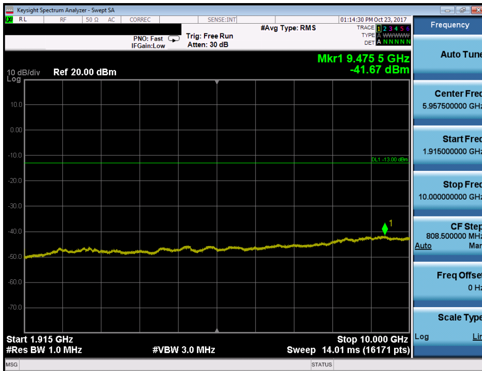
Plot 7-86. Conducted Spurious Plot (Band 25/2 - 10.0MHz QPSK - RB Size 1, RB Offset 0 - Low Channel)
