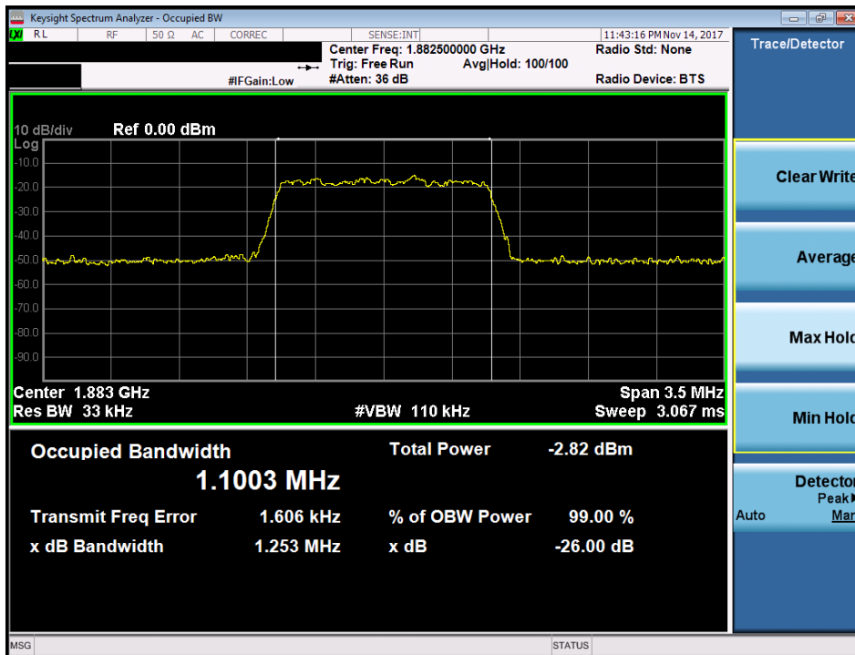
Plot 7-36. Occupied Bandwidth Plot (Band 25/2 - 1.4 MHz 16-QAM - Full RB Configuration)
