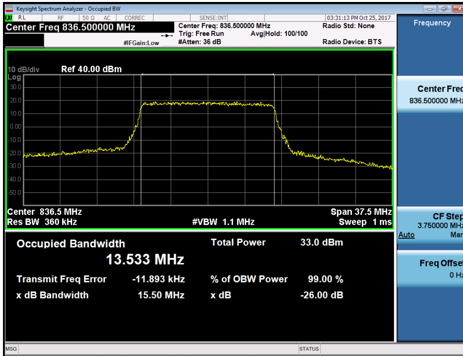
Plot 7-21. Occupied Bandwidth Plot (Band 26 - 15.0MHz QPSK - Full RB Configuration)
