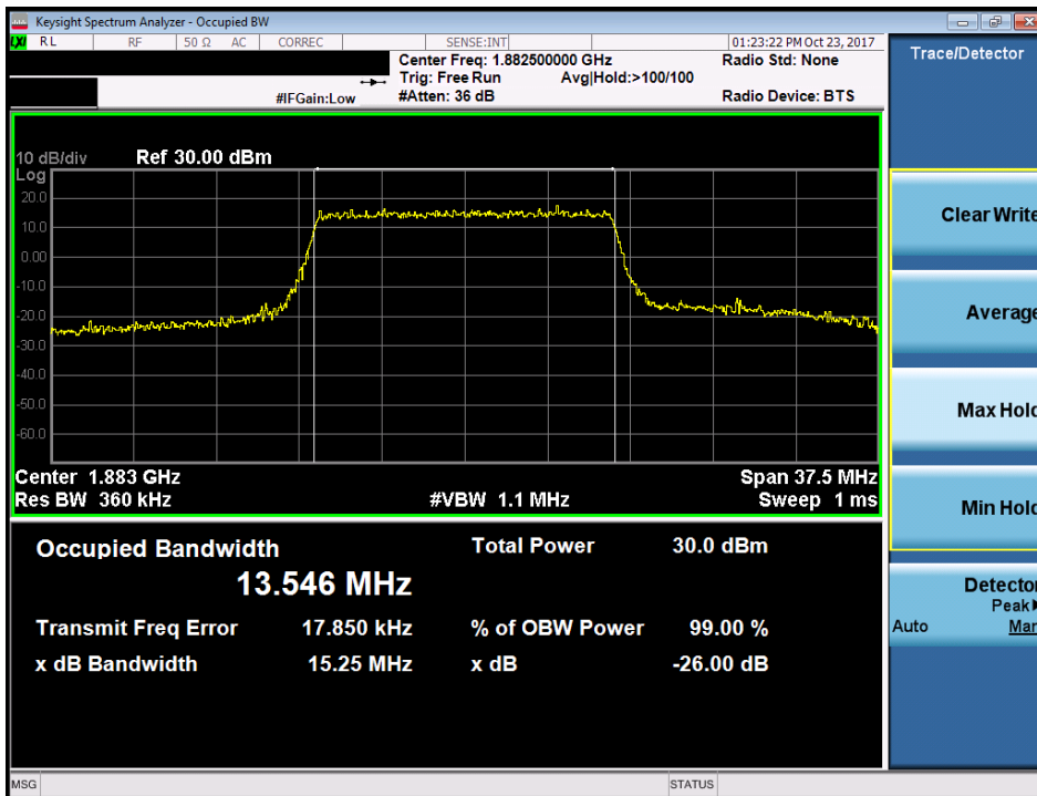
Plot 7-44. Occupied Bandwidth Plot (Band 25/2 - 15.0MHz 16-QAM - Full RB Configuration)
