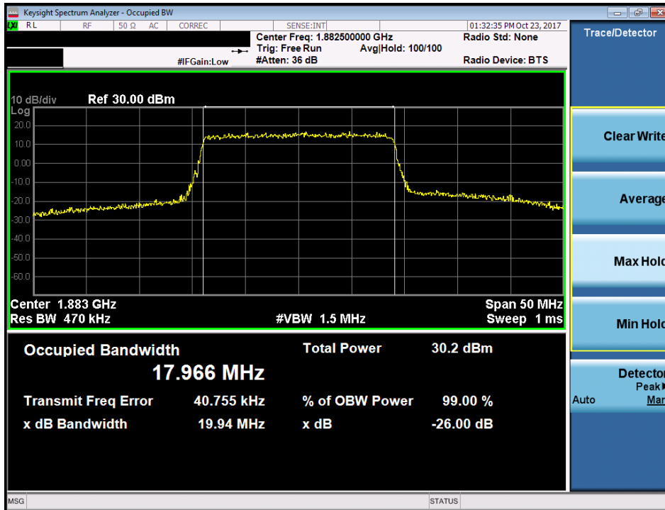
Plot 7-46. Occupied Bandwidth Plot (Band 25/2 - 20.0MHz 16-QAM - Full RB Configuration)
