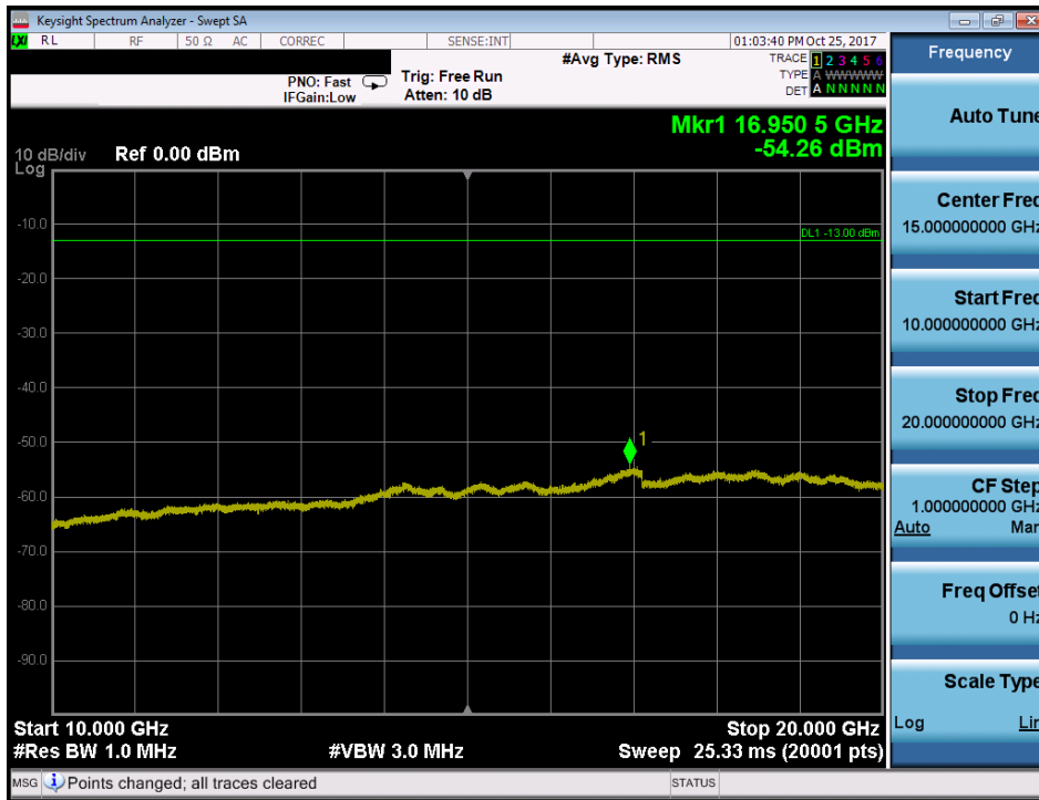
Plot 7-84. Conducted Spurious Plot (Band 66/4 - 5.0MHz QPSK - RB Size 1, RB Offset 0 - High Channel)
