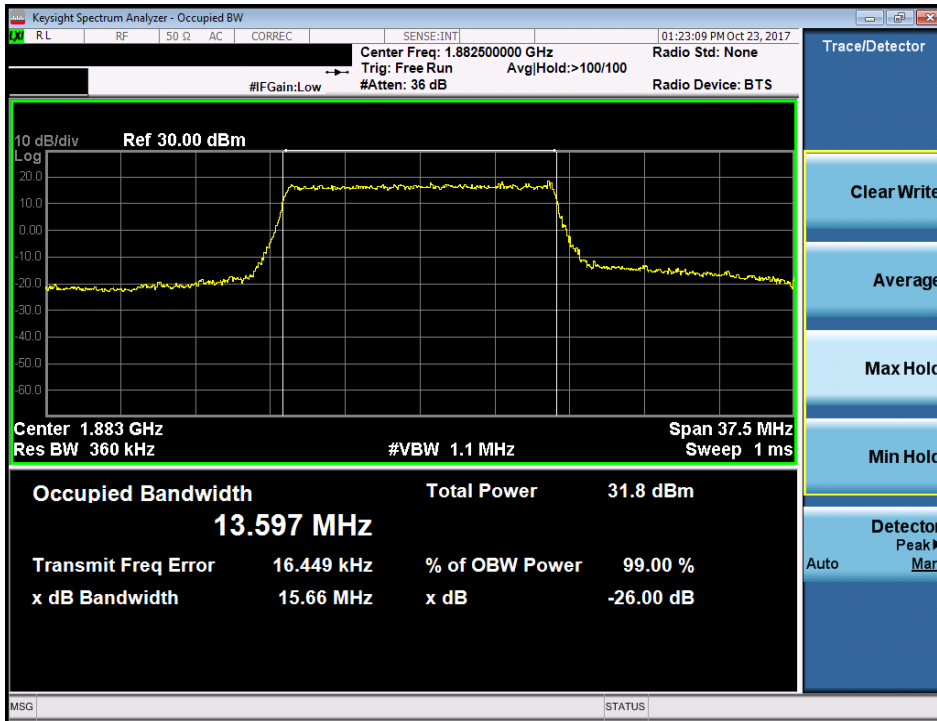
Plot 7-43. Occupied Bandwidth Plot (Band 25/2 - 15.0MHz QPSK - Full RB Configuration)
