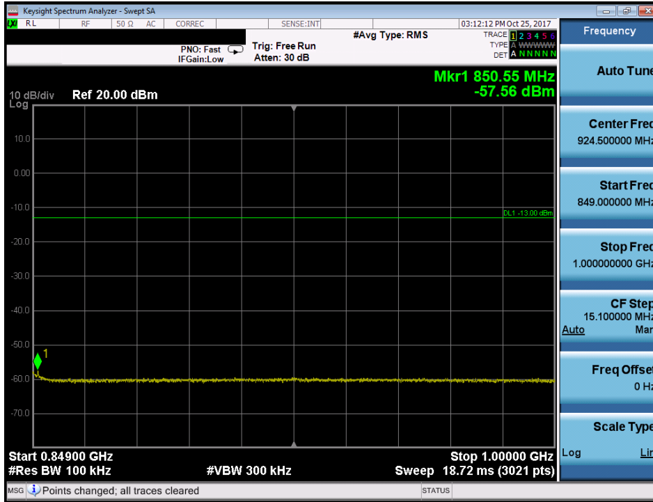
Plot 7-71. Conducted Spurious Plot (Band 26/5 - 3.0MHz QPSK - RB Size 1, RB Offset 0 - Mid Channel)
