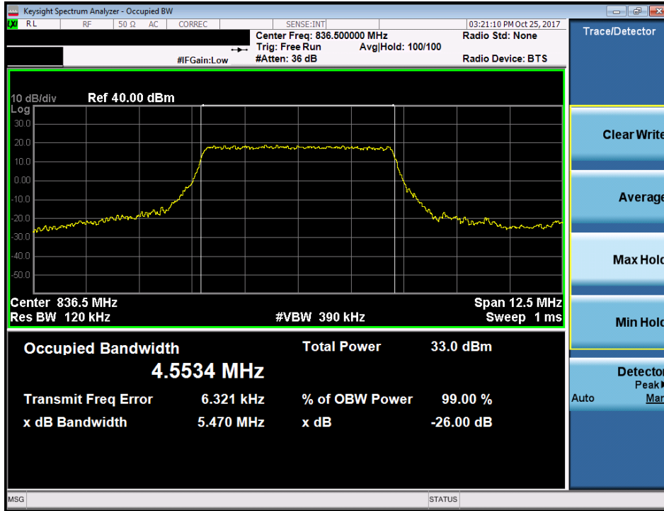
Plot 7-17. Occupied Bandwidth Plot (Band 26/5 - 5.0MHz QPSK - Full RB Configuration)
