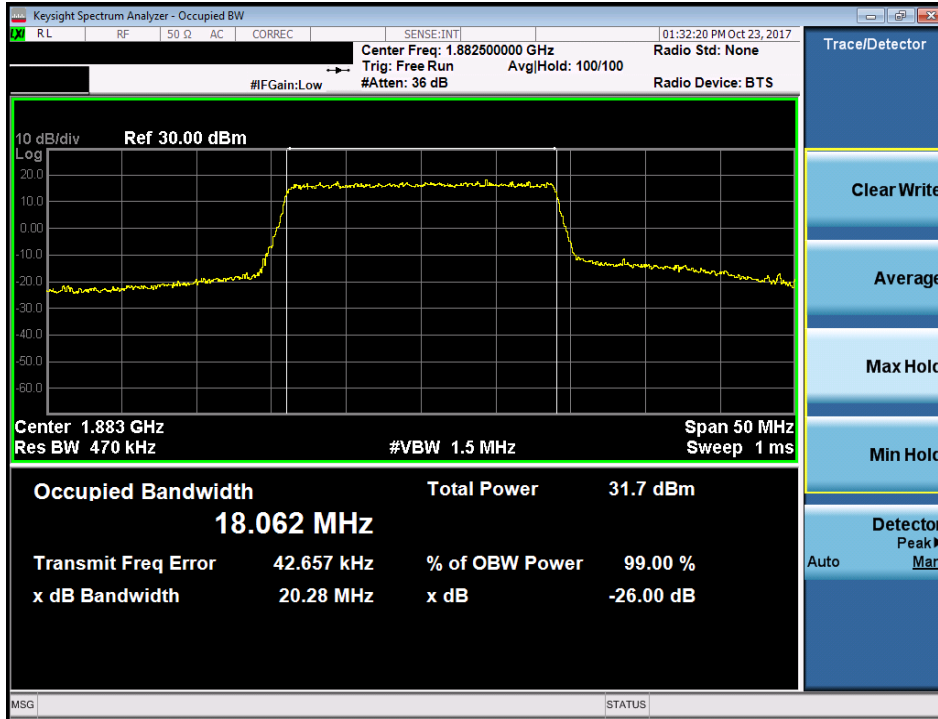
Plot 7-45. Occupied Bandwidth Plot (Band 25/2 - 20.0MHz QPSK - Full RB Configuration)
