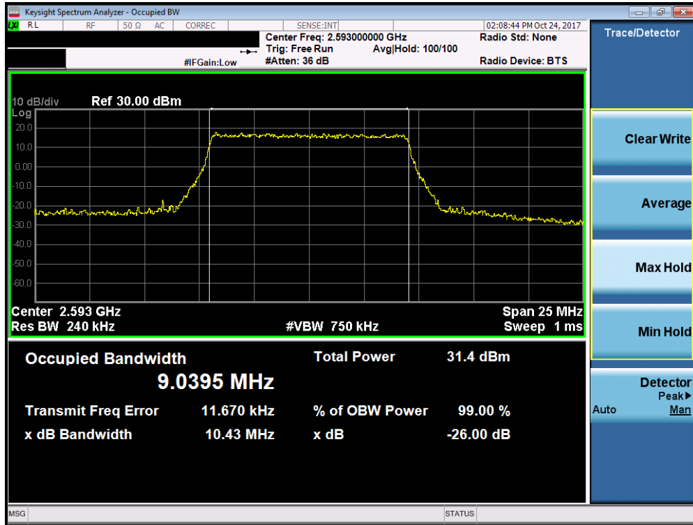
Plot 7-49. Occupied Bandwidth Plot (Band 41 - 10.0MHz QPSK - Full RB Configuration)
