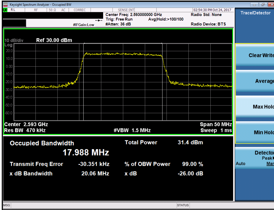
Plot 7-53. Occupied Bandwidth Plot (Band 41 - 20.0MHz QPSK - Full RB Configuration)
