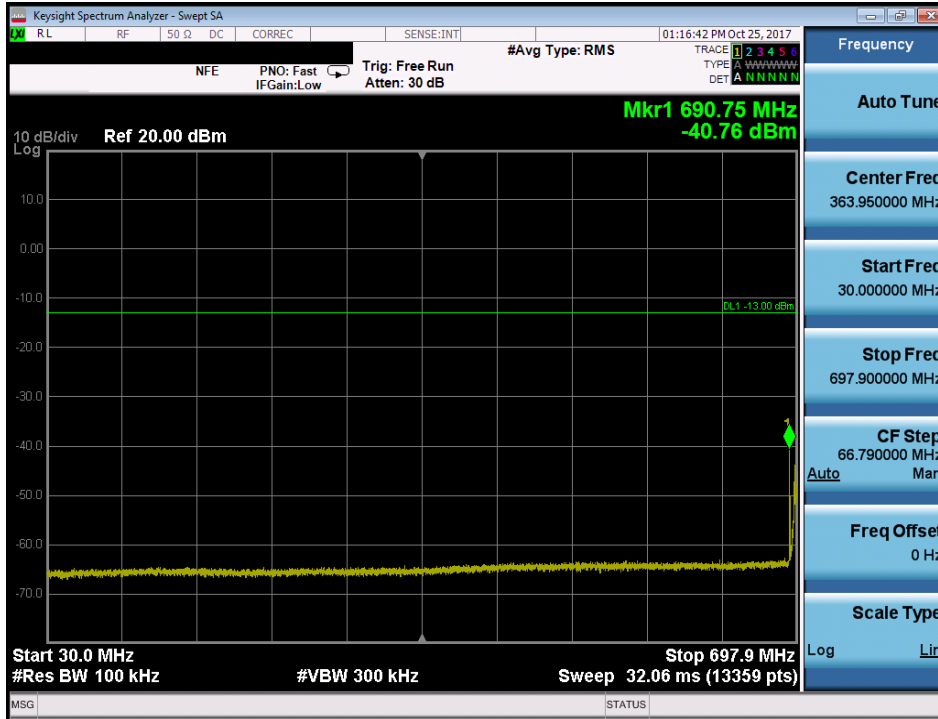
Plot 7-55. Conducted Spurious Plot (Band 12/17 - 10.0MHz QPSK - RB Size 1, RB Offset 0 - Low Channel)
