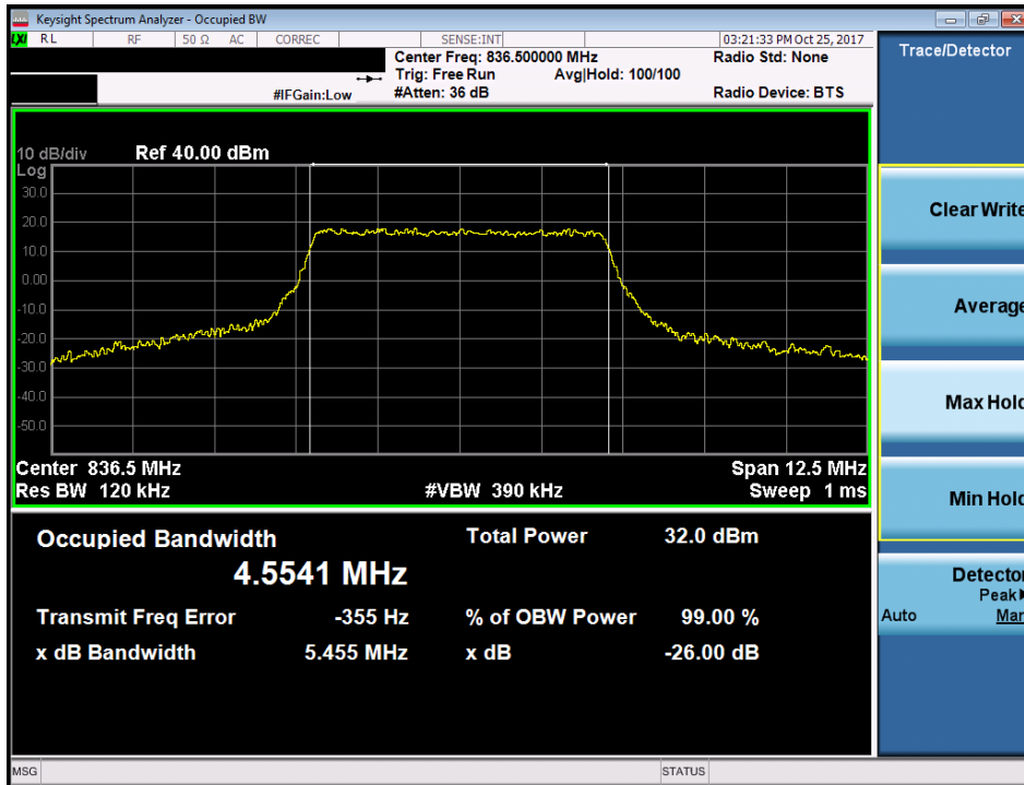
Plot 7-18. Occupied Bandwidth Plot (Band 26/5 - 5.0MHz 16-QAM - Full RB Configuration)
