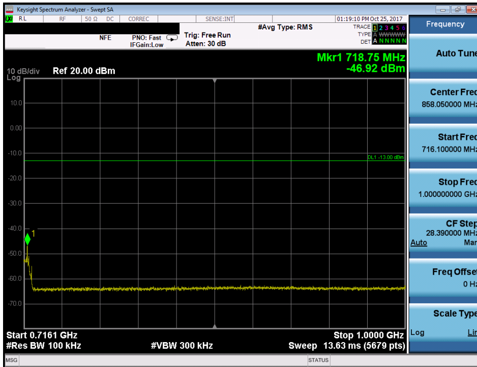
Plot 7-62. Conducted Spurious Plot (Band 12/17 - 10.0MHz QPSK - RB Size 1, RB Offset 0 - High Channel)
