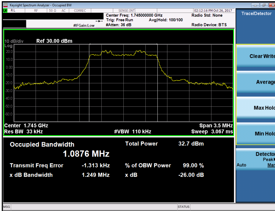
Plot 7-23. Occupied Bandwidth Plot (Band 66/4 - 1.4 MHz QPSK - Full RB Configuration)
