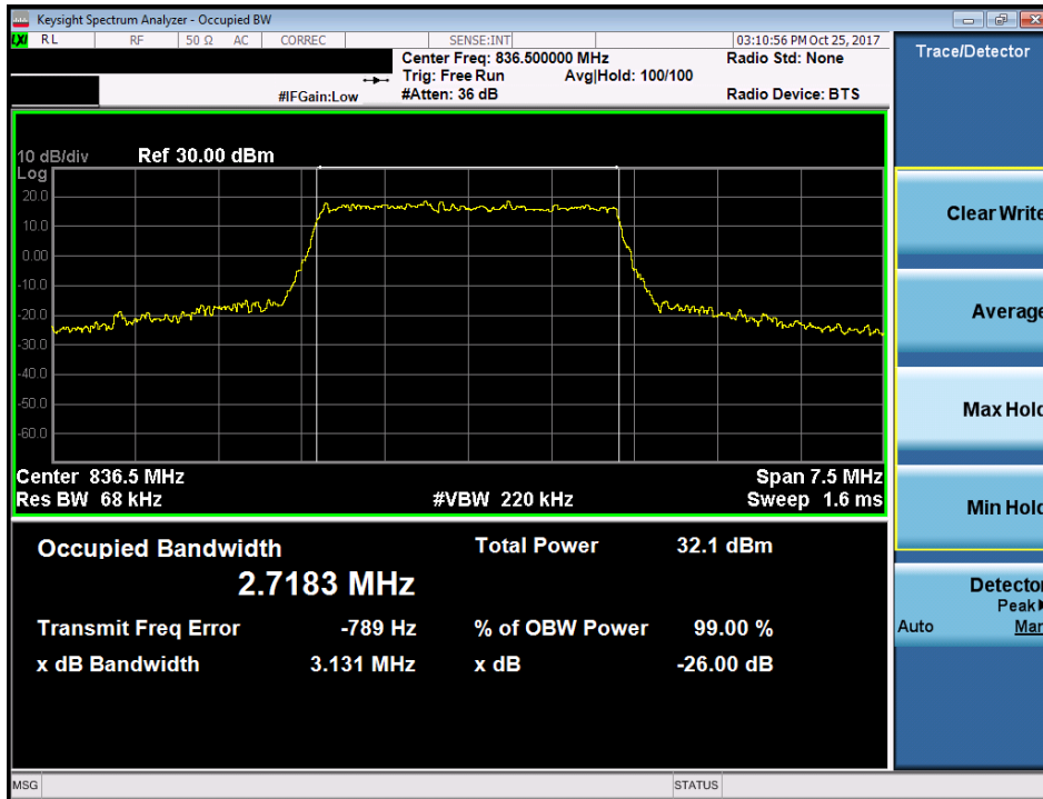
Plot 7-16. Occupied Bandwidth Plot (Band 26/5 - 3.0MHz 16-QAM - Full RB Configuration)
