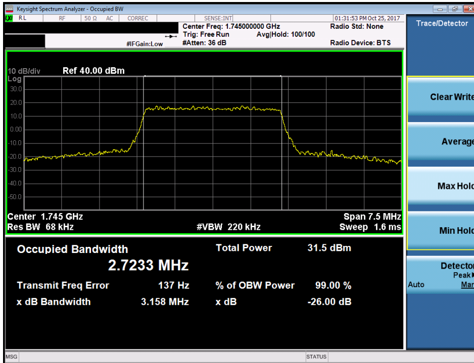
Plot 7-26. Occupied Bandwidth Plot (Band 66/4 - 3.0MHz 16-QAM - Full RB Configuration)
