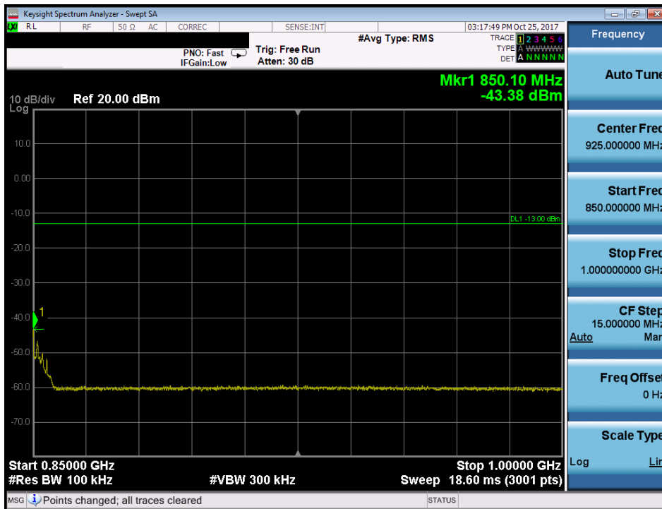
Plot 7-74. Conducted Spurious Plot (Band 26/5 - 3.0MHz QPSK - RB Size 1, RB Offset 0 - High Channel)
