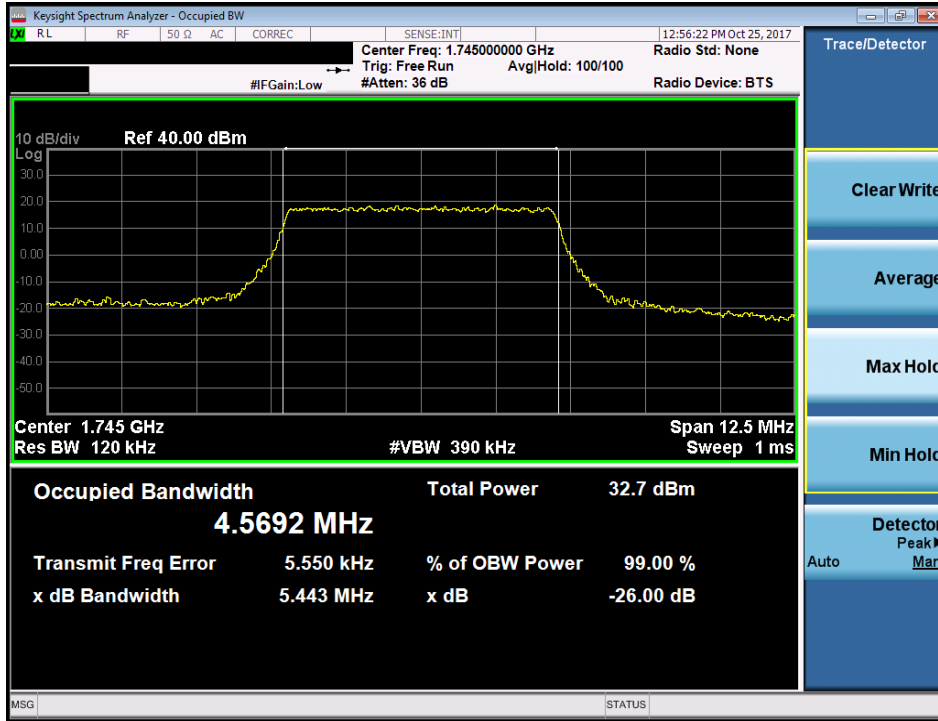
Plot 7-27. Occupied Bandwidth Plot (Band 66/4 - 5.0MHz QPSK - Full RB Configuration)
