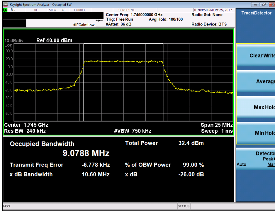
Plot 7-29. Occupied Bandwidth Plot (Band 66/4 - 10.0MHz QPSK - Full RB Configuration)
