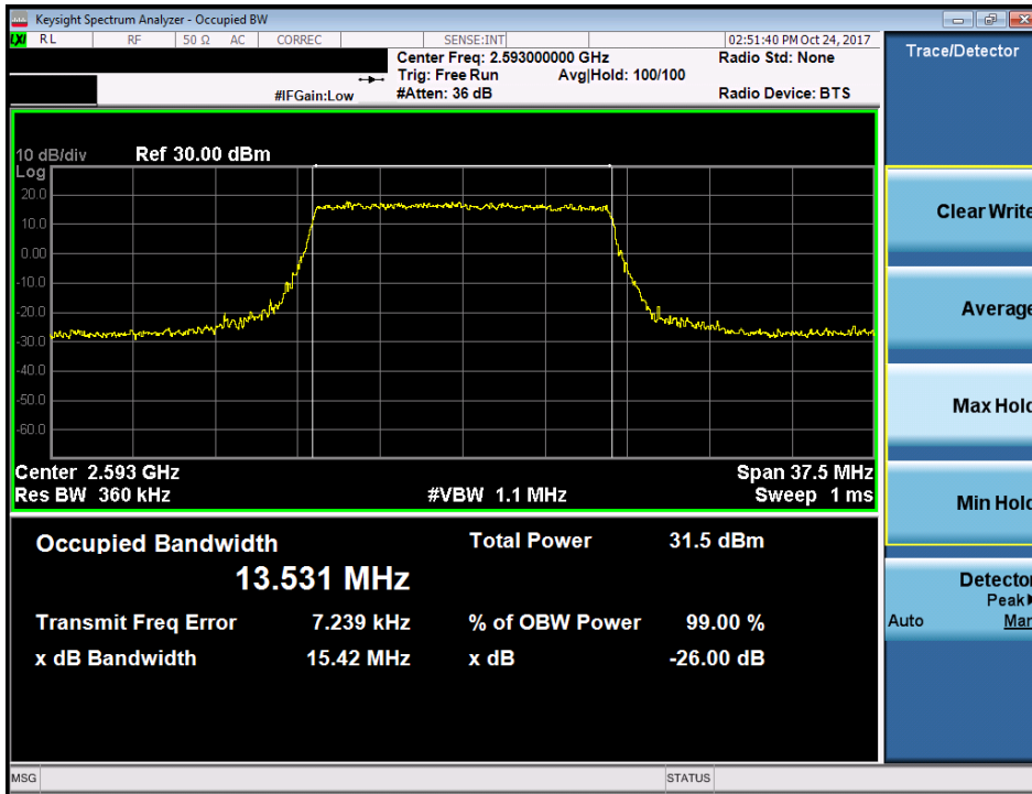
Plot 7-51. Occupied Bandwidth Plot (Band 41 - 15.0MHz QPSK - Full RB Configuration)
