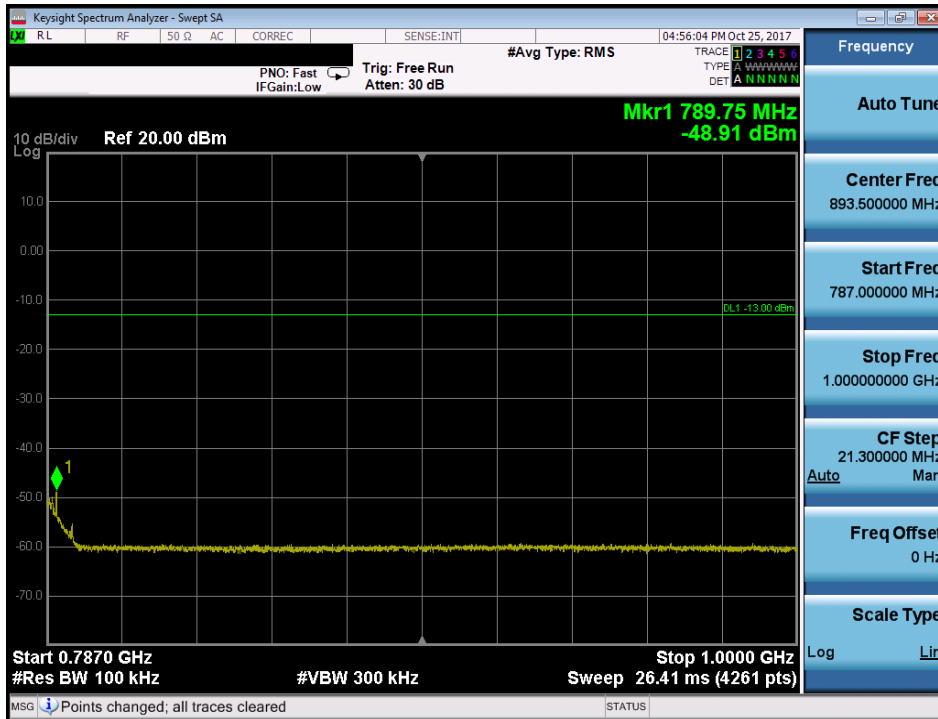
Plot 7-65. Conducted Spurious Plot (Band 13 - 10.0MHz QPSK - RB Size 1, RB Offset 0)
