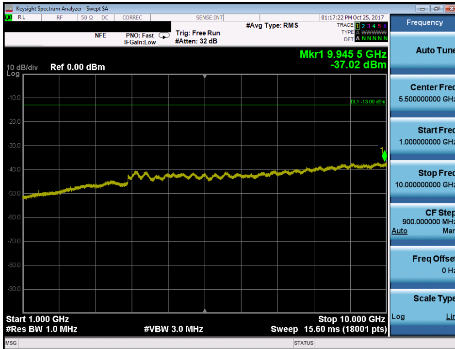
Plot 7-57. Conducted Spurious Plot (Band 12/17 - 10.0MHz QPSK - RB Size 1, RB Offset 0 - Low Channel)
