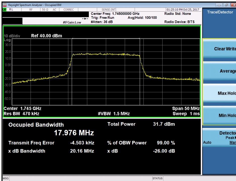
Plot 7-34. Occupied Bandwidth Plot (Band 66/4 - 20.0MHz 16-QAM - Full RB Configuration)
