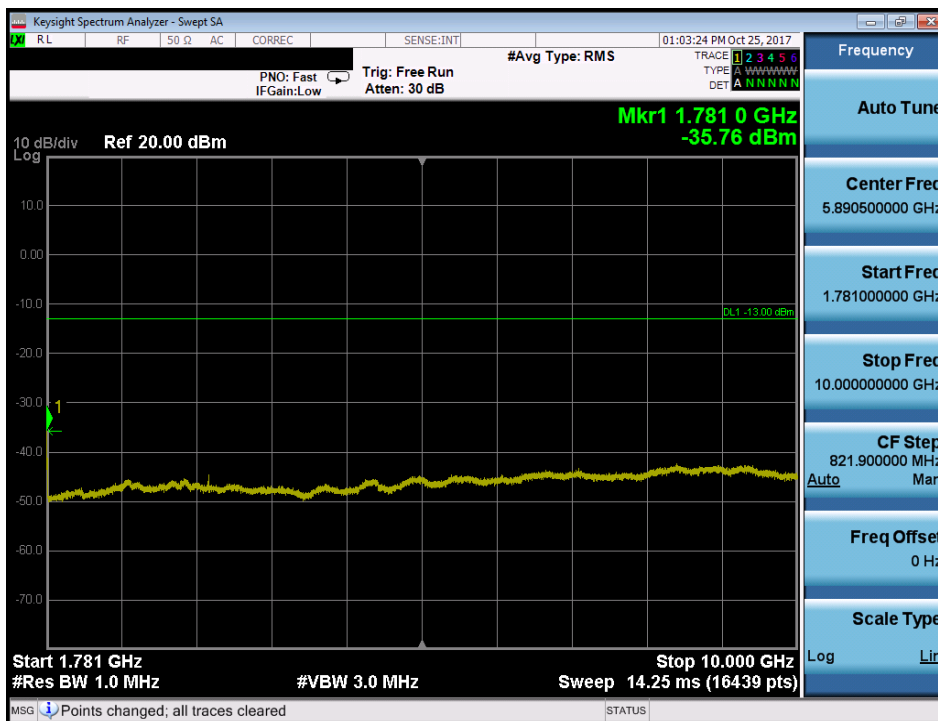
Plot 7-83. Conducted Spurious Plot (Band 66/4 - 5.0MHz QPSK - RB Size 1, RB Offset 0 - High Channel)
