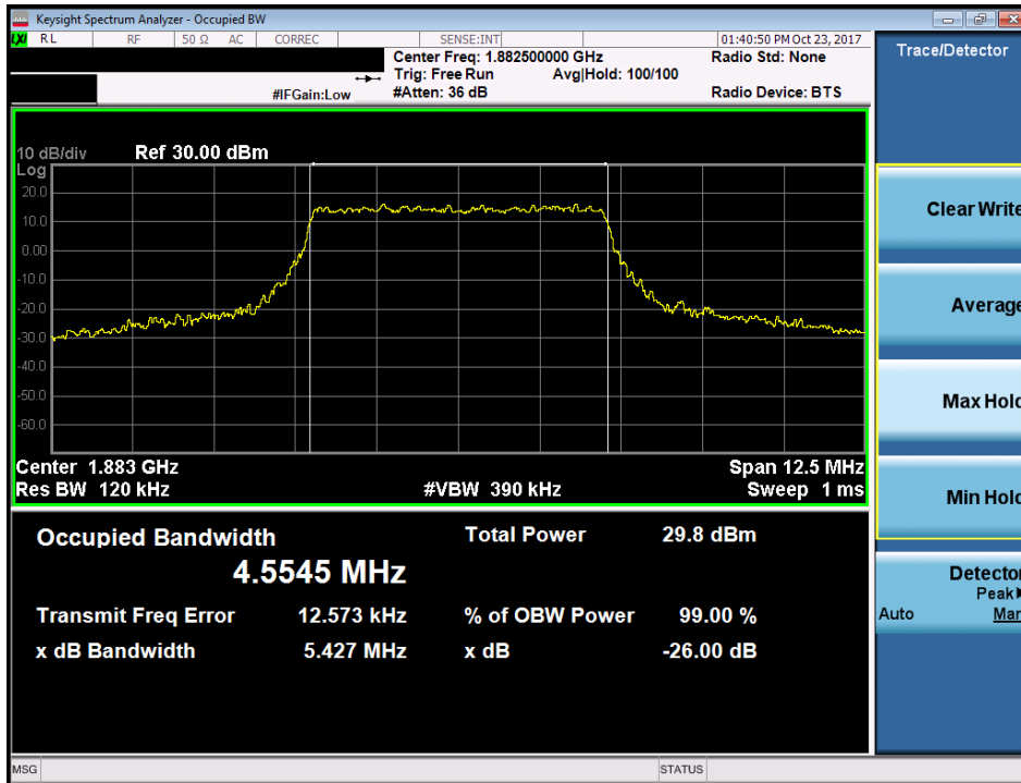
Plot 7-40. Occupied Bandwidth Plot (Band 25/2 - 5.0MHz 16-QAM - Full RB Configuration)
