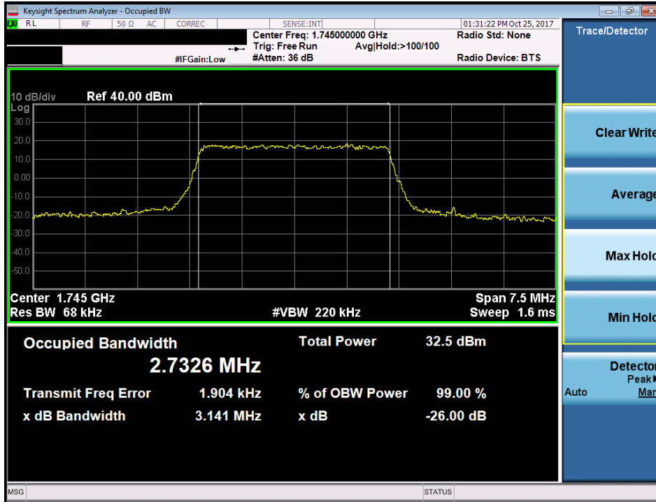
Plot 7-25. Occupied Bandwidth Plot (Band 66/4 - 3.0MHz QPSK - Full RB Configuration)
