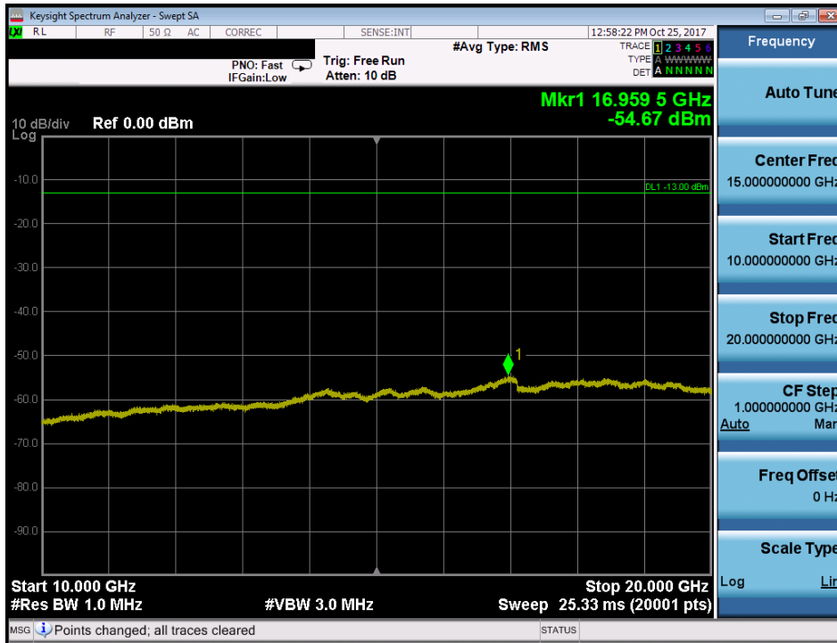
Plot 7-81. Conducted Spurious Plot (Band 66/4 - 5.0MHz QPSK - RB Size 1, RB Offset 0 - Mid Channel)
