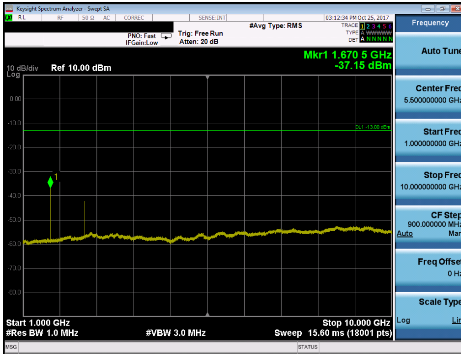
Plot 7-72. Conducted Spurious Plot (Band 26/5 - 3.0MHz QPSK - RB Size 1, RB Offset 0 - Mid Channel)
