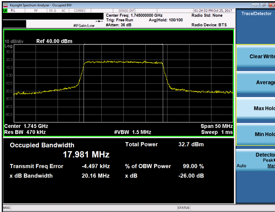
Plot 7-33. Occupied Bandwidth Plot (Band 66/4 - 20.0MHz QPSK - Full RB Configuration)
