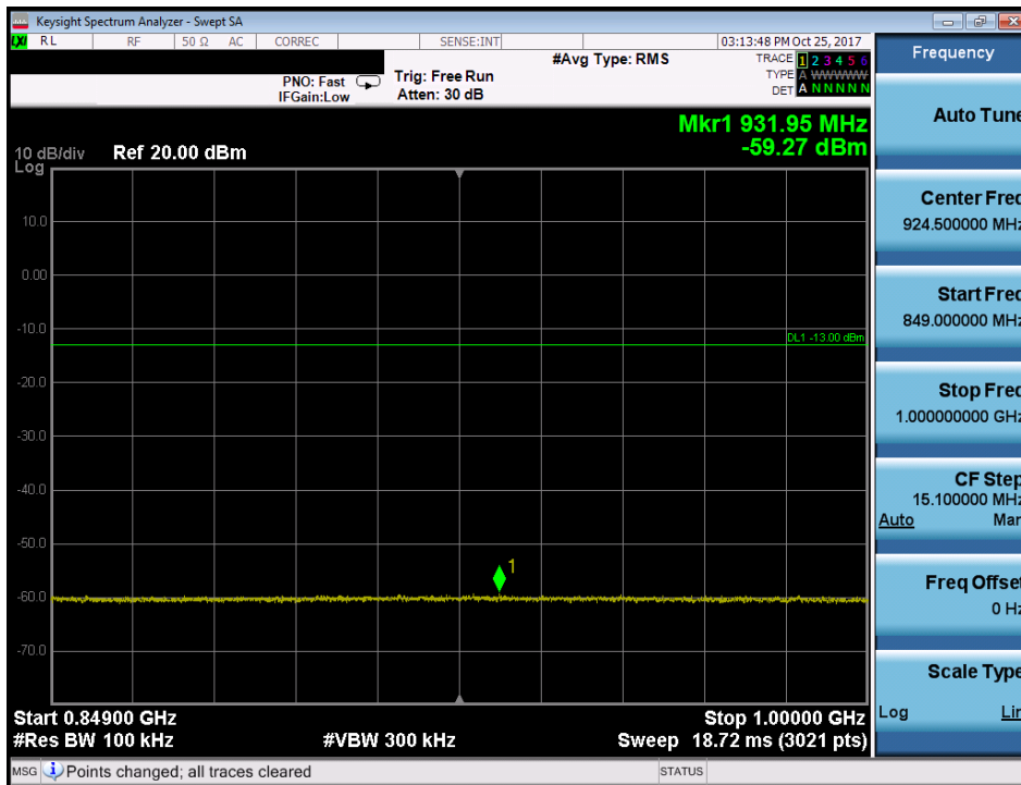
Plot 7-68. Conducted Spurious Plot (Band 26/5 - 3.0MHz QPSK - RB Size 1, RB Offset 0 - Low Channel)
