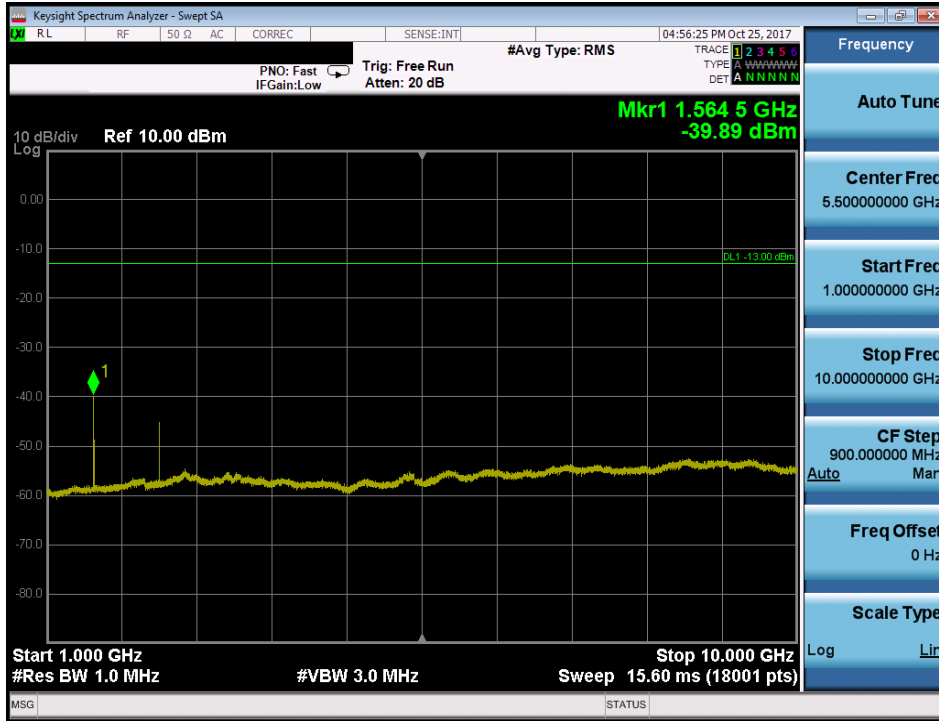
Plot 7-66. Conducted Spurious Plot (Band 13 - 10.0MHz QPSK - RB Size 1, RB Offset 0)
