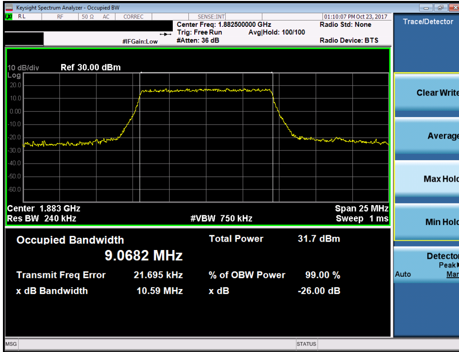
Plot 7-41. Occupied Bandwidth Plot (Band 25/2 - 10.0MHz QPSK - Full RB Configuration)
