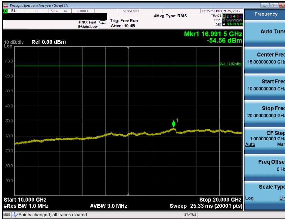
Plot 7-78. Conducted Spurious Plot (Band 66/4 - 5.0MHz QPSK - RB Size 1, RB Offset 0 - Low Channel)
