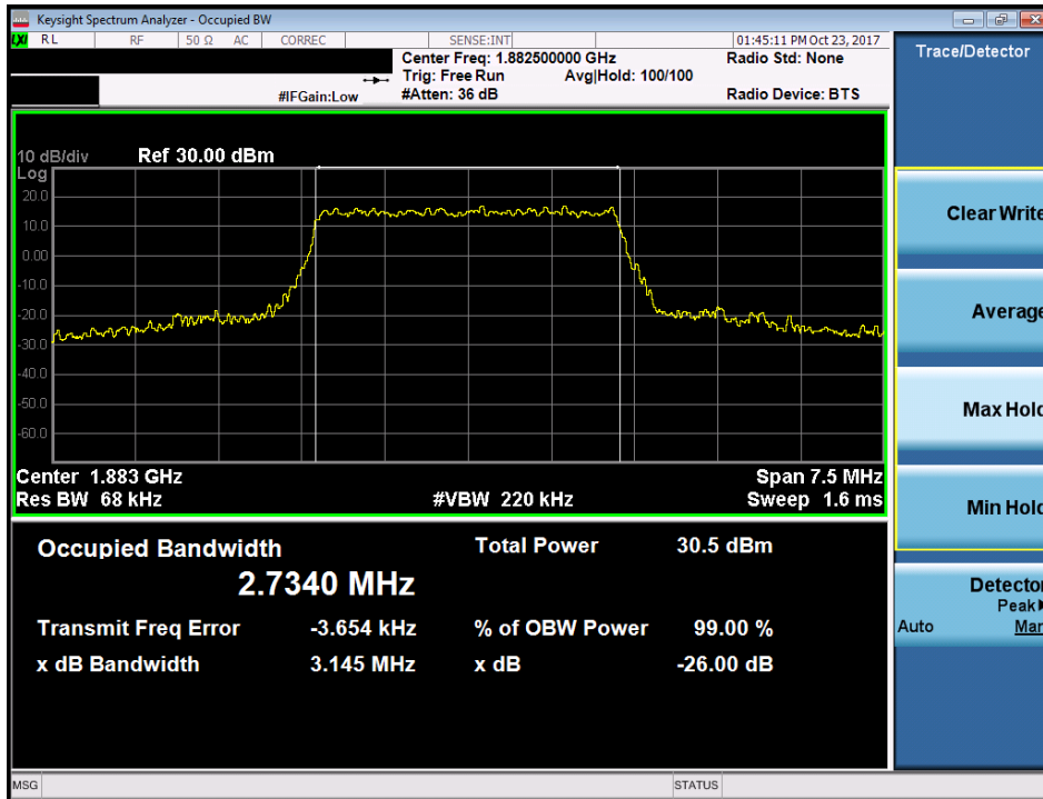
Plot 7-38. Occupied Bandwidth Plot (Band 25/2 - 3.0MHz 16-QAM - Full RB Configuration)
