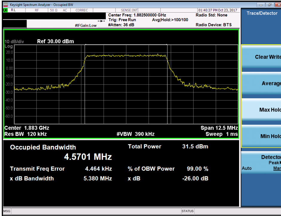
Plot 7-39. Occupied Bandwidth Plot (Band 25/2 - 5.0MHz QPSK - Full RB Configuration)
