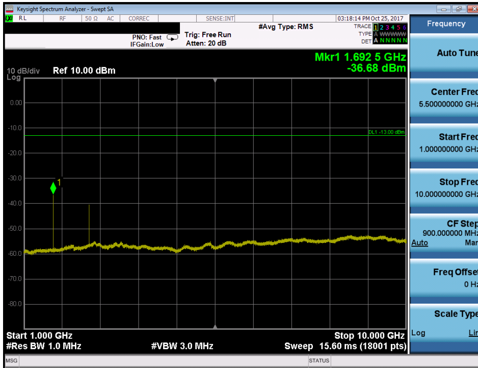
Plot 7-75. Conducted Spurious Plot (Band 26/5 - 3.0MHz QPSK - RB Size 1, RB Offset 0 - High Channel)
