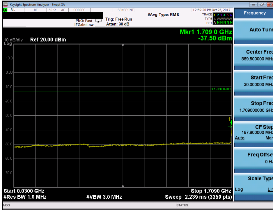
Plot 7-76. Conducted Spurious Plot (Band 66/4 - 5.0MHz QPSK - RB Size 1, RB Offset 0 - Low Channel)
