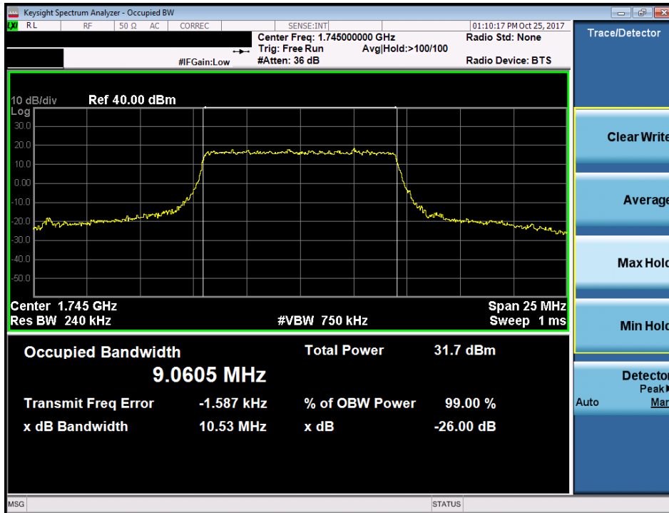
Plot 7-30. Occupied Bandwidth Plot (Band 66/4 - 10.0MHz 16-QAM - Full RB Configuration)
