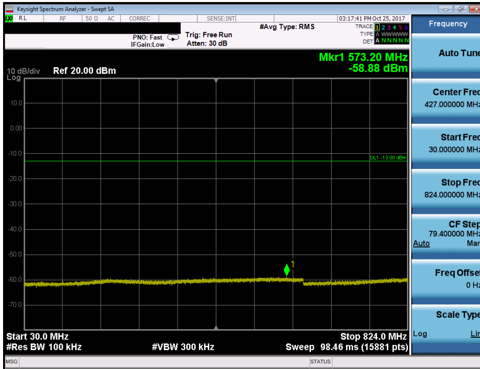
Plot 7-73. Conducted Spurious Plot (Band 26/5 - 3.0MHz QPSK - RB Size 1, RB Offset 0 - High Channel)
