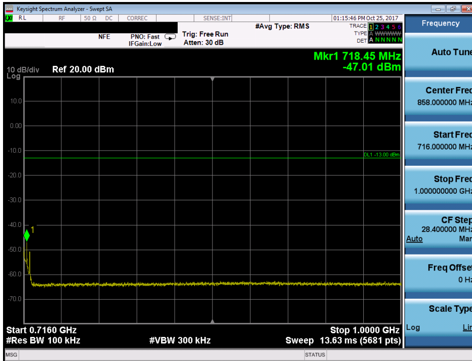
Plot 7-59. Conducted Spurious Plot (Band 12/17 - 10.0MHz QPSK - RB Size 1, RB Offset 0 - Mid Channel)
