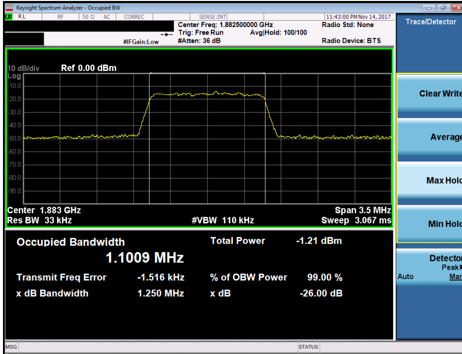
Plot 7-35. Occupied Bandwidth Plot (Band 25/2 - 1.4 MHz QPSK - Full RB Configuration)
