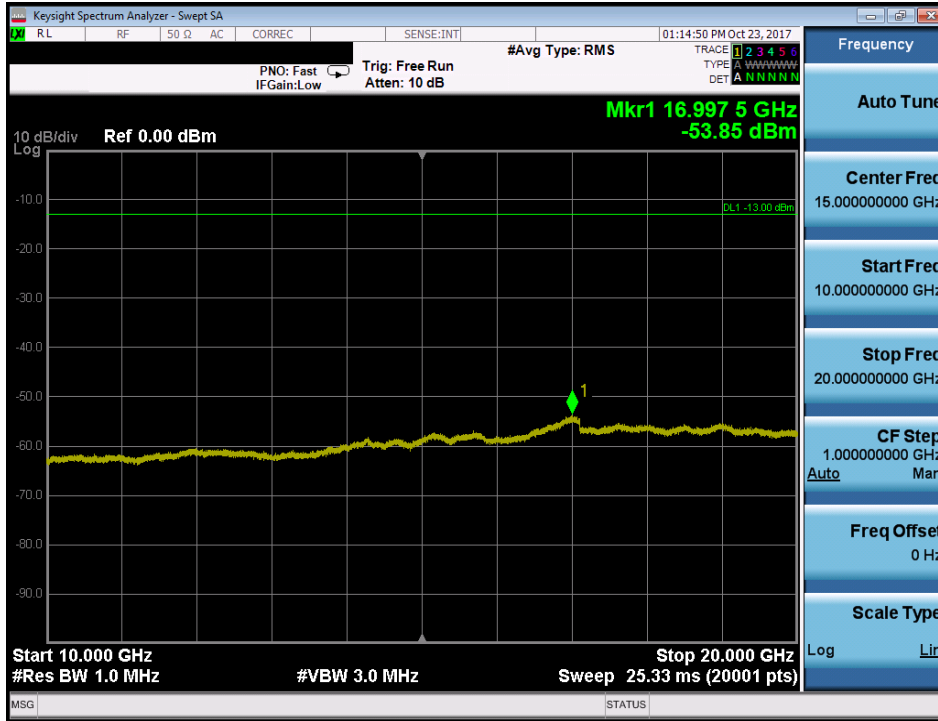
Plot 7-87. Conducted Spurious Plot (Band 25/2 - 10.0MHz QPSK - RB Size 1, RB Offset 0 - Low Channel)
