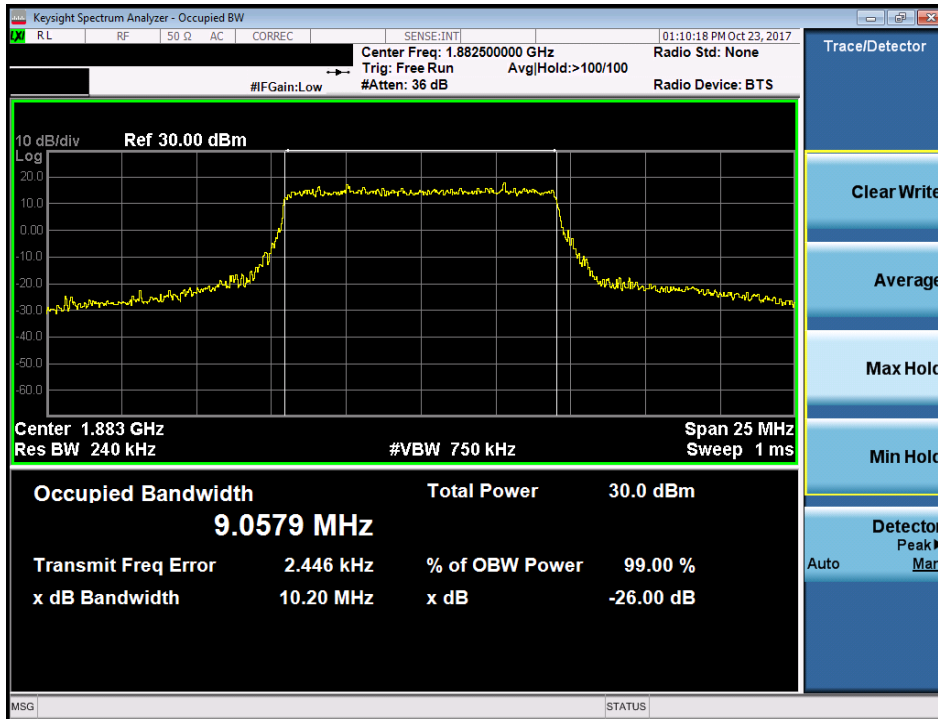
Plot 7-42. Occupied Bandwidth Plot (Band 25/2 - 10.0MHz 16-QAM - Full RB Configuration)
