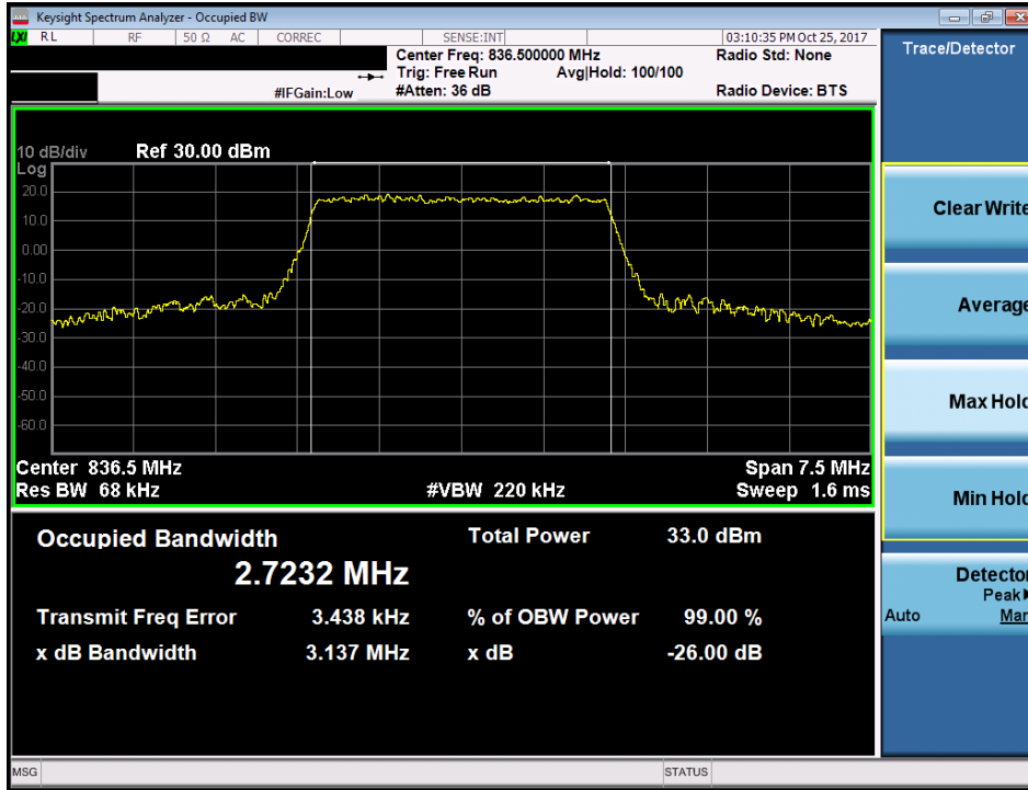
Plot 7-15. Occupied Bandwidth Plot (Band 26/5 - 3.0MHz QPSK - Full RB Configuration)
