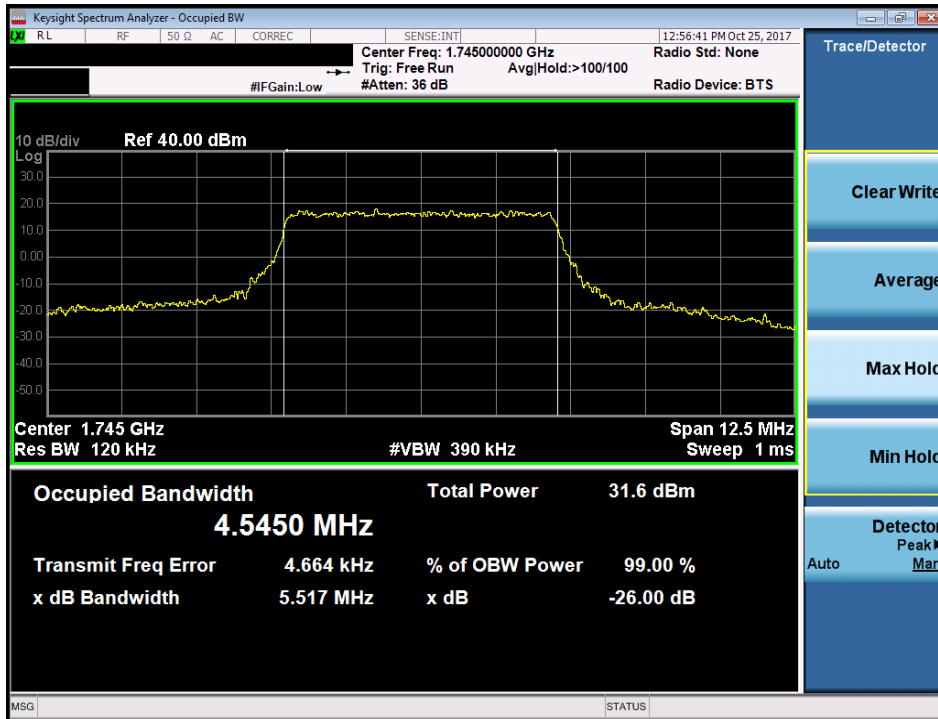
Plot 7-28. Occupied Bandwidth Plot (Band 66/4 - 5.0MHz 16-QAM - Full RB Configuration)
