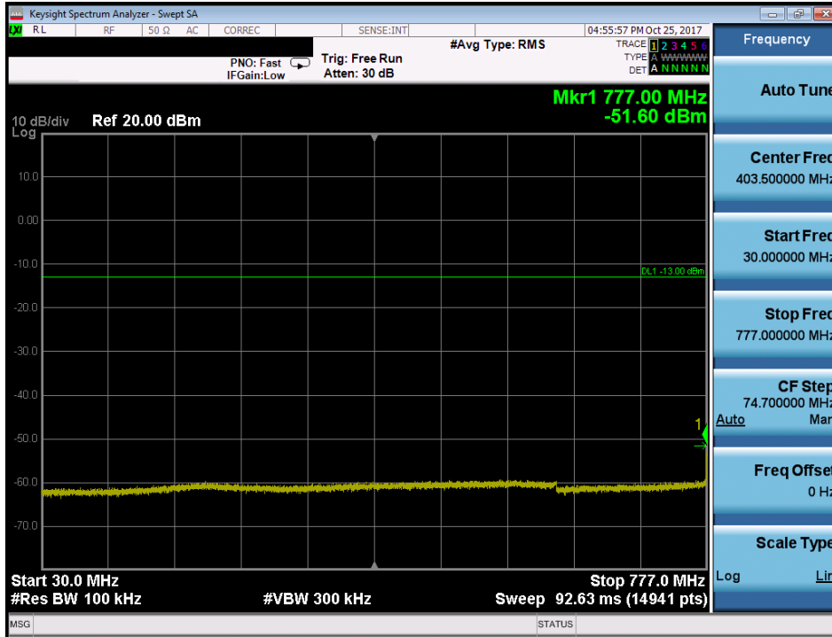
Plot 7-64. Conducted Spurious Plot (Band 13 - 10.0MHz QPSK - RB Size 1, RB Offset 0)
