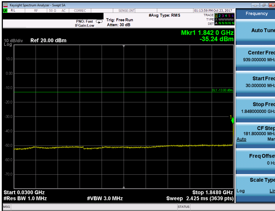
Plot 7-85. Conducted Spurious Plot (Band 25/2 - 10.0MHz QPSK - RB Size 1, RB Offset 0 - Low Channel)
