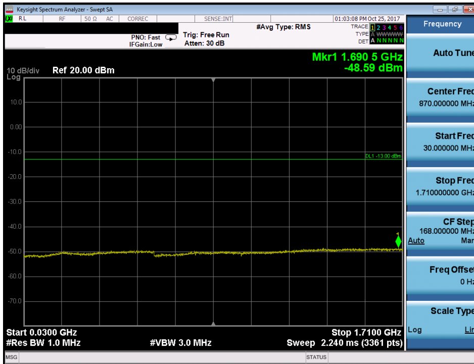
Plot 7-82. Conducted Spurious Plot (Band 66/4 - 5.0MHz QPSK - RB Size 1, RB Offset 0 - High Channel)
