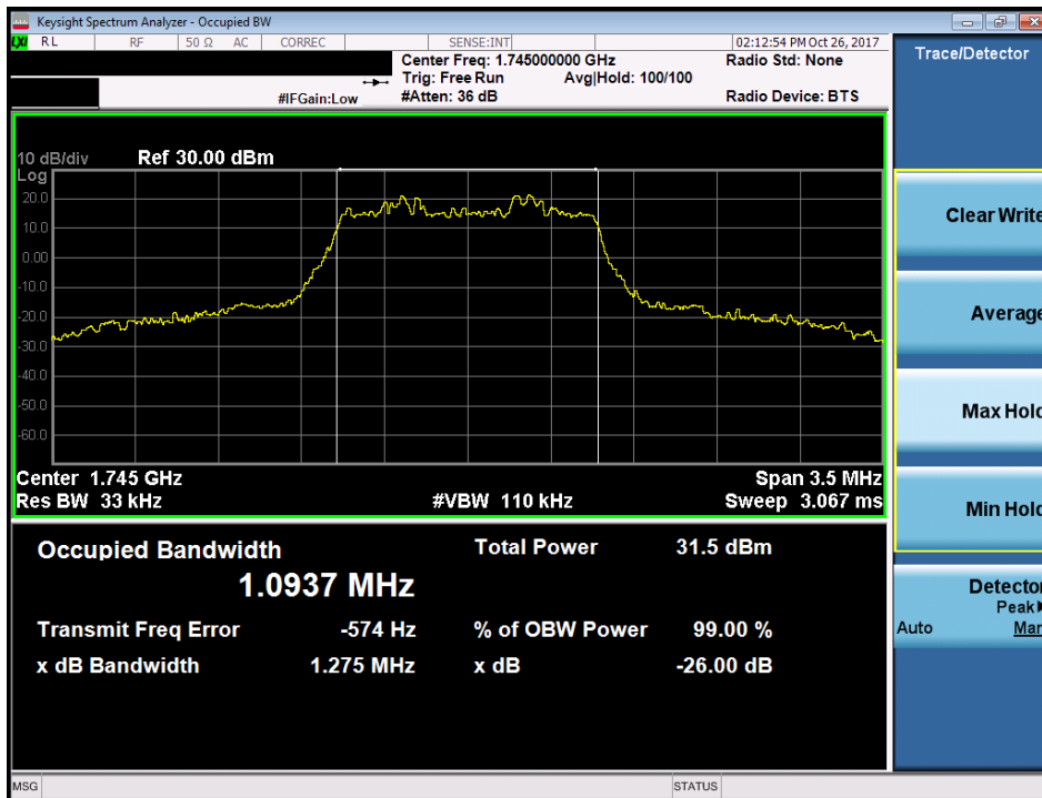
Plot 7-24. Occupied Bandwidth Plot (Band 66/4 - 1.4 MHz 16-QAM - Full RB Configuration)
