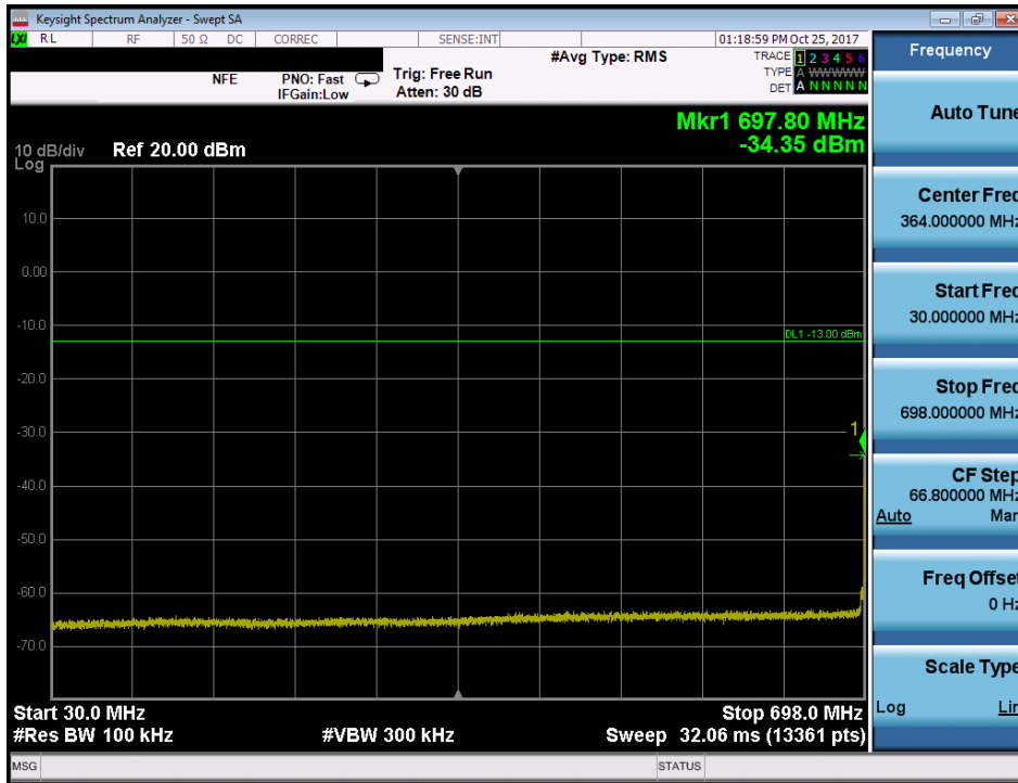
Plot 7-61. Conducted Spurious Plot (Band 12/17 - 10.0MHz QPSK - RB Size 1, RB Offset 0 - High Channel)
