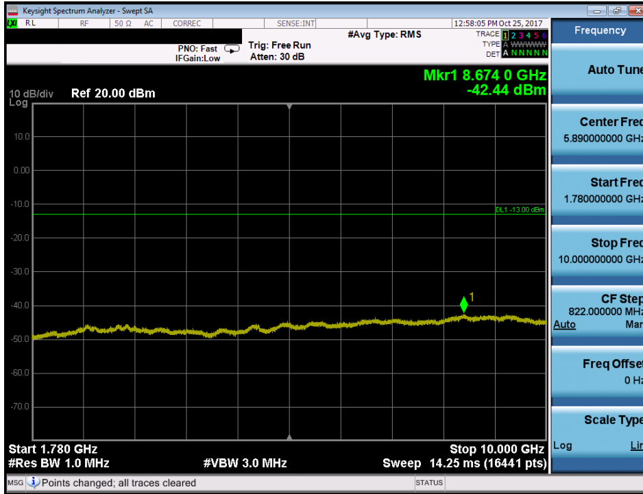
Plot 7-80. Conducted Spurious Plot (Band 66/4 - 5.0MHz QPSK - RB Size 1, RB Offset 0 - Mid Channel)
