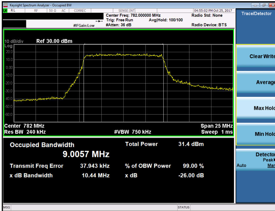
Plot 7-12. Occupied Bandwidth Plot (Band 13 - 10.0MHz 16-QAM - Full RB Configuration)
