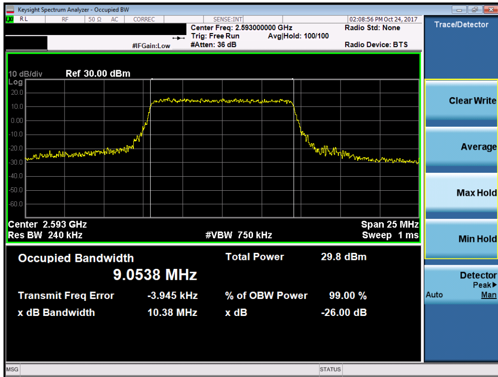
Plot 7-50. Occupied Bandwidth Plot (Band 41 - 10.0MHz 16-QAM - Full RB Configuration)
