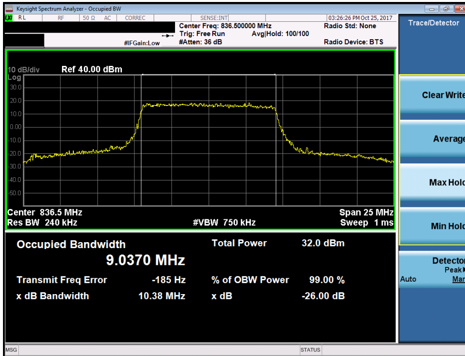
Plot 7-20. Occupied Bandwidth Plot (Band 26/5 - 10.0MHz 16-QAM - Full RB Configuration)
