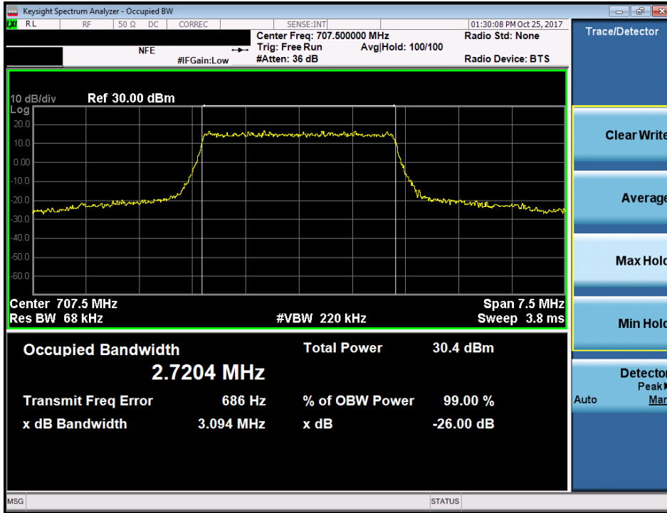
Plot 7-3. Occupied Bandwidth Plot (Band 12 - 3.0MHz QPSK - Full RB Configuration)
