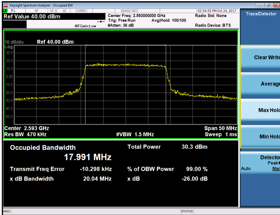
Plot 7-54. Occupied Bandwidth Plot (Band 41 - 20.0MHz 16-QAM - Full RB Configuration)
