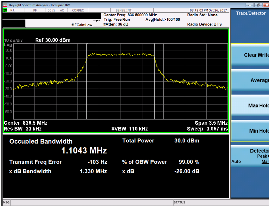
Plot 7-14. Occupied Bandwidth Plot (Band 26/5 - 1.4 MHz 16-QAM - Full RB Configuration)
