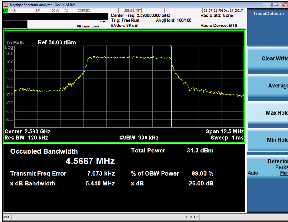
Plot 7-47. Occupied Bandwidth Plot (Band 41 - 5.0MHz QPSK - Full RB Configuration)
