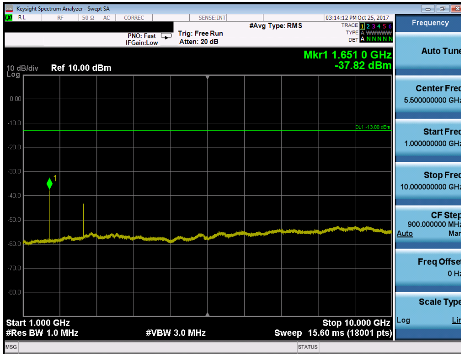
Plot 7-69. Conducted Spurious Plot (Band 26/5 - 3.0MHz QPSK - RB Size 1, RB Offset 0 - Low Channel)
