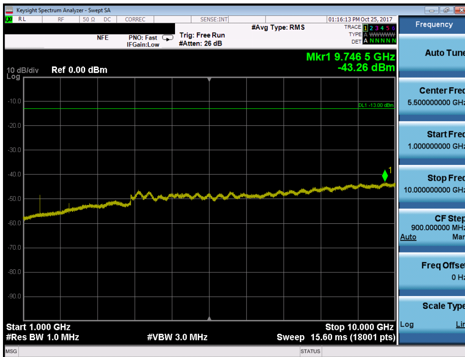
Plot 7-60. Conducted Spurious Plot (Band 12/17 - 10.0MHz QPSK - RB Size 1, RB Offset 0 - Mid Channel)
