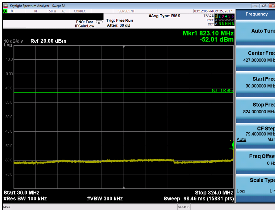
Plot 7-70. Conducted Spurious Plot (Band 26/5 - 3.0MHz QPSK - RB Size 1, RB Offset 0 - Mid Channel)
