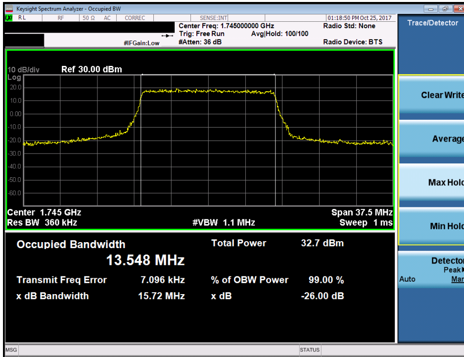
Plot 7-31. Occupied Bandwidth Plot (Band 66/4 - 15.0MHz QPSK - Full RB Configuration)
