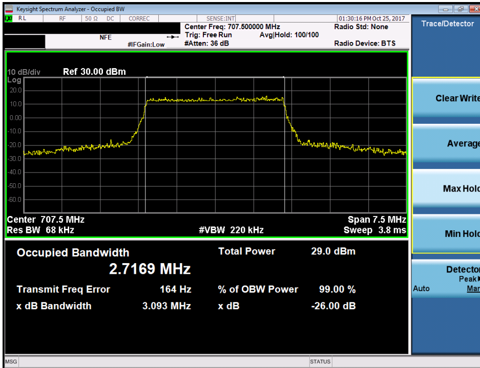
Plot 7-4. Occupied Bandwidth Plot (Band 12 - 3.0MHz 16-QAM - Full RB Configuration)
