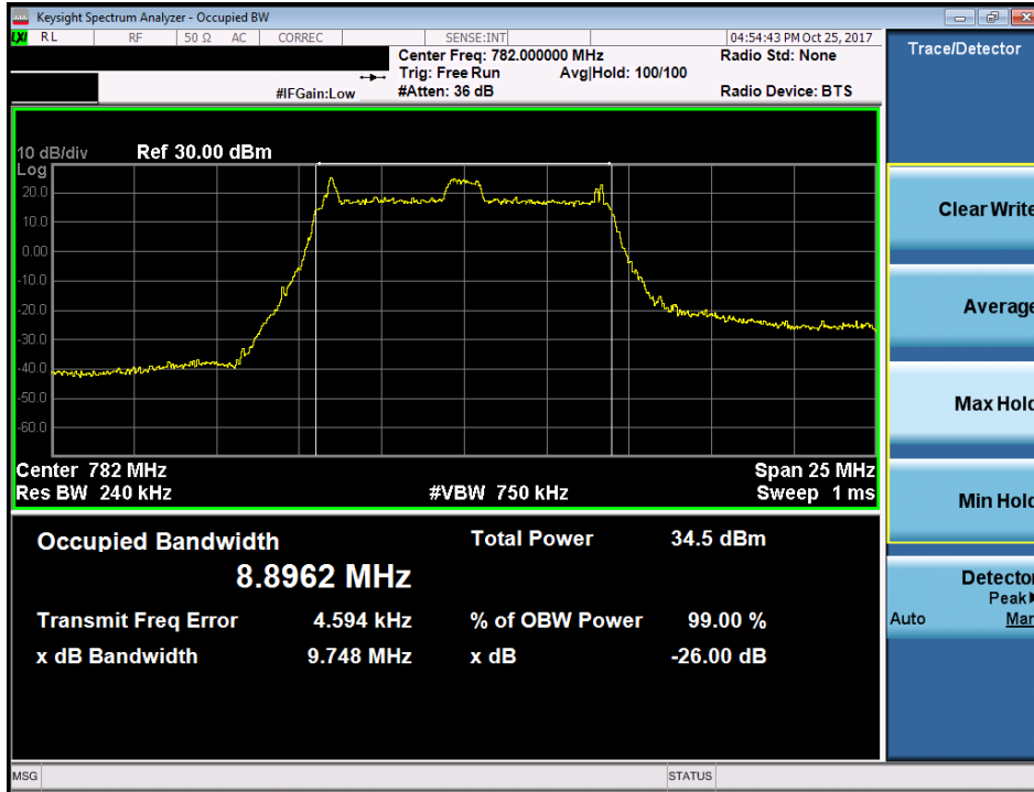
Plot 7-11. Occupied Bandwidth Plot (Band 13 - 10.0MHz QPSK - Full RB Configuration)
