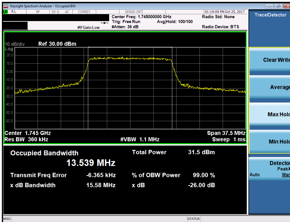
Plot 7-32. Occupied Bandwidth Plot (Band 66/4 - 15.0MHz 16-QAM - Full RB Configuration)
