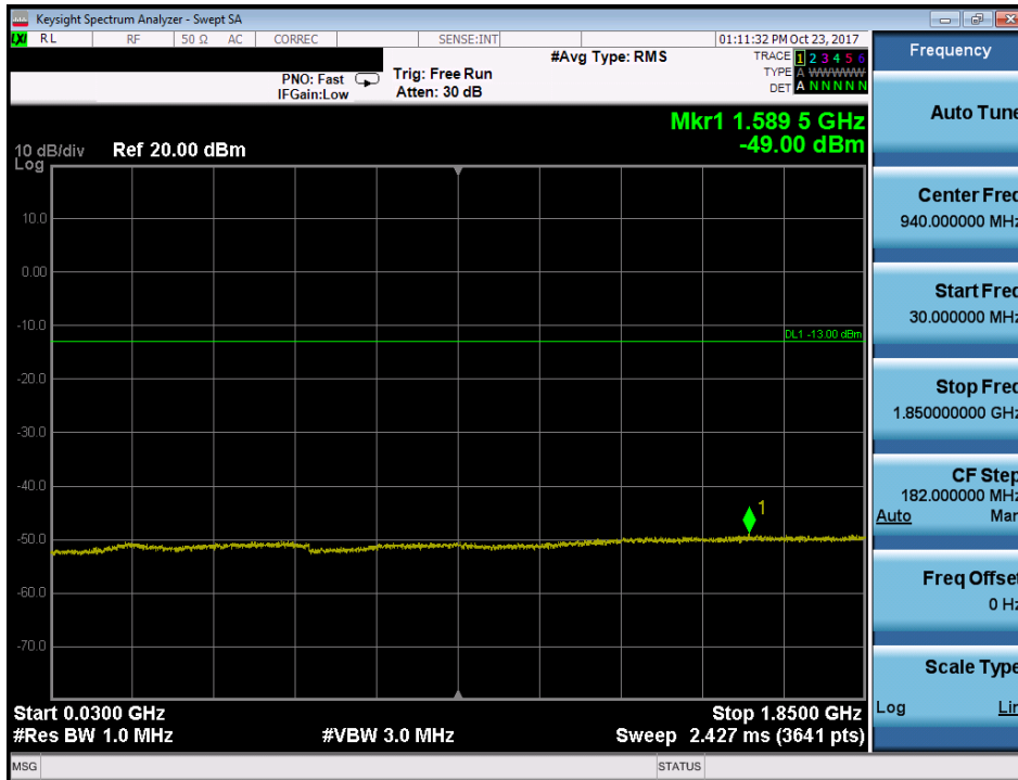
Plot 7-88. Conducted Spurious Plot (Band 25/2 - 10.0MHz QPSK - RB Size 1, RB Offset 0 - Mid Channel)
