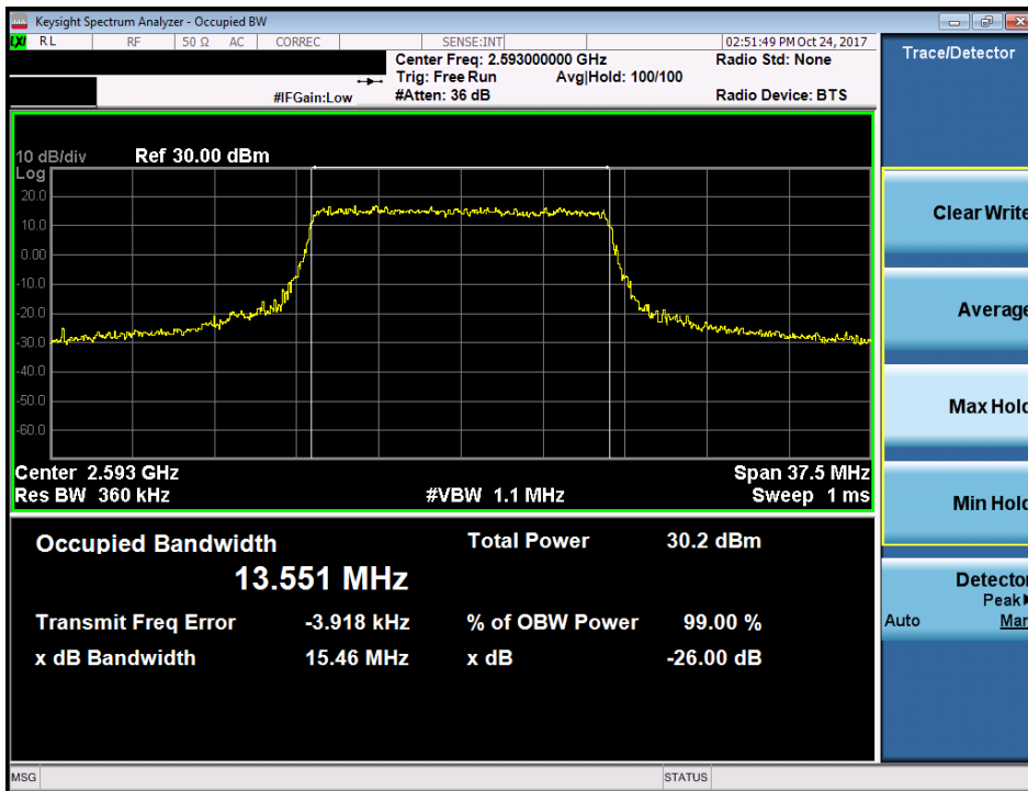
Plot 7-52. Occupied Bandwidth Plot (Band 41 - 15.0MHz 16-QAM - Full RB Configuration)
