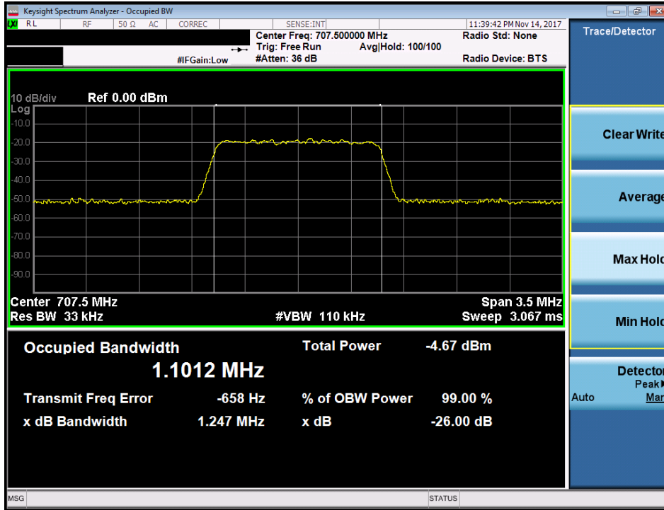
Plot 7-1. Occupied Bandwidth Plot (Band 12 - 1.4 MHz QPSK - Full RB Configuration)
