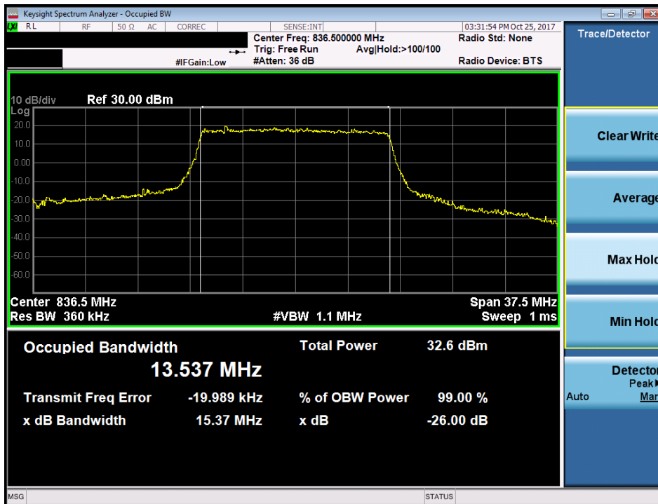
Plot 7-22. Occupied Bandwidth Plot (Band 26 - 15.0MHz 16-QAM - Full RB Configuration)
