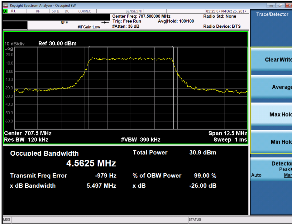
Plot 7-5. Occupied Bandwidth Plot (Band 12/17 - 5.0MHz QPSK - Full RB Configuration)
