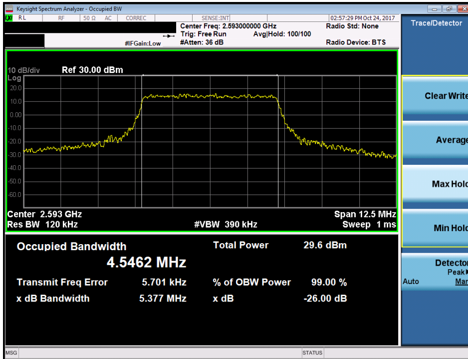
Plot 7-48. Occupied Bandwidth Plot (Band 41 - 5.0MHz 16-QAM - Full RB Configuration)
