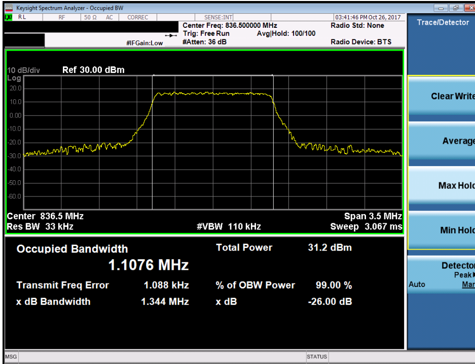
Plot 7-13. Occupied Bandwidth Plot (Band 26/5 - 1.4 MHz QPSK - Full RB Configuration)
