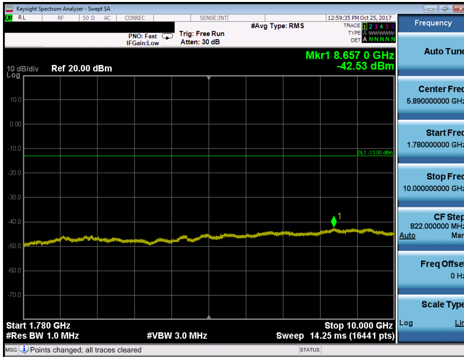
Plot 7-77. Conducted Spurious Plot (Band 66/4 - 5.0MHz QPSK - RB Size 1, RB Offset 0 - Low Channel)
