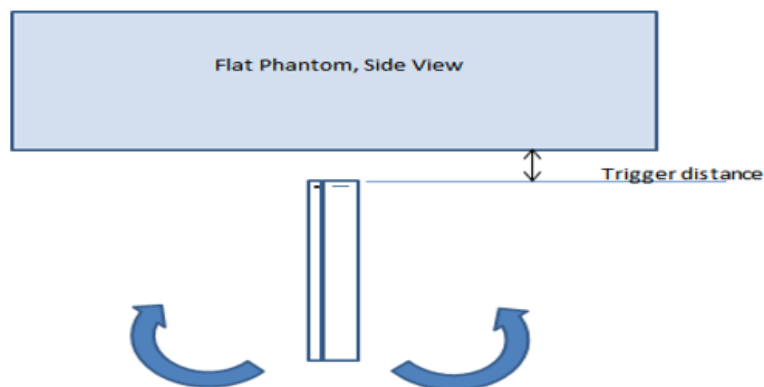
Proximity sensor tilt angle assessment (Edge 3) KDB 616217 §6.4
