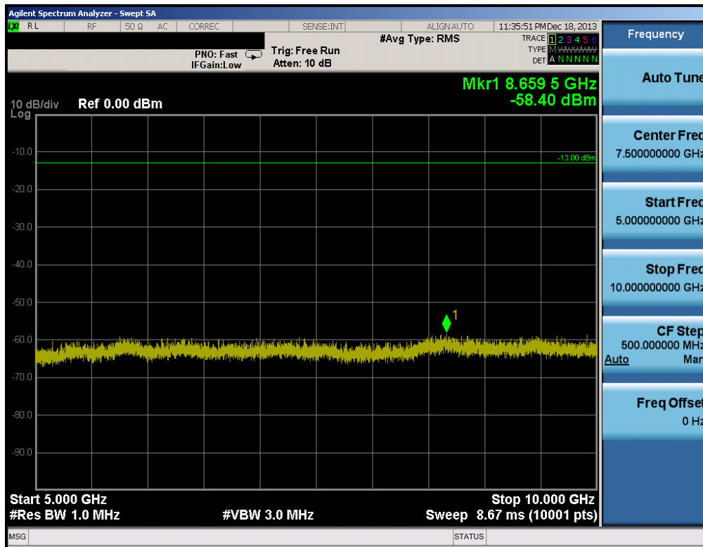
Plot 8-9. Conducted Spurious Plot (3.0MHz QPSK – RB Size 1, RB Offset 0 – Low Channel)
