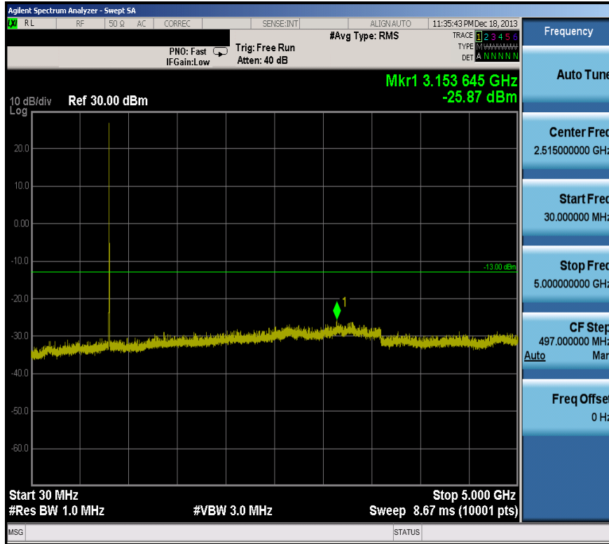
Plot 8-8. Conducted Spurious Plot (3.0MHz QPSK – RB Size 1, RB Offset 0 – Low Channel)
