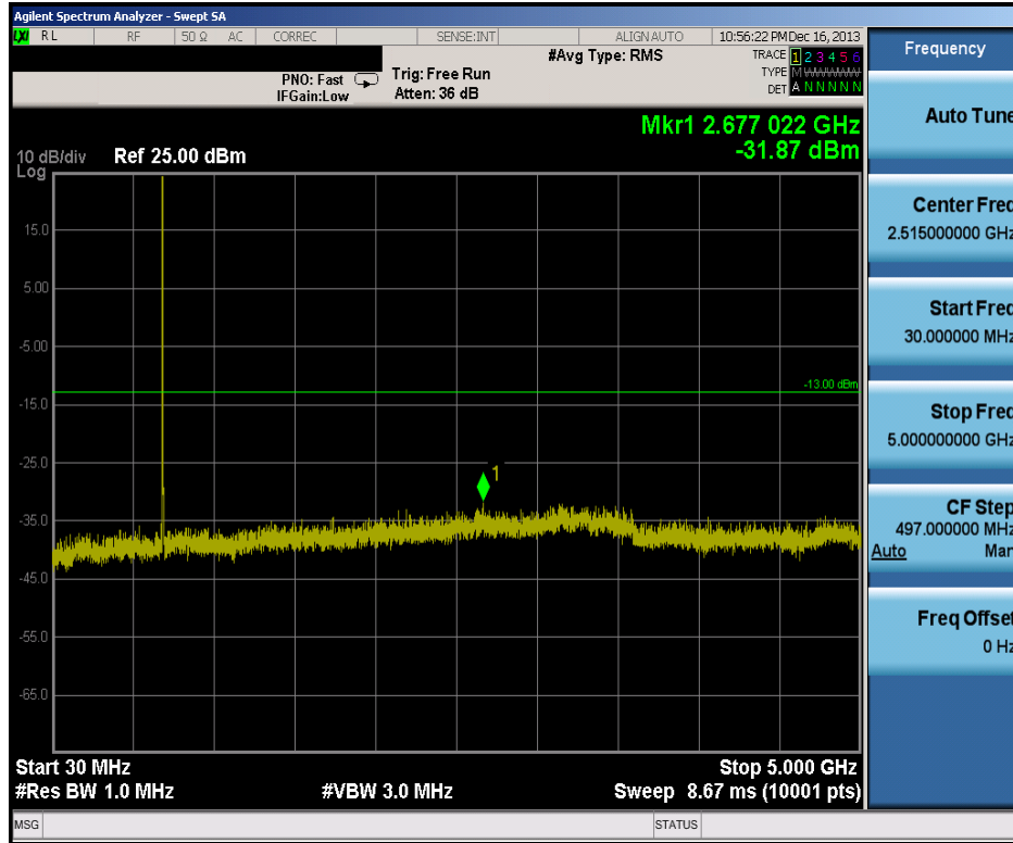
Plot 7-6. Conducted Spurious Plot (5.0MHz QPSK – RB Size 1, RB Offset 0 – Mid Channel)
