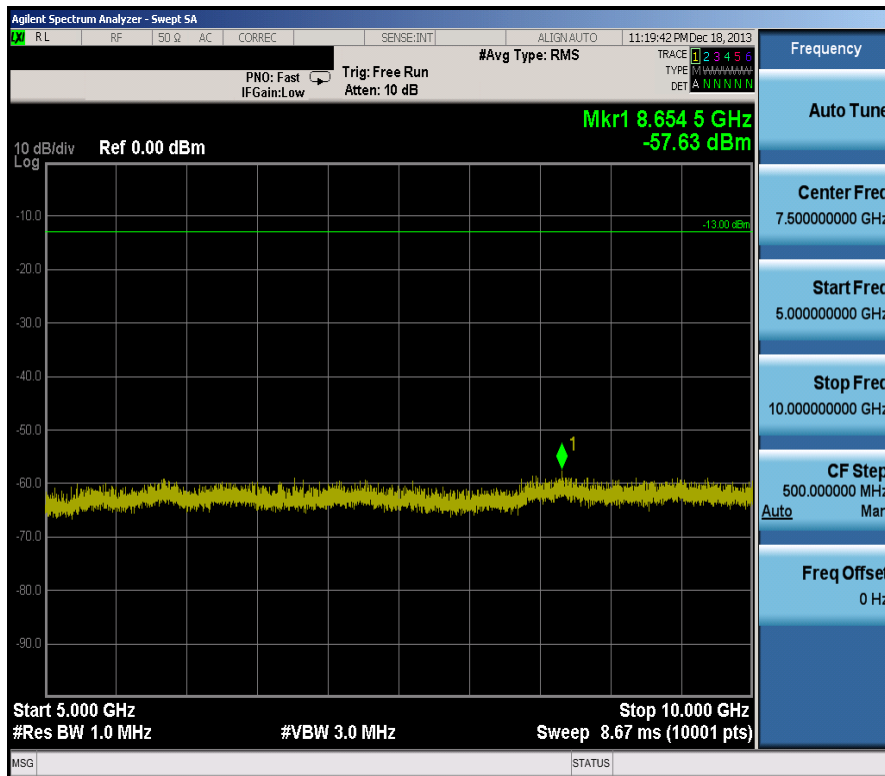
Plot 7-9. Conducted Spurious Plot (5.0MHz QPSK – RB Size 1, RB Offset 0 – High Channel)
