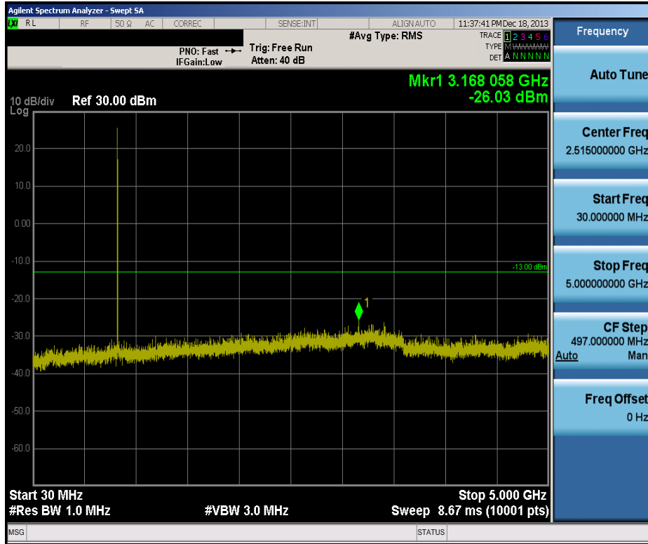
Plot 8-12. Conducted Spurious Plot (3.0MHz QPSK – RB Size 1, RB Offset 0 – High Channel)
