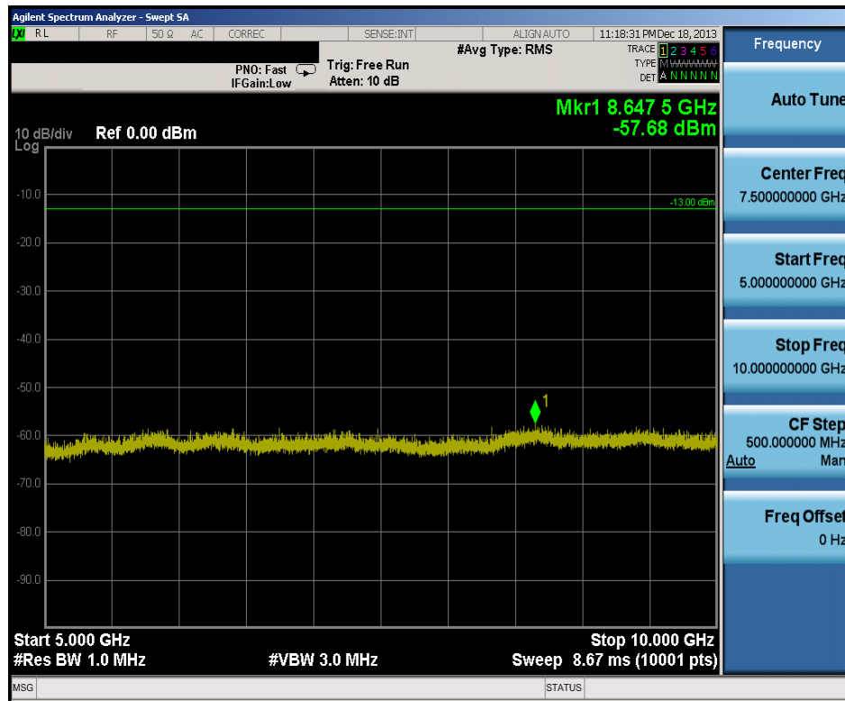
Plot 7-5. Conducted Spurious Plot (5.0MHz QPSK – RB Size 1, RB Offset 0 – Low Channel)
