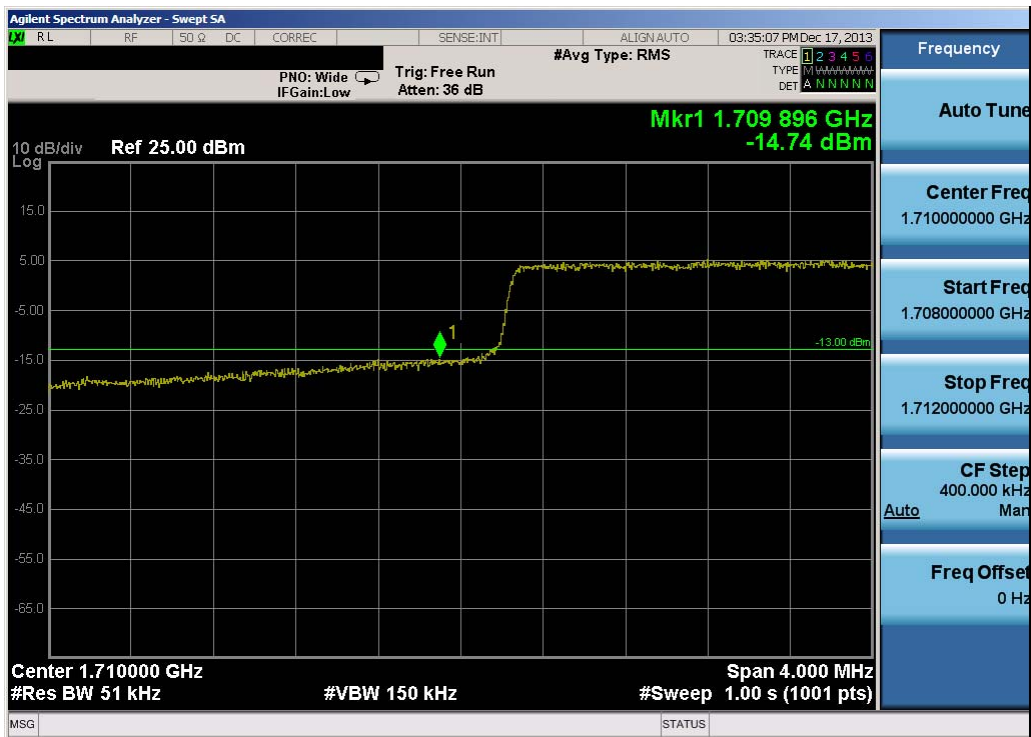
Plot 9-17. Lower Band Edge Plot (5.0MHz QPSK – RB Size 25)
