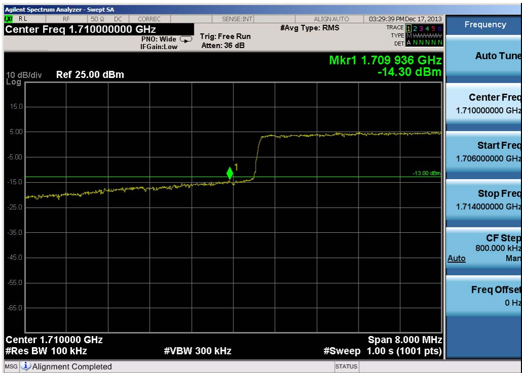
Plot 9-25. Lower Band Edge Plot (10.0MHz QPSK – RB Size 50)
