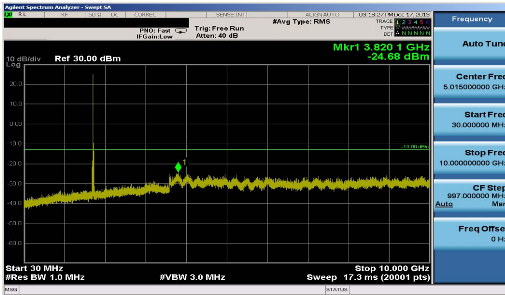
Plot 9-31. Conducted Spurious Plot (10.0MHz QPSK – RB Size 1, RB Offset 0 – Mid Channel)
