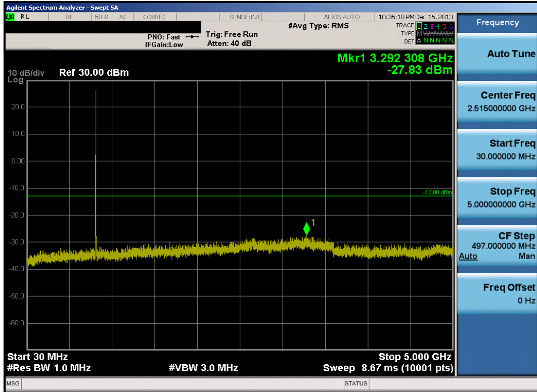
Plot 8-10. Conducted Spurious Plot (3.0MHz QPSK – RB Size 1, RB Offset 0 – Mid Channel)
