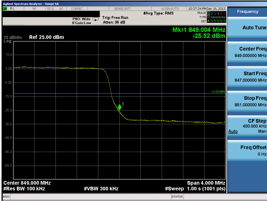
Plot 8-18. Upper Band Edge Plot (5.0MHz QPSK – RB Size 25)
