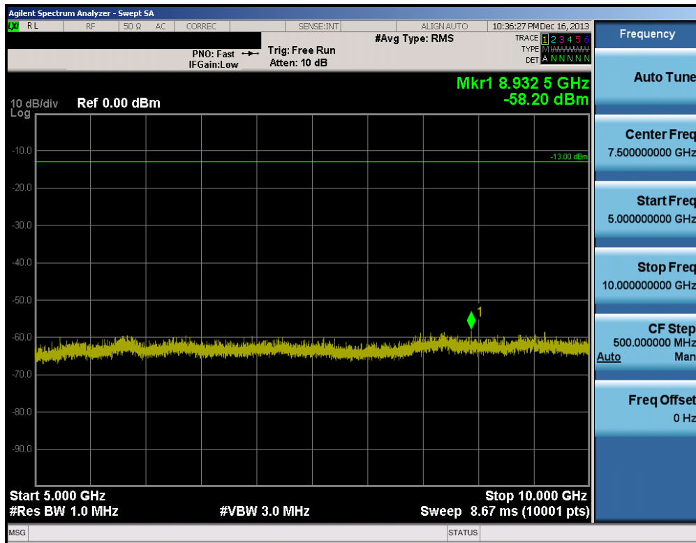
Plot 8-11. Conducted Spurious Plot (3.0MHz QPSK – RB Size 1, RB Offset 0 – Mid Channel)
