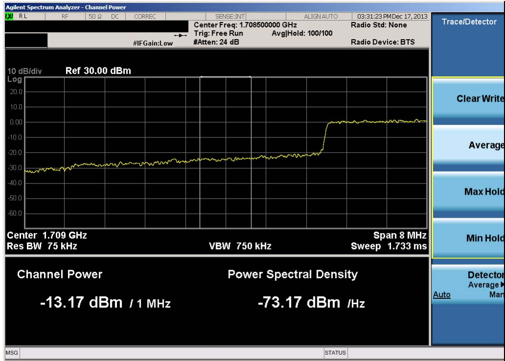
Plot 9-26. Lower Extended Band Edge Plot (10.0MHz QPSK – RB Size 50)
