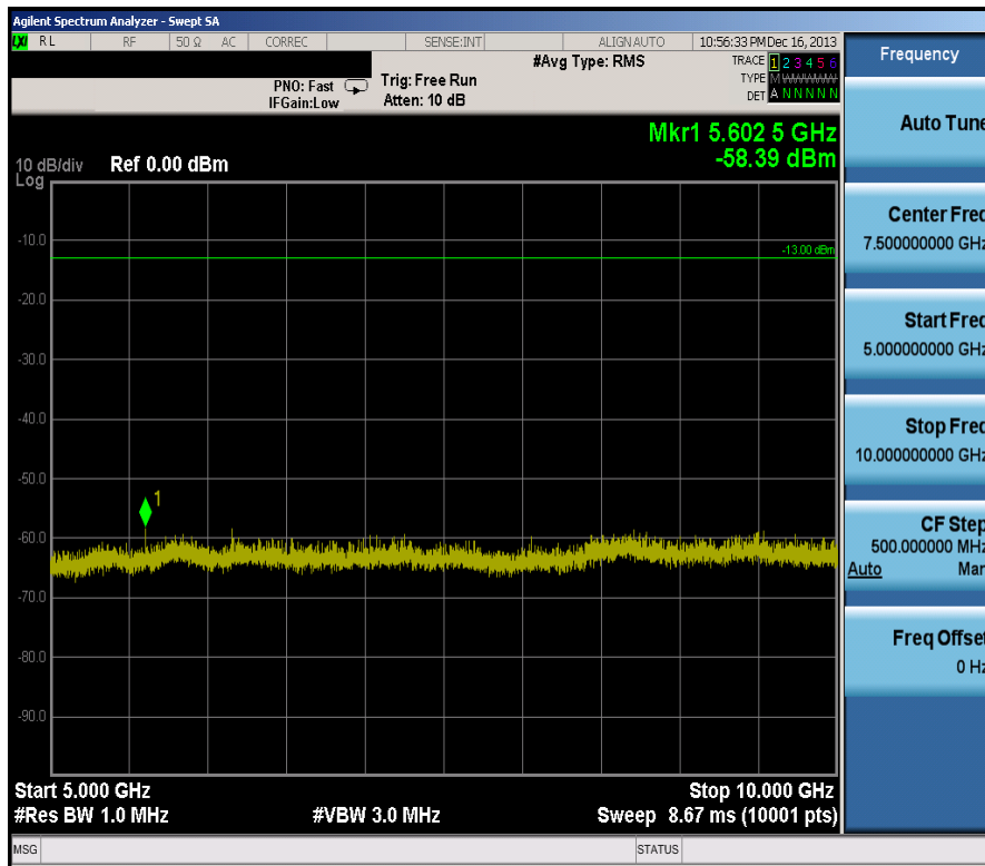
Plot 7-7. Conducted Spurious Plot (5.0MHz QPSK – RB Size 1, RB Offset 0 – Mid Channel)
