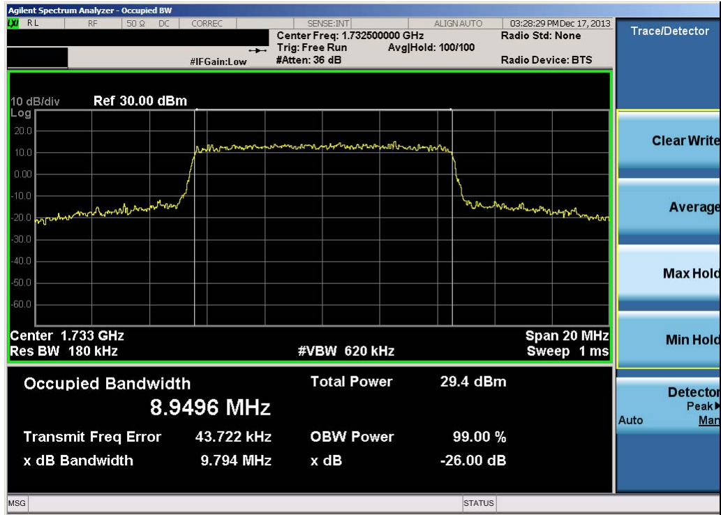
Plot 9-28. Occupied Bandwidth Plot (10.0MHz 16-QAM – RB Size 50)
