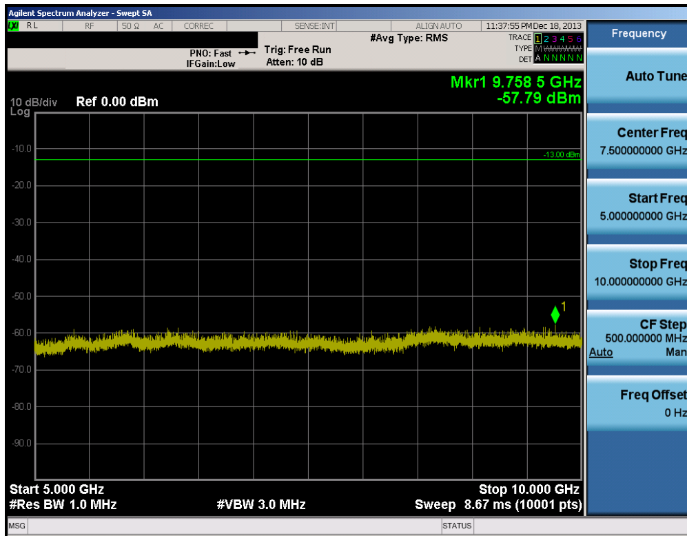
Plot 8-13. Conducted Spurious Plot (3.0MHz QPSK – RB Size 1, RB Offset 0 – High Channel)
