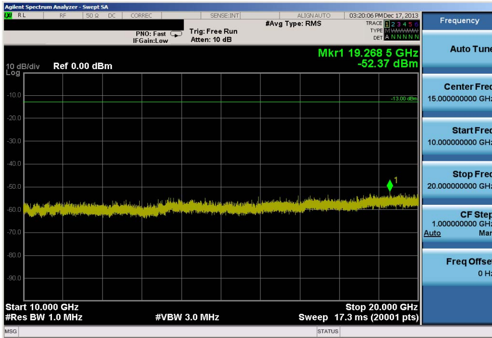
Plot 9-30. Conducted Spurious Plot (10.0MHz QPSK – RB Size 1, RB Offset 0 – Low Channel)
