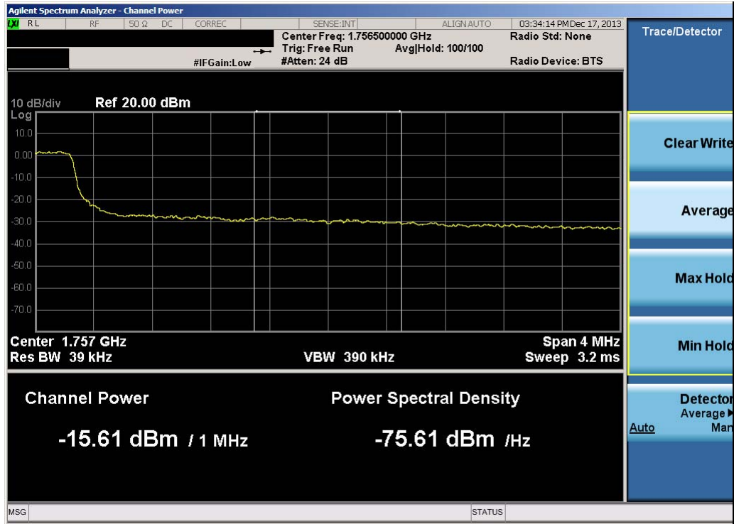
Plot 9-22. Upper Extended Band Edge Plot (5.0MHz QPSK – RB Size 25)
