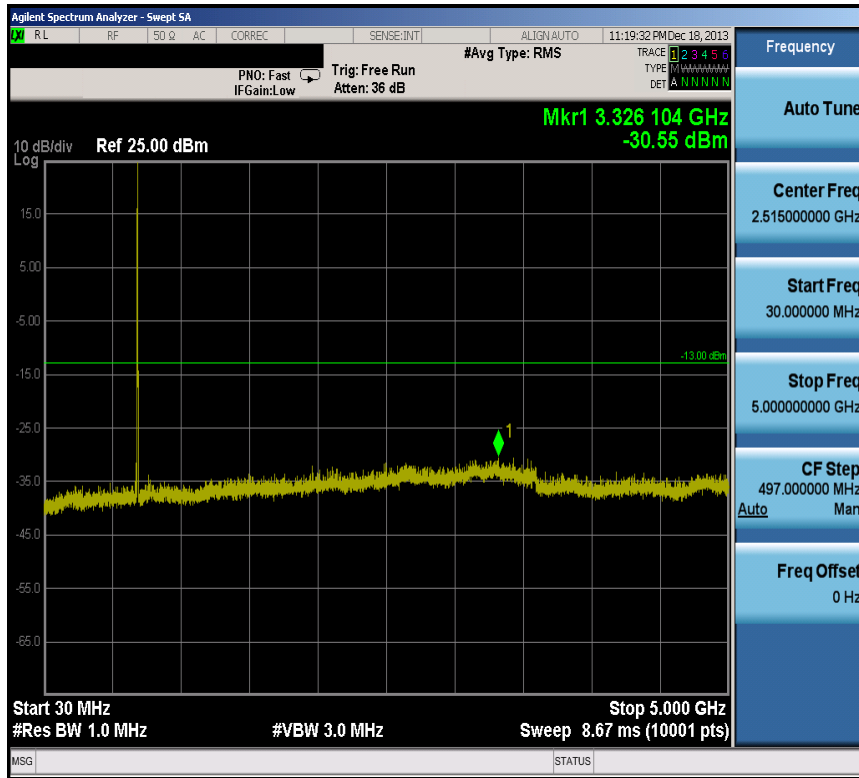
Plot 7-8. Conducted Spurious Plot (5.0MHz QPSK – RB Size 1, RB Offset 0 – High Channel)
