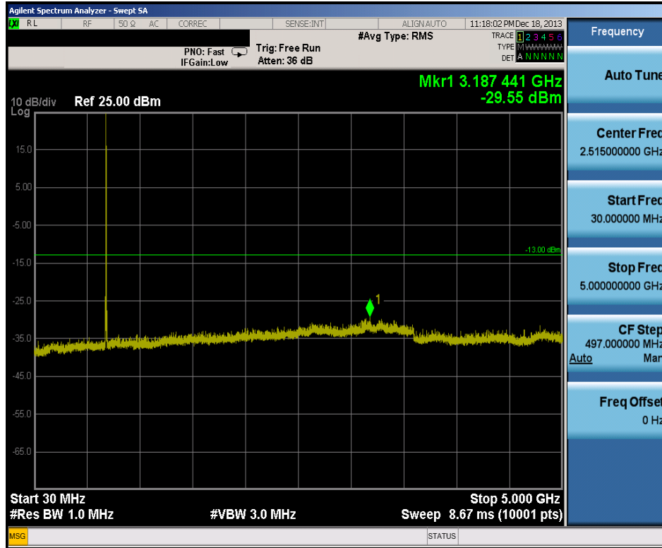
Plot 7-4. Conducted Spurious Plot (5.0MHz QPSK – RB Size 1, RB Offset 0 – Low Channel)
