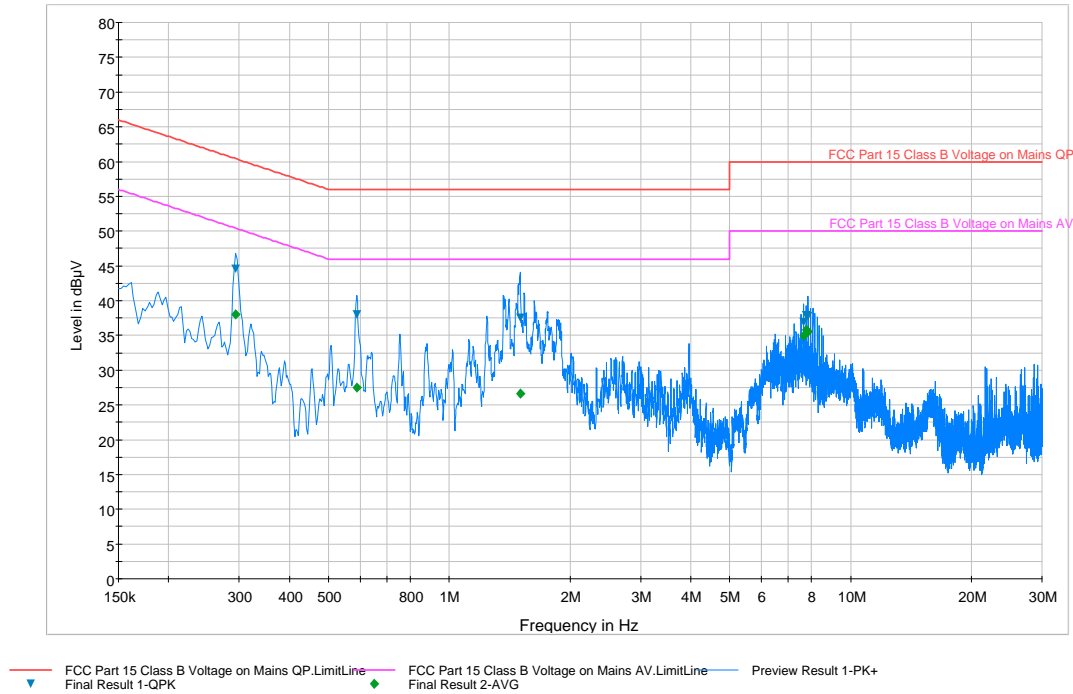
Plot 6-70. Line Conducted Plot with 802.11a UNII Band 1 (L1)
