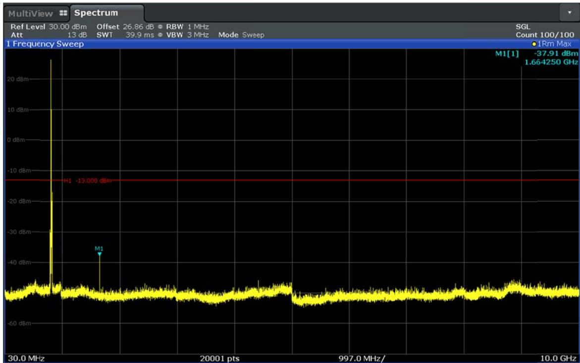
Plot 6-19. Conducted Spurious Plot (Band 5–10.0MHz–QPSK–RB Size 1–RB Offset 24– Ch.20525)
