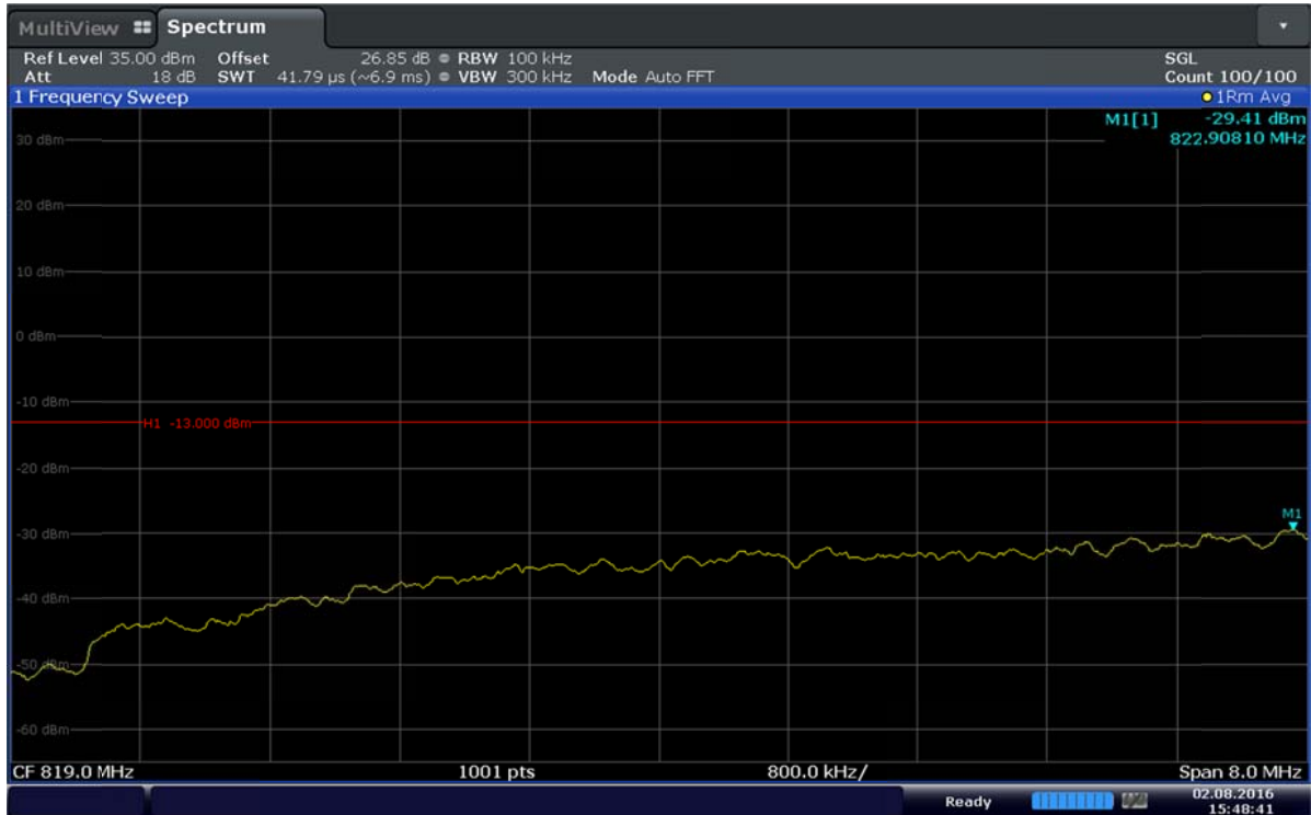
Plot 6-34. . Extended Lower Band Edge Plot (Band 5 – 10.0MHz – QPSK – RB Size 50)
