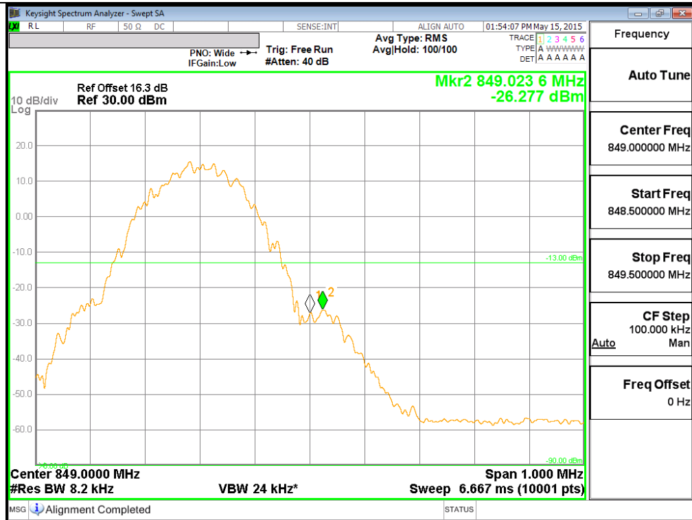
GSM850 GPRS High channel
