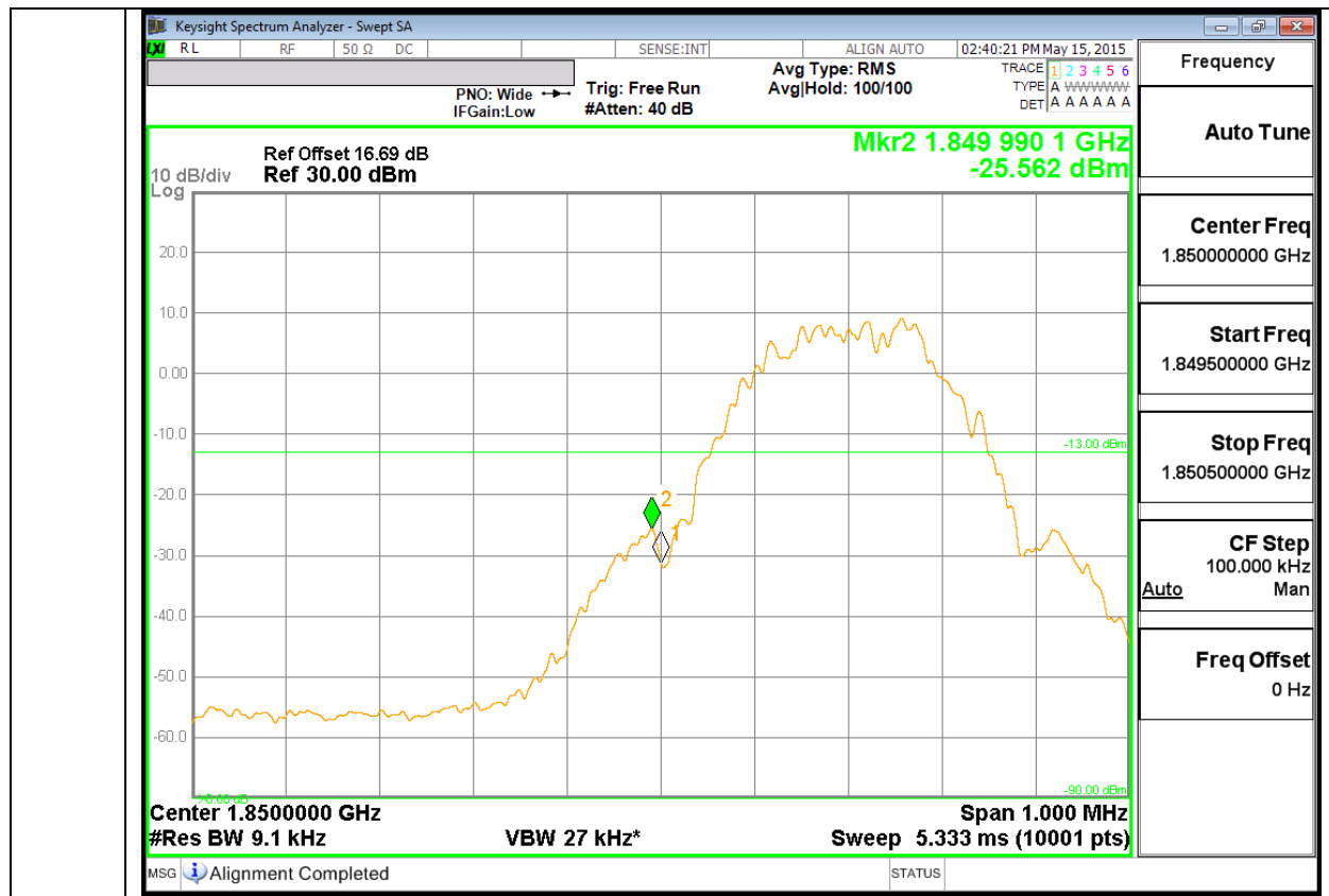
GSM1900 GPRS Low channel
