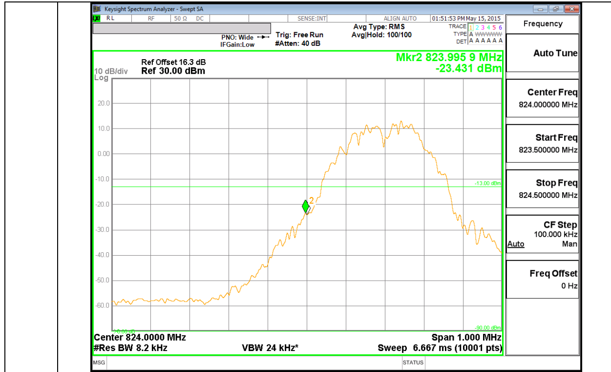
GSM850 GPRS Low channel
