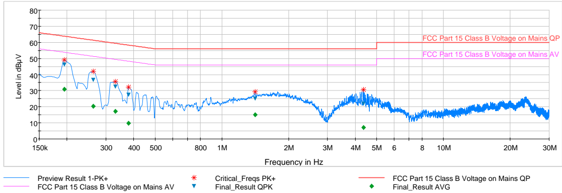
Plot 7-2. Line Conducted Plot (LN)
