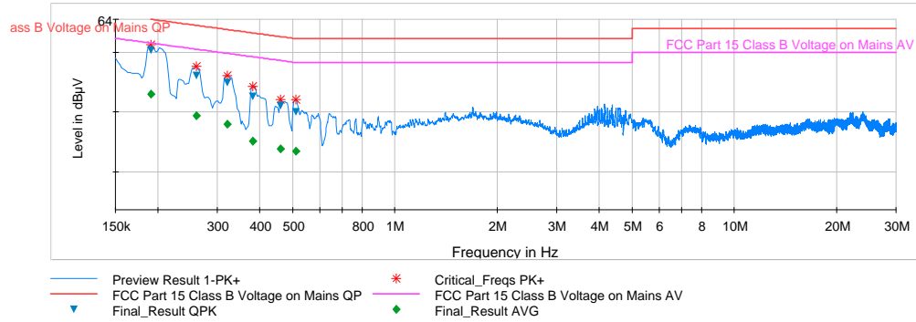
Plot 7-1. Line Conducted Plot (L1)
