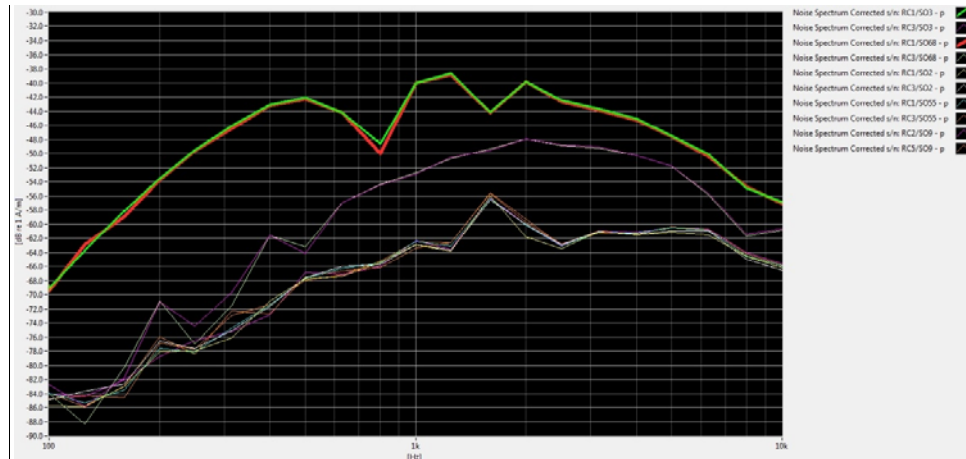
Figure 6-1 CDMA Audio Band Magnetic Noise
