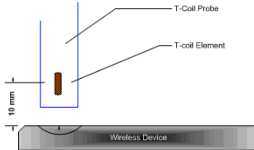
Figure 5-10 Measurement Distance
