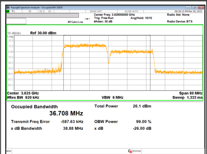
LTE B48 20MHz + 20MHz 16QAM RB100-0 + RB100-0
