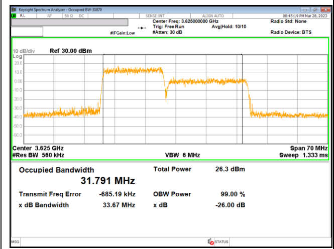
LTE B48 15MHz + 20MHz 16QAM RB100-0 + RB100-0
