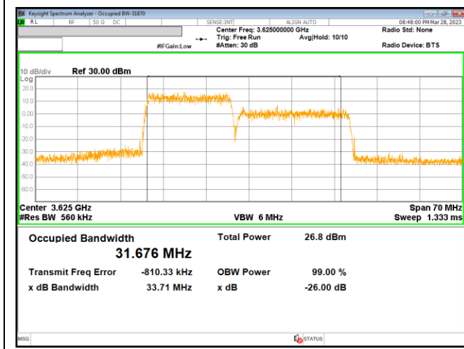
LTE B48 15MHz + 20MHz QPSK RB100-0 + RB100-0
