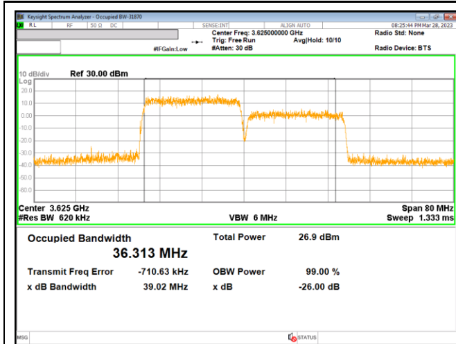
LTE B48 20MHz + 20MHz QPSK RB100-0 + RB100-0
