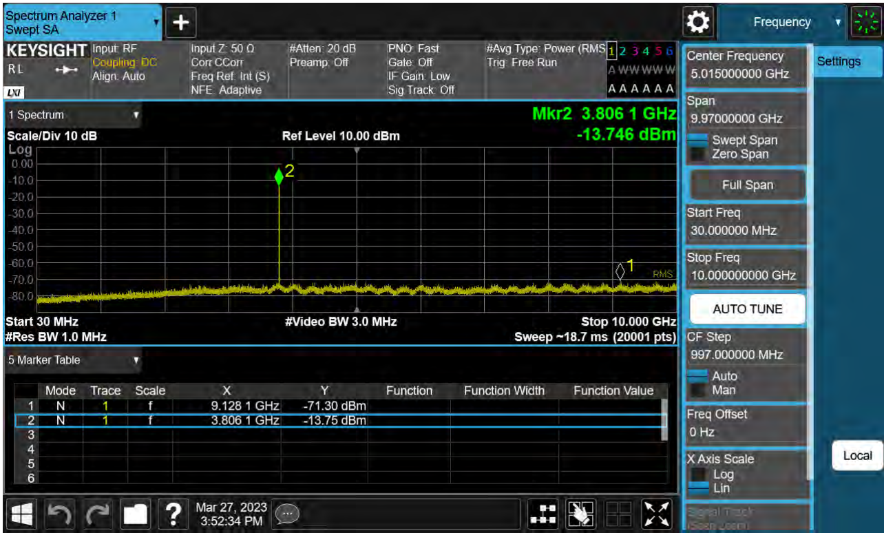
Sub6 n77. Conducted Spurious Plot_1 (656000ch_70 MHz_BPSK)
