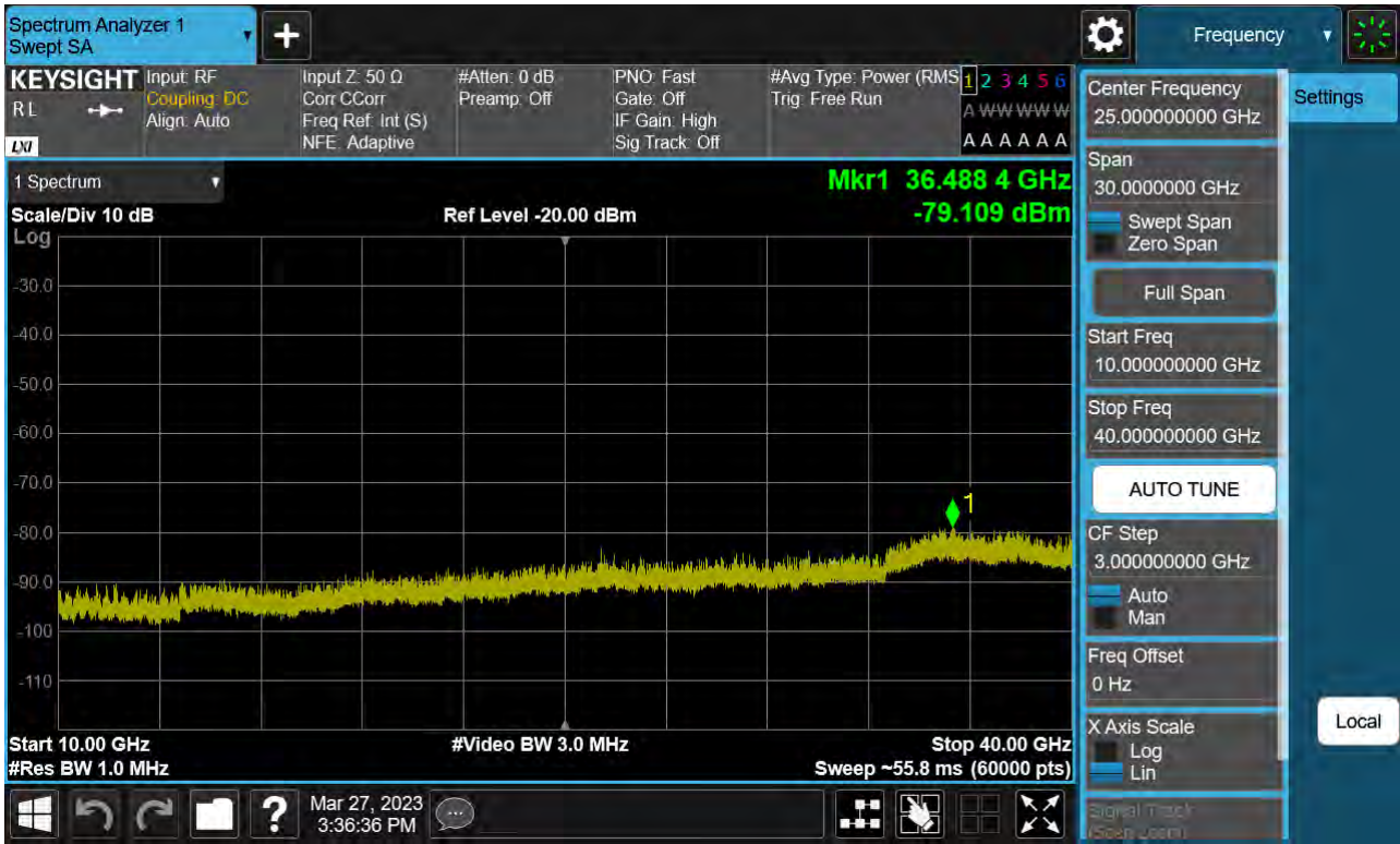
Sub6 n77. Conducted Spurious Plot_2 (648668ch_60 MHz_BPSK)
