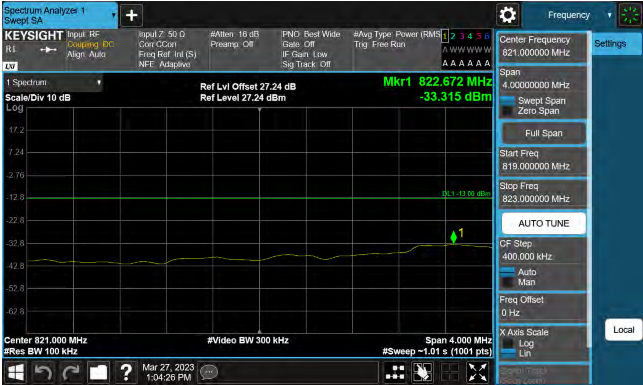
Sub6 n5. Lower Extended Band Edge Plot (20 M BW Ch.166800 BPSK_RB100_0)
