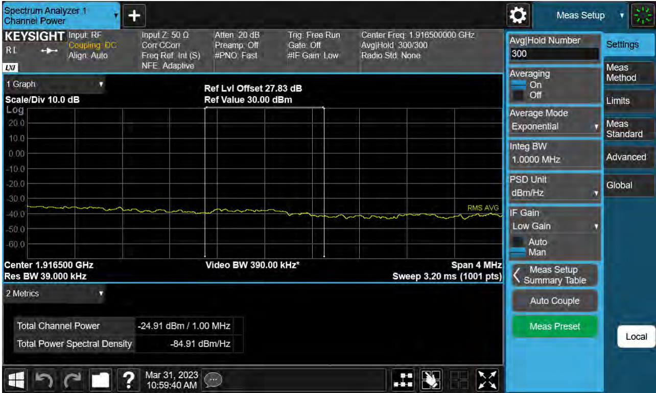
Sub6 n25(2). Upper Extended Band Edge Plot (15 M BW Ch.381500 BPSK_RB75_0) -2
