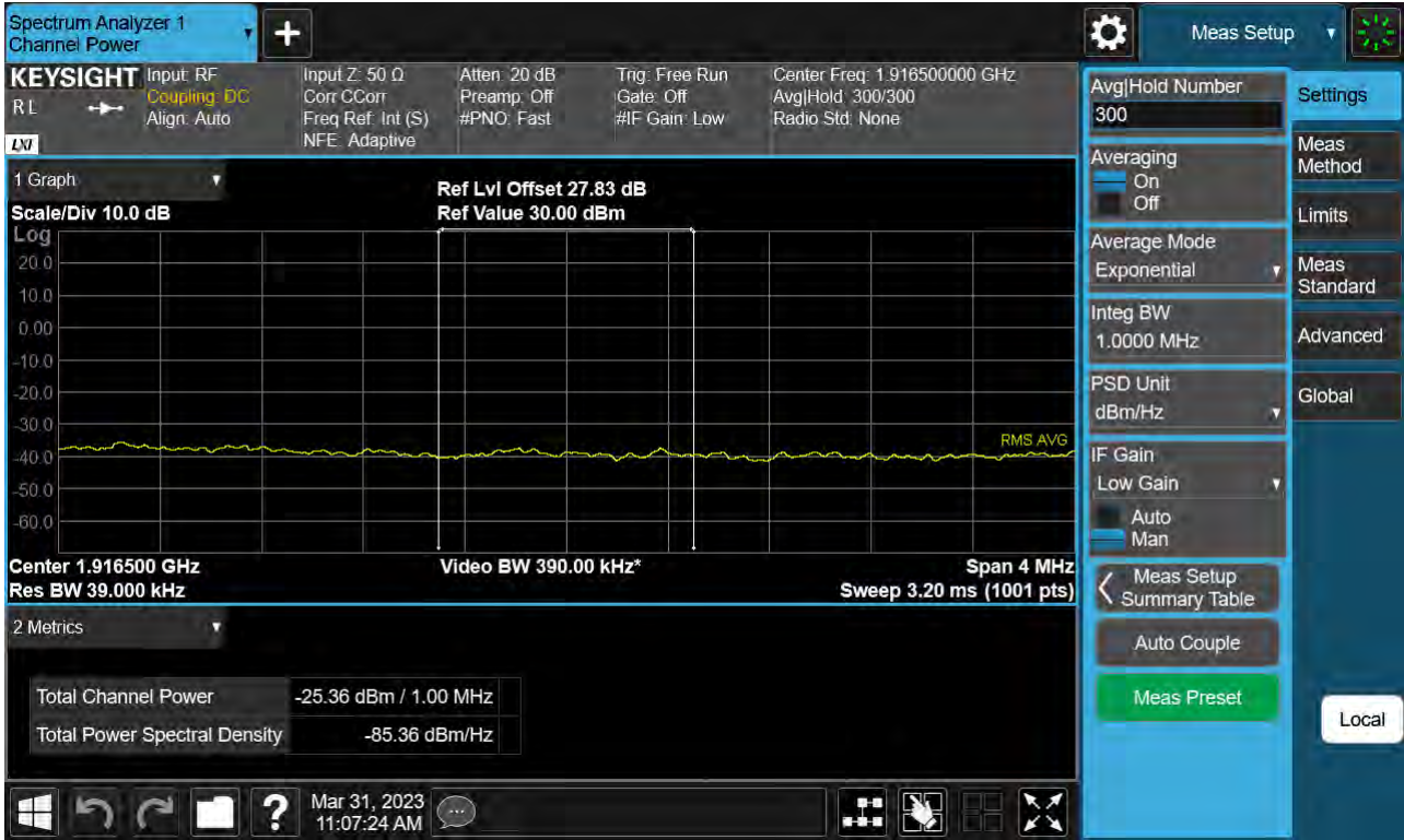
Sub6 n25(2). Upper Extended Band Edge Plot (20 M BW Ch.381000 BPSK_RB100_0) -2
