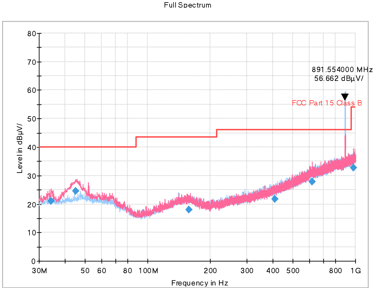
Figure 1: [EUT_Unfolded+TA] LTE B5+5G NR n5 High ch Idle
