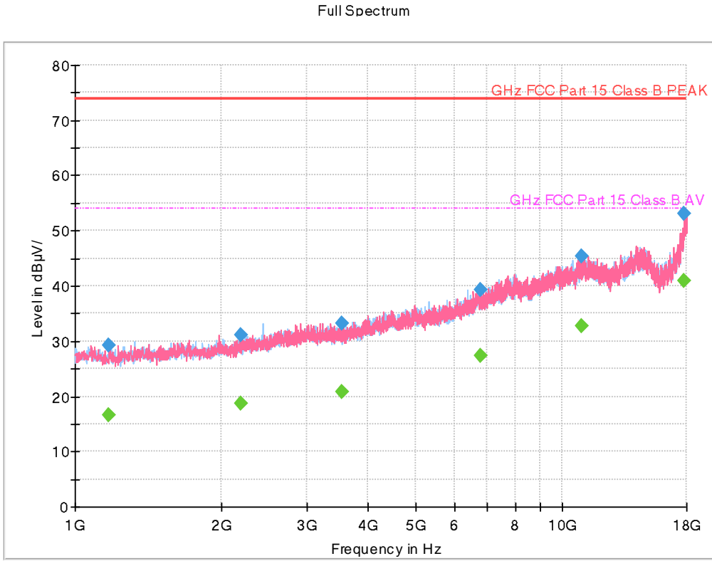
Figure 7: [EUT_Folded+ TA] LTE B5+5G NR n5 High ch Idle
