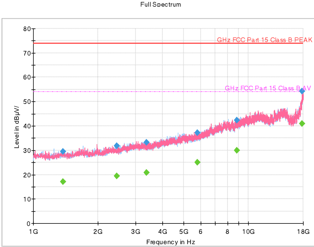
Figure 6: [EUT_Unfolded+TA] LTE B5+5G NR n5 High ch Idle
