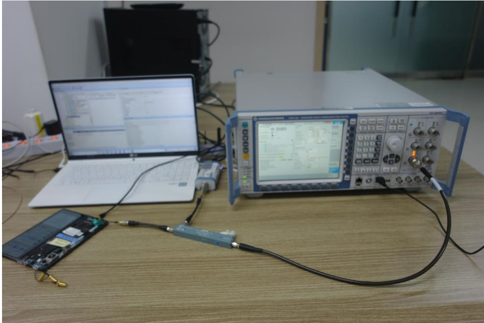
Test setup photo-1 (7-1(a) Legacy)
