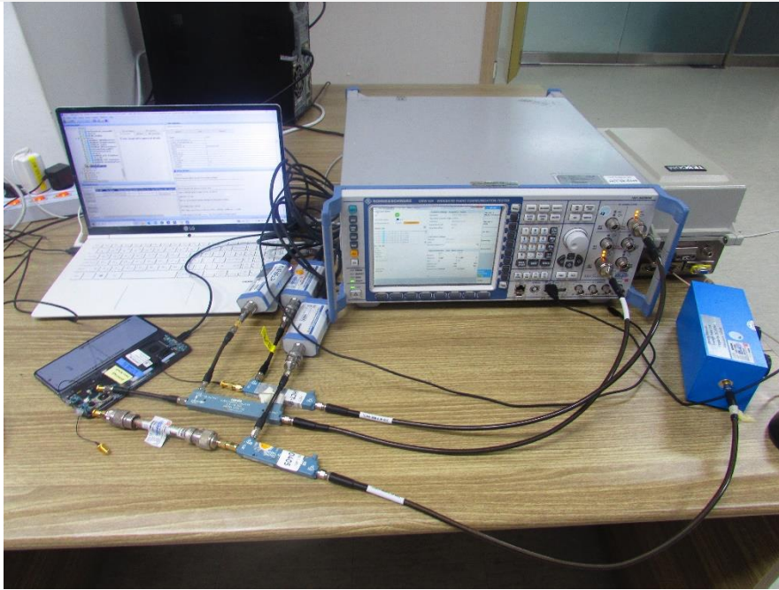
Test setup photo- (7-1 (f) System level compliance continuity)
