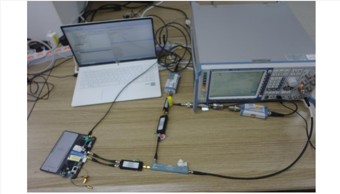
Test setup photo- (7-1(c) Legacy Inter ULCA)
