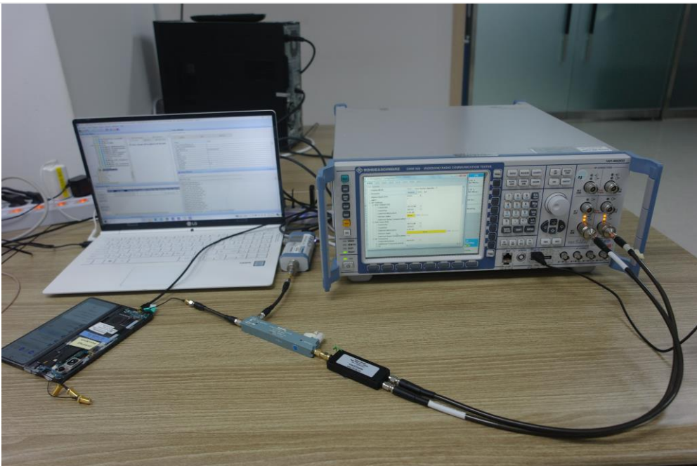
Test setup photo-2 (7-1(b) Legacy)
