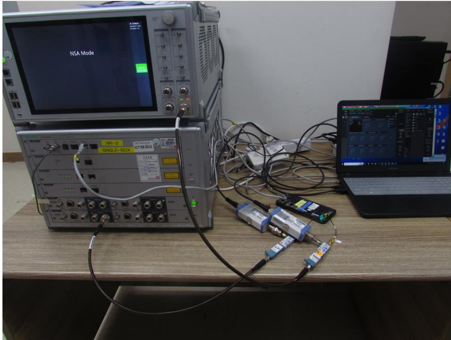
Test setup photo-4 (7-1(c) 5G Sub 6)
