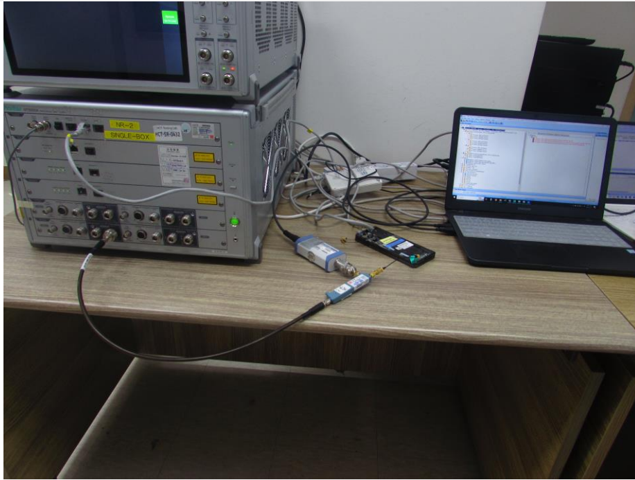
Test setup photo-3 (7-1(a) 5G Sub 6 setup)
