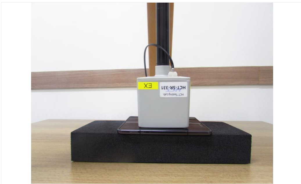
H Field Front side
