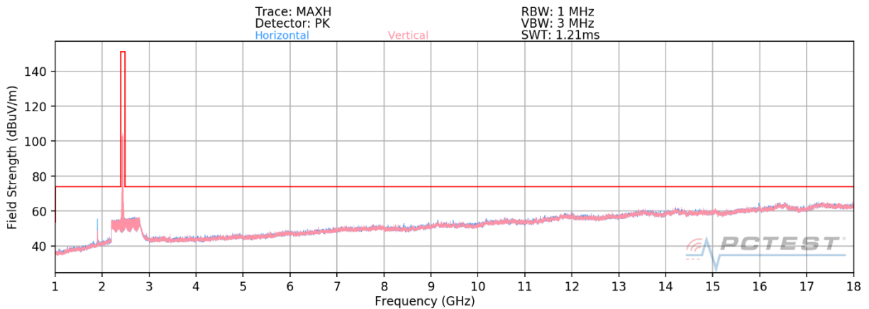
Plot 7-88. Radiated Spurious Plot above 1GHz SISO ANT2 (802.11ax OFDMA – 242 Tones – Ch. 6) – OPEN (Q)
