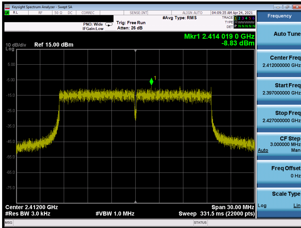
Plot 7-40. Power Spectral Density Plot MIMO ANT1 (802.11ax OFDMA – 242 Tones – Ch. 1) - N
