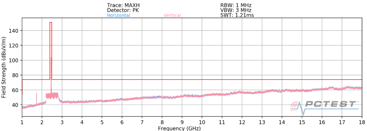
Plot 7-89. Radiated Spurious Plot above 1GHz SISO ANT2 (802.11ax OFDMA – 242 Tones – Ch. 11) – OPEN (Q)
