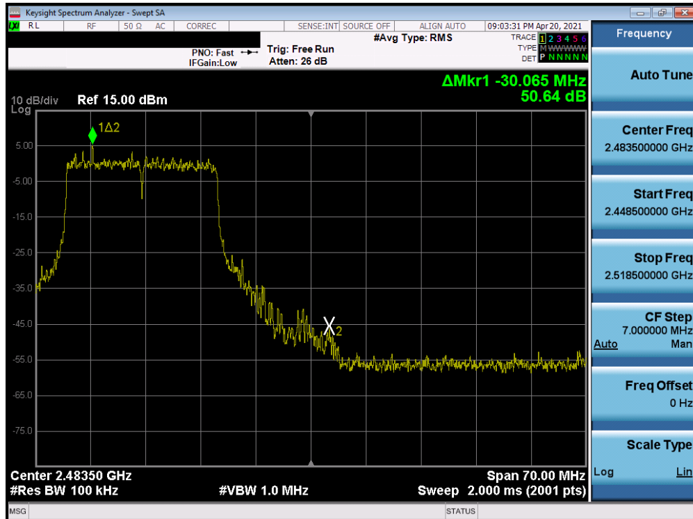
Plot 7-52. Band Edge Plot SISO ANT2 (802.11ax OFDMA – 242 Tones – Ch. 11) - Q
