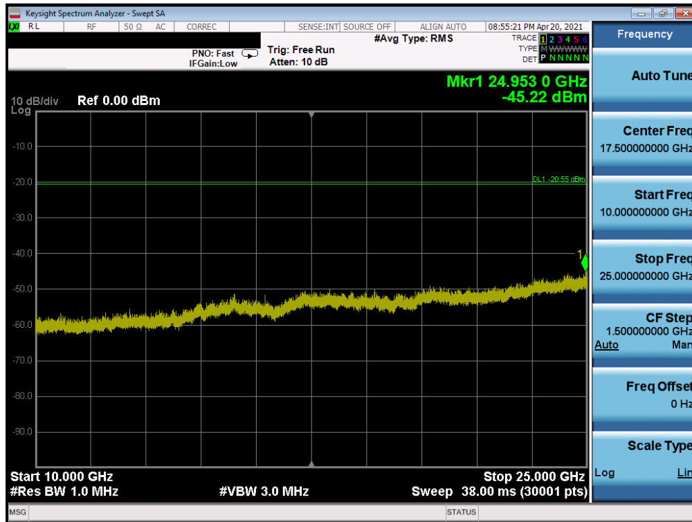
Plot 7-62. Conducted Spurious Plot SISO ANT2 (802.11ax OFDMA – 26 Tones – Ch. 11) - Q
