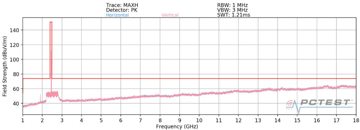
Plot 7-83. Radiated Spurious Plot above 1GHz SISO ANT2 (802.11ax OFDMA – 26 Tones – Ch. 11) – OPEN (Q)
