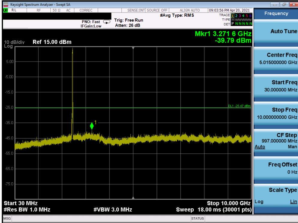
Plot 7-67. Conducted Spurious Plot SISO ANT2 (802.11ax OFDMA – 242 Tones – Ch. 11) - Q
