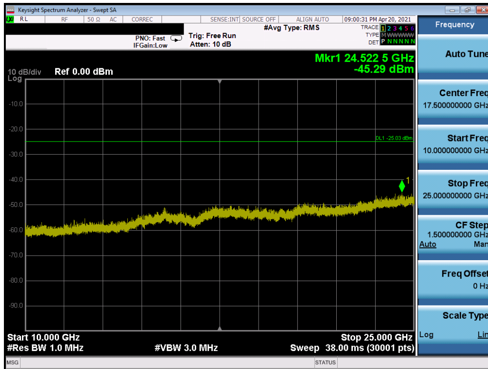
Plot 7-64. Conducted Spurious Plot SISO ANT2 (802.11ax OFDMA – 242 Tones – Ch. 1) - Q
