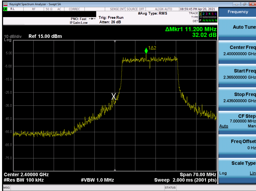
Plot 7-51. Band Edge Plot SISO ANT2 (802.11ax OFDMA – 242 Tones – Ch. 1) - Q
