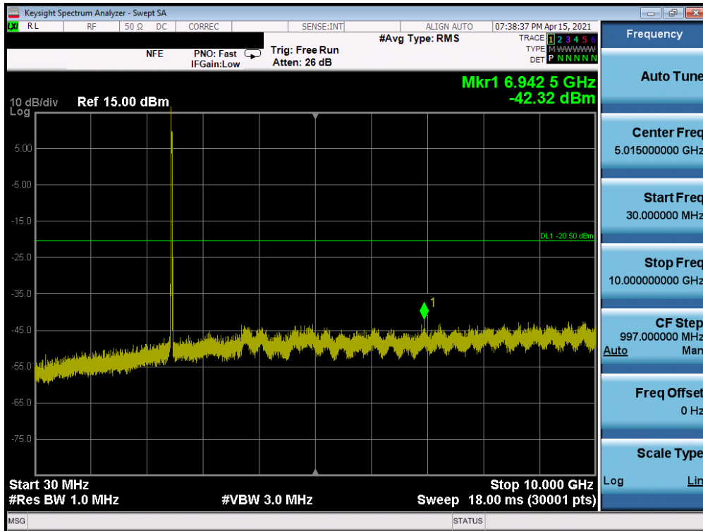
Plot 7-73. Conducted Spurious Plot SISO ANT2 (802.11ax OFDMA – 26 Tones – Ch. 11) - N
