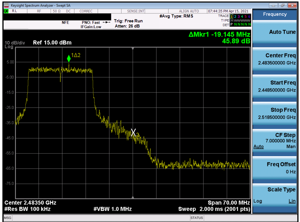
Plot 7-56. Band Edge Plot SISO ANT2 (802.11ax OFDMA – 242 Tones – Ch. 11) - N
