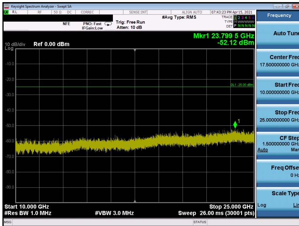
Plot 7-76. Conducted Spurious Plot SISO ANT2 (802.11ax OFDMA – 242 Tones – Ch. 1) - N
