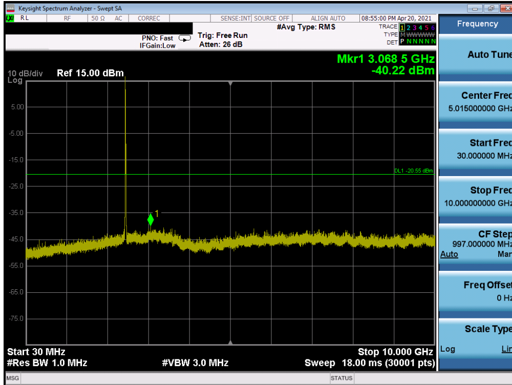
Plot 7-61. Conducted Spurious Plot SISO ANT2 (802.11ax OFDMA – 26 Tones – Ch. 11) - Q
