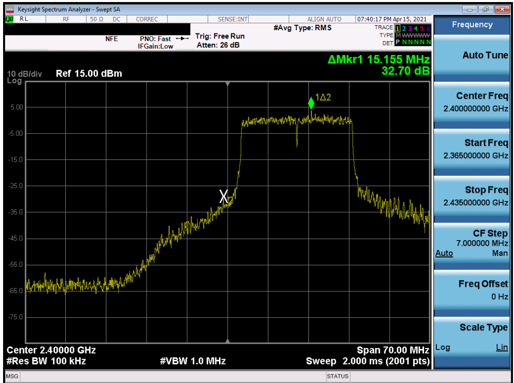
Plot 7-55. Band Edge Plot SISO ANT2 (802.11ax OFDMA – 242 Tones – Ch. 1) - N
