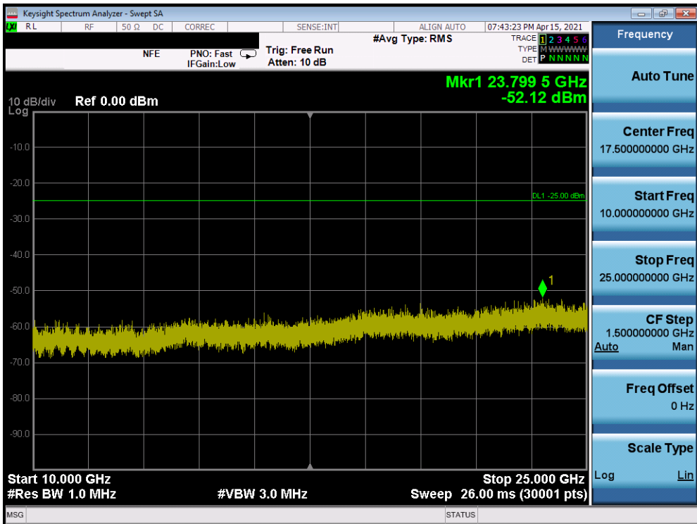
Plot 7-78. Conducted Spurious Plot SISO ANT2 (802.11ax OFDMA – 242 Tones – Ch. 6) - N
