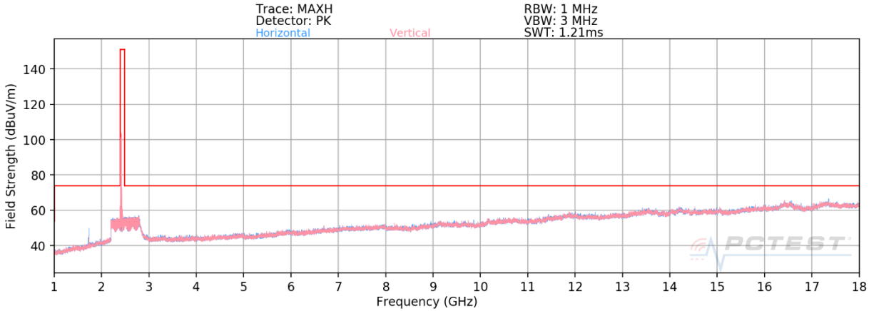
Plot 7-87. Radiated Spurious Plot above 1GHz SISO ANT2 (802.11ax OFDMA – 242 Tones – Ch. 1) – OPEN (Q)
