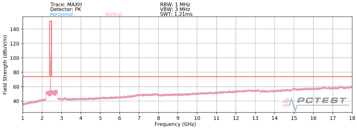
Plot 7-85. Radiated Spurious Plot above 1GHz SISO ANT2 (802.11ax OFDMA – 26 Tones – Ch. 6) – CLOSED (Q)
