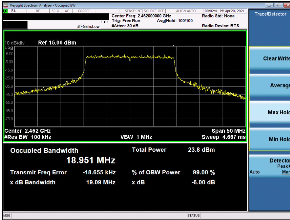
Plot 7-6. 6dB Bandwidth Plot SISO ANT1 (802.11ax OFDMA – 242 Tones – Ch. 11) - Q
