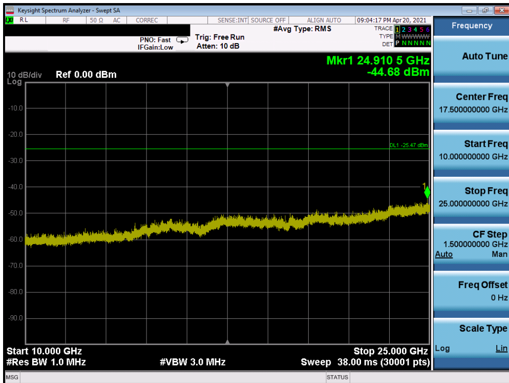
Plot 7-68. Conducted Spurious Plot SISO ANT2 (802.11ax OFDMA – 242 Tones – Ch. 11) - Q
