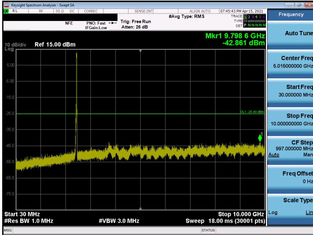
Plot 7-79. Conducted Spurious Plot SISO ANT2 (802.11ax OFDMA – 242 Tones – Ch. 11) - N
