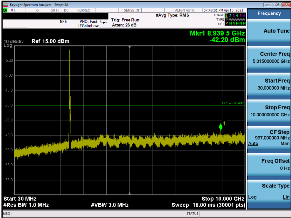
Plot 7-77. Conducted Spurious Plot SISO ANT2 (802.11ax OFDMA – 242 Tones – Ch. 6) - N
