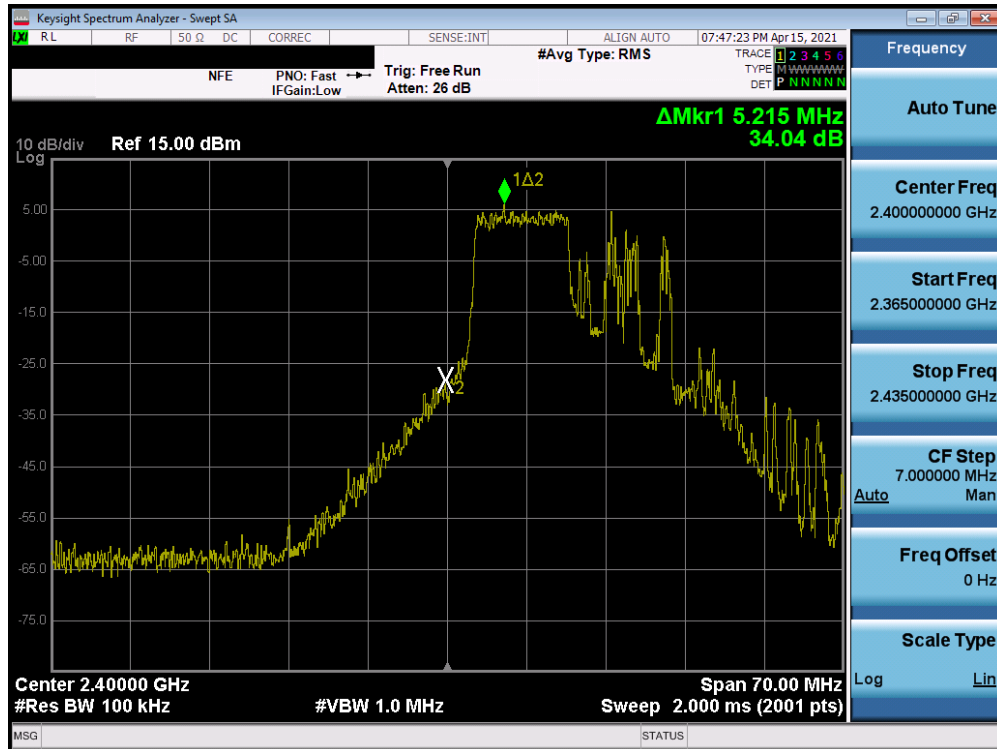
Plot 7-53. Band Edge Plot SISO ANT2 (802.11ax OFDMA – 106 Tones – Ch. 1) - N
