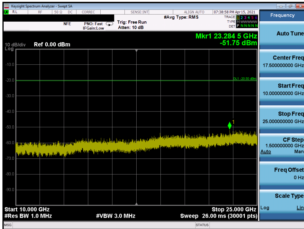
Plot 7-74. Conducted Spurious Plot SISO ANT2 (802.11ax OFDMA – 26 Tones – Ch. 11) - N
