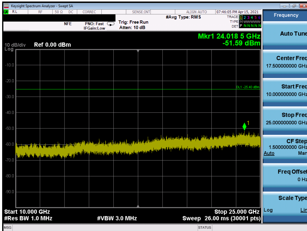
Plot 7-80. Conducted Spurious Plot SISO ANT2 (802.11ax OFDMA – 242 Tones – Ch. 11) - N
