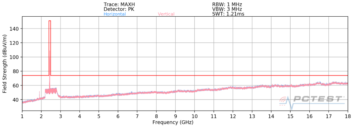
Plot 7-82. Radiated Spurious Plot above 1GHz SISO ANT2 (802.11ax OFDMA – 26 Tones – Ch. 6) – OPEN (Q)
