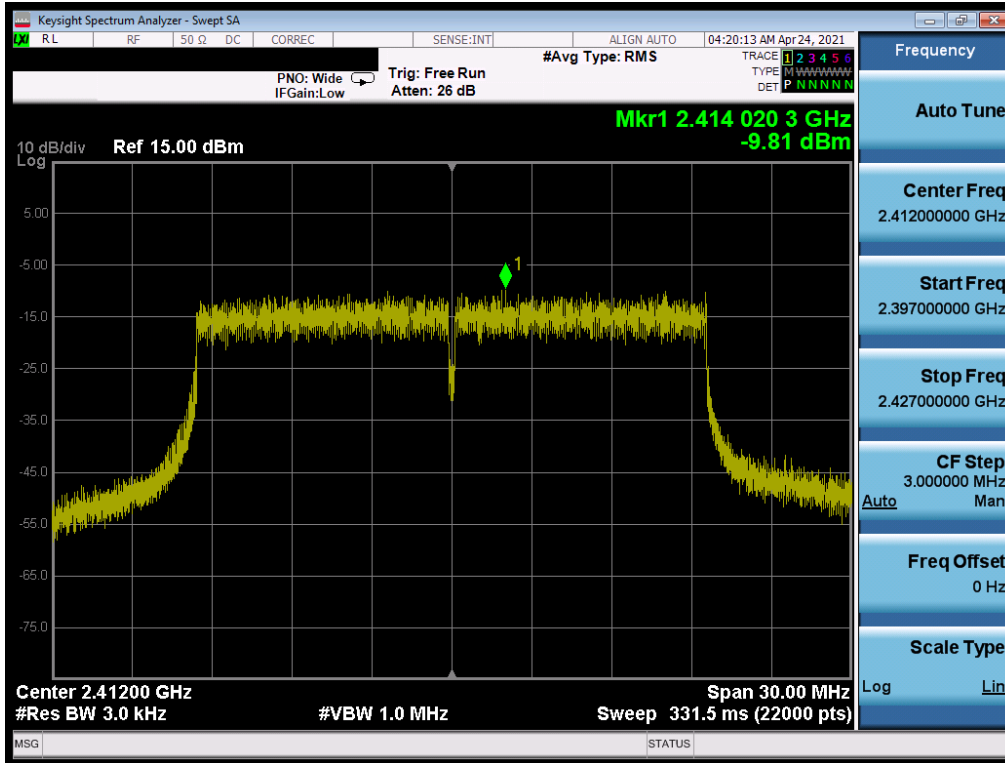
Plot 7-46. Power Spectral Density Plot MIMO ANT2 (802.11ax OFDMA – 242 Tones – Ch. 1) - N
