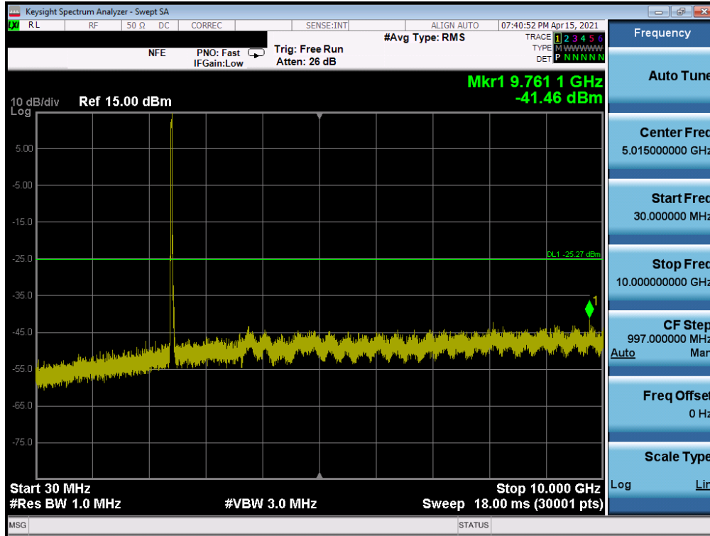
Plot 7-75. Conducted Spurious Plot SISO ANT2 (802.11ax OFDMA – 242 Tones – Ch. 1) - N
