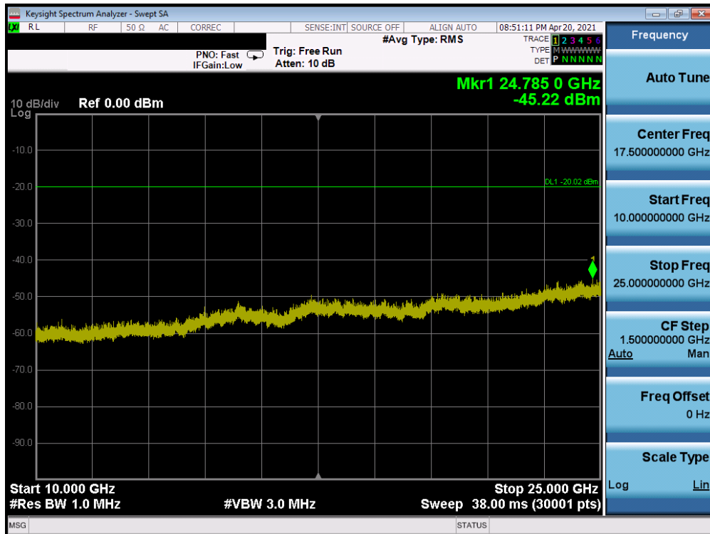
Plot 7-58. Conducted Spurious Plot SISO ANT2 (802.11ax OFDMA – 26 Tones – Ch. 1) - Q
