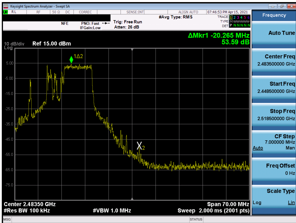
Plot 7-54. Band Edge Plot SISO ANT2 (802.11ax OFDMA – 106 Tones – Ch. 11) - N
