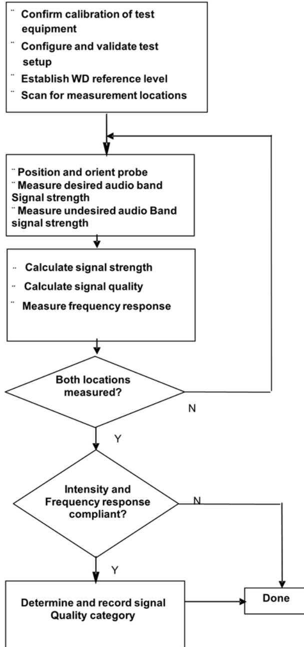
Figure 4-13 C63.19 T-Coil Signal Test Process
