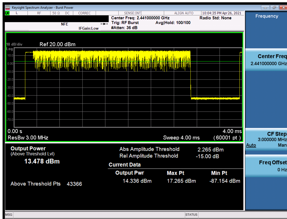
Plot 7-104. Average Conducted Power (3Mbps, ePA - Ch. 39) - ANT1
