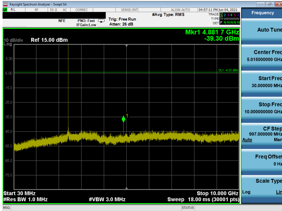
Plot 7-149. Conducted Spurious Plot (Bluetooth, 1Mbps – Ch. 39, iPA) – ANT0
