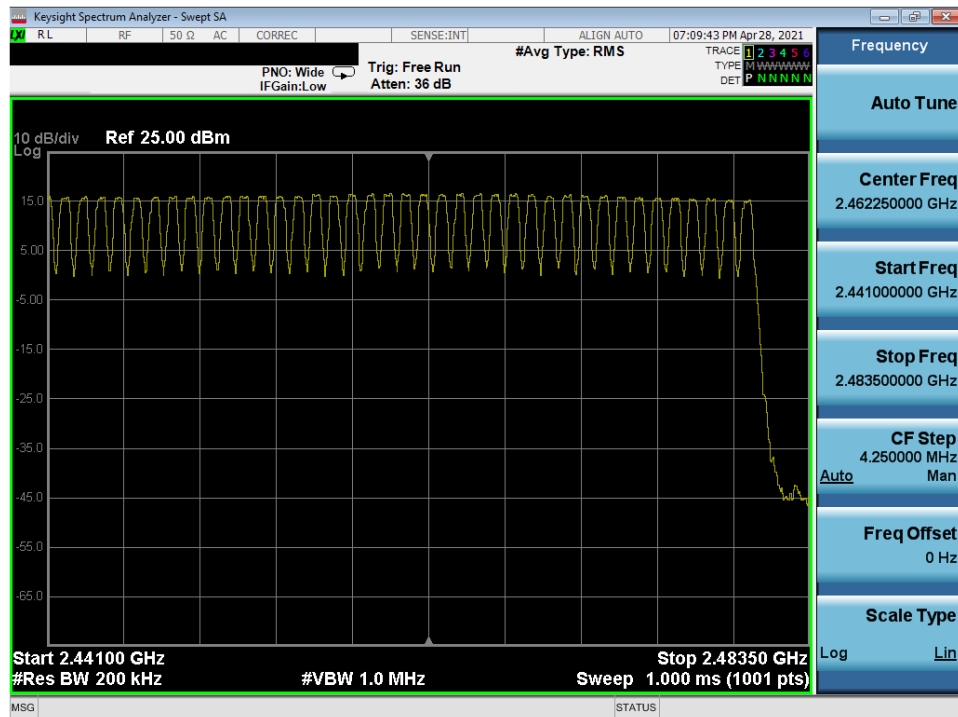
Plot 7-134. High End Spectrum Channel Hopping Plot (Bluetooth, ePA) – ANT0
