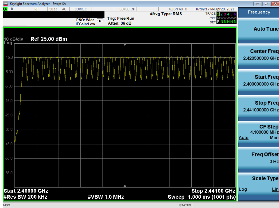
Plot 7-133. Low End Spectrum Channel Hopping Plot (Bluetooth, ePA) – ANT0
