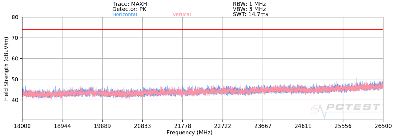
Plot 7-171. Radiated Spurious Plot above 18GHz – OPEN
