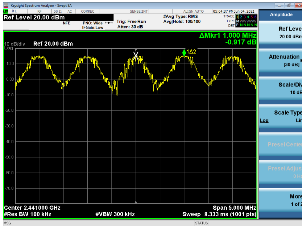
Plot 7-126. Channel Spacing Plot (Bluetooth, iPA) – ANT0
