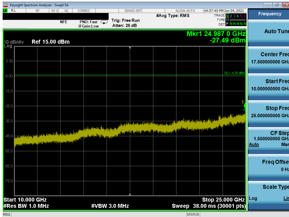
Plot 7-150. Conducted Spurious Plot (Bluetooth, 1Mbps – Ch. 39, iPA) – ANT0
