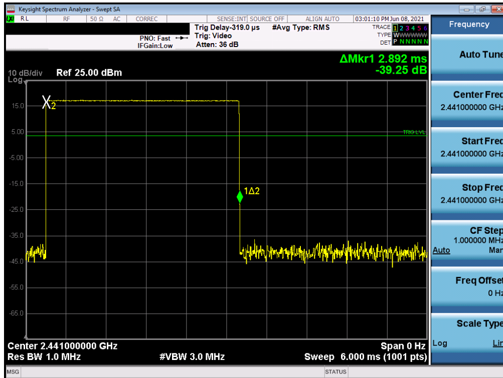
Plot 7-130. Time of Occupancy Plot (Bluetooth, iPA) – ANT0
