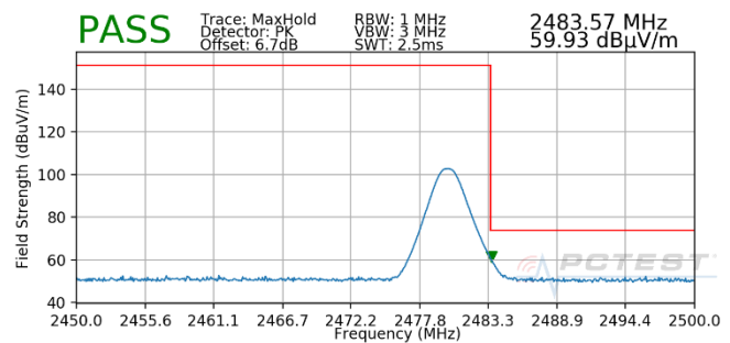
Plot 7-174. Radiated Restricted Upper Band Edge Measurement (Peak) – ANT0
