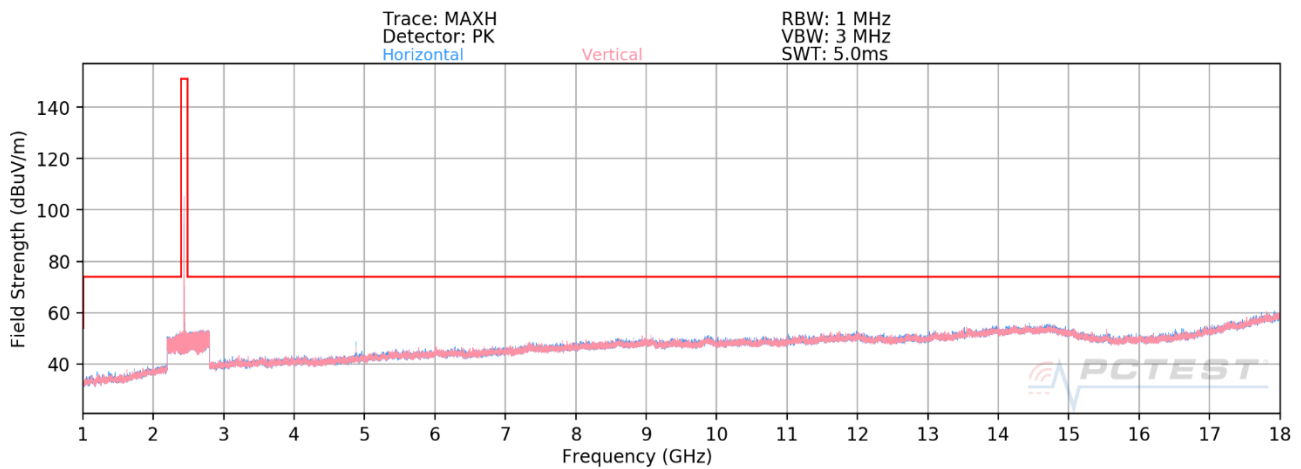
Plot 7-166. Radiated Spurious Plot above 1GHz (BT- Ch. 39) -- OPEN
