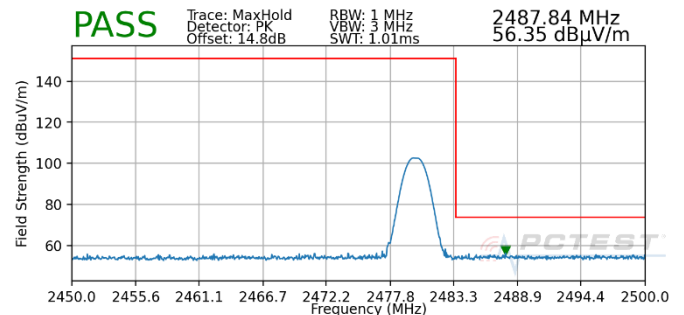
Plot 7-180. Radiated Restricted Upper Band Edge Measurement with WCP (Peak) – ANT1
