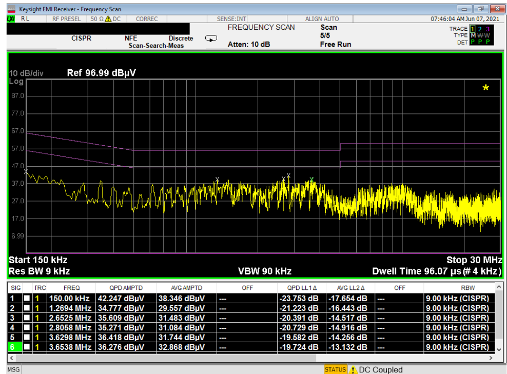
Plot 7-186. Line-Conducted Test Plot with WCP (N)
