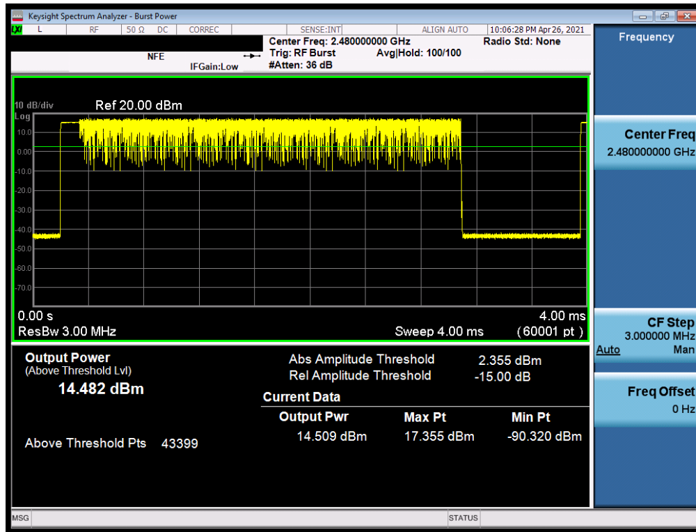
Plot 7-105. Average Conducted Power (3Mbps, ePA - Ch. 78) - ANT1
