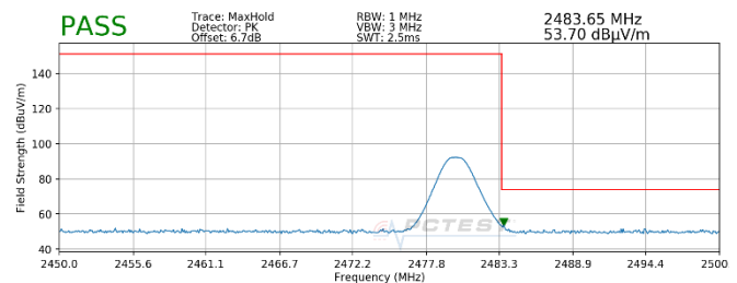
Plot 7-52. Radiated Restricted Upper Band Edge Measurement (Peak) - Open
