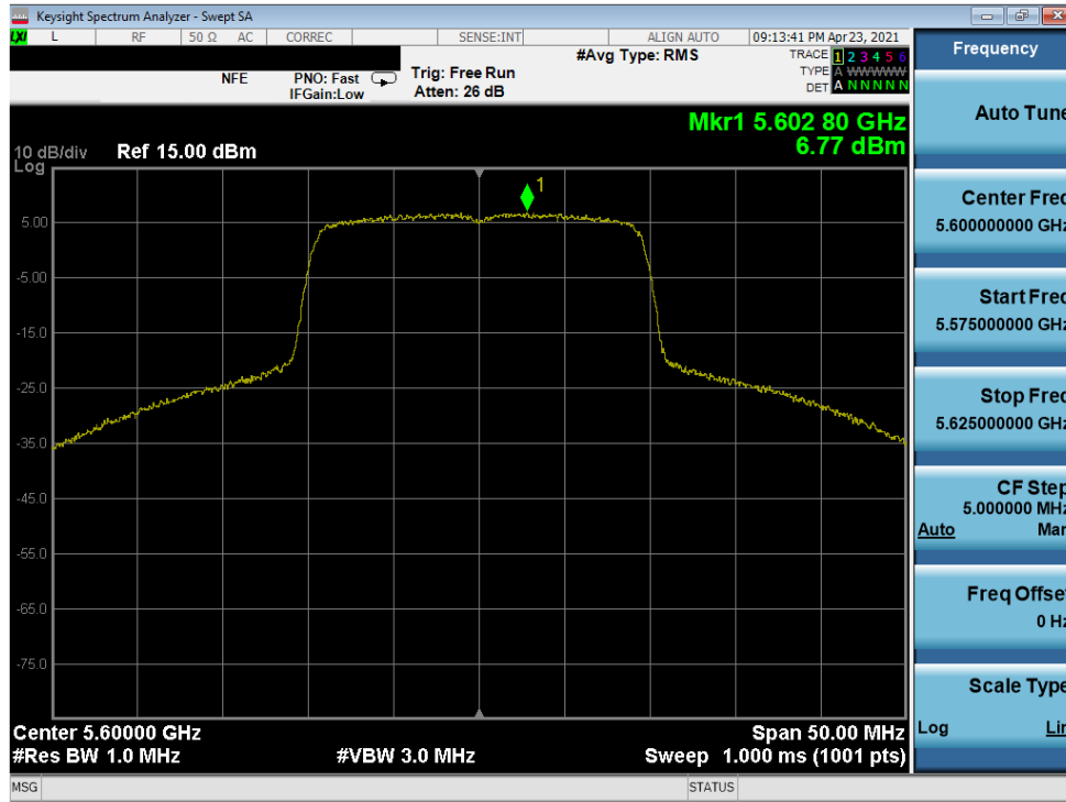
Plot 7-287. Power Spectral Density Plot MIMO ANT2 (20MHz 802.11ax (UNII Band 2C) – Ch. 120)
