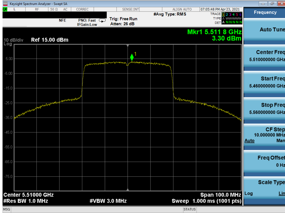
Plot 7-241. Power Spectral Density Plot MIMO ANT1 (40MHz 802.11ax (UNII Band 2C) – Ch. 102)
