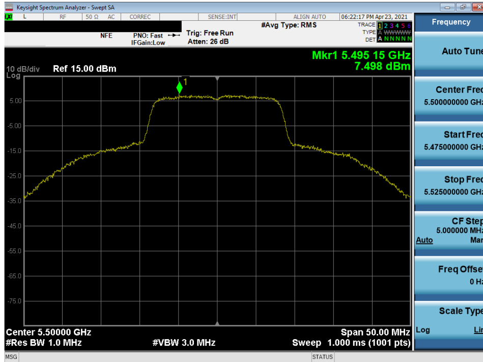
Plot 7-229. Power Spectral Density Plot MIMO ANT1 (20MHz 802.11a (UNII Band 2C) – Ch. 100)
