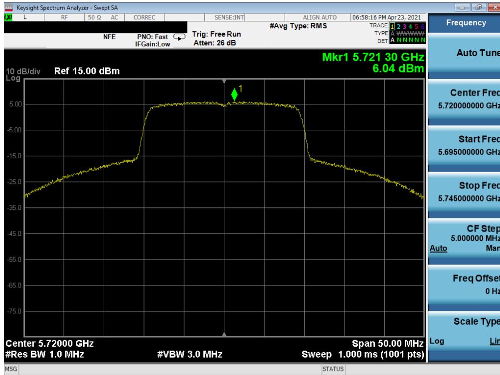
Plot 7-237. Power Spectral Density Plot MIMO ANT1 (20MHz 802.11ax (UNII Band 2C) – Ch.144)
