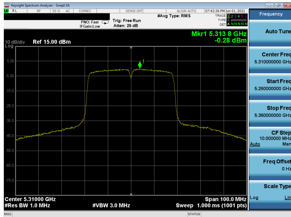
Plot 7-224. Power Spectral Density Plot MIMO ANT1 (40MHz 802.11n (UNII Band 2A) – Ch. 62)
