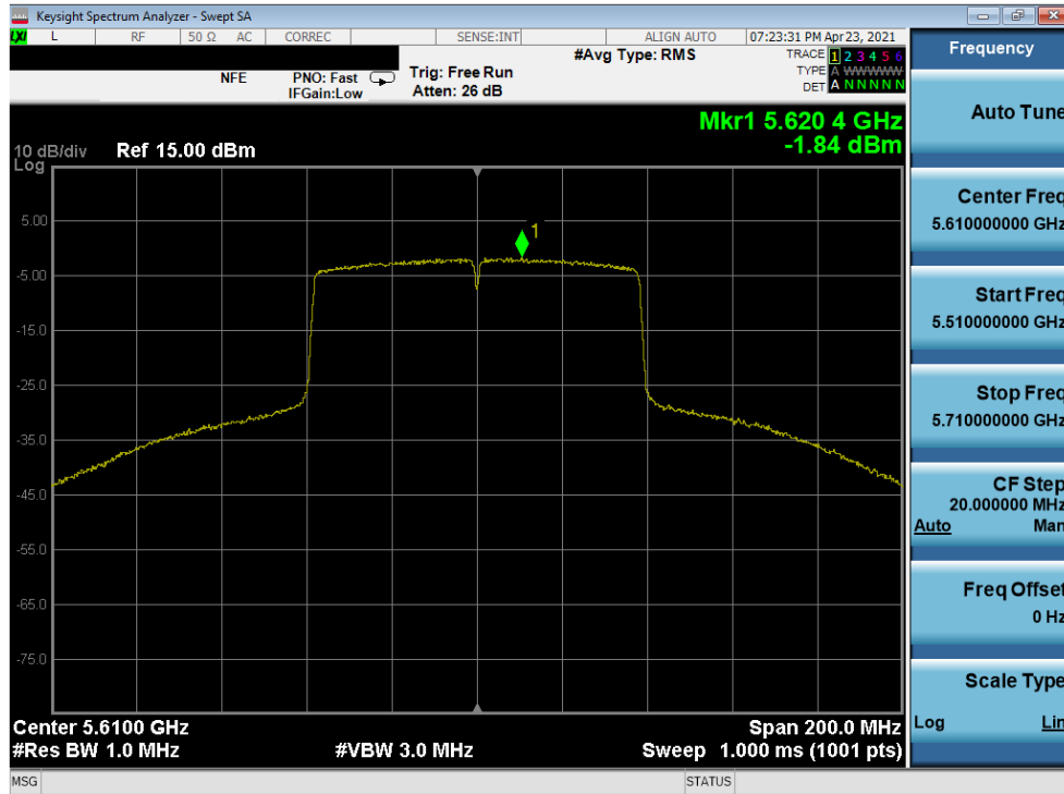
Plot 7-245. Power Spectral Density Plot MIMO ANT1 (80MHz 802.11ac (UNII Band 2C) – Ch. 122)
