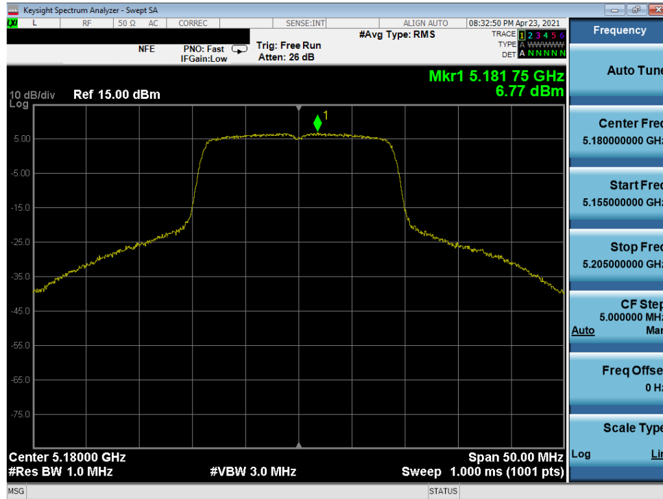
Plot 7-253. Power Spectral Density Plot MIMO ANT2 (20MHz 802.11n (UNII Band 1) – Ch. 36)
