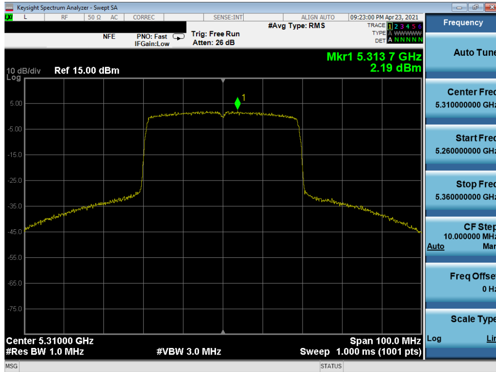
Plot 7-277. Power Spectral Density Plot MIMO ANT2 (40MHz 802.11ax (UNII Band 2A) – Ch. 62)
