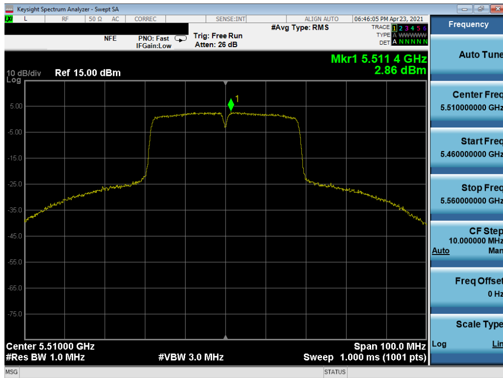
Plot 7-238. Power Spectral Density Plot MIMO ANT1 (40MHz 802.11n (UNII Band 2C) – Ch. 102)
