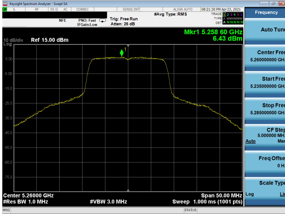
Plot 7-265. Power Spectral Density Plot MIMO ANT2 (20MHz 802.11a (UNII Band 2A) – Ch. 52)
