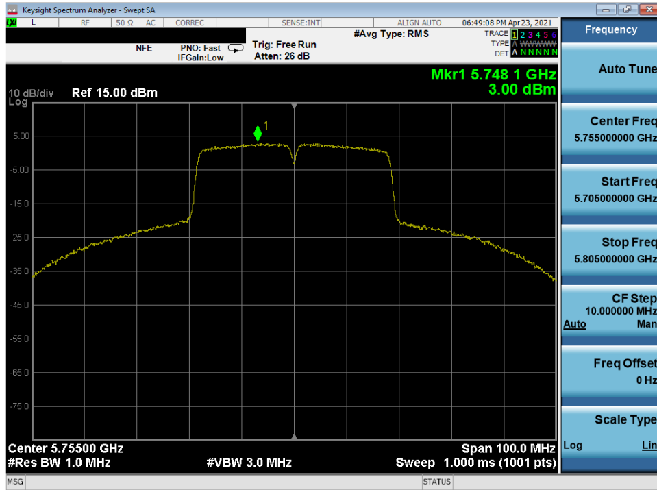
Plot 7-310. Power Spectral Density Plot MIMO ANT1 (40MHz 802.11n (UNII Band 3) – Ch. 151)
