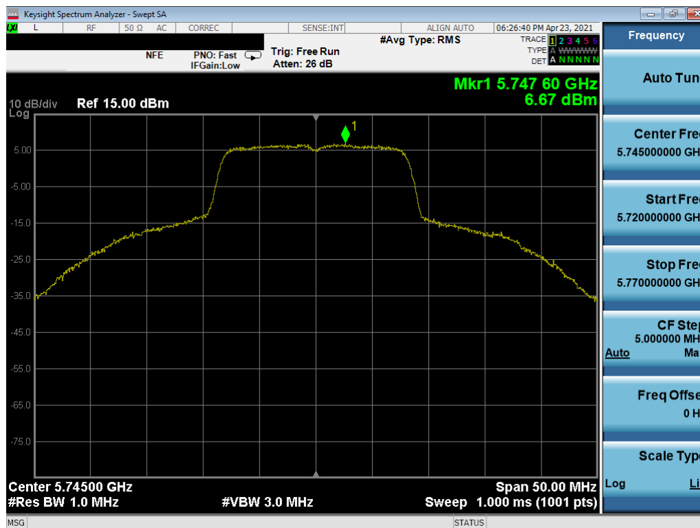
Plot 7-301. Power Spectral Density Plot MIMO ANT1 (20MHz 802.11a (UNII Band 3) – Ch. 149)
