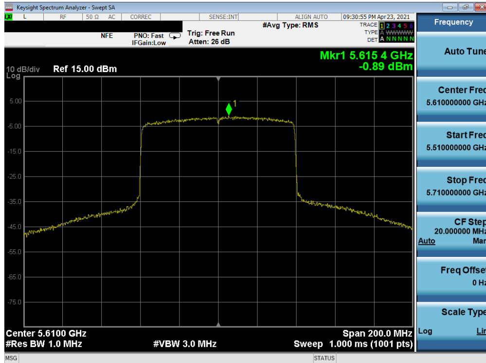
Plot 7-299. Power Spectral Density Plot MIMO ANT2 (80MHz 802.11ax (UNII Band 2C) – Ch. 122)
