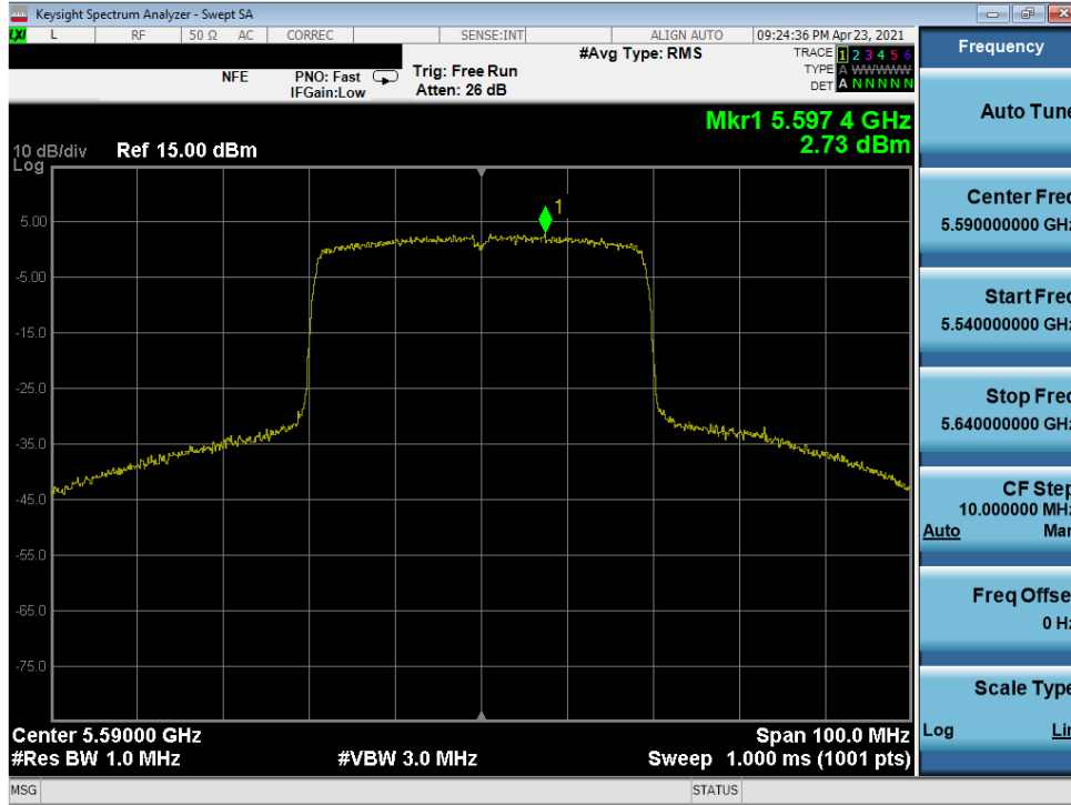
Plot 7-293. Power Spectral Density Plot MIMO ANT2 (40MHz 802.11ax (UNII Band 2C) – Ch. 118)
