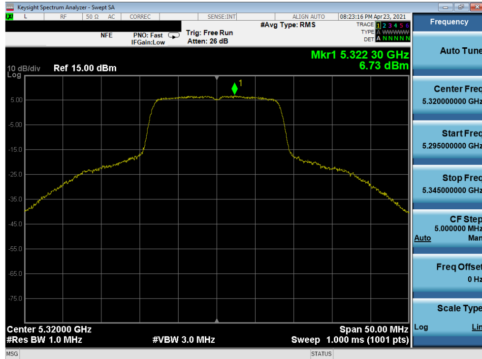
Plot 7-267. Power Spectral Density Plot MIMO ANT2 (20MHz 802.11a (UNII Band 2A) – Ch. 64)
