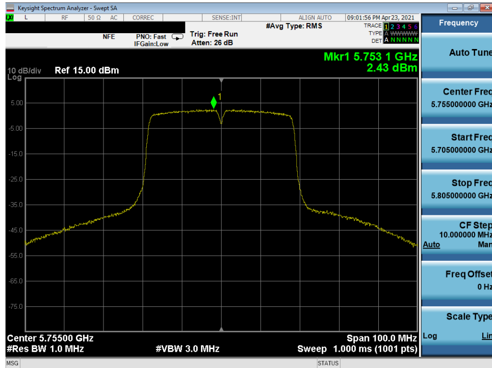
Plot 7-325. Power Spectral Density Plot MIMO ANT2 (40MHz 802.11n (UNII Band 3) – Ch. 151)
