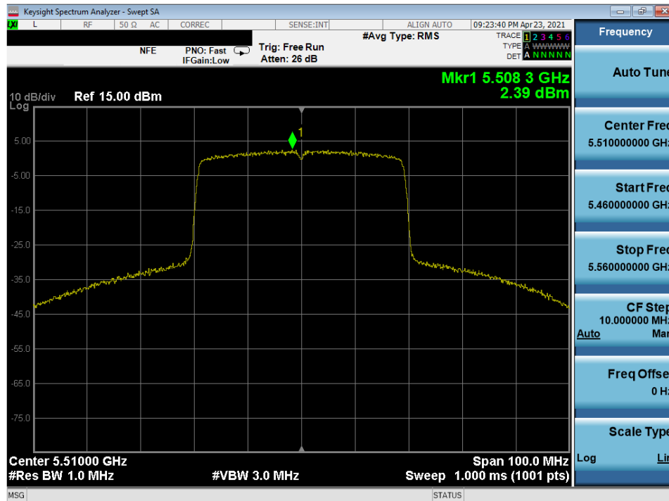
Plot 7-292. Power Spectral Density Plot MIMO ANT2 (40MHz 802.11ax (UNII Band 2C) – Ch. 102)
