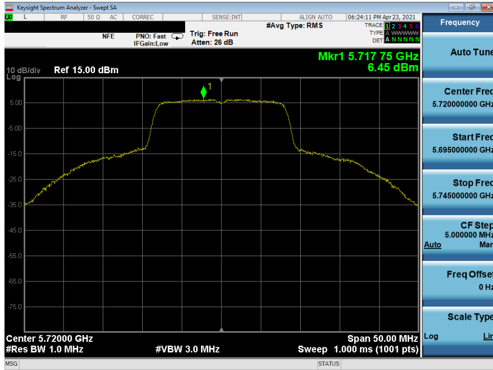
Plot 7-231. Power Spectral Density Plot MIMO ANT1 (20MHz 802.11a (UNII Band 2C) – Ch.144)
