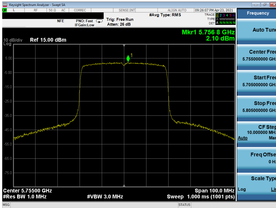
Plot 7-327. Power Spectral Density Plot MIMO ANT2 (40MHz 802.11ax (UNII Band 3) – Ch. 151)
