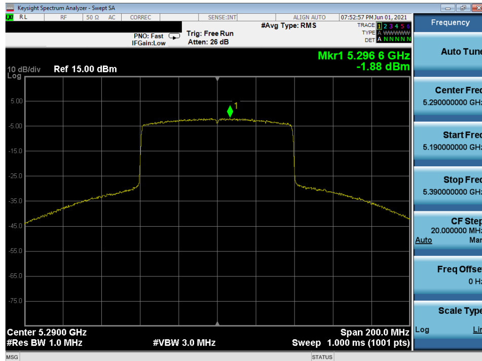
Plot 7-228. Power Spectral Density Plot MIMO ANT1 (80MHz 802.11ax (UNII Band 2A) – Ch. 58)
