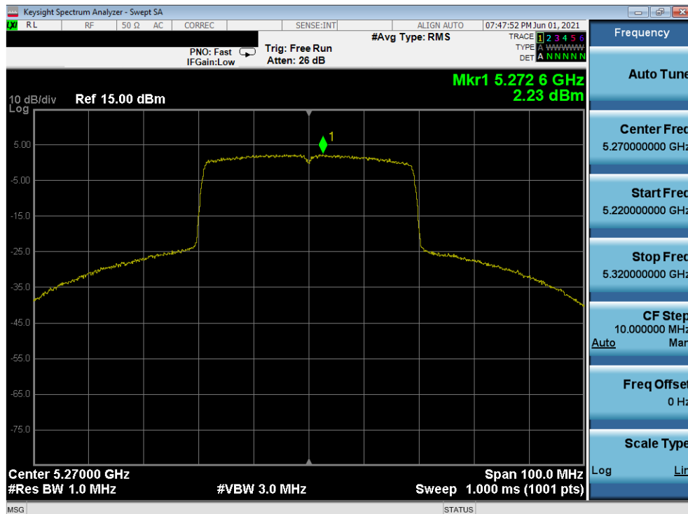
Plot 7-276. Power Spectral Density Plot MIMO ANT2 (40MHz 802.11ax (UNII Band 2A) – Ch. 54)
