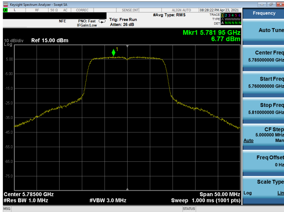
Plot 7-317. Power Spectral Density Plot MIMO ANT2 (20MHz 802.11a (UNII Band 3) – Ch. 157)
