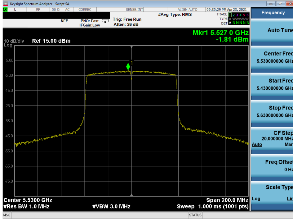
Plot 7-295. Power Spectral Density Plot MIMO ANT2 (80MHz 802.11ac (UNII Band 2C) – Ch. 106)
