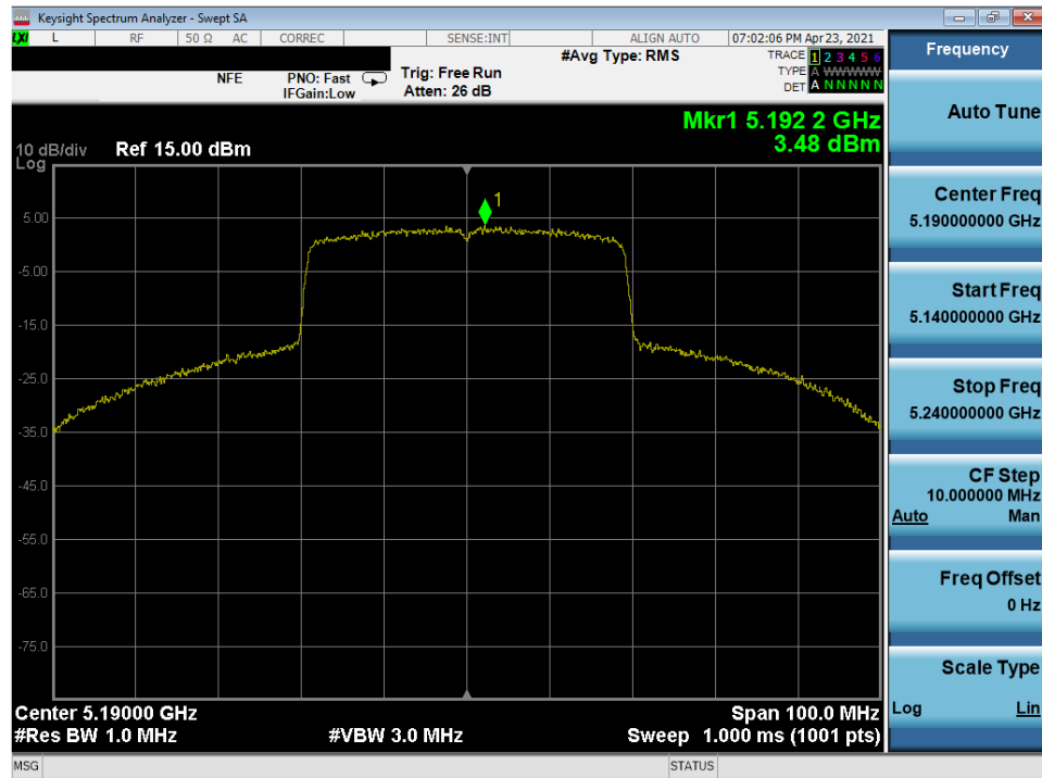
Plot 7-210. Power Spectral Density Plot MIMO ANT1 (40MHz 802.11ax (UNII Band 1) – Ch. 38)
