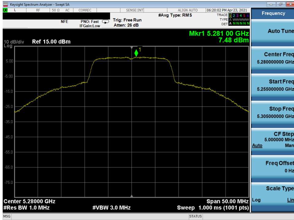
Plot 7-215. Power Spectral Density Plot MIMO ANT1 (20MHz 802.11a (UNII Band 2A) – Ch. 56)
