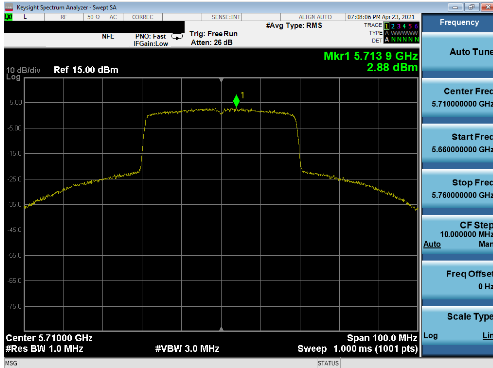
Plot 7-243. Power Spectral Density Plot MIMO ANT1 (40MHz 802.11ax (UNII Band 2C) – Ch.142)
