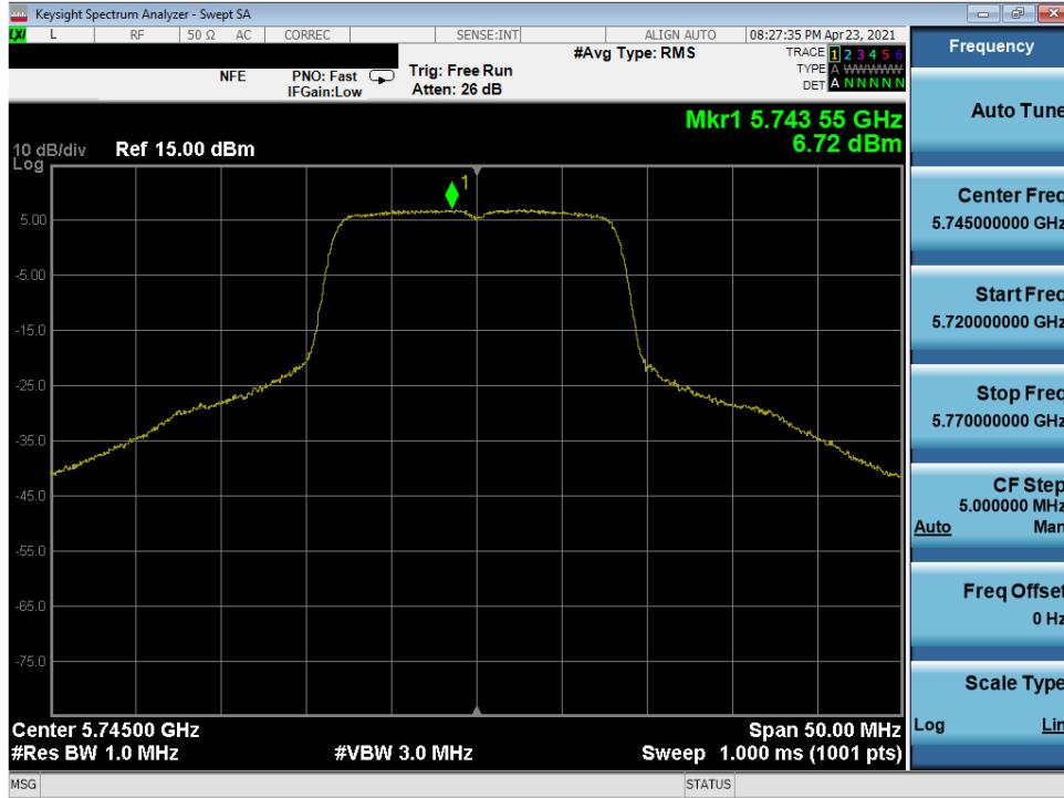
Plot 7-316. Power Spectral Density Plot MIMO ANT2 (20MHz 802.11a (UNII Band 3) – Ch. 149)
