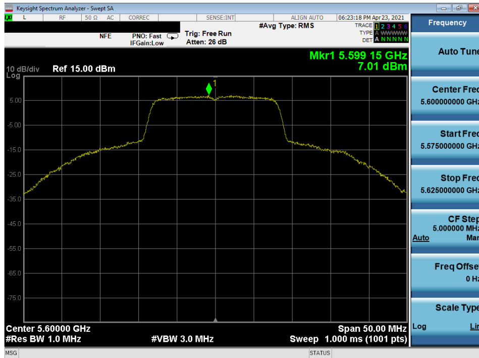
Plot 7-230. Power Spectral Density Plot MIMO ANT1 (20MHz 802.11a (UNII Band 2C) – Ch. 120)
