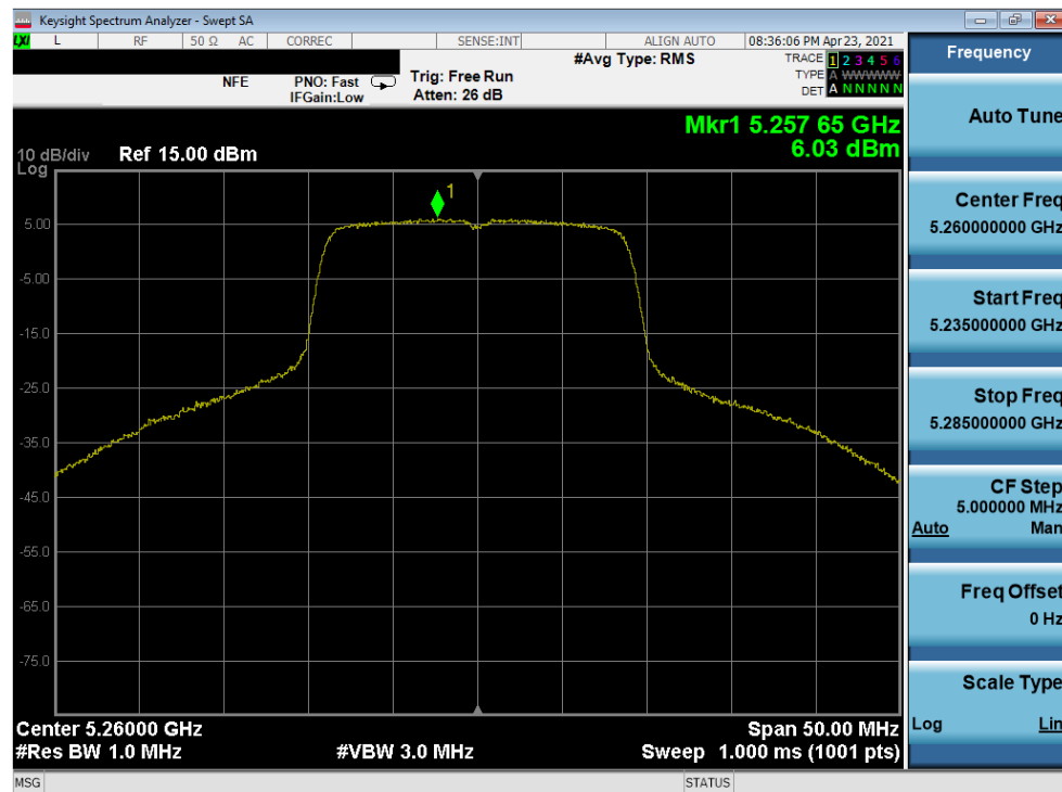
Plot 7-268. Power Spectral Density Plot MIMO ANT2 (20MHz 802.11n (UNII Band 2A) – Ch. 52)
