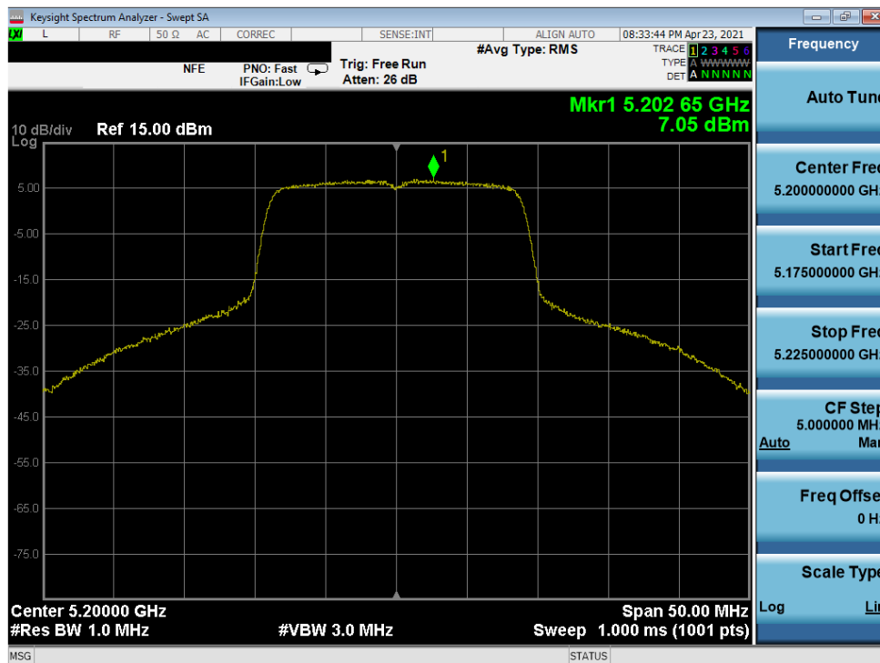
Plot 7-254. Power Spectral Density Plot MIMO ANT2 (20MHz 802.11n (UNII Band 1) – Ch. 40)
