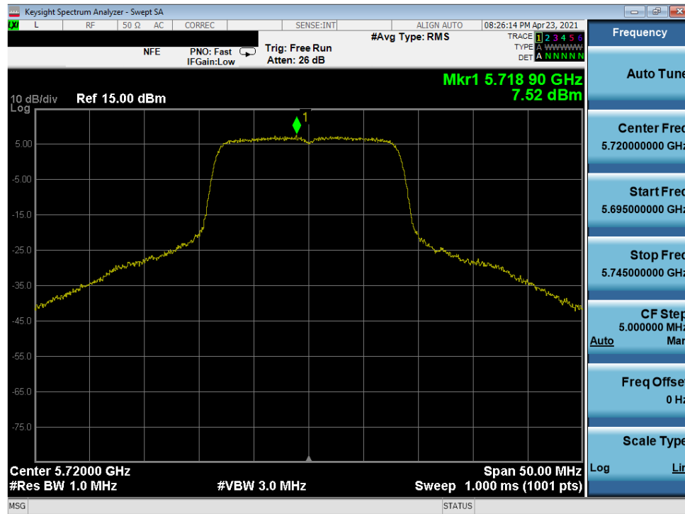
Plot 7-282. Power Spectral Density Plot MIMO ANT2 (20MHz 802.11a (UNII Band 2C) – Ch.144)
