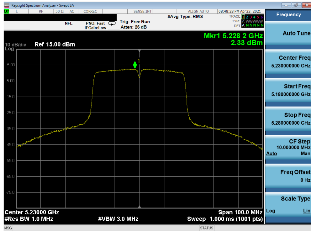
Plot 7-260. Power Spectral Density Plot MIMO ANT2 (40MHz 802.11n (UNII Band 1) – Ch. 46)
