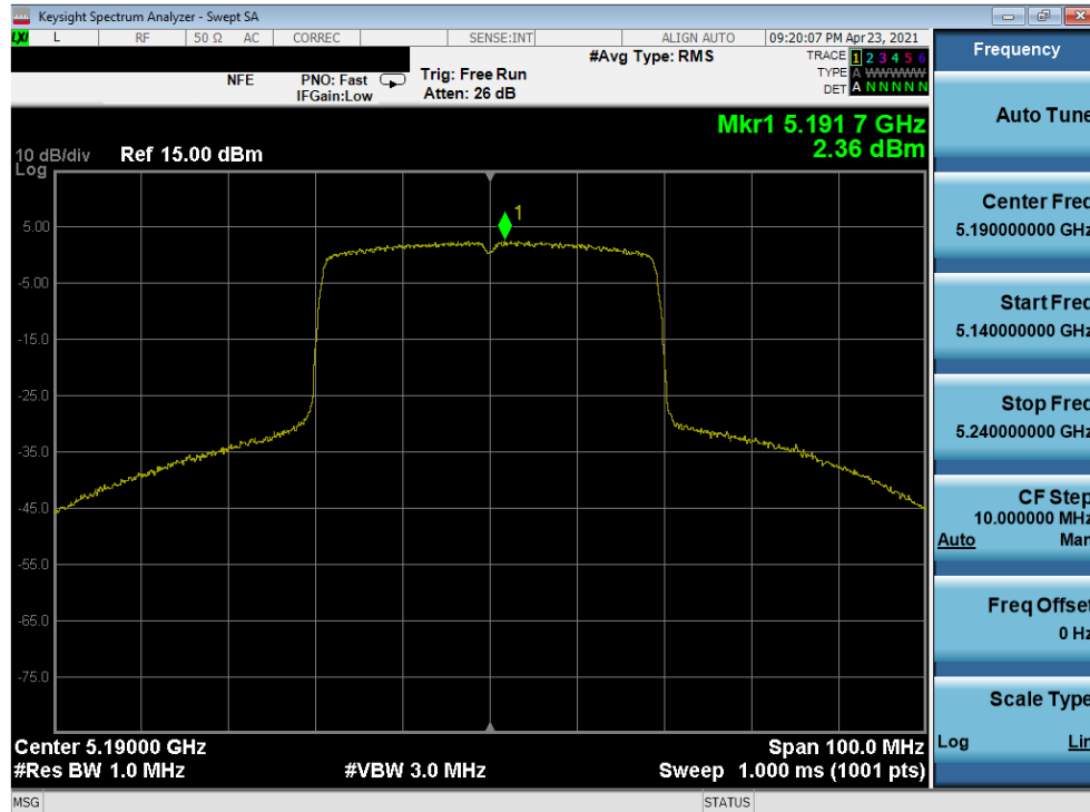
Plot 7-261. Power Spectral Density Plot MIMO ANT2 (40MHz 802.11ax (UNII Band 1) – Ch. 38)
