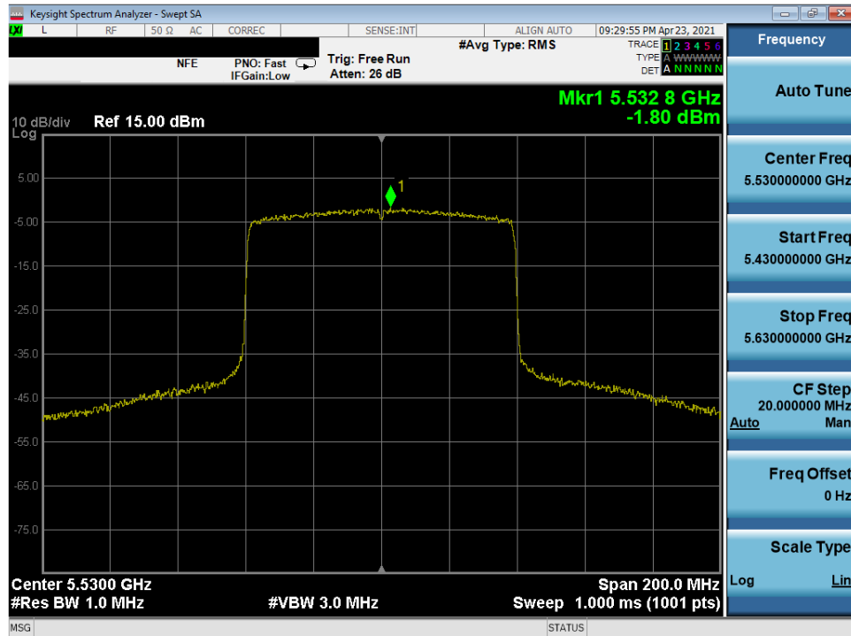
Plot 7-298. Power Spectral Density Plot MIMO ANT2 (80MHz 802.11ax (UNII Band 2C) – Ch. 106)
