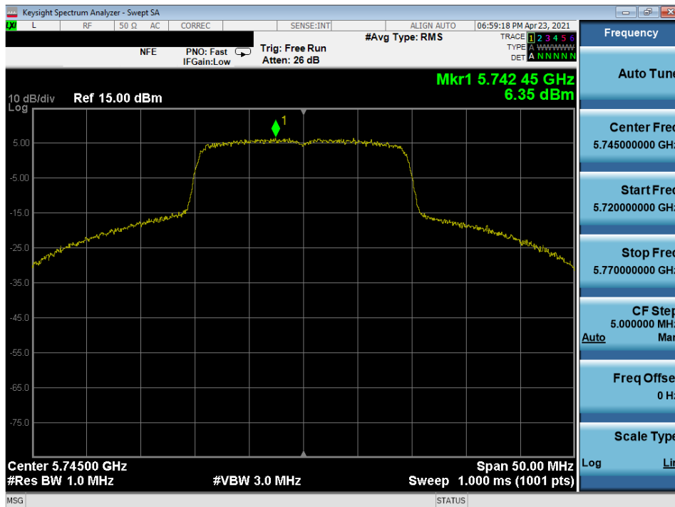
Plot 7-307. Power Spectral Density Plot MIMO ANT1 (20MHz 802.11ax (UNII Band 3) – Ch. 149)
