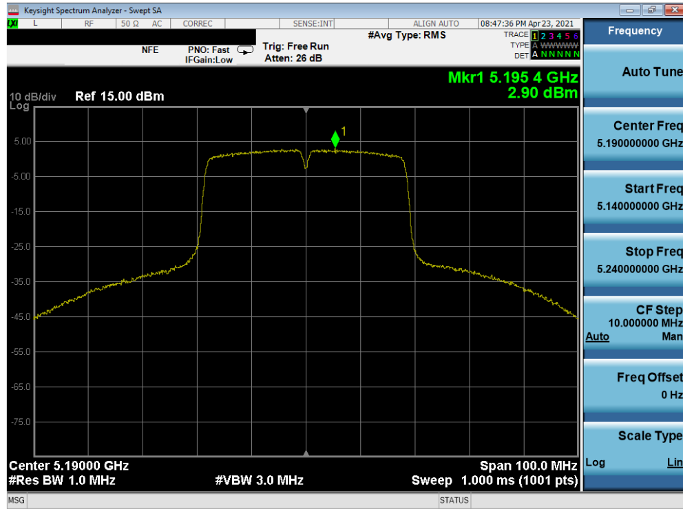
Plot 7-259. Power Spectral Density Plot MIMO ANT2 (40MHz 802.11n (UNII Band 1) – Ch. 38)
