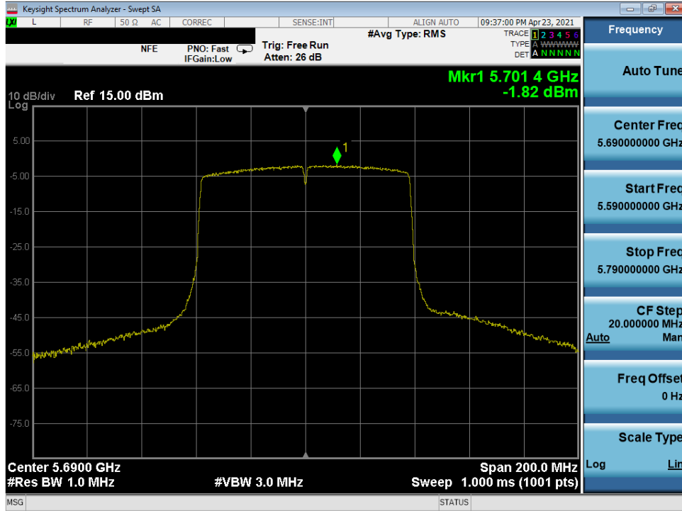
Plot 7-297. Power Spectral Density Plot MIMO ANT2 (80MHz 802.11ac (UNII Band 2C) – Ch.138)
