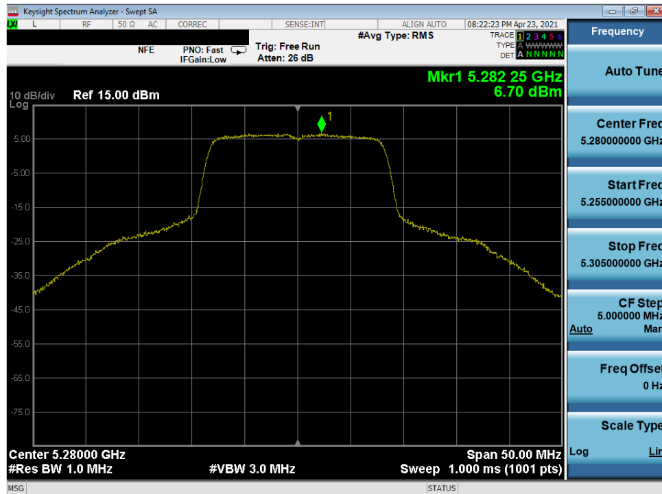
Plot 7-266. Power Spectral Density Plot MIMO ANT2 (20MHz 802.11a (UNII Band 2A) – Ch. 56)
