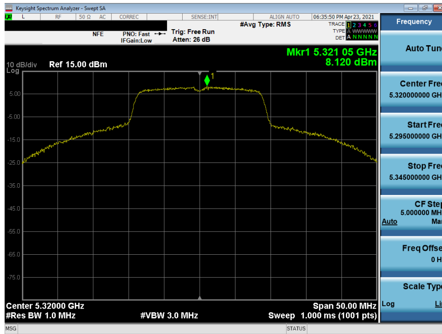
Plot 7-219. Power Spectral Density Plot MIMO ANT1 (20MHz 802.11n (UNII Band 2A) – Ch. 64)
