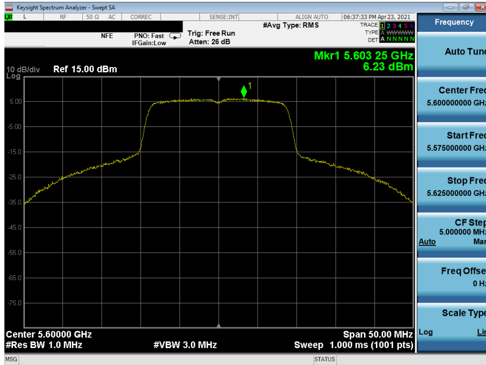
Plot 7-233. Power Spectral Density Plot MIMO ANT1 (20MHz 802.11n (UNII Band 2C) – Ch. 120)
