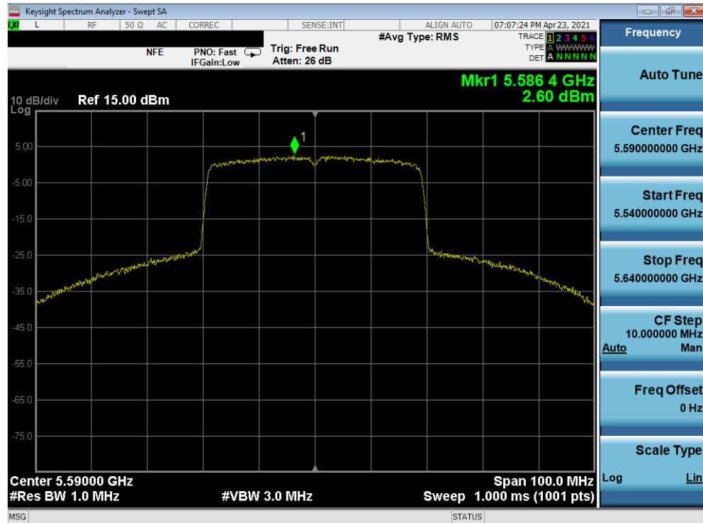
Plot 7-242. Power Spectral Density Plot MIMO ANT1 (40MHz 802.11ax (UNII Band 2C) – Ch. 118)
