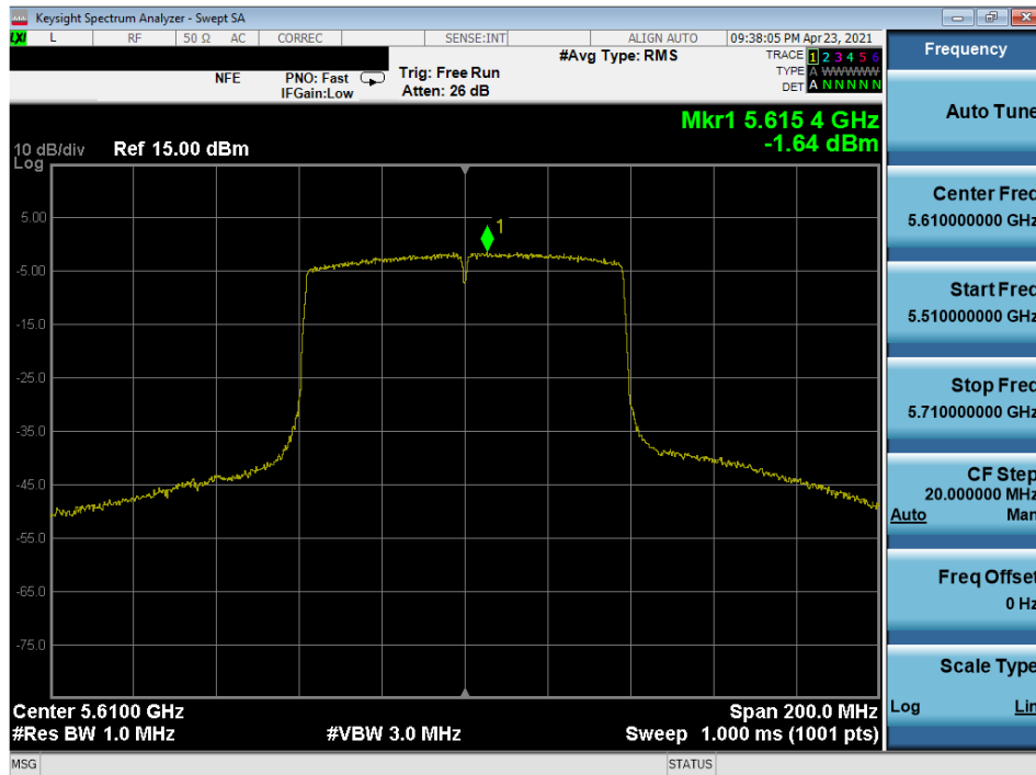
Plot 7-296. Power Spectral Density Plot MIMO ANT2 (80MHz 802.11ac (UNII Band 2C) – Ch. 122)
