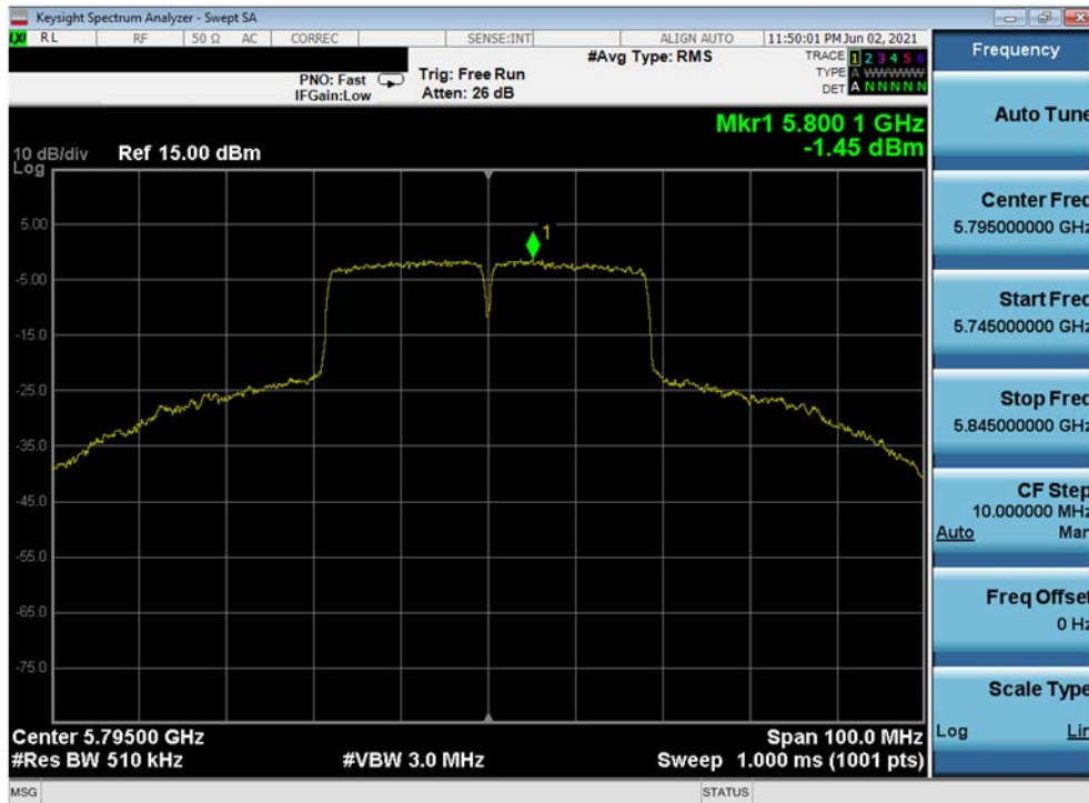
Plot 7-311. Power Spectral Density Plot MIMO ANT1 (40MHz 802.11n (UNII Band 3) – Ch. 159)
