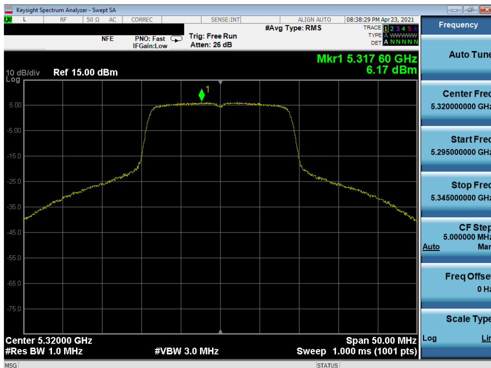
Plot 7-270. Power Spectral Density Plot MIMO ANT2 (20MHz 802.11n (UNII Band 2A) – Ch. 64)
