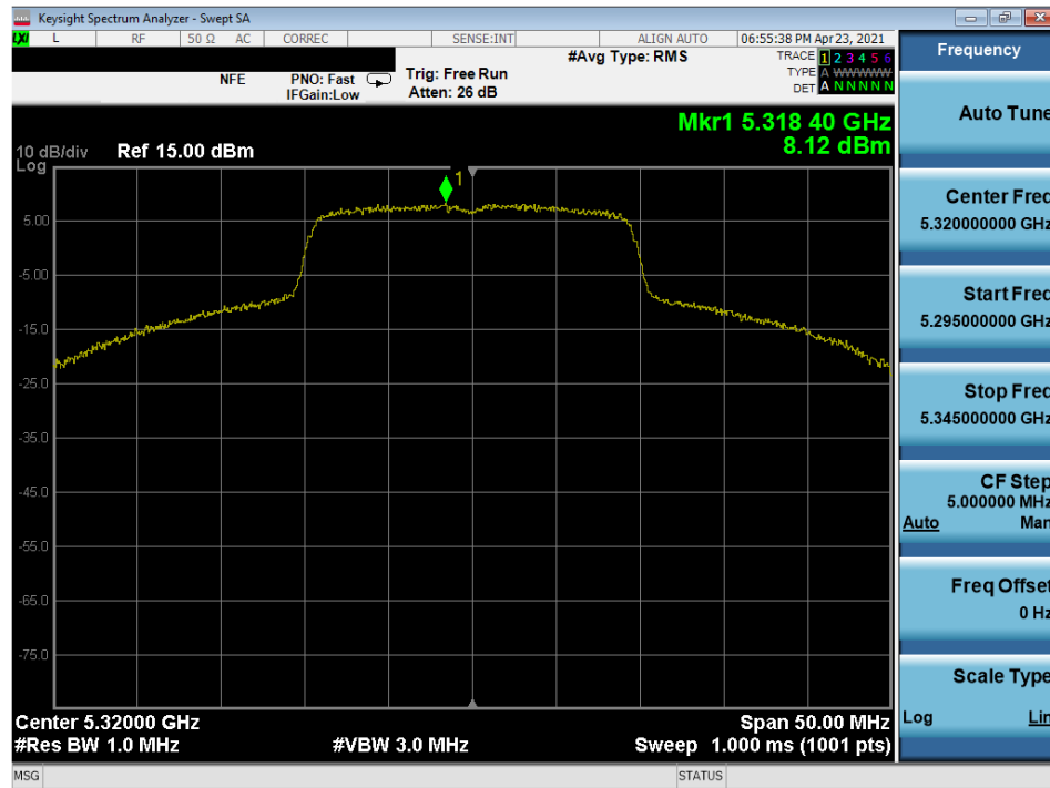
Plot 7-222. Power Spectral Density Plot MIMO ANT1 (20MHz 802.11ax (UNII Band 2A) – Ch. 64)
