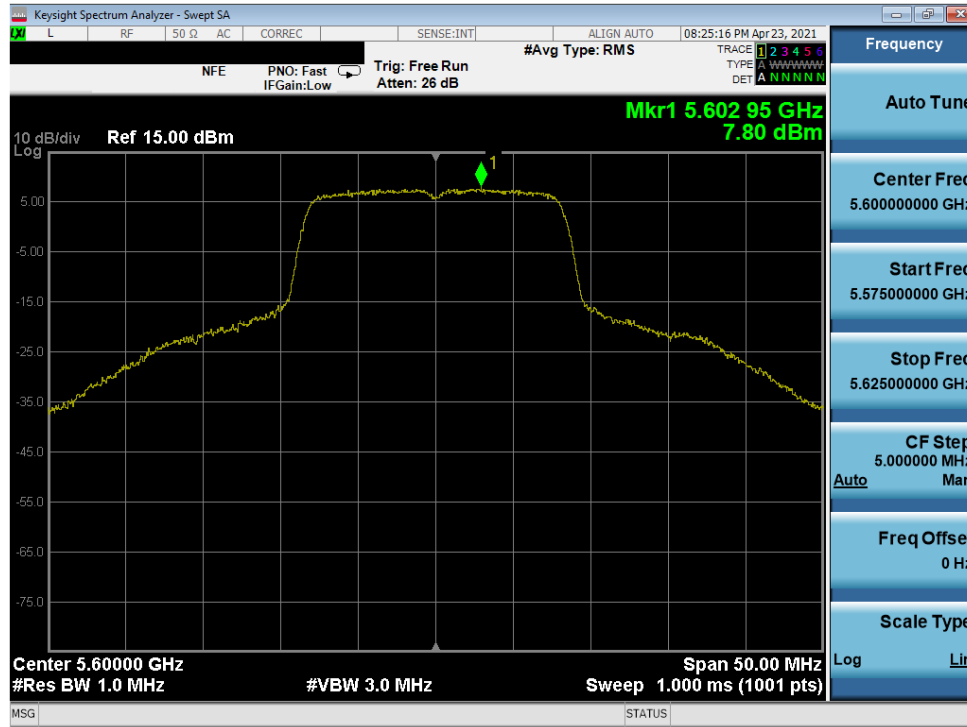
Plot 7-281. Power Spectral Density Plot MIMO ANT2 (20MHz 802.11a (UNII Band 2C) – Ch. 120)
