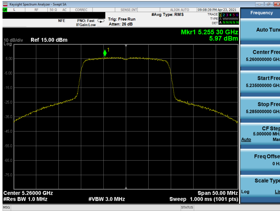
Plot 7-271. Power Spectral Density Plot MIMO ANT2 (20MHz 802.11ax (UNII Band 2A) – Ch. 52)
