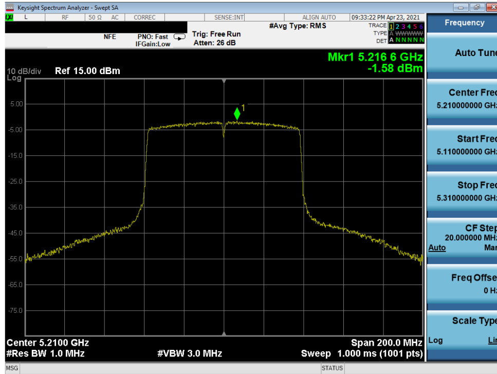
Plot 7-263. Power Spectral Density Plot MIMO ANT2 (80MHz 802.11ac (UNII Band 1) – Ch. 42)
