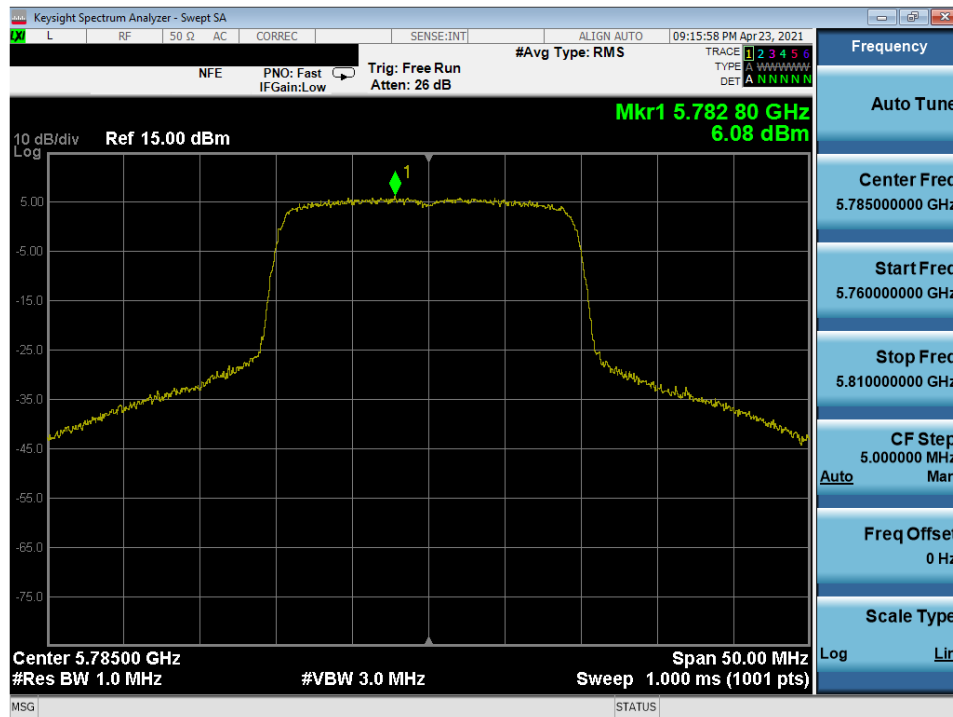
Plot 7-323. Power Spectral Density Plot MIMO ANT2 (20MHz 802.11ax (UNII Band 3) – Ch. 157)
