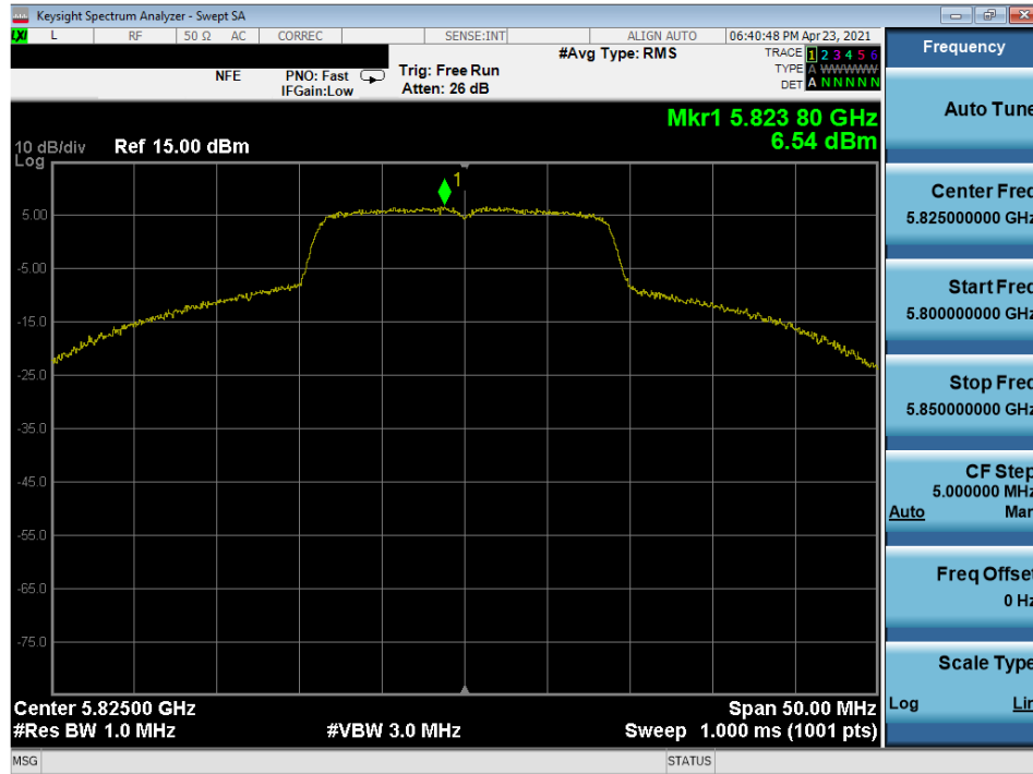
Plot 7-306. Power Spectral Density Plot MIMO ANT1 (20MHz 802.11n (UNII Band 3) – Ch. 165)
