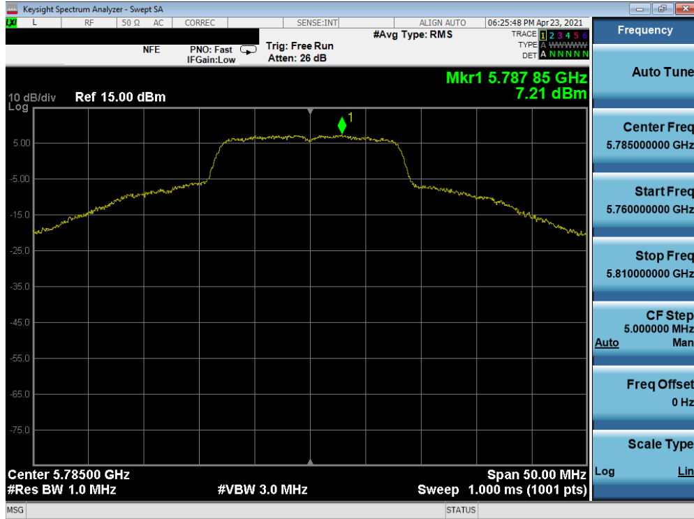
Plot 7-302. Power Spectral Density Plot MIMO ANT1 (20MHz 802.11a (UNII Band 3) – Ch. 157)
