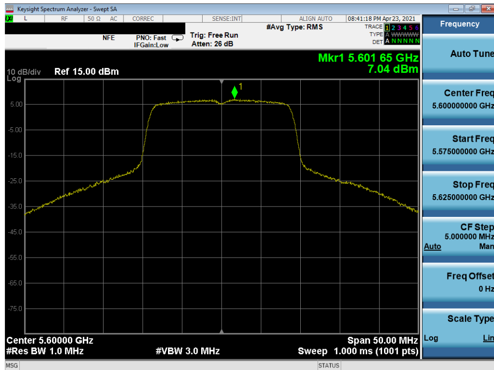
Plot 7-284. Power Spectral Density Plot MIMO ANT2 (20MHz 802.11n (UNII Band 2C) – Ch. 120)
