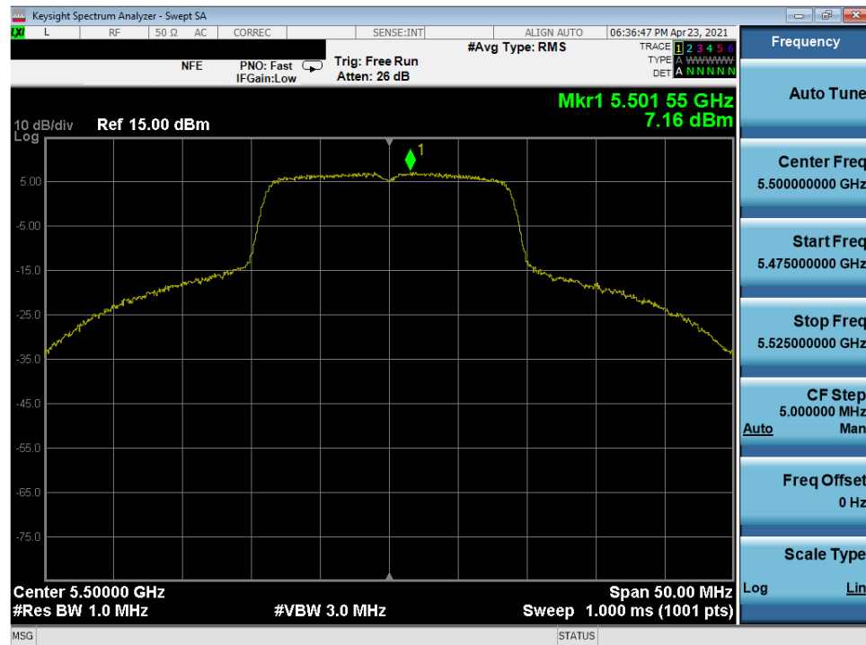
Plot 7-232. Power Spectral Density Plot MIMO ANT1 (20MHz 802.11n (UNII Band 2C) – Ch. 100)
