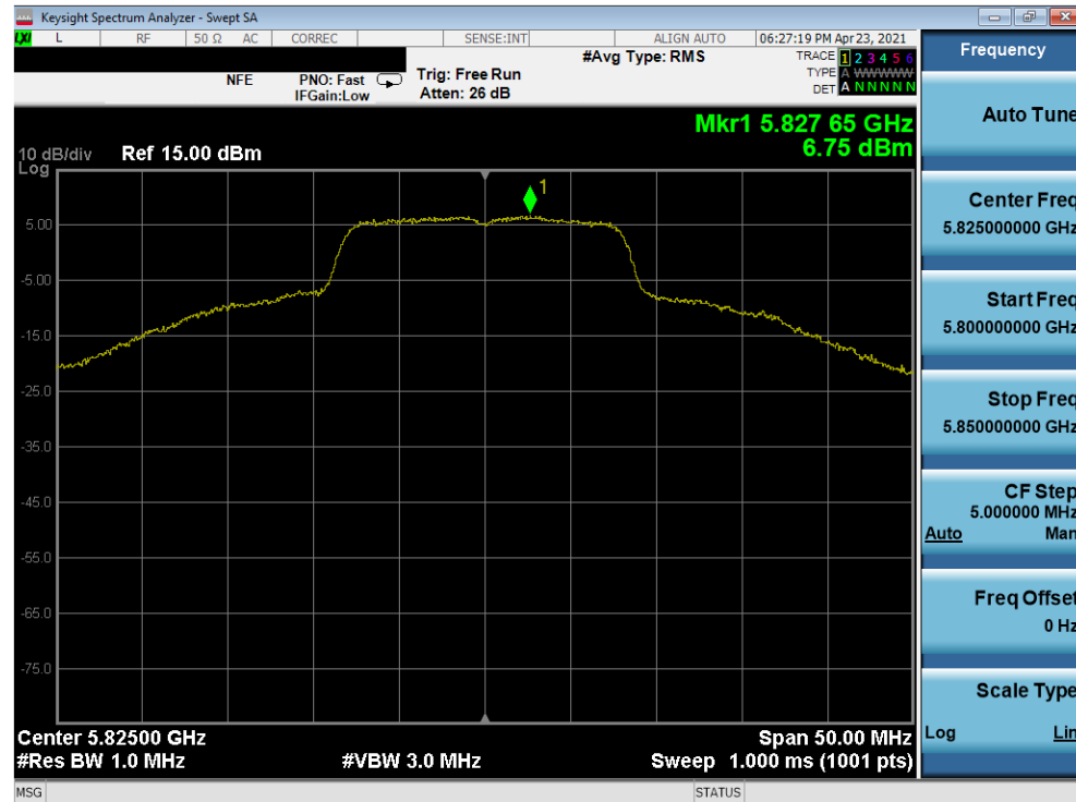
Plot 7-303. Power Spectral Density Plot MIMO ANT1 (20MHz 802.11a (UNII Band 3) – Ch. 165)
