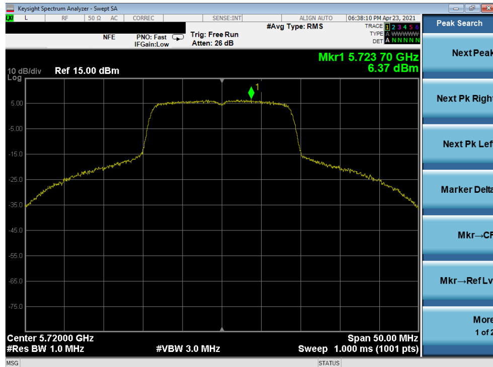
Plot 7-234. Power Spectral Density Plot MIMO ANT1 (20MHz 802.11n (UNII Band 2C) – Ch.144)
