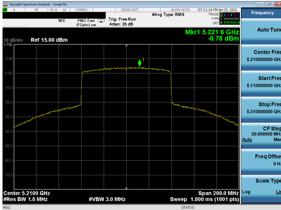
Plot 7-213. Power Spectral Density Plot MIMO ANT1 (80MHz 802.11ax (UNII Band 1) – Ch. 42)
