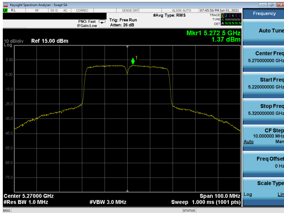
Plot 7-274. Power Spectral Density Plot SISO ANT2 (40MHz 802.11n (UNII Band 2A) – Ch. 54)
