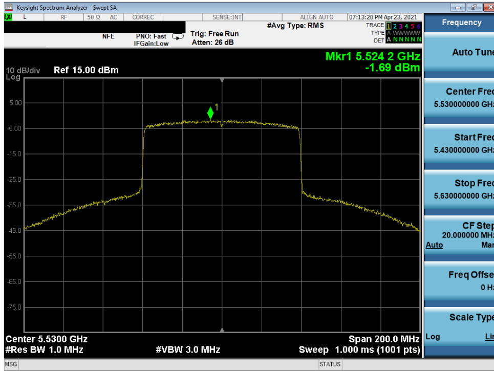
Plot 7-247. Power Spectral Density Plot MIMO ANT1 (80MHz 802.11ax (UNII Band 2C) – Ch. 106)
