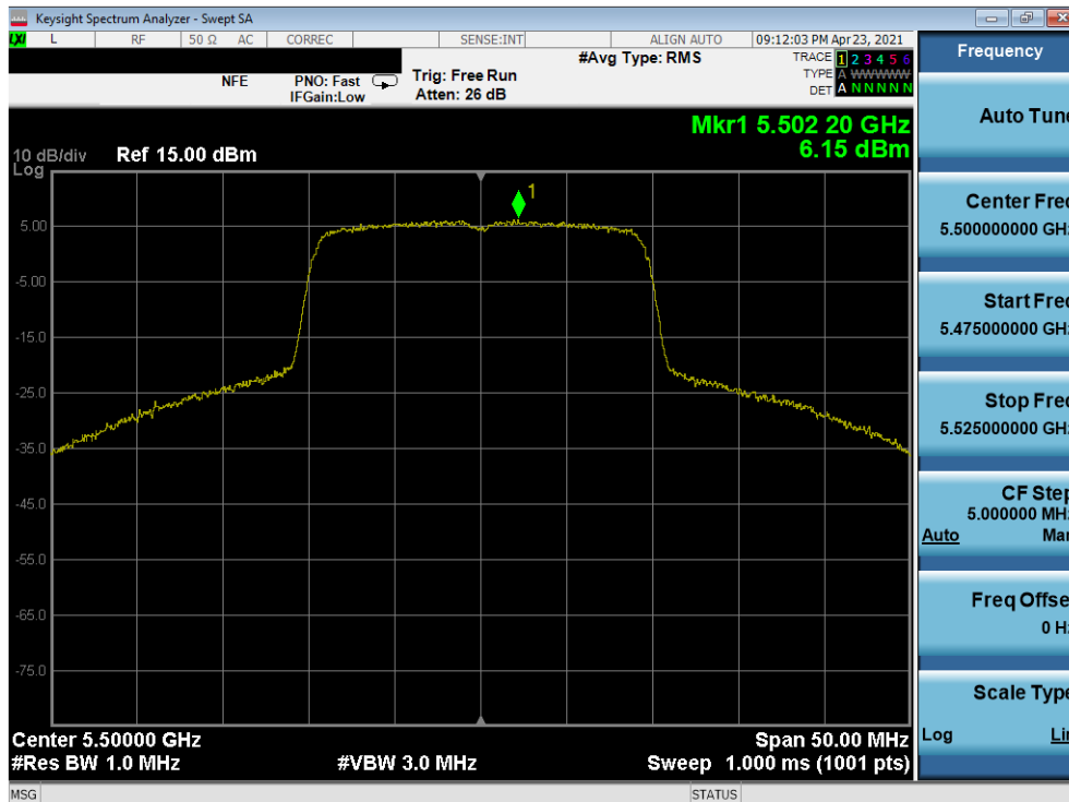
Plot 7-286. Power Spectral Density Plot MIMO ANT2 (20MHz 802.11ax (UNII Band 2C) – Ch. 100)
