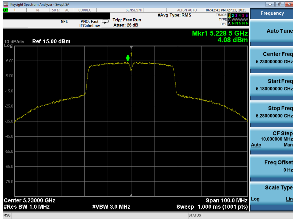
Plot 7-209. Power Spectral Density Plot MIMO ANT1 (40MHz 802.11n (UNII Band 1) – Ch. 46)
