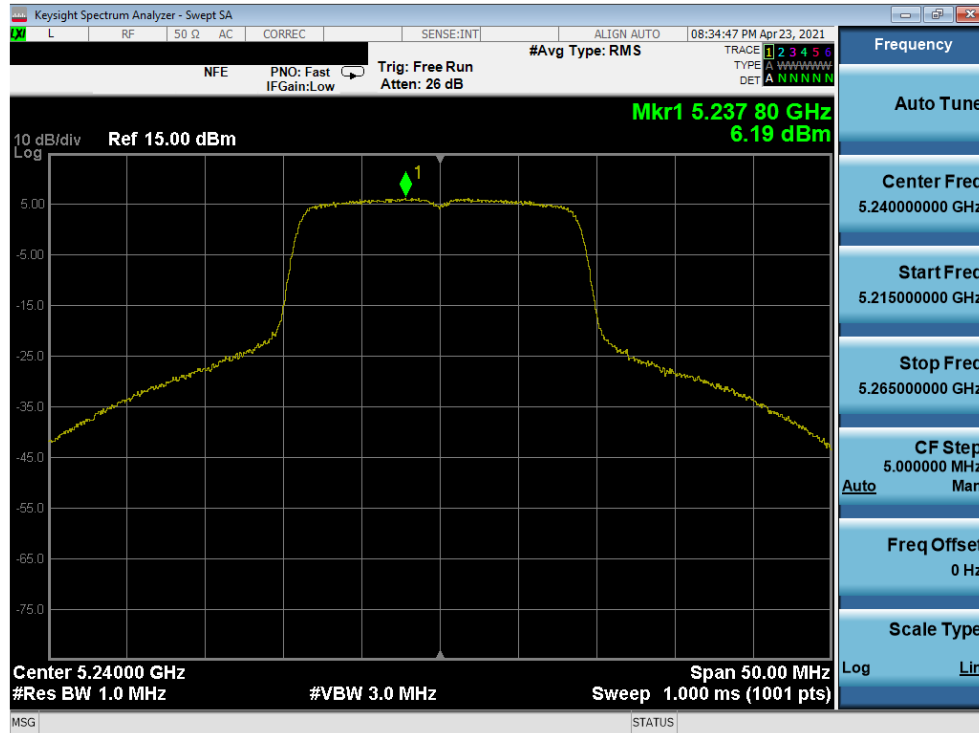
Plot 7-255. Power Spectral Density Plot MIMO ANT2 (20MHz 802.11n (UNII Band 1) – Ch. 48)
