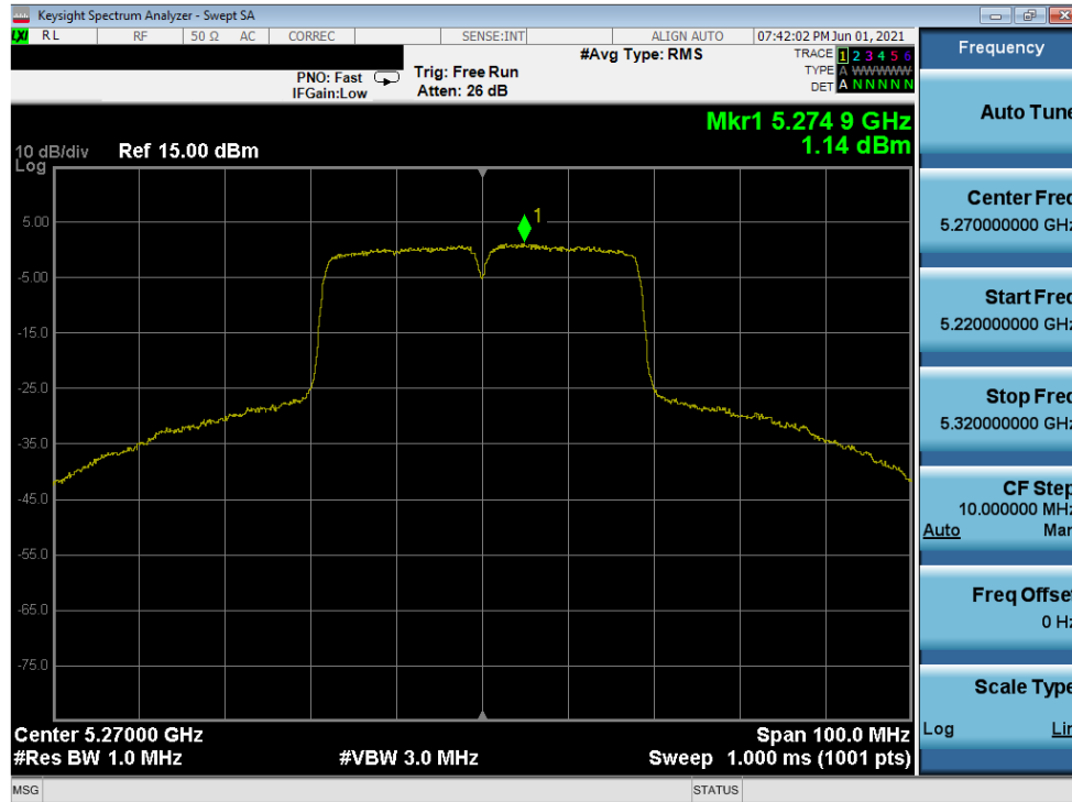
Plot 7-223. Power Spectral Density Plot SISO ANT1 (40MHz 802.11n (UNII Band 2A) – Ch. 54)
