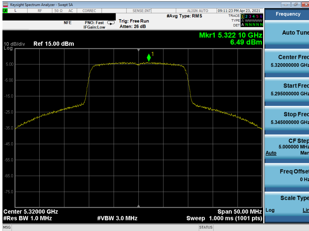
Plot 7-273. Power Spectral Density Plot MIMO ANT2 (20MHz 802.11ax (UNII Band 2A) – Ch. 64)
