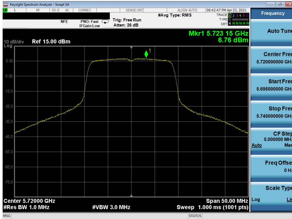
Plot 7-285. Power Spectral Density Plot MIMO ANT2 (20MHz 802.11n (UNII Band 2C) – Ch.144)
