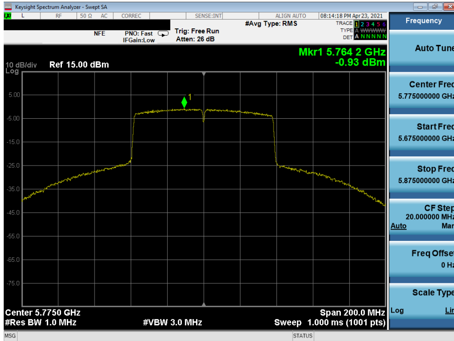
Plot 7-314. Power Spectral Density Plot SISO ANT1 (80MHz 802.11ac (UNII Band 3) – Ch. 155)
