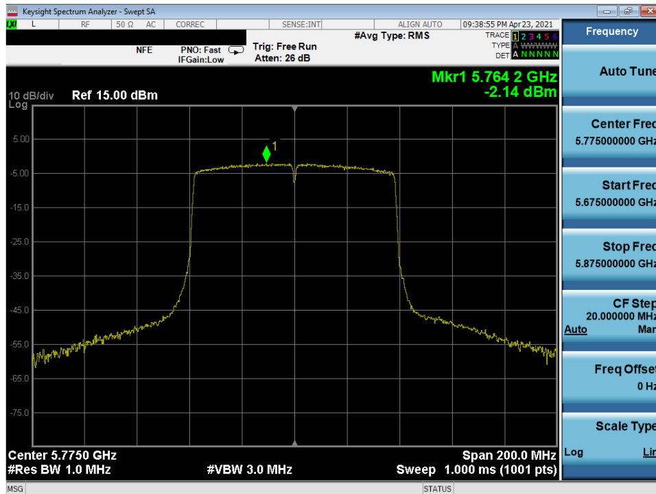
Plot 7-329. Power Spectral Density Plot SISO ANT2 (80MHz 802.11ac (UNII Band 3) – Ch. 155)
