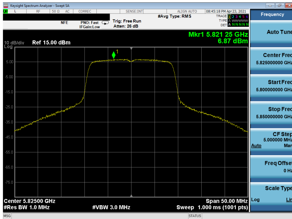
Plot 7-321. Power Spectral Density Plot MIMO ANT2 (20MHz 802.11n (UNII Band 3) – Ch. 165)
