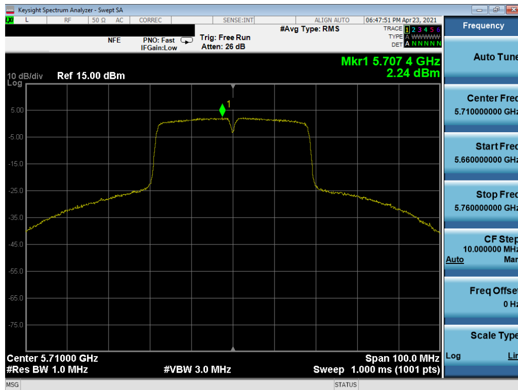
Plot 7-240. Power Spectral Density Plot MIMO ANT1 (40MHz 802.11n (UNII Band 2C) – Ch.142)
