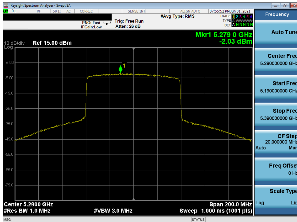
Plot 7-278. Power Spectral Density Plot MIMO ANT2 (80MHz 802.11ac (UNII Band 2A) – Ch. 58)
