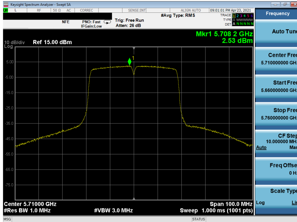
Plot 7-291. Power Spectral Density Plot MIMO ANT2 (40MHz 802.11n (UNII Band 2C) – Ch.142)
