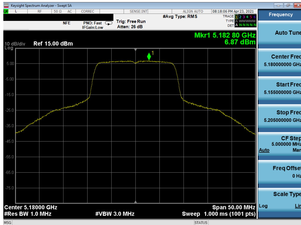
Plot 7-250. Power Spectral Density Plot MIMO ANT2 (20MHz 802.11a (UNII Band 1) – Ch. 36)
