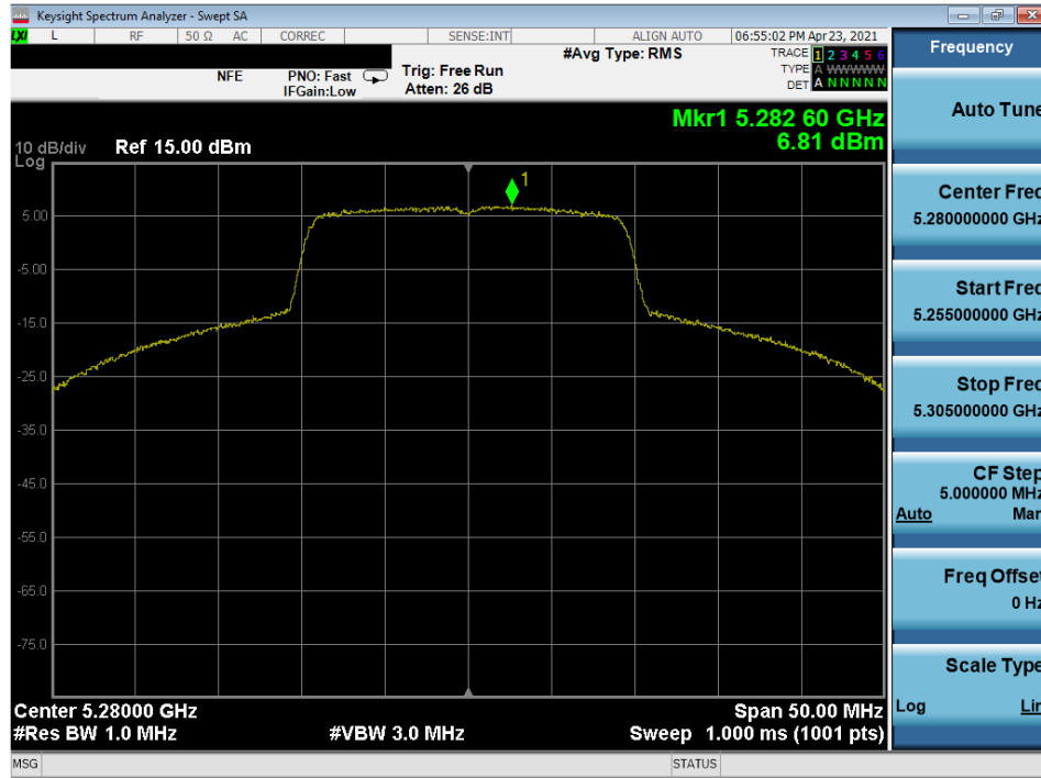
Plot 7-221. Power Spectral Density Plot MIMO ANT1 (20MHz 802.11ax (UNII Band 2A) – Ch. 56)
