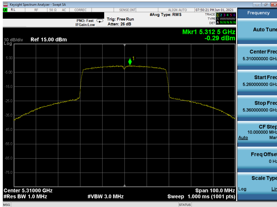
Plot 7-226. Power Spectral Density Plot MIMO ANT1 (40MHz 802.11ax (UNII Band 2A) – Ch. 62)
