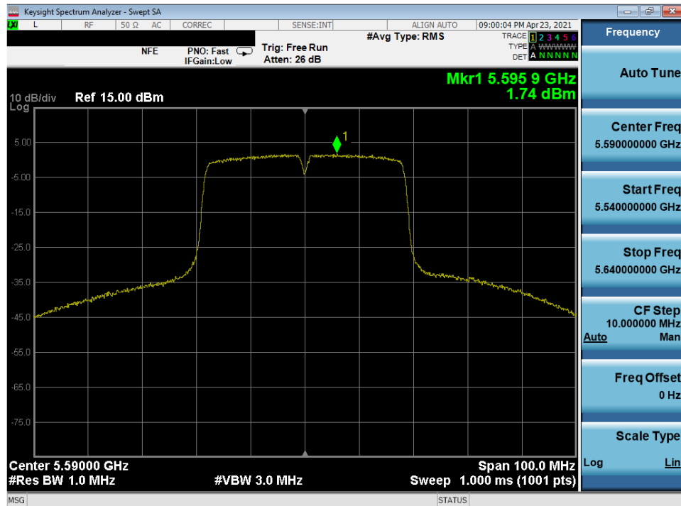
Plot 7-290. Power Spectral Density Plot MIMO ANT2 (40MHz 802.11n (UNII Band 2C) – Ch. 118)
