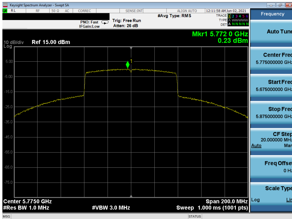
Plot 7-315. Power Spectral Density Plot MIMO ANT1 (80MHz 802.11ax (UNII Band 3) – Ch. 155)
