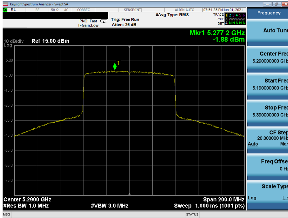
Plot 7-279. Power Spectral Density Plot MIMO ANT2 (80MHz 802.11ax (UNII Band 2A) – Ch. 58)
