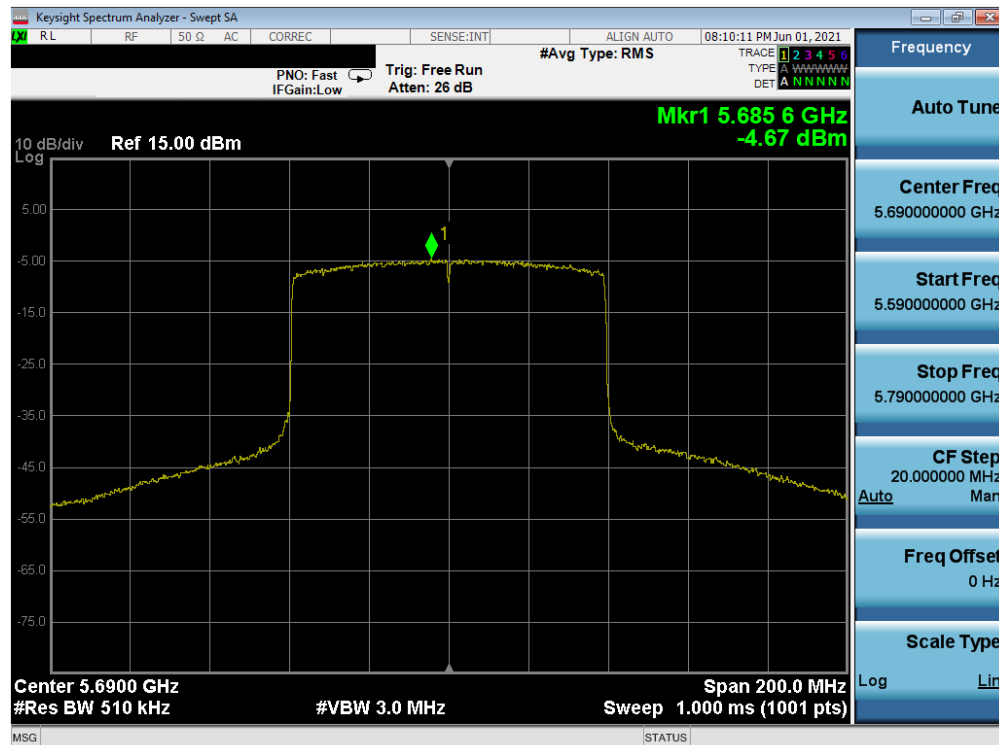
Plot 7-300. Power Spectral Density Plot MIMO ANT2 (80MHz 802.11ax (UNII Band 2C) – Ch.138)
