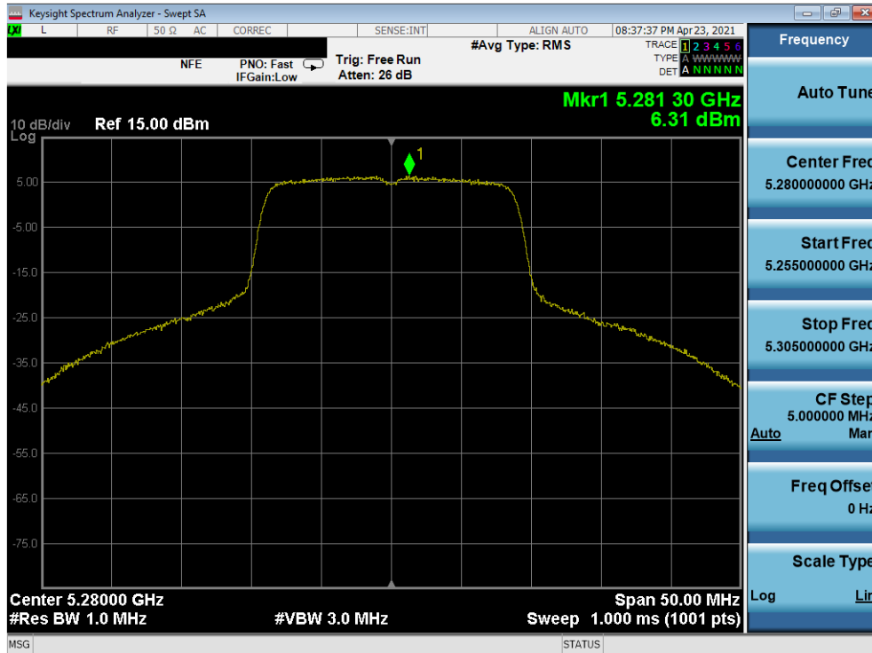
Plot 7-269. Power Spectral Density Plot MIMO ANT2 (20MHz 802.11n (UNII Band 2A) – Ch. 56)
