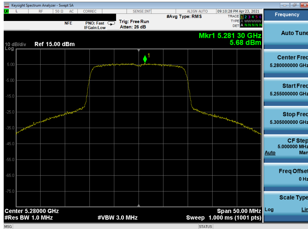
Plot 7-272. Power Spectral Density Plot MIMO ANT2 (20MHz 802.11ax (UNII Band 2A) – Ch. 56)
