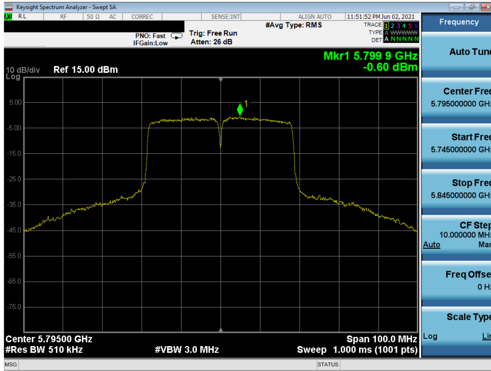
Plot 7-326. Power Spectral Density Plot MIMO ANT2 (40MHz 802.11n (UNII Band 3) – Ch. 159)
