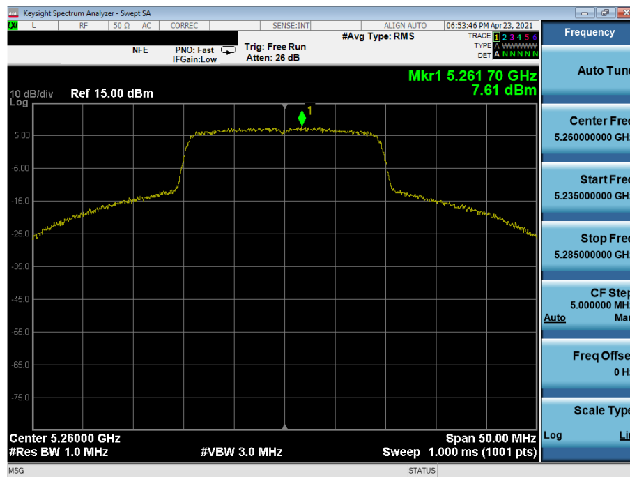
Plot 7-220. Power Spectral Density Plot MIMO ANT1 (20MHz 802.11ax (UNII Band 2A) – Ch. 52)
