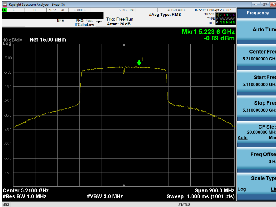
Plot 7-212. Power Spectral Density Plot MIMO ANT1 (80MHz 802.11ac (UNII Band 1) – Ch. 42)
