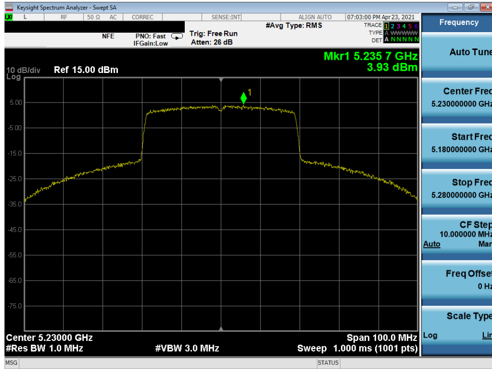
Plot 7-211. Power Spectral Density Plot MIMO ANT1 (40MHz 802.11ax (UNII Band 1) – Ch. 46)
