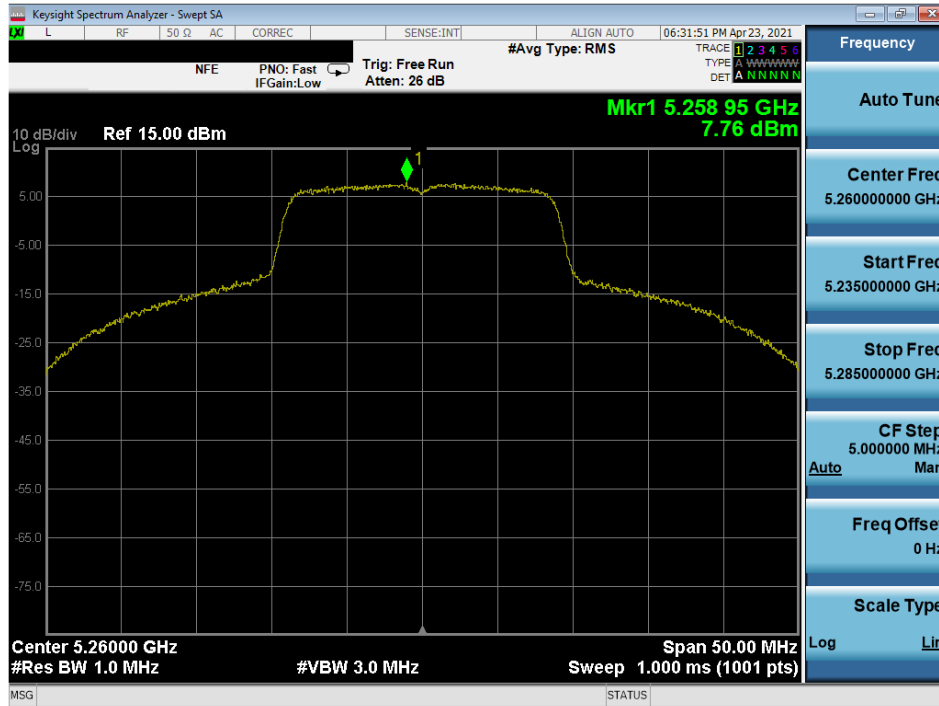
Plot 7-217. Power Spectral Density Plot MIMO ANT1 (20MHz 802.11n (UNII Band 2A) – Ch. 52)
