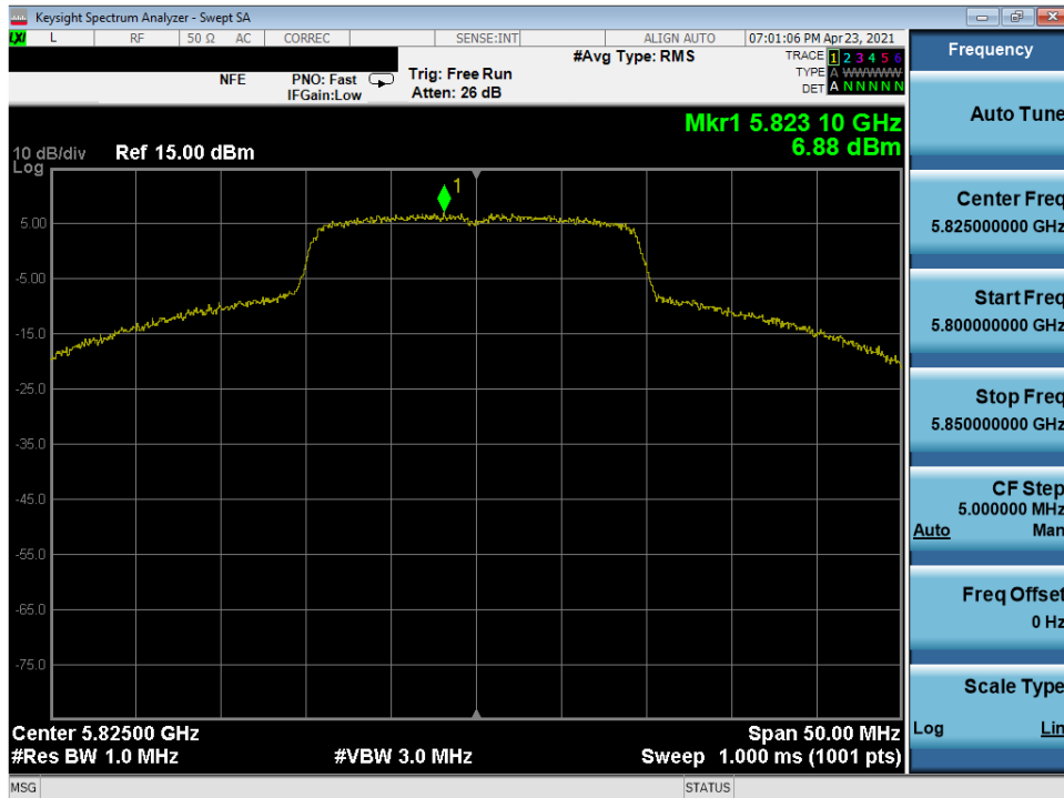
Plot 7-309. Power Spectral Density Plot MIMO ANT1 (20MHz 802.11ax (UNII Band 3) – Ch. 165)
