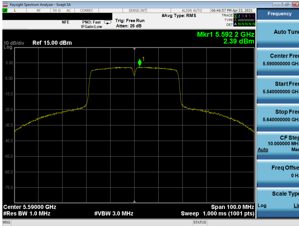
Plot 7-239. Power Spectral Density Plot MIMO ANT1 (40MHz 802.11n (UNII Band 2C) – Ch. 118)
