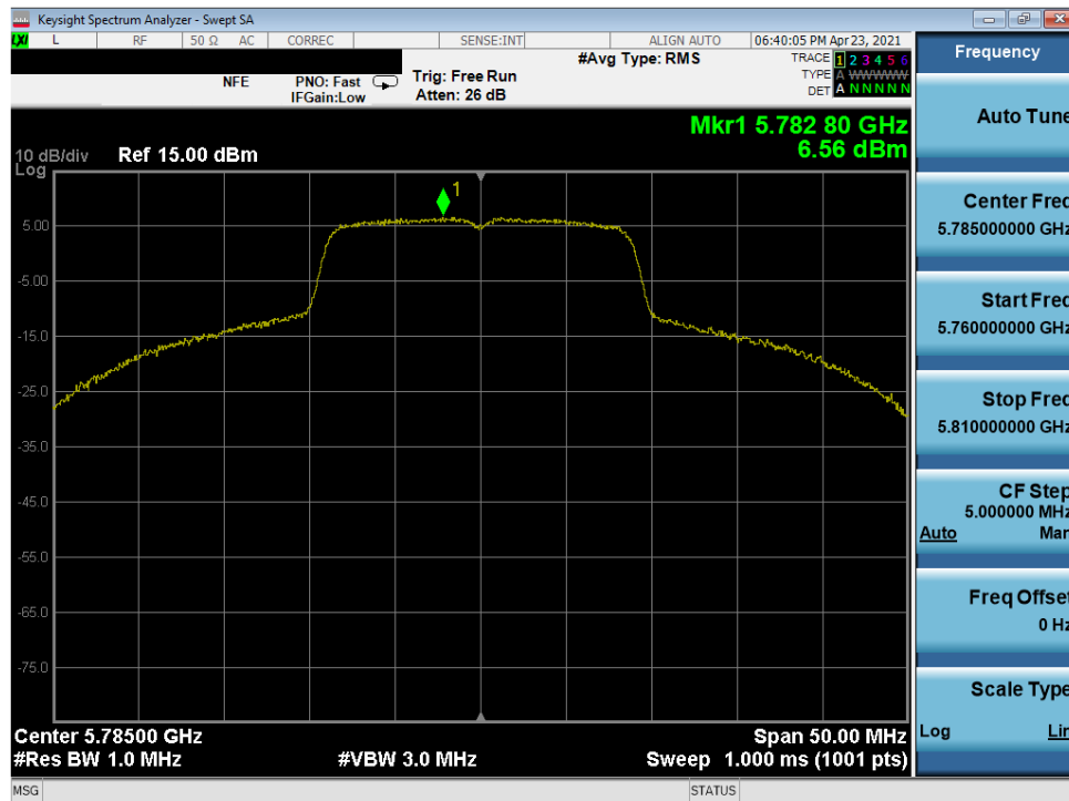
Plot 7-305. Power Spectral Density Plot MIMO ANT1 (20MHz 802.11n (UNII Band 3) – Ch. 157)
