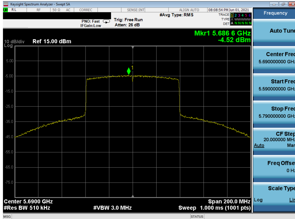
Plot 7-249. Power Spectral Density Plot MIMO ANT1 (80MHz 802.11ax (UNII Band 2C) – Ch.138)
