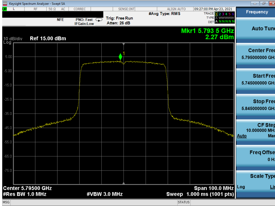
Plot 7-328. Power Spectral Density Plot MIMO ANT2 (40MHz 802.11ax (UNII Band 3) – Ch. 159)
