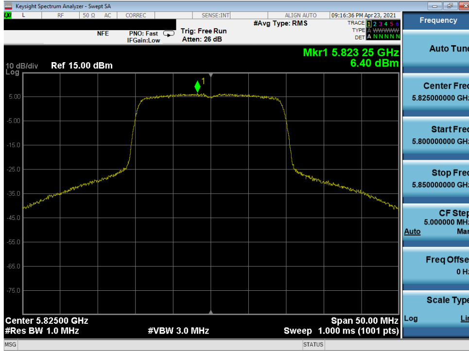
Plot 7-324. Power Spectral Density Plot MIMO ANT2 (20MHz 802.11ax (UNII Band 3) – Ch. 165)
