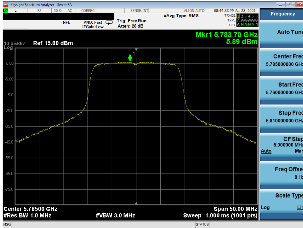
Plot 7-320. Power Spectral Density Plot MIMO ANT2 (20MHz 802.11n (UNII Band 3) – Ch. 157)
