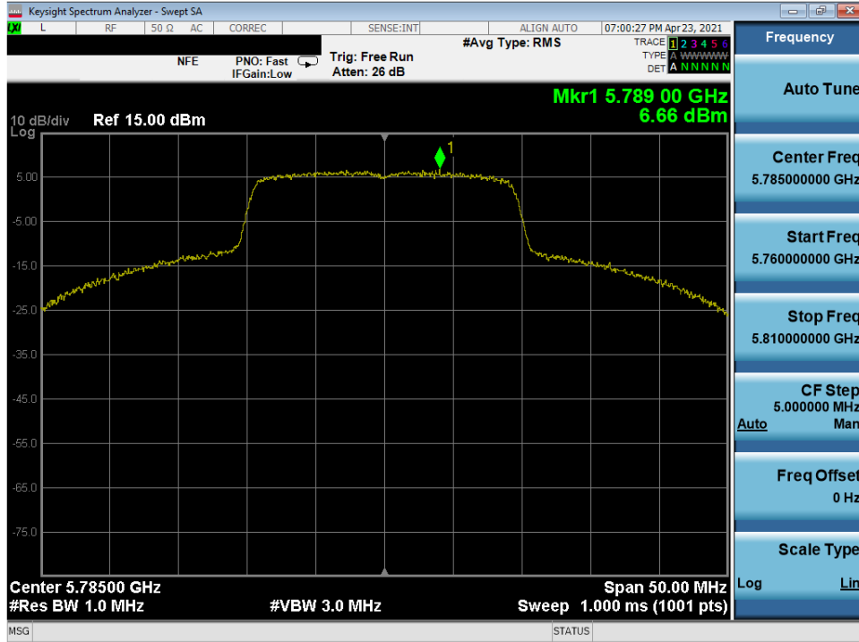
Plot 7-308. Power Spectral Density Plot MIMO ANT1 (20MHz 802.11ax (UNII Band 3) – Ch. 157)
