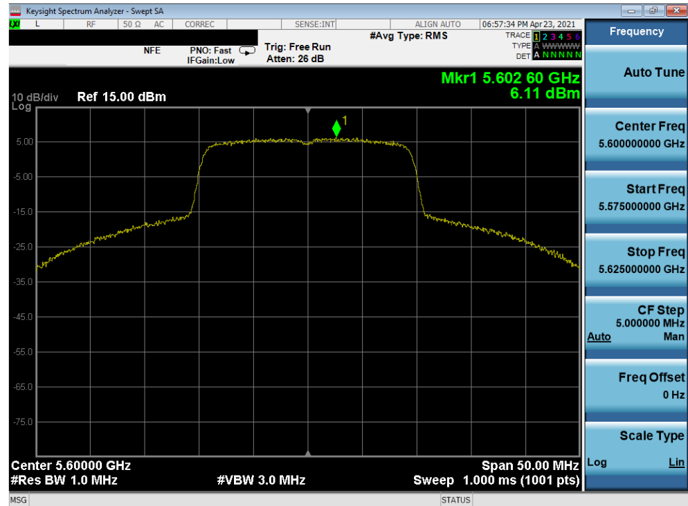
Plot 7-236. Power Spectral Density Plot MIMO ANT1 (20MHz 802.11ax (UNII Band 2C) – Ch. 120)
