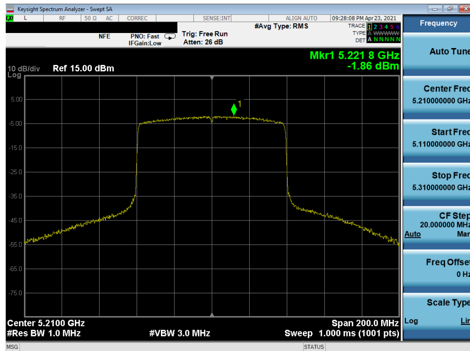
Plot 7-264. Power Spectral Density Plot MIMO ANT2 (80MHz 802.11ax (UNII Band 1) – Ch. 42)
