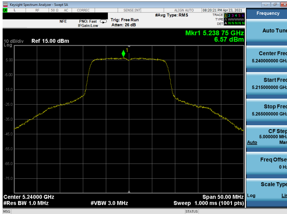
Plot 7-252. Power Spectral Density Plot MIMO ANT2 (20MHz 802.11a (UNII Band 1) – Ch. 48)
