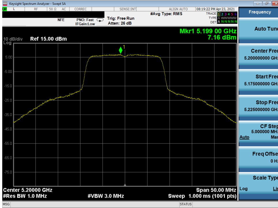
Plot 7-251. Power Spectral Density Plot MIMO ANT2 (20MHz 802.11a (UNII Band 1) – Ch. 40)
