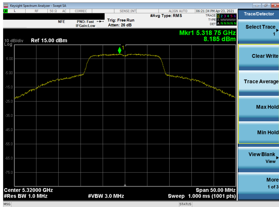
Plot 7-216. Power Spectral Density Plot MIMO ANT1 (20MHz 802.11a (UNII Band 2A) – Ch. 64)
