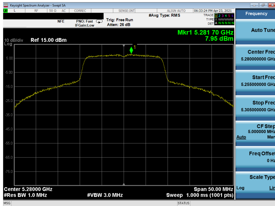
Plot 7-218. Power Spectral Density Plot MIMO ANT1 (20MHz 802.11n (UNII Band 2A) – Ch. 56)
