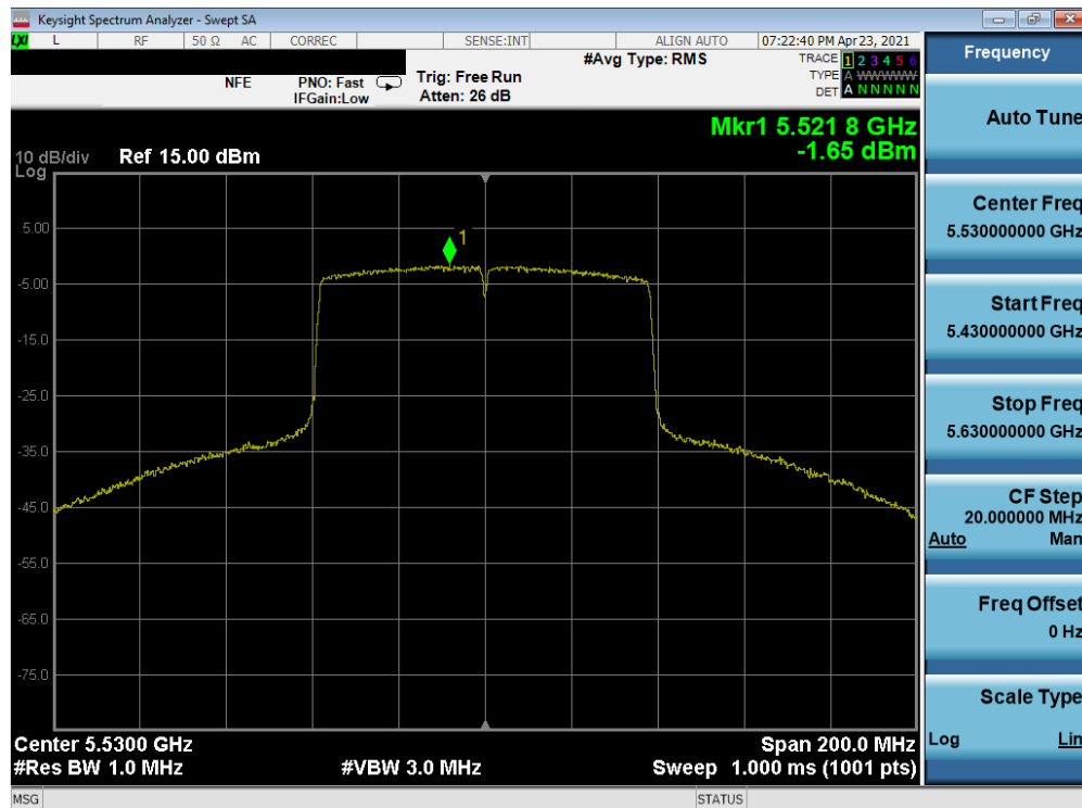
Plot 7-244. Power Spectral Density Plot MIMO ANT1 (80MHz 802.11ac (UNII Band 2C) – Ch. 106)
