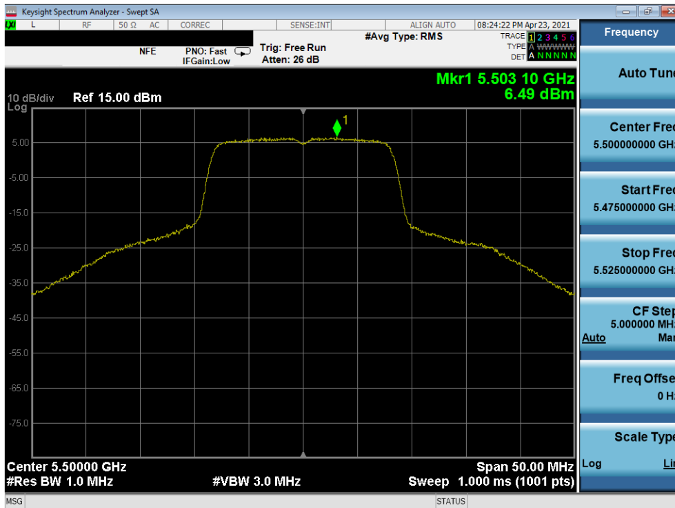
Plot 7-280. Power Spectral Density Plot MIMO ANT2 (20MHz 802.11a (UNII Band 2C) – Ch. 100)
