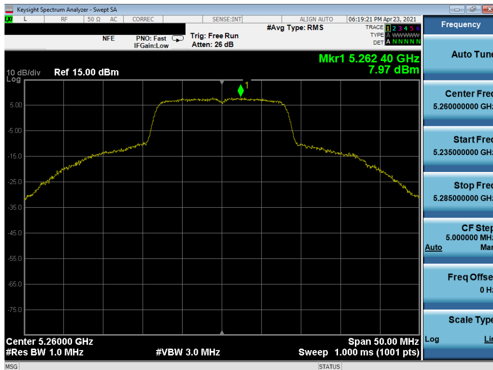
Plot 7-214. Power Spectral Density Plot MIMO ANT1 (20MHz 802.11a (UNII Band 2A) – Ch. 52)
