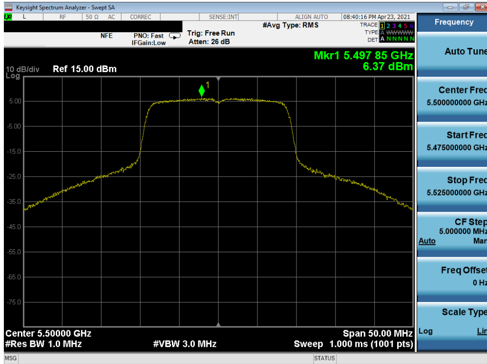
Plot 7-283. Power Spectral Density Plot MIMO ANT2 (20MHz 802.11n (UNII Band 2C) – Ch. 100)
