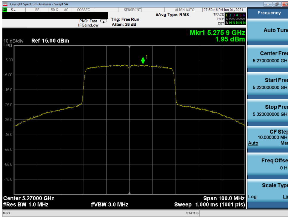
Plot 7-225. Power Spectral Density Plot MIMO ANT1 (40MHz 802.11ax (UNII Band 2A) – Ch. 54)
