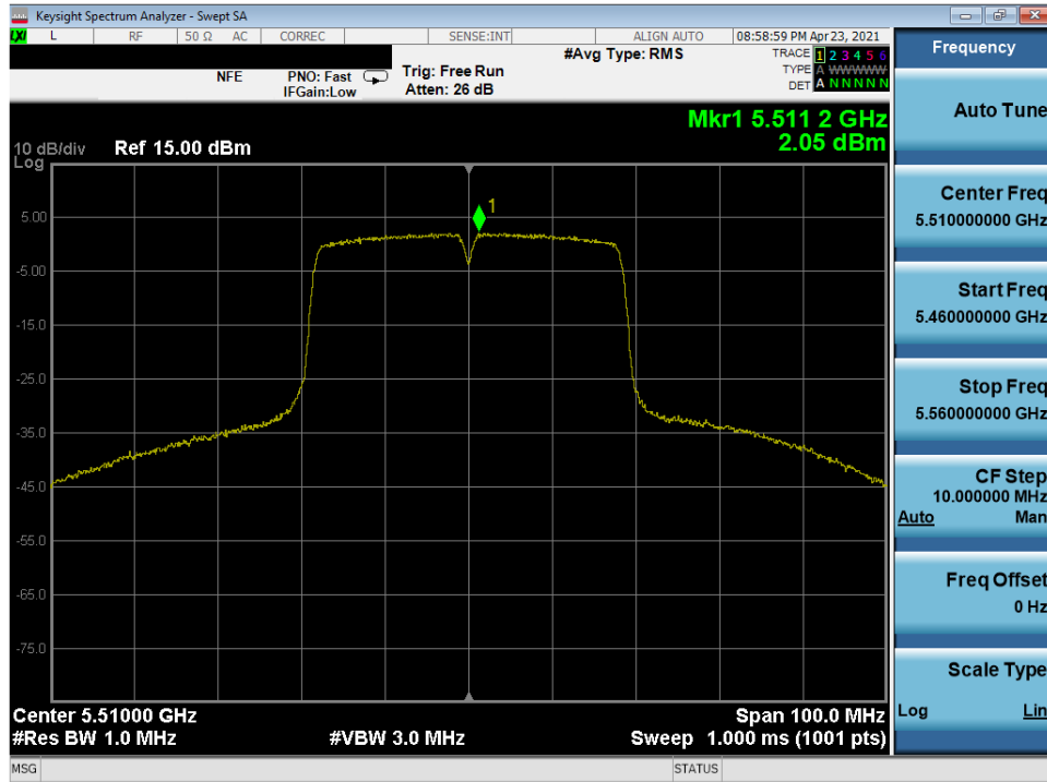
Plot 7-289. Power Spectral Density Plot MIMO ANT2 (40MHz 802.11n (UNII Band 2C) – Ch. 102)
