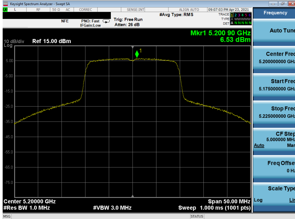
Plot 7-257. Power Spectral Density Plot MIMO ANT2 (20MHz 802.11ax (UNII Band 1) – Ch. 40)
