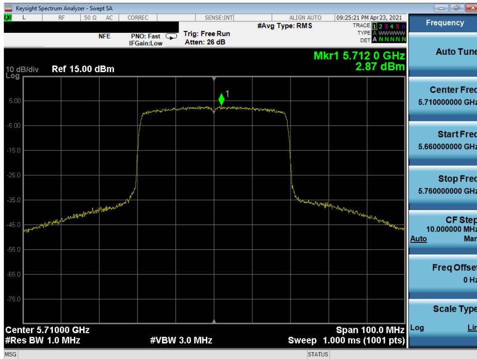
Plot 7-294. Power Spectral Density Plot MIMO ANT2 (40MHz 802.11ax (UNII Band 2C) – Ch.142)
