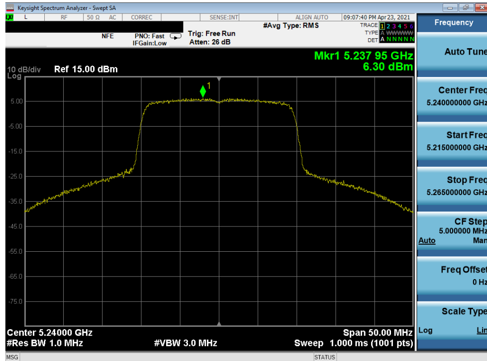
Plot 7-258. Power Spectral Density Plot MIMO ANT2 (20MHz 802.11ax (UNII Band 1) – Ch. 48)
