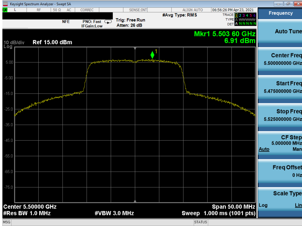
Plot 7-235. Power Spectral Density Plot MIMO ANT1 (20MHz 802.11ax (UNII Band 2C) – Ch. 100)
