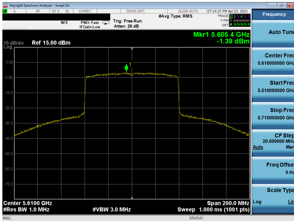
Plot 7-248. Power Spectral Density Plot MIMO ANT1 (80MHz 802.11ax (UNII Band 2C) – Ch. 122)
