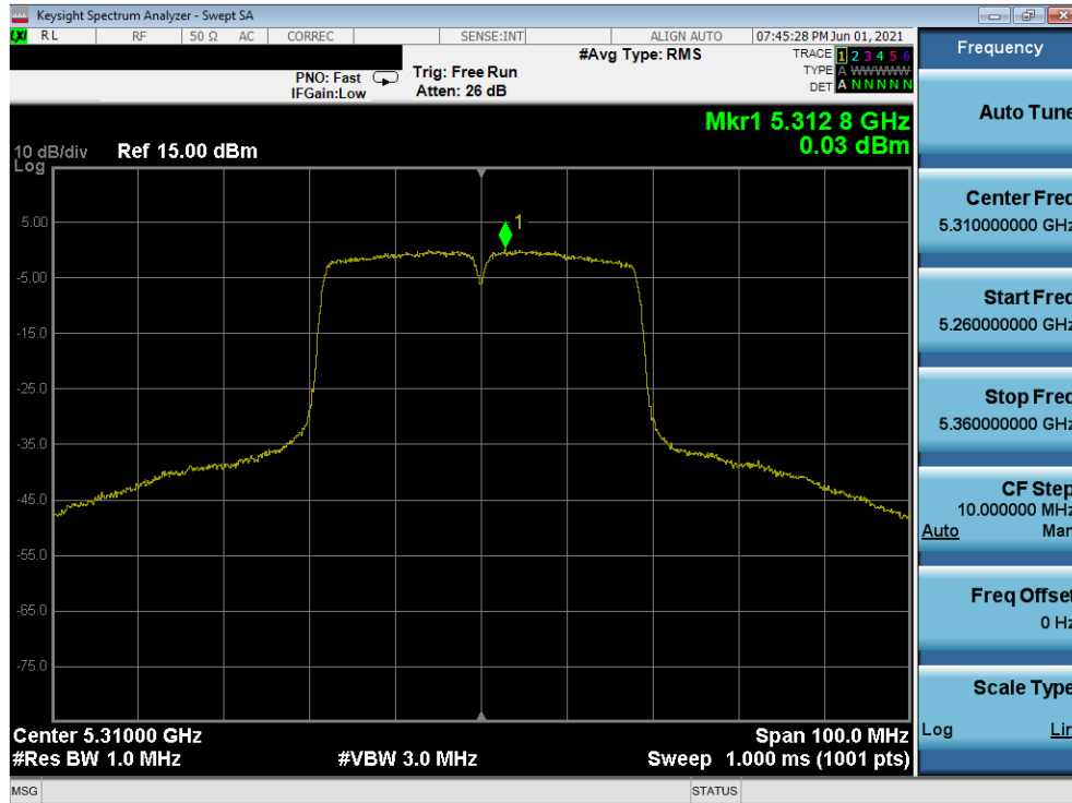
Plot 7-275. Power Spectral Density Plot MIMO ANT2 (40MHz 802.11n (UNII Band 2A) – Ch. 62)
