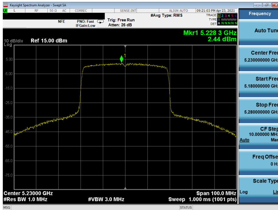
Plot 7-262. Power Spectral Density Plot MIMO ANT2 (40MHz 802.11ax (UNII Band 1) – Ch. 46)
