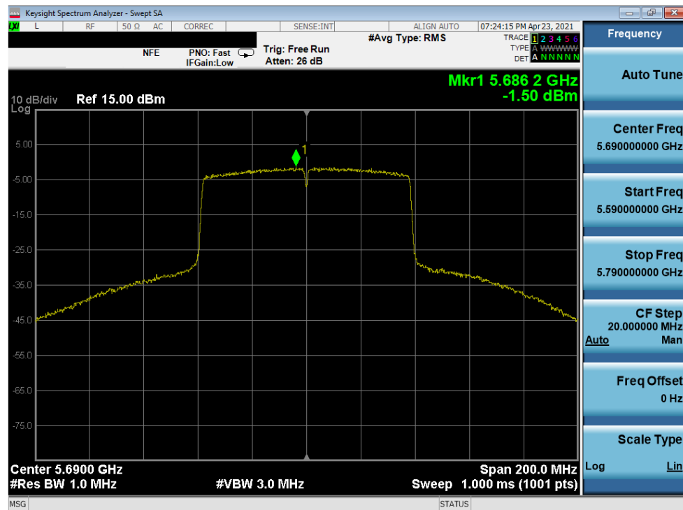
Plot 7-246. Power Spectral Density Plot MIMO ANT1 (80MHz 802.11ac (UNII Band 2C) – Ch.138)
