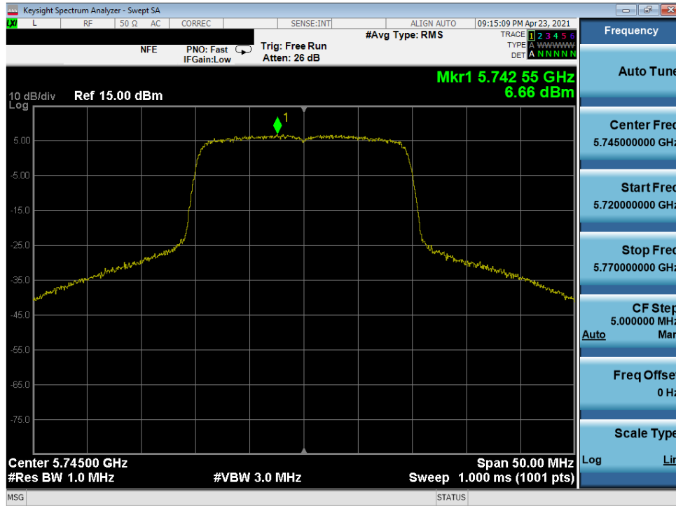
Plot 7-322. Power Spectral Density Plot MIMO ANT2 (20MHz 802.11ax (UNII Band 3) – Ch. 149)
