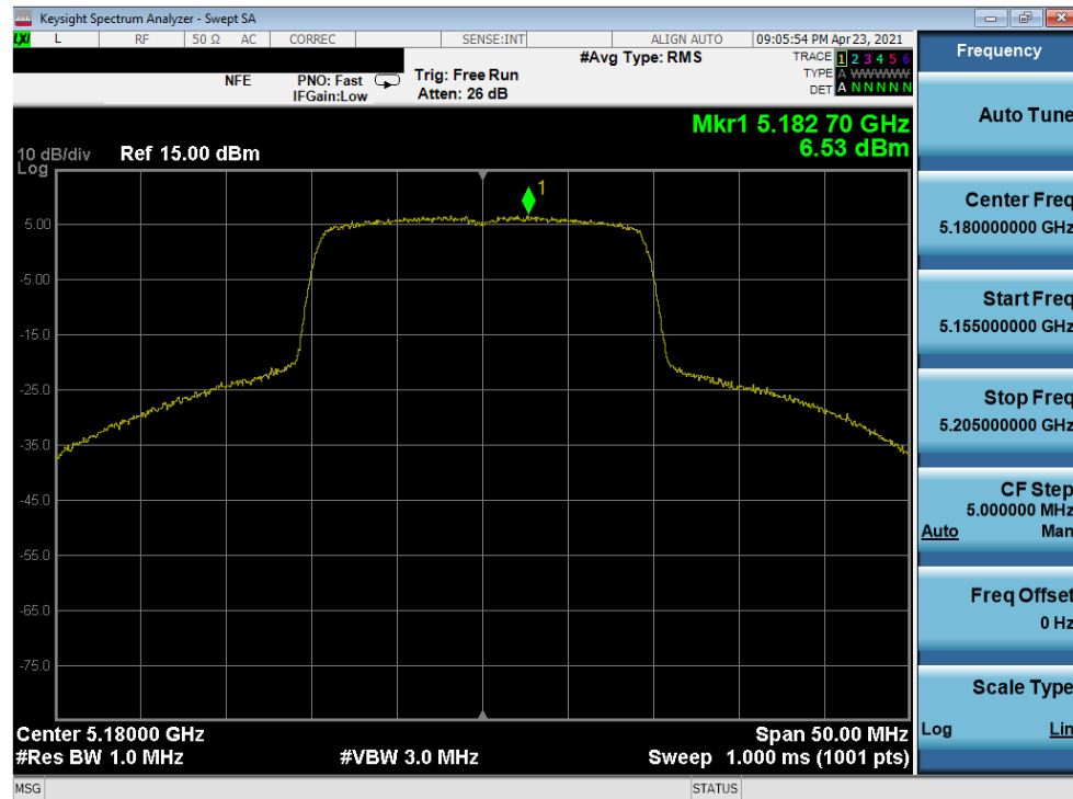
Plot 7-256. Power Spectral Density Plot MIMO ANT2 (20MHz 802.11ax (UNII Band 1) – Ch. 36)
