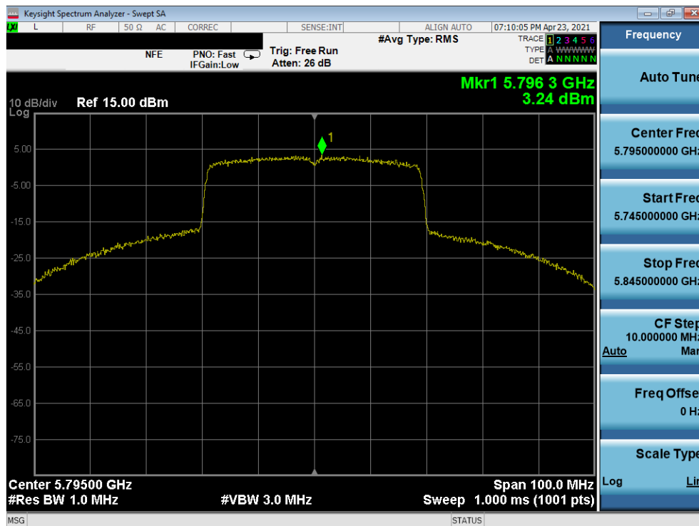
Plot 7-313. Power Spectral Density Plot MIMO ANT1 (40MHz 802.11ax (UNII Band 3) – Ch. 159)
