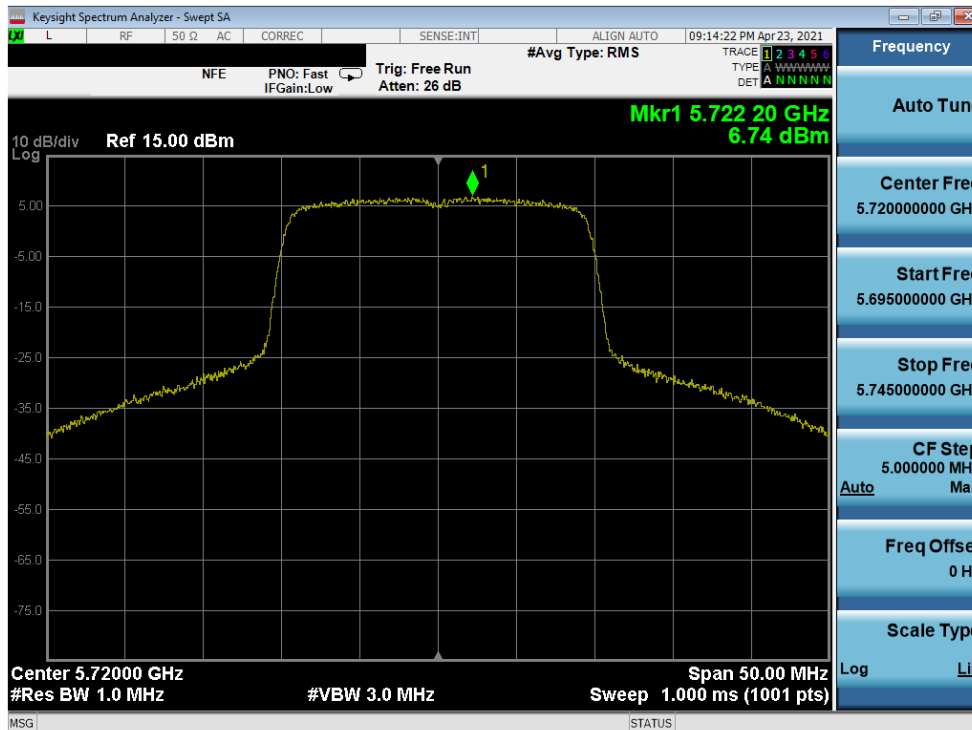
Plot 7-288. Power Spectral Density Plot MIMO ANT2 (20MHz 802.11ax (UNII Band 2C) – Ch.144)
