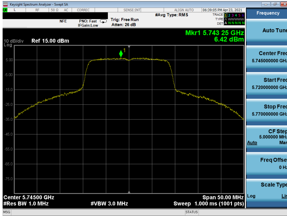
Plot 7-304. Power Spectral Density Plot MIMO ANT1 (20MHz 802.11n (UNII Band 3) – Ch. 149)
