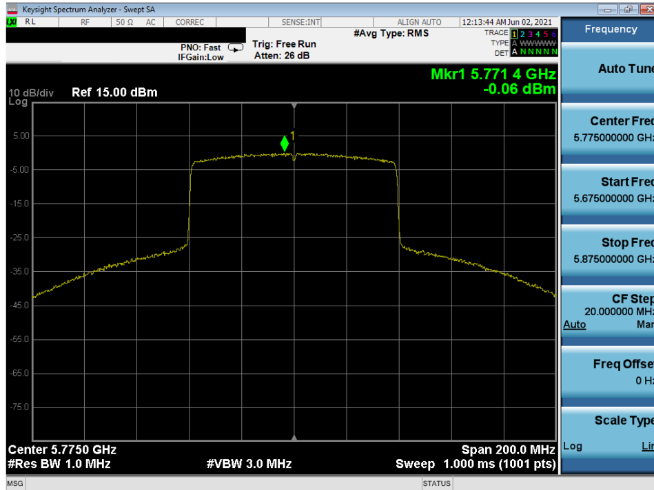
Plot 7-330. Power Spectral Density Plot MIMO ANT2 (80MHz 802.11ax (UNII Band 3) – Ch. 155)
