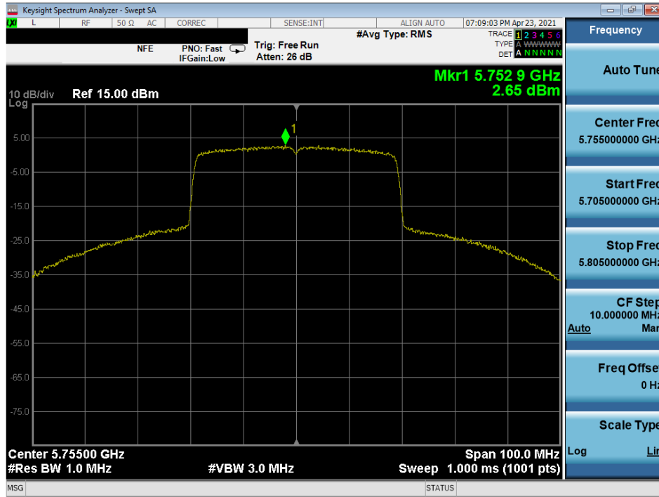
Plot 7-312. Power Spectral Density Plot MIMO ANT1 (40MHz 802.11ax (UNII Band 3) – Ch. 151)
