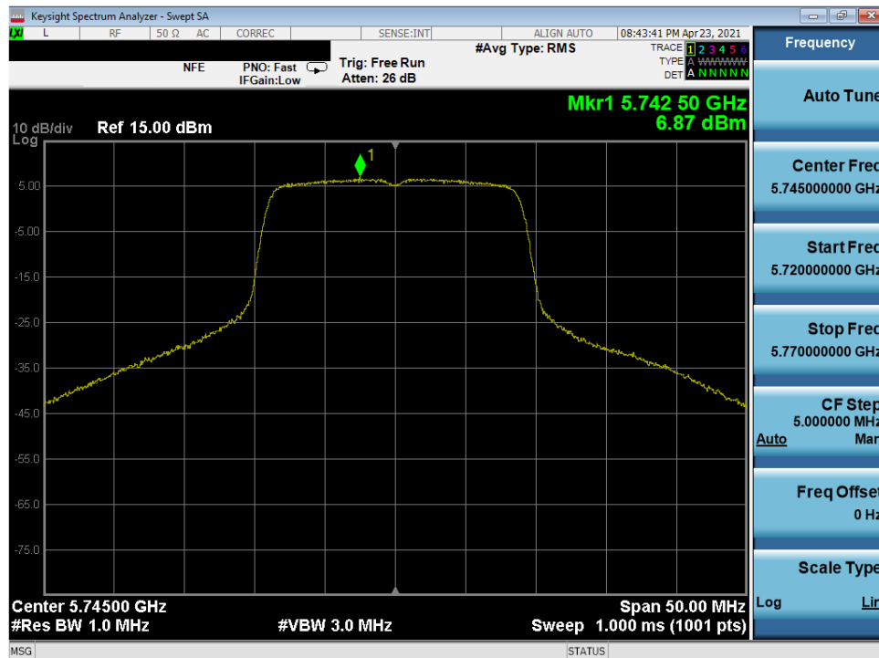
Plot 7-319. Power Spectral Density Plot MIMO ANT2 (20MHz 802.11n (UNII Band 3) – Ch. 149)
