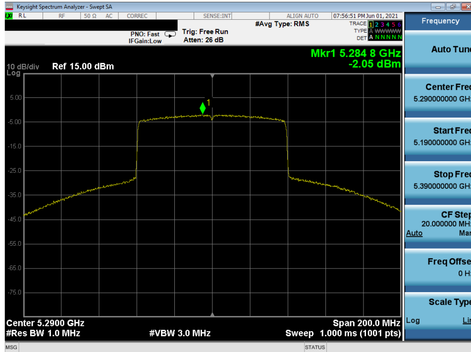
Plot 7-227. Power Spectral Density Plot MIMO ANT1 (80MHz 802.11ac (UNII Band 2A) – Ch. 58)
