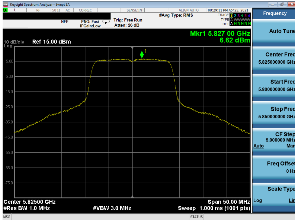
Plot 7-318. Power Spectral Density Plot MIMO ANT2 (20MHz 802.11a (UNII Band 3) – Ch. 165)
