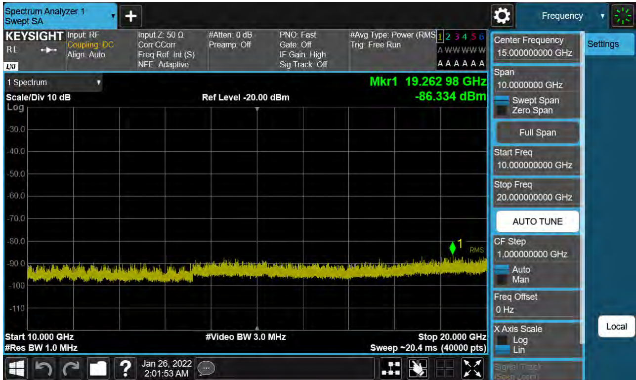
Sub6 n66. Conducted Spurious Plot_2 (343000ch_10 MHz_BPSK_ RB 1_1)
