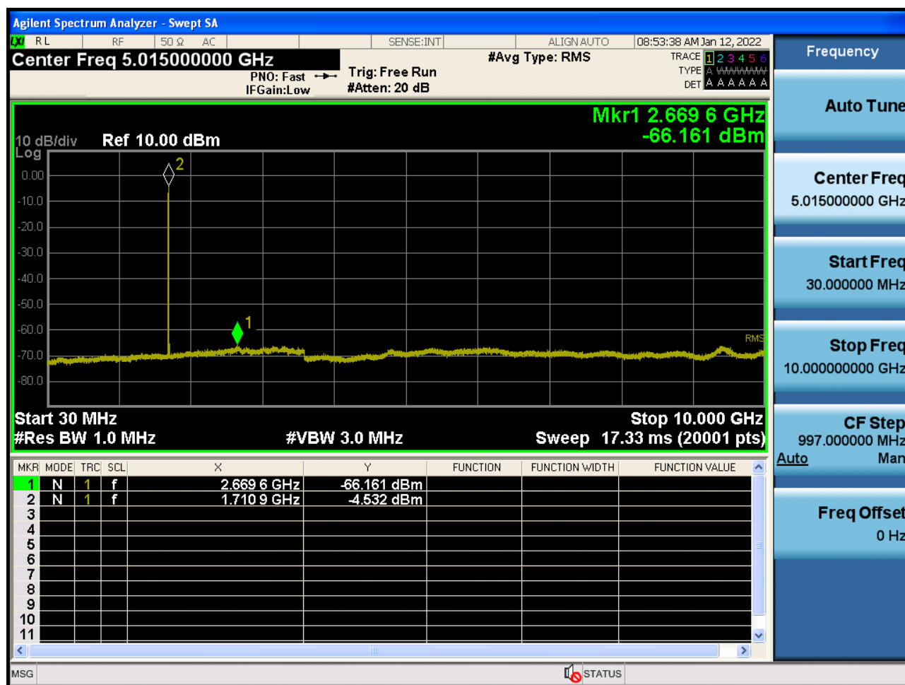
Sub6 n66. Conducted Spurious Plot_1 (344000ch_20 MHz_BPSK_ RB 1_1)
