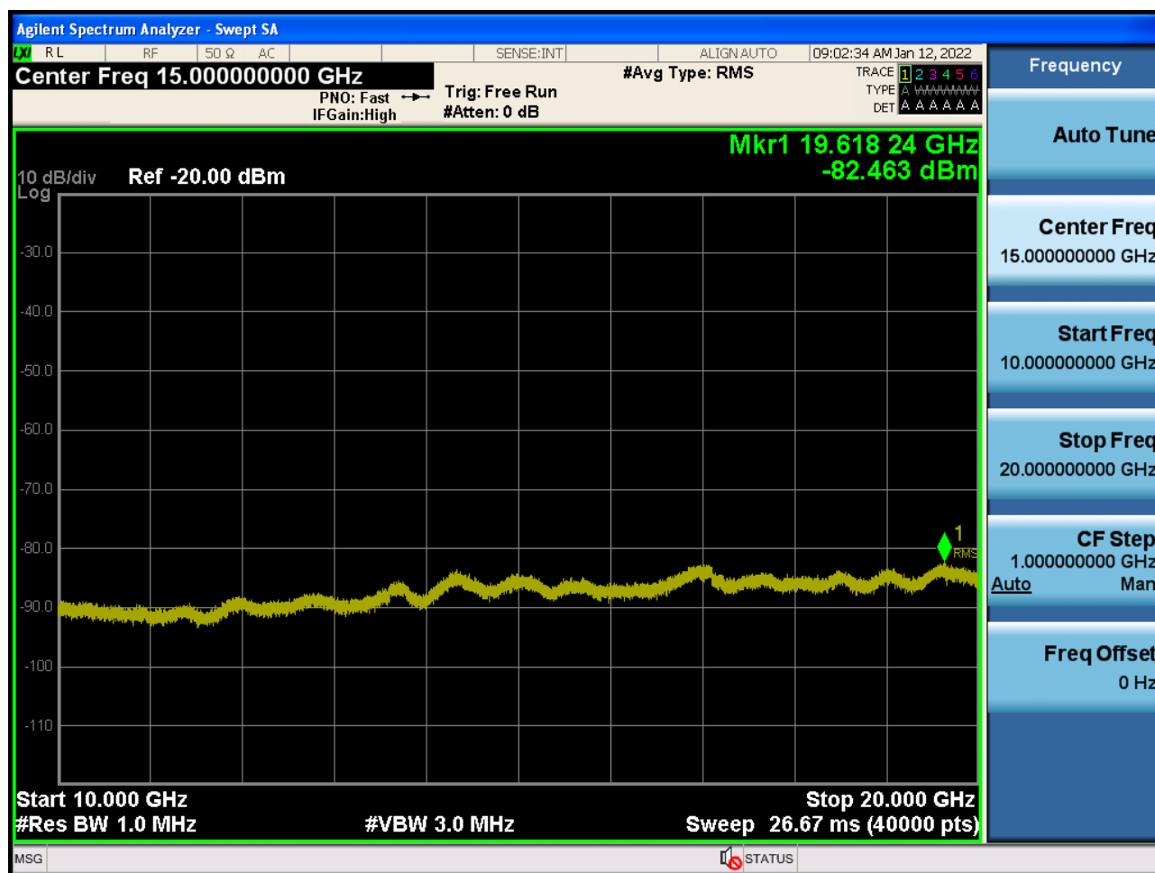
Sub6 n66. Conducted Spurious Plot_2 (354000ch_20 MHz_BPSK_ RB 1_1)
