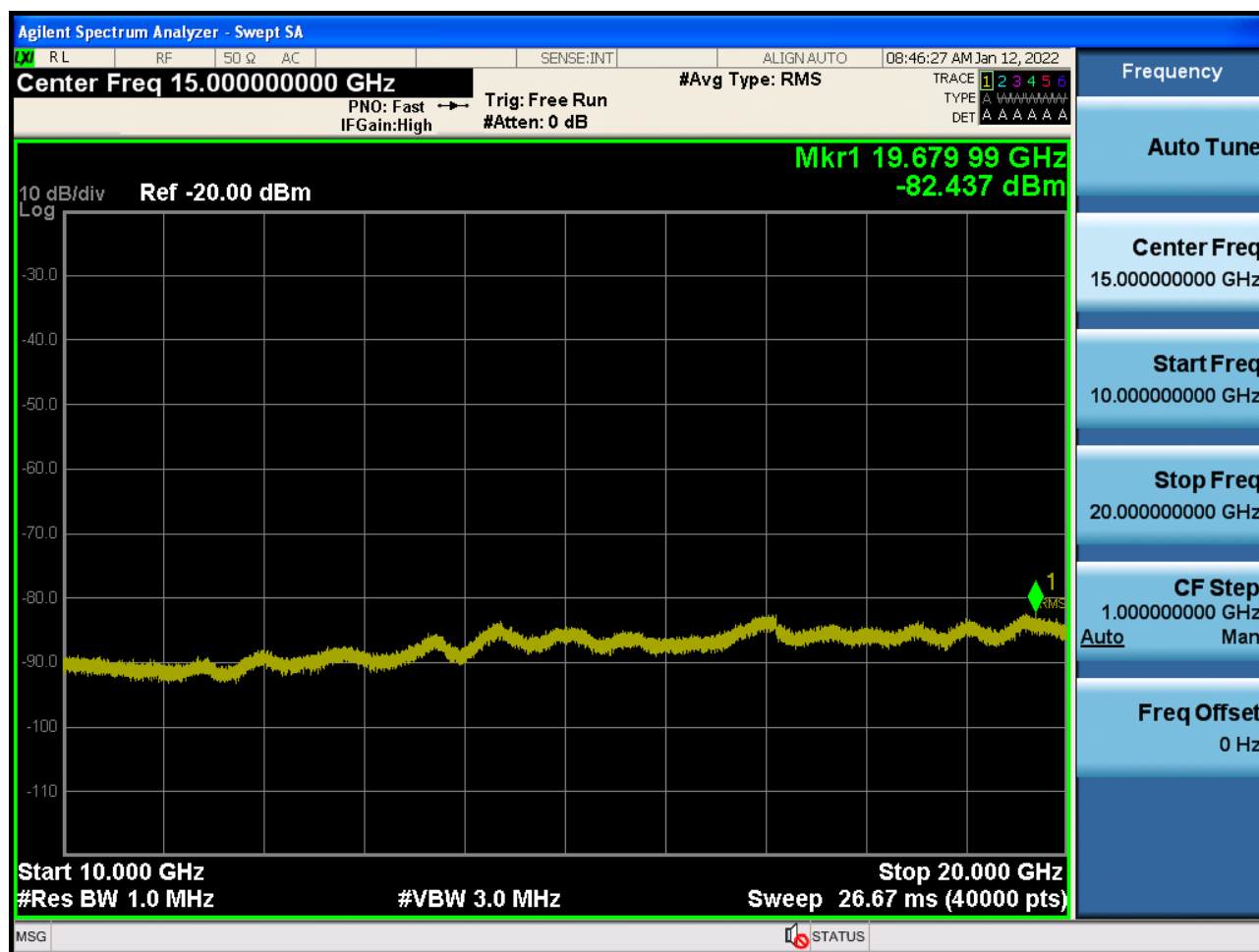
Sub6 n66. Conducted Spurious Plot_2 (349000ch_15 MHz_BPSK_ RB 1_1)
