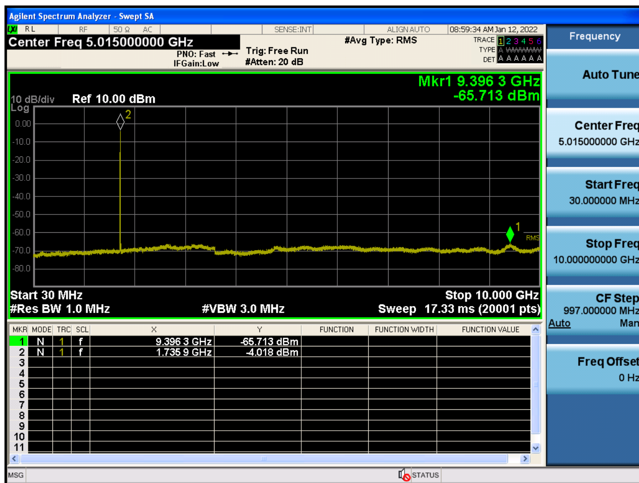
Sub6 n66. Conducted Spurious Plot_1 (349000ch_20 MHz_BPSK_ RB 1_1)
