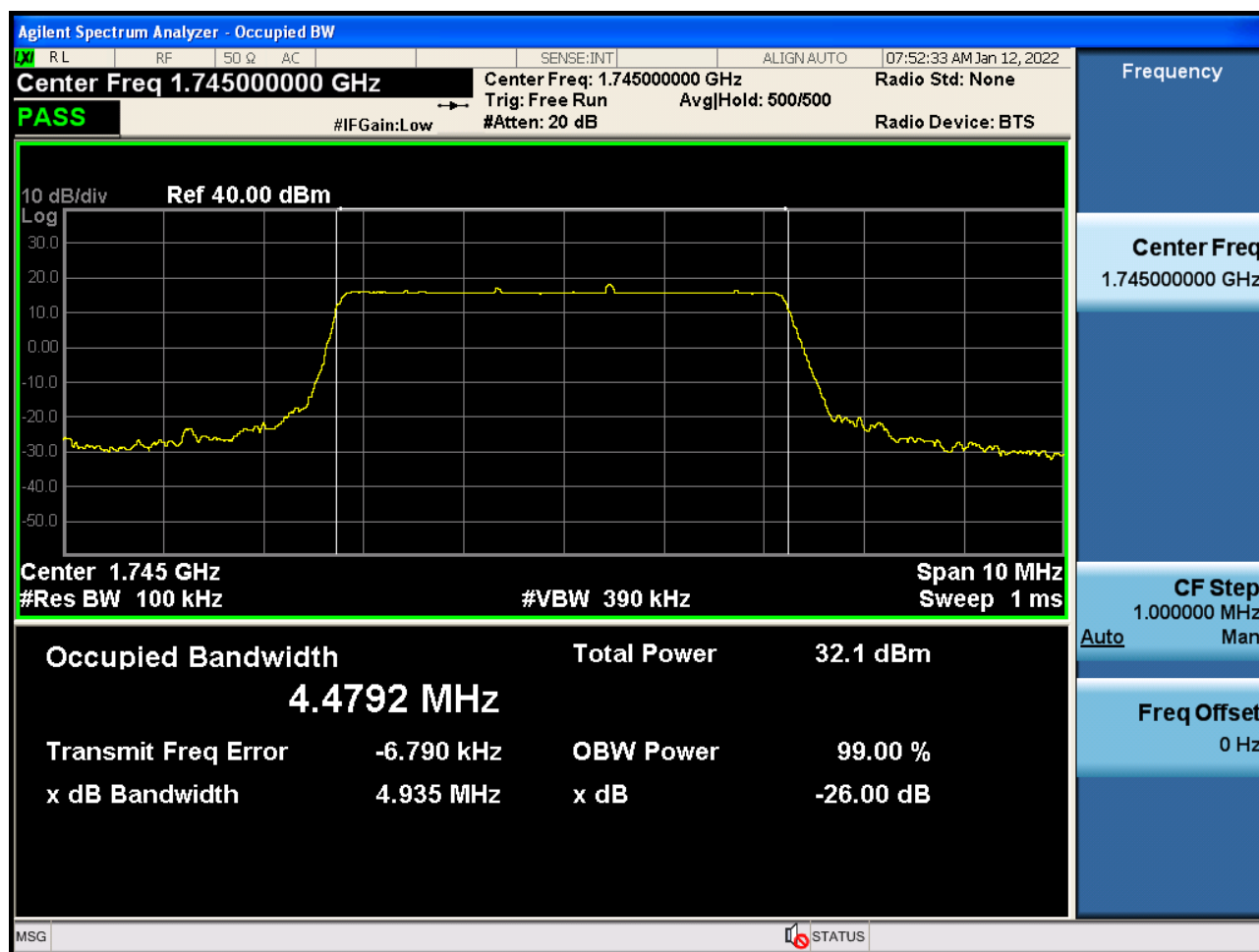
Sub6 n66. Occupied Bandwidth Plot (5 M BW Ch.349000 QPSK Full RB)
