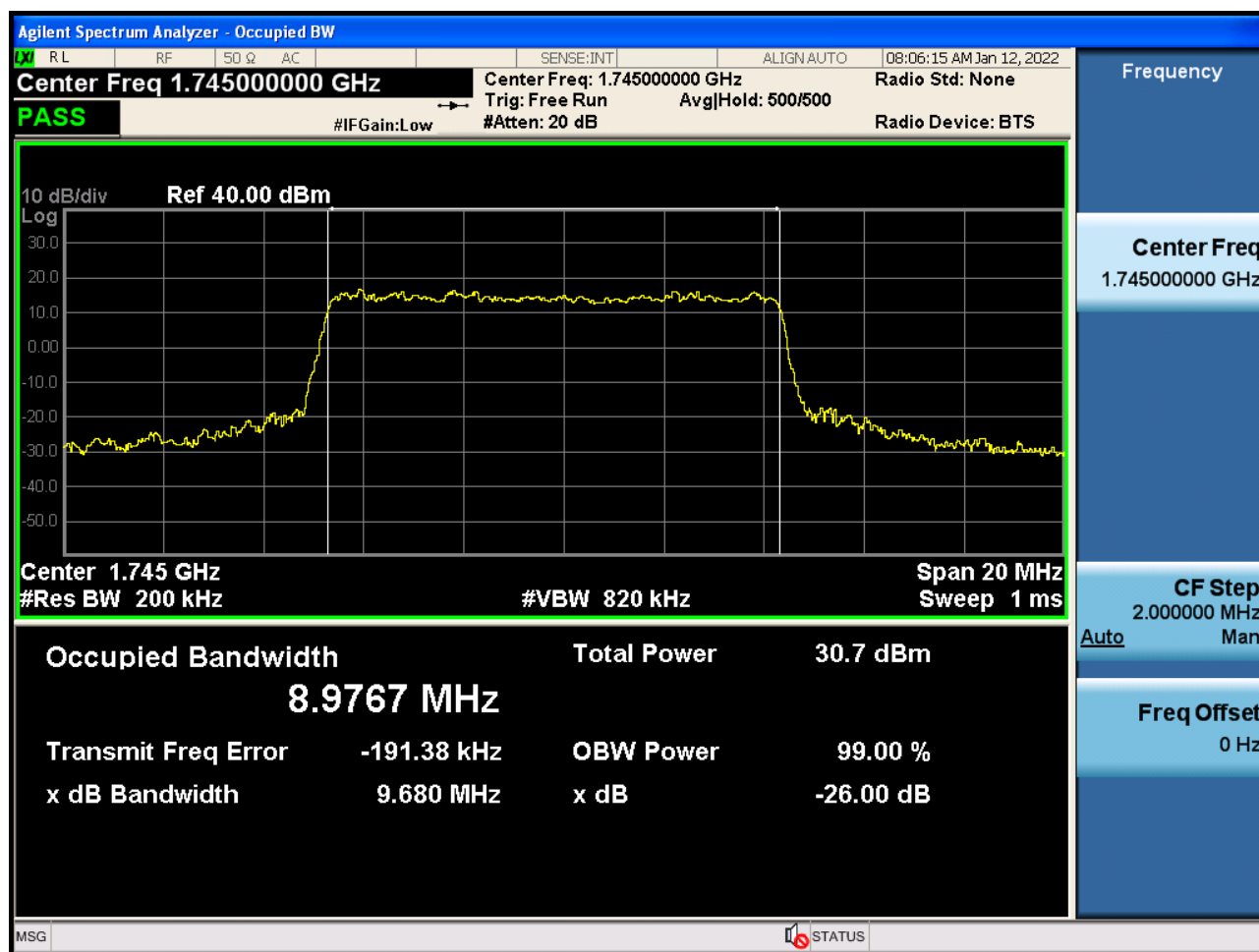
Sub6 n66. Occupied Bandwidth Plot (10 M BW Ch.349000 16QAM Full RB)
