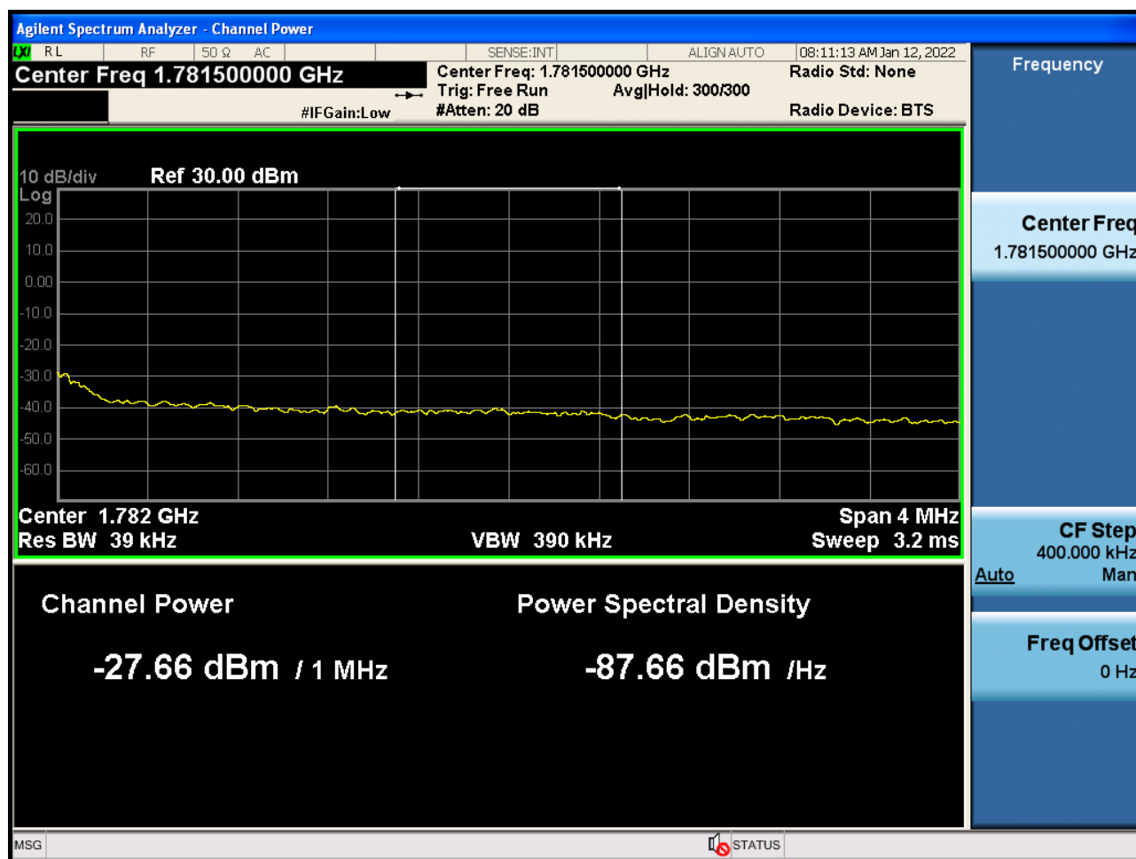
Sub6 n66. Upper Extended Band Edge Plot (10 M BW Ch.355000 BPSK_ Full RB) -3
