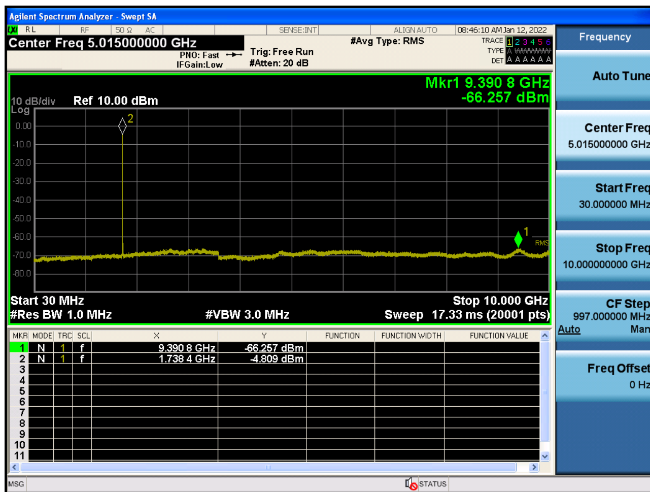
Sub6 n66. Conducted Spurious Plot_1 (349000ch_15 MHz_BPSK_ RB 1_1)
