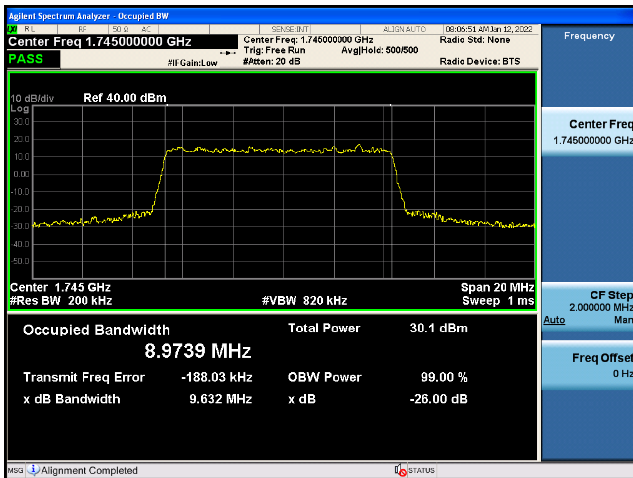
Sub6 n66. Occupied Bandwidth Plot (10 M BW Ch.349000 64QAM Full RB)
