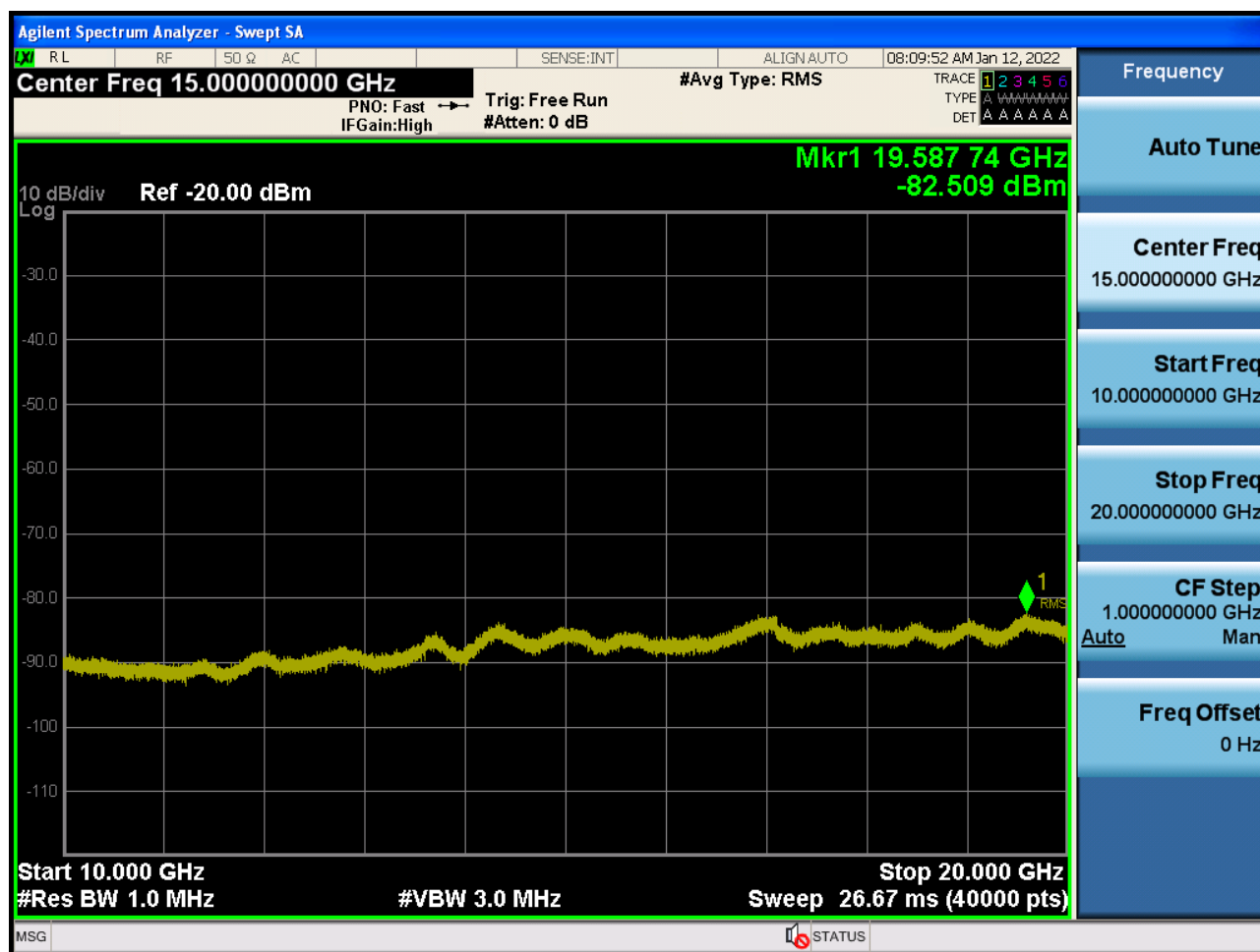
Sub6 n66. Conducted Spurious Plot_2 (349000ch_10 MHz_BPSK_ RB 1_1)
