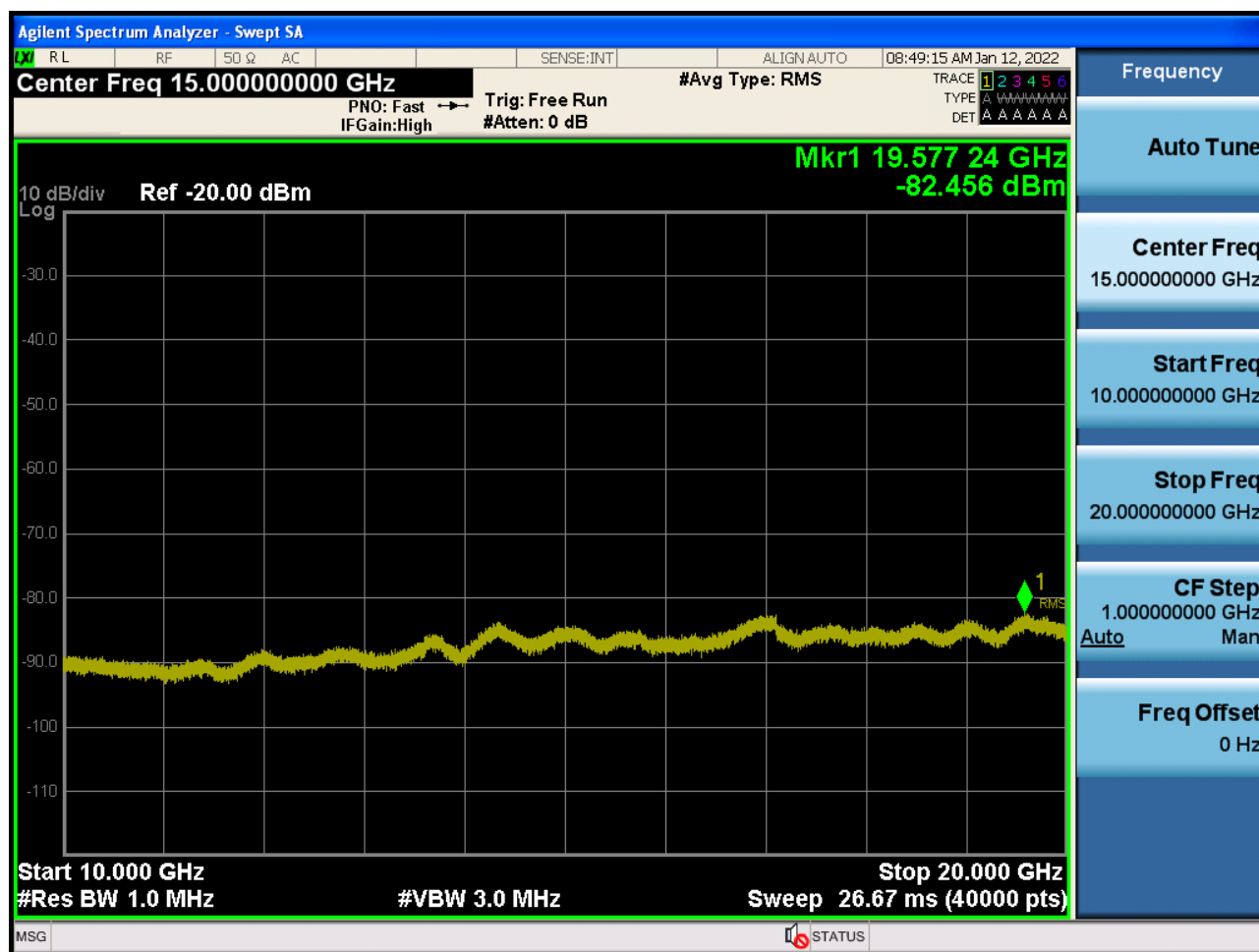
Sub6 n66. Conducted Spurious Plot_2 (354500ch_15 MHz_BPSK_ RB 1_1)
