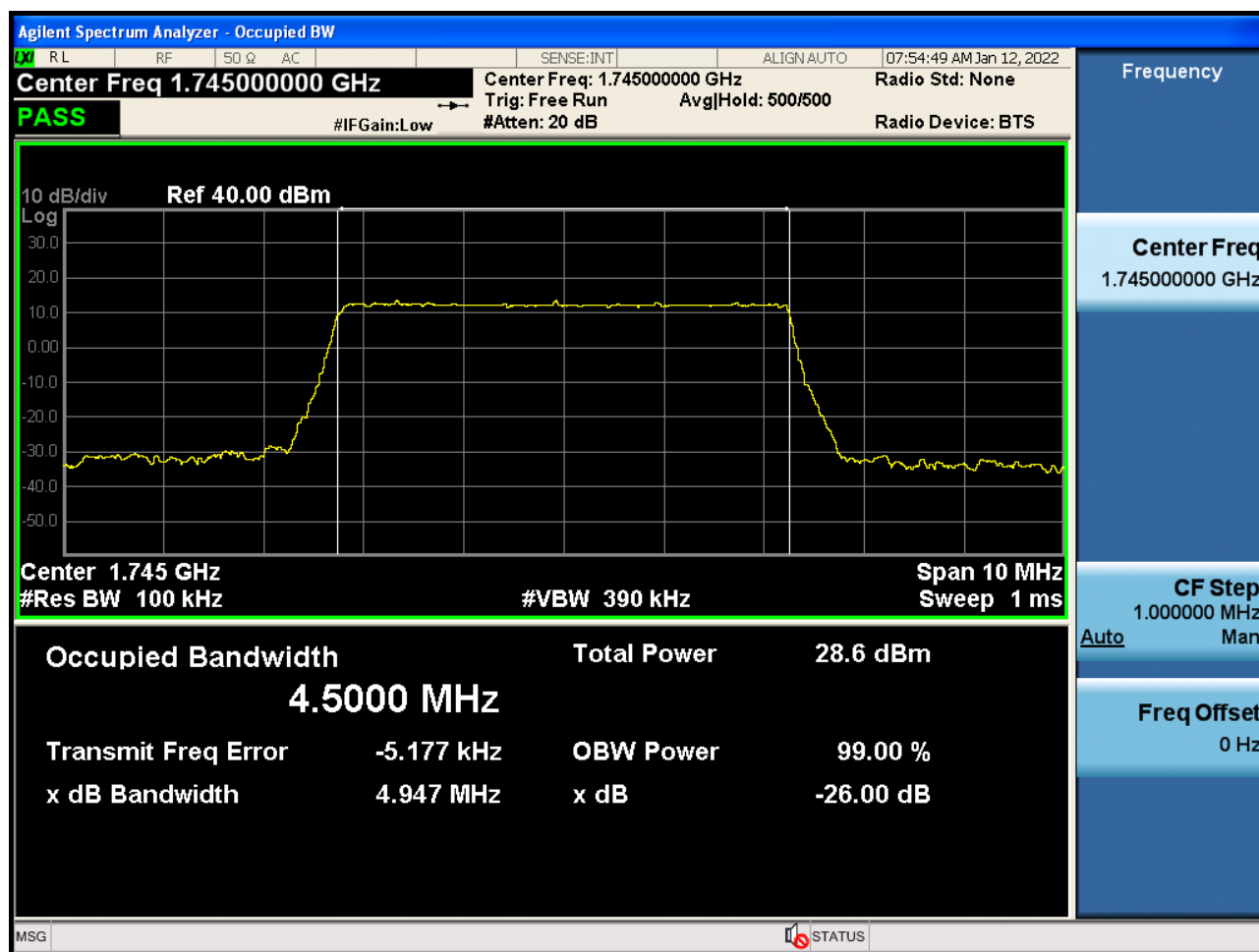
Sub6 n66. Occupied Bandwidth Plot (5 M BW Ch.349000 256QAM Full RB)
