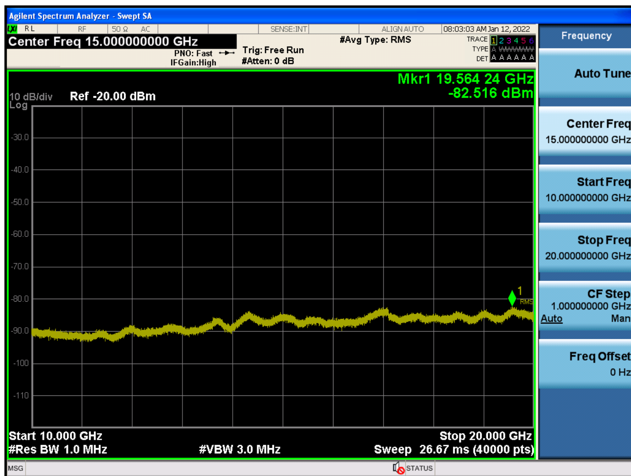
Sub6 n66. Conducted Spurious Plot_2 (343000ch_10 MHz_BPSK_ RB 1_1)
