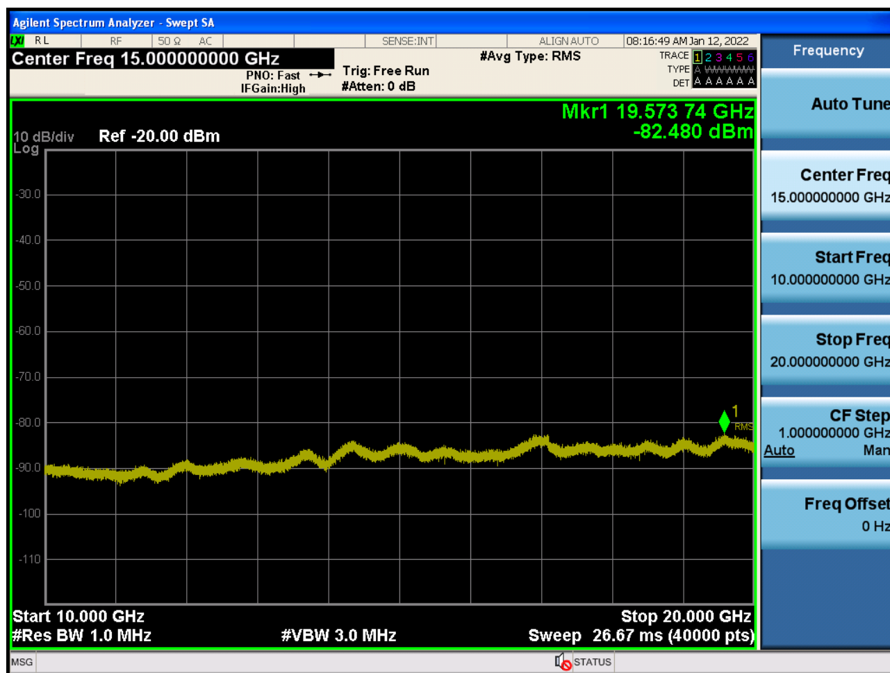
Sub6 n66. Conducted Spurious Plot_2 (343500ch_15 MHz_BPSK_ RB 1_1)
