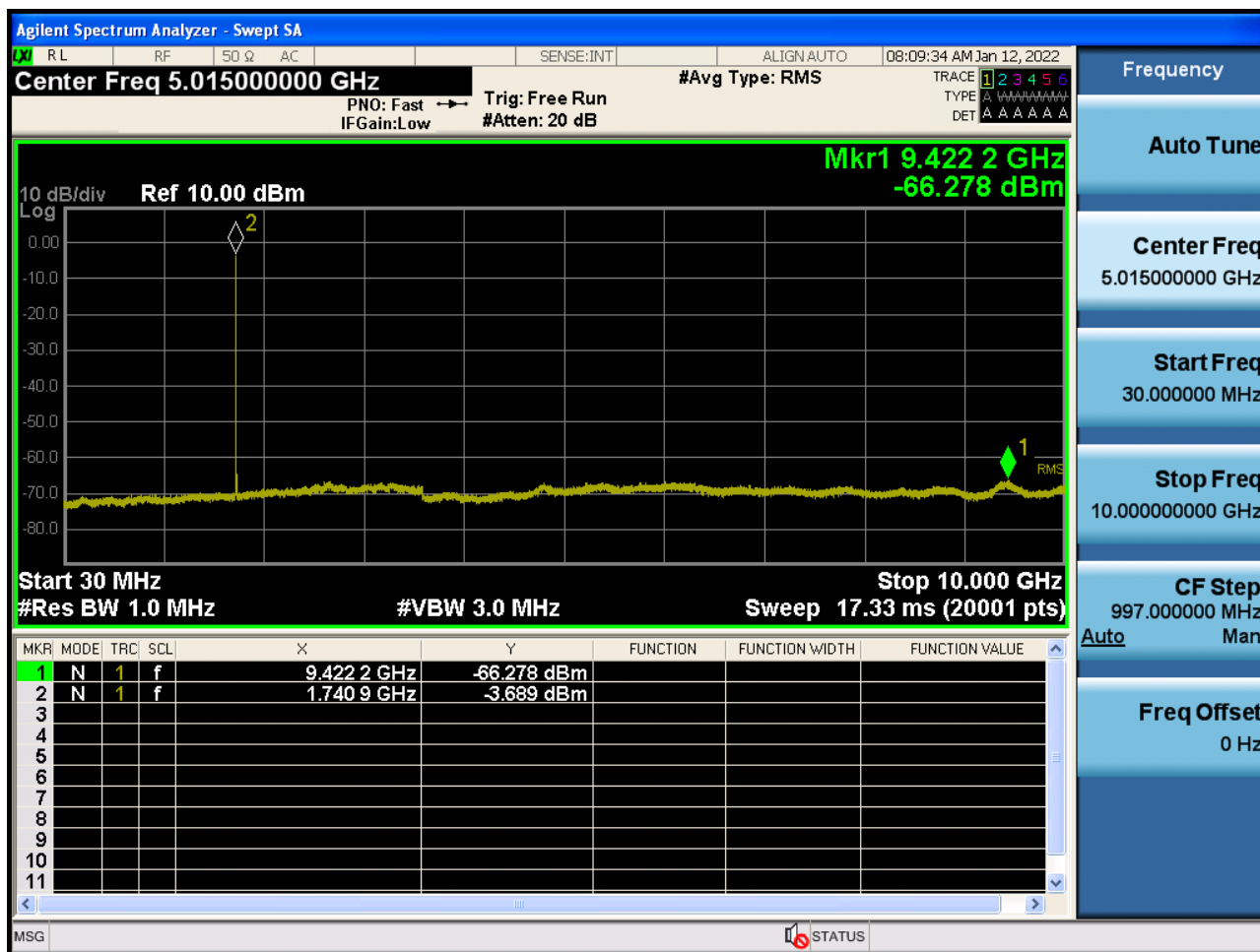
Sub6 n66. Conducted Spurious Plot_1 (349000ch_10 MHz_BPSK_ RB 1_1)
