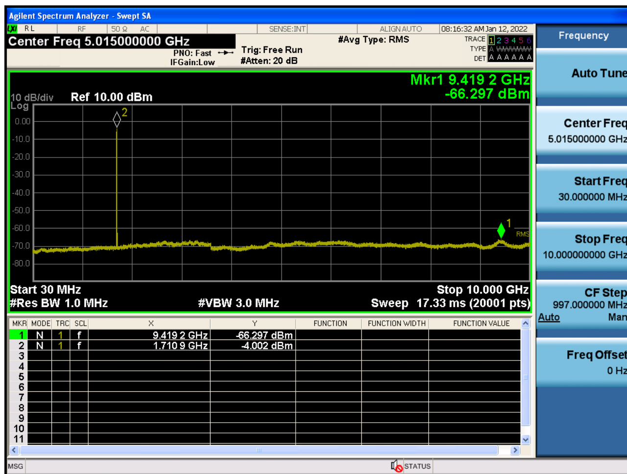
Sub6 n66. Conducted Spurious Plot_1 (343500ch_15 MHz_BPSK_ RB 1_1)
