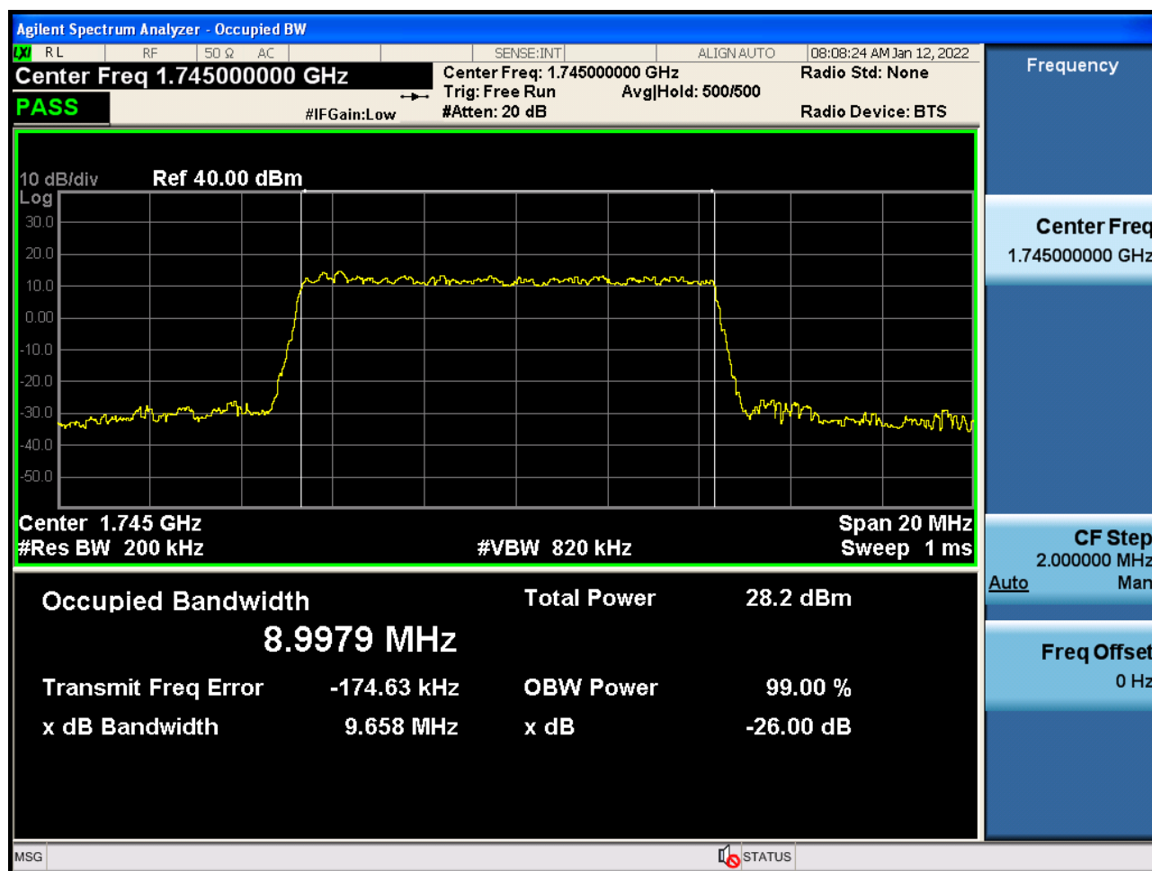
Sub6 n66. Occupied Bandwidth Plot (10 M BW Ch.349000 256QAM Full RB)
