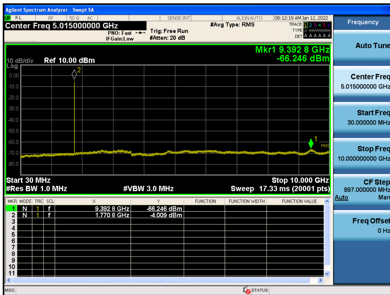
Sub6 n66. Conducted Spurious Plot_1 (355000ch_10 MHz_BPSK_ RB 1_1)
