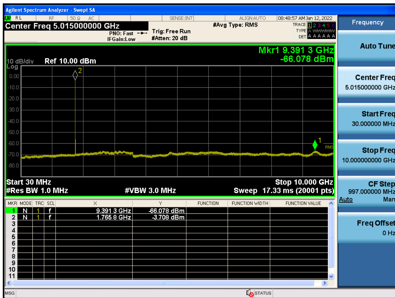
Sub6 n66. Conducted Spurious Plot_1 (354500ch_15 MHz_BPSK_ RB 1_1)
