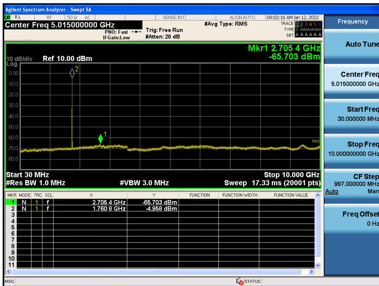
Sub6 n66. Conducted Spurious Plot_1 (354000ch_20 MHz_BPSK_ RB 1_1)
