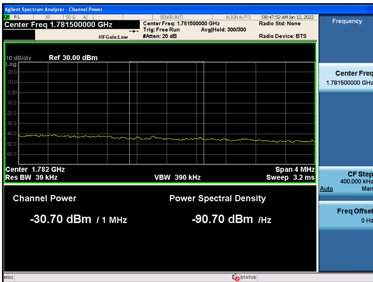
Sub6 n66. Upper Extended Band Edge Plot (15 M BW Ch.354500 BPSK_ Full RB) -3
