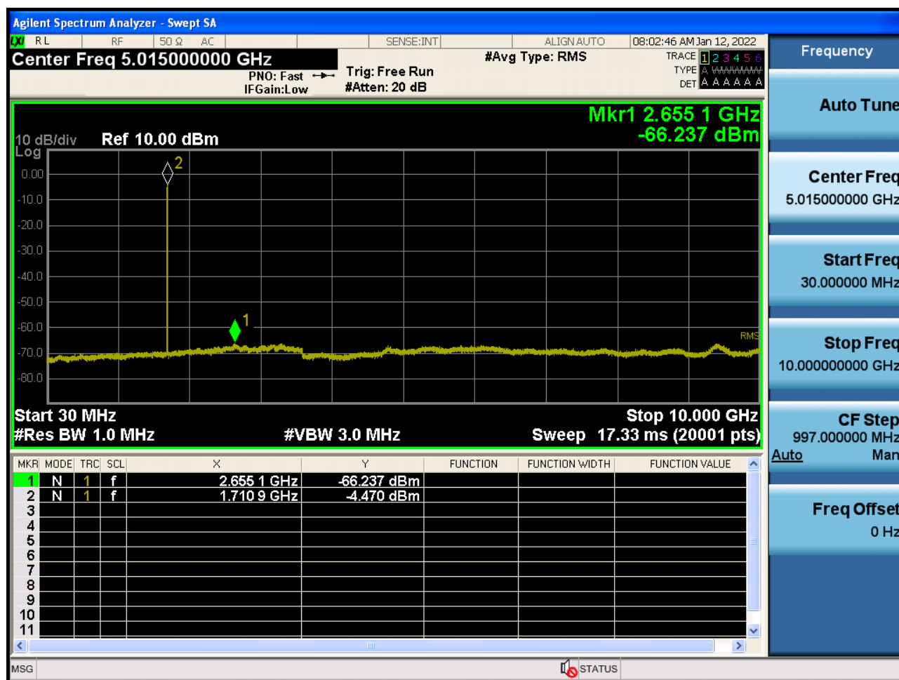
Sub6 n66. Conducted Spurious Plot_1 (343000ch_10 MHz_BPSK_ RB 1_1)
