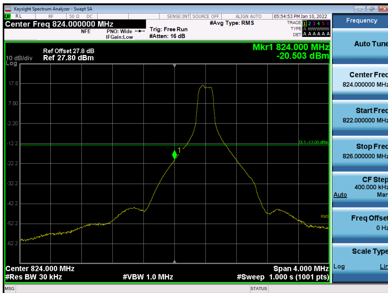
Sub6 n5. Lower Band Edge Plot (10 M BW Ch.165800 BPSK_RB1_Offset 0)
