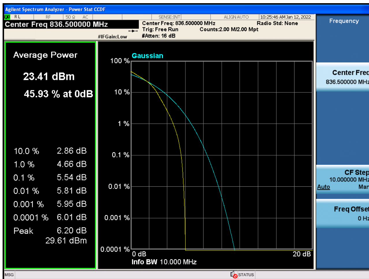
Sub6 n5. PAR Plot (10 M BW_Ch. 167300_16QAM_ Full RB _0)
