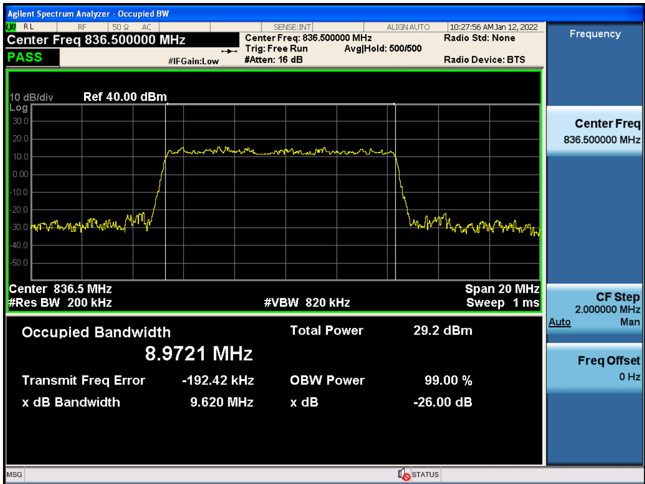
Sub6 n5. Occupied Bandwidth Plot (10 M BW Ch.167300 256QAM_ Full RB _0)
