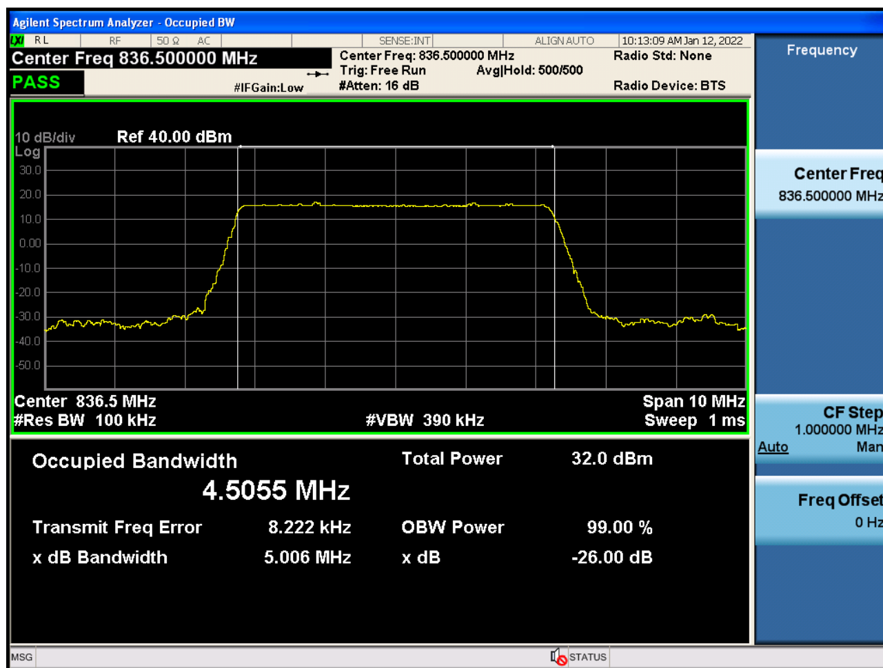
Sub6 n5. Occupied Bandwidth Plot (5 M BW Ch.167300 BPSK_Full RB_0)
