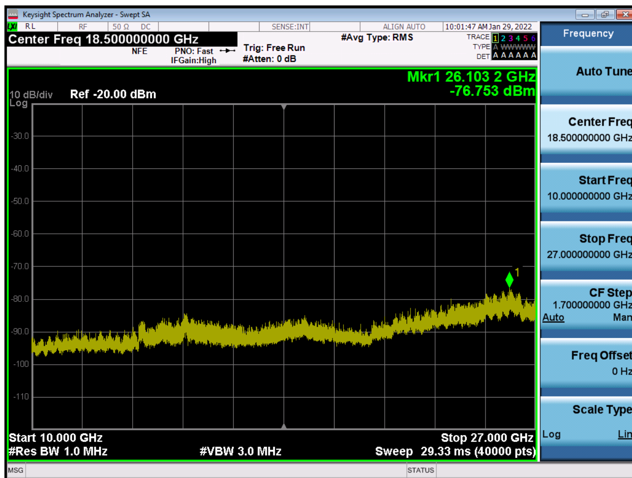
Sub6 n41. Conducted Spurious Plot 2 (40 MHz Ch.518598 BPSK RB 1)
