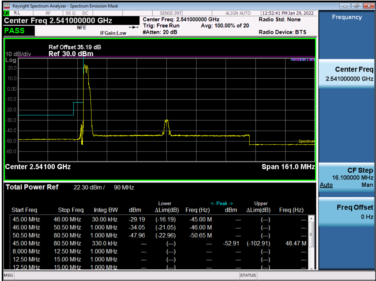
Sub6 n41. Low Channel Edge Plot (90 MHz Ch.508200 BPSK RB 1)-1
