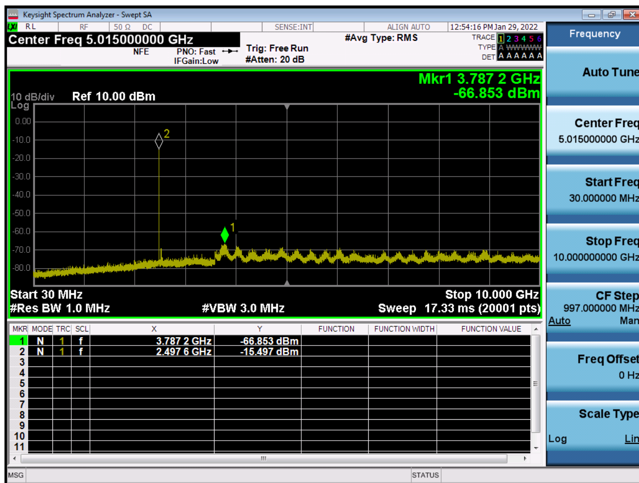
Sub6 n41. Conducted Spurious Plot 1 (90 MHz Ch.508200 BPSK RB 1)
