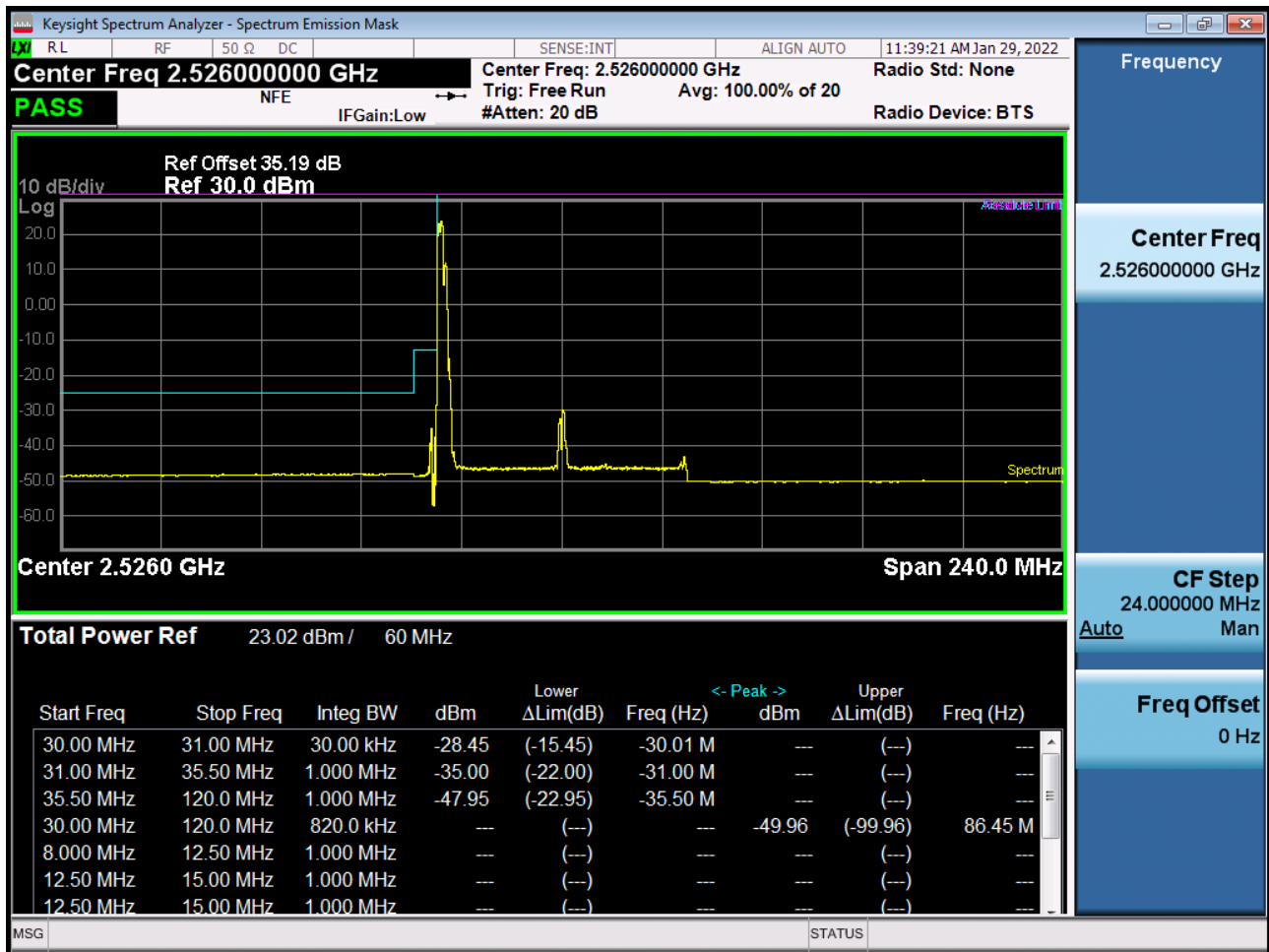
Sub6 n41. Low Channel Edge Plot (60 MHz Ch.505200 BPSK RB 1)-1
