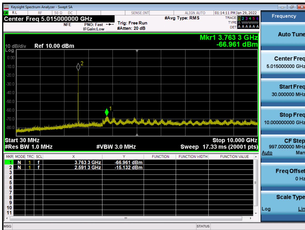
Sub6 n41. Conducted Spurious Plot 1 (100 MHz Ch.528000 BPSK RB 1)
