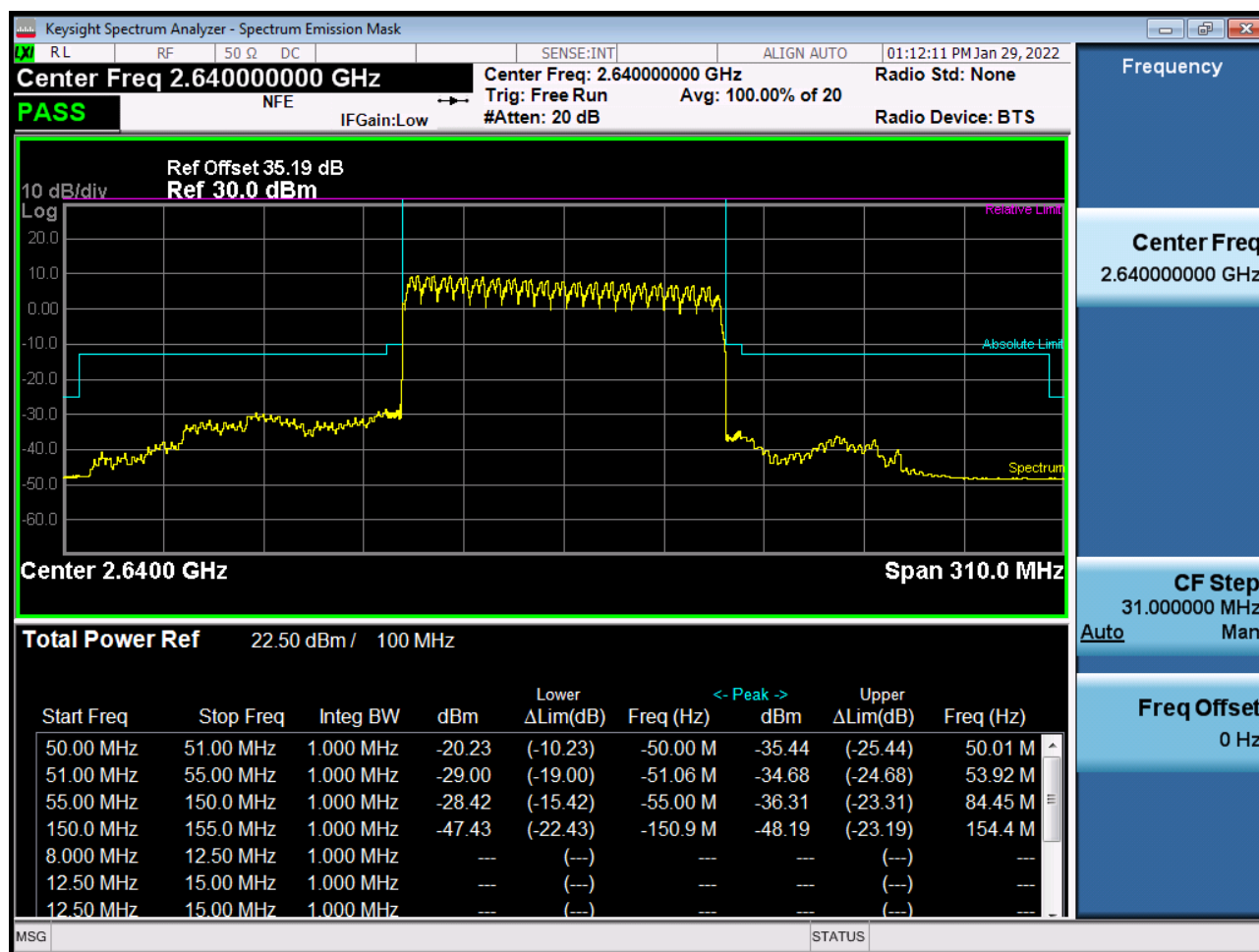
Sub6 n41. High Channel Edge Plot (100 MHz Ch.528000 BPSK)
