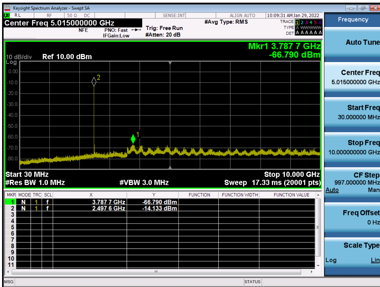
Sub6 n41. Conducted Spurious Plot 1 (50 MHz Ch.504204 BPSK RB 1)
