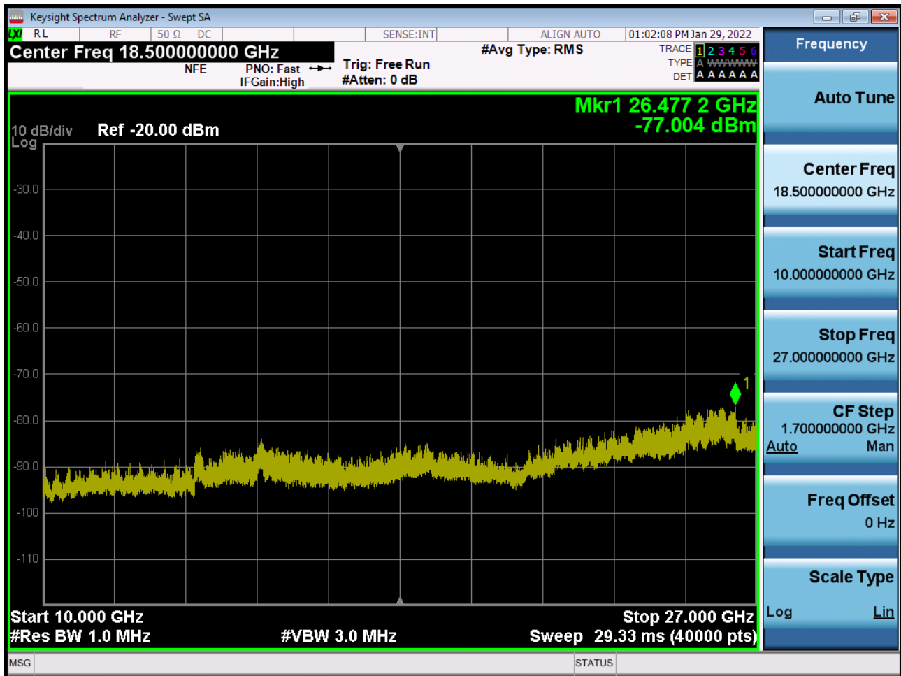
Sub6 n41. Conducted Spurious Plot 2 (90 MHz Ch.528996 BPSK RB 1)
