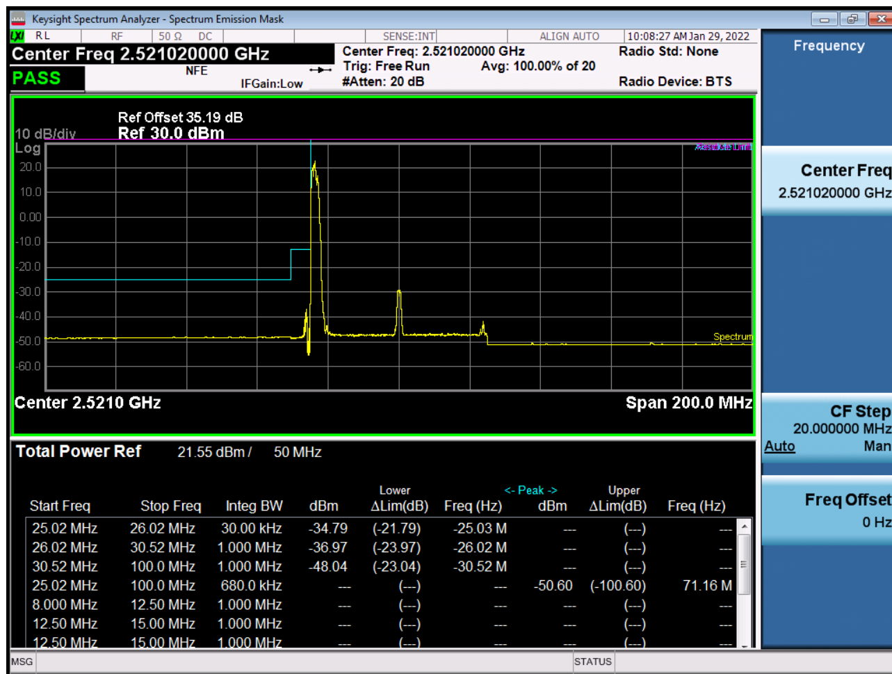
Sub6 n41. Low Channel Edge Plot (50 MHz Ch.504204 BPSK RB 1)-1
