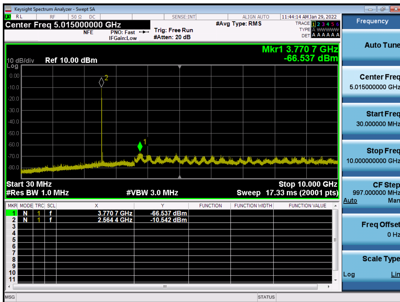
Sub6 n41. Conducted Spurious Plot 1 (60 MHz Ch.518598 BPSK RB 1)
