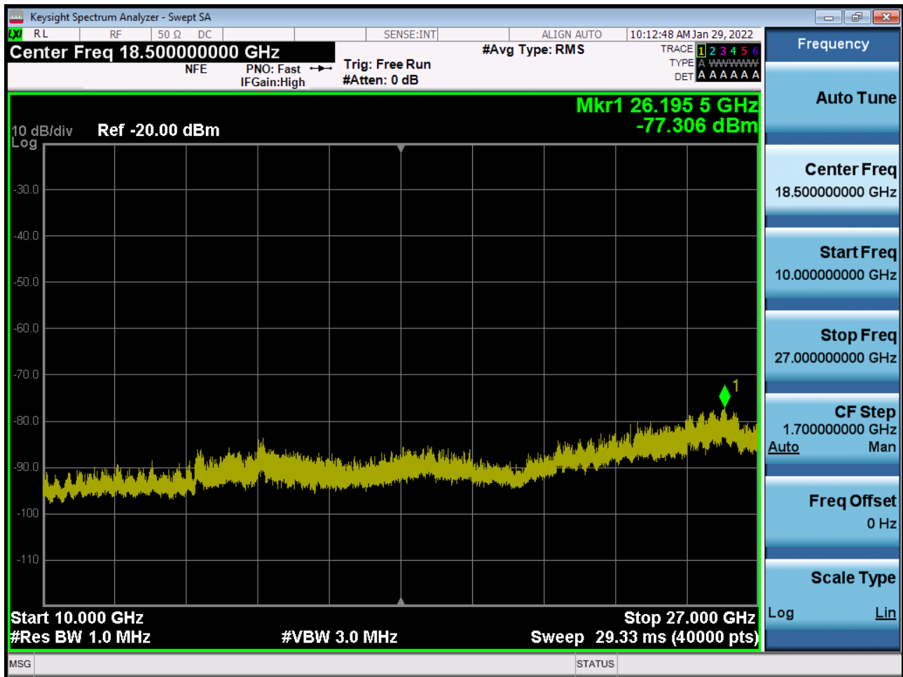
Sub6 n41. Conducted Spurious Plot 2 (50 MHz Ch. 518598 BPSK RB 1)
