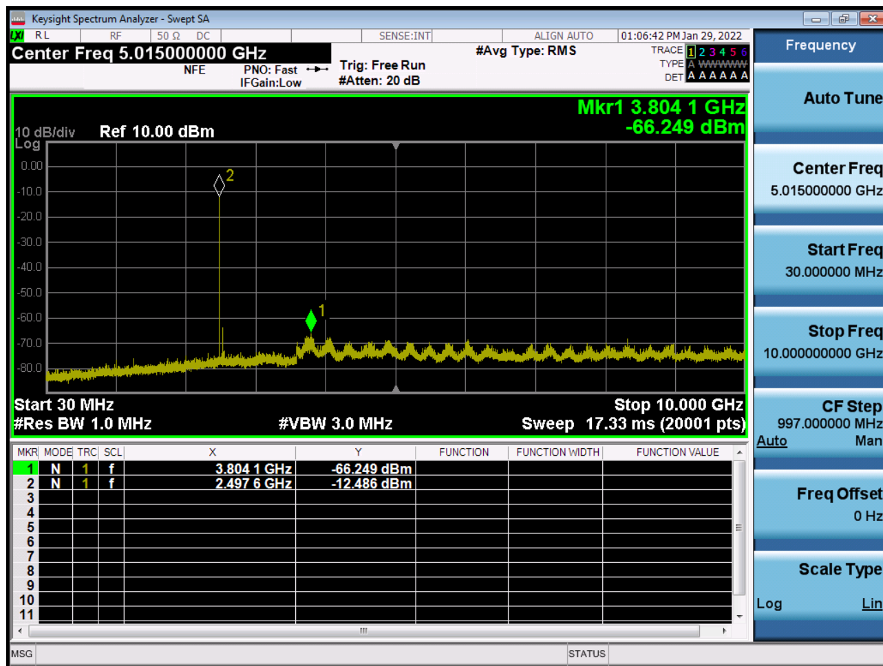
Sub6 n41. Conducted Spurious Plot 1 (100 MHz Ch.509202 BPSK RB 1)
