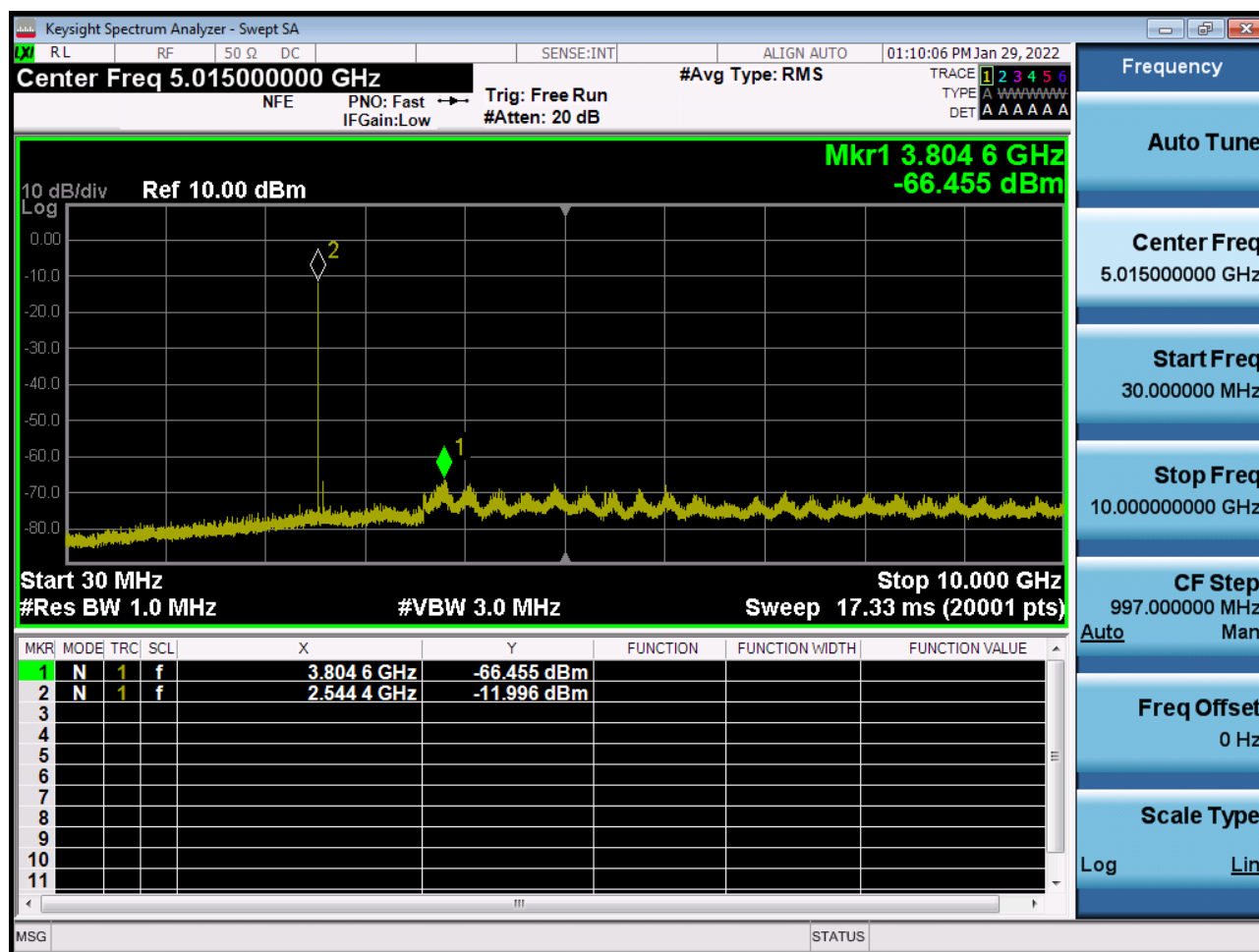
Sub6 n41. Conducted Spurious Plot 1 (100 MHz Ch.518598 BPSK RB 1)
