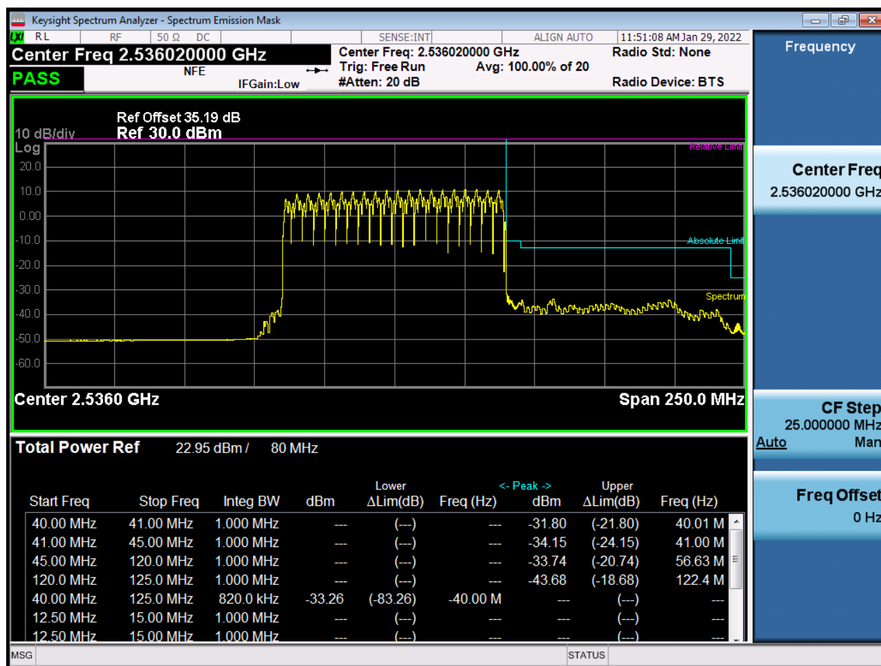
Sub6 n41. Low Channel Edge Plot (80 MHz Ch.507204 BPSK)-2
