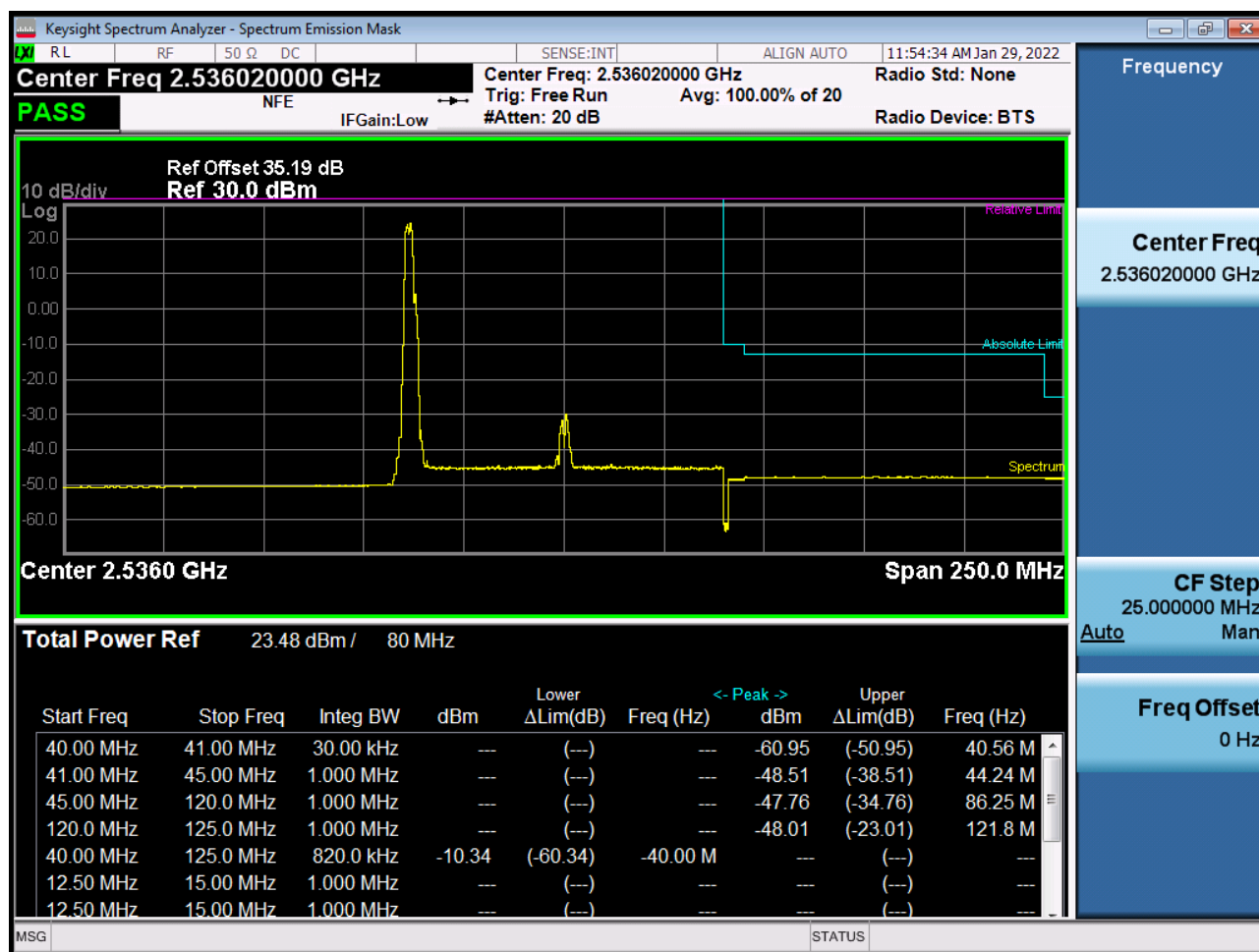
Sub6 n41. Low Channel Edge Plot (80 MHz Ch.507204 BPSK_RB1)-2
