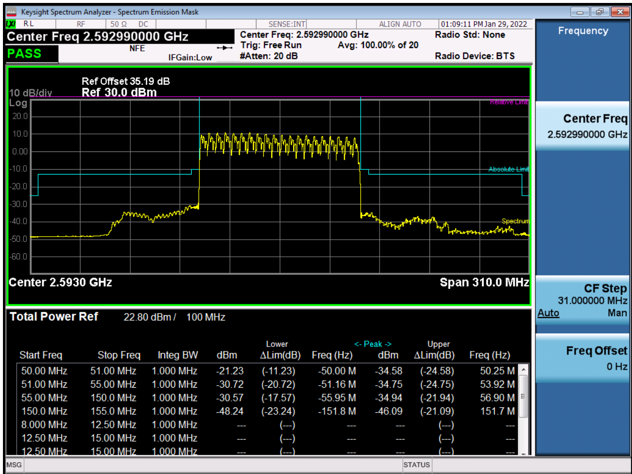
Sub6 n41. Mid Channel Edge Plot (100 MHz Ch.518598 BPSK )
