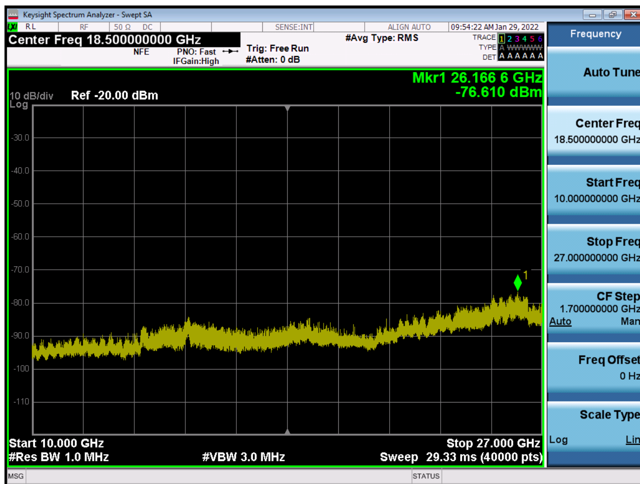
Sub6 n41. Conducted Spurious Plot 2 (30 MHz Ch.534996 BPSK RB 1)
