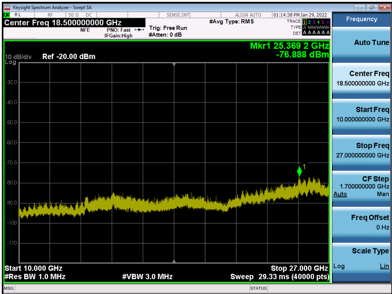
Sub6 n41. Conducted Spurious Plot 2 (100 MHz Ch.528000 BPSK RB 1)
