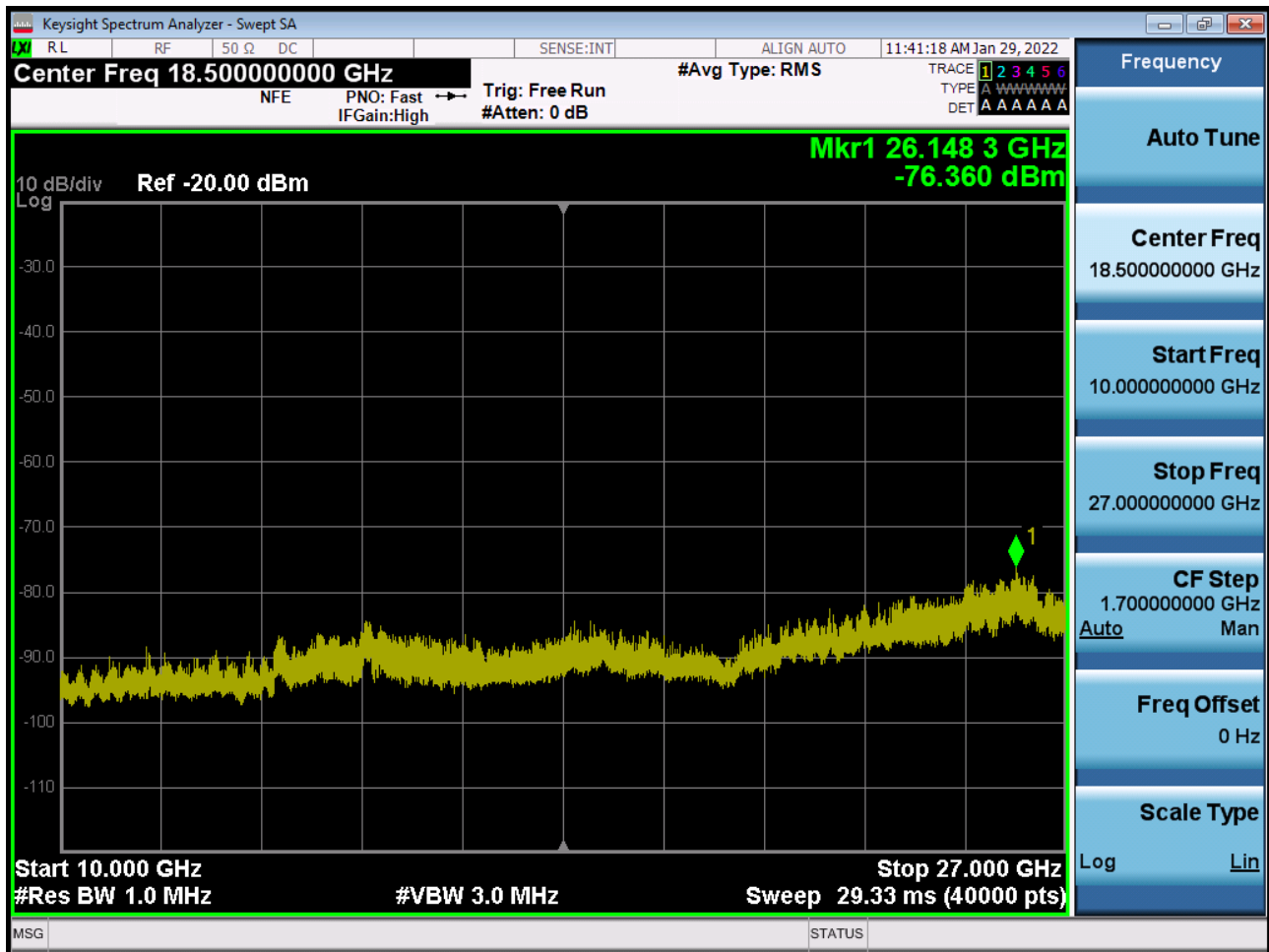
Sub6 n41. Conducted Spurious Plot 2 (60 MHz Ch.505200 BPSK RB 1)
