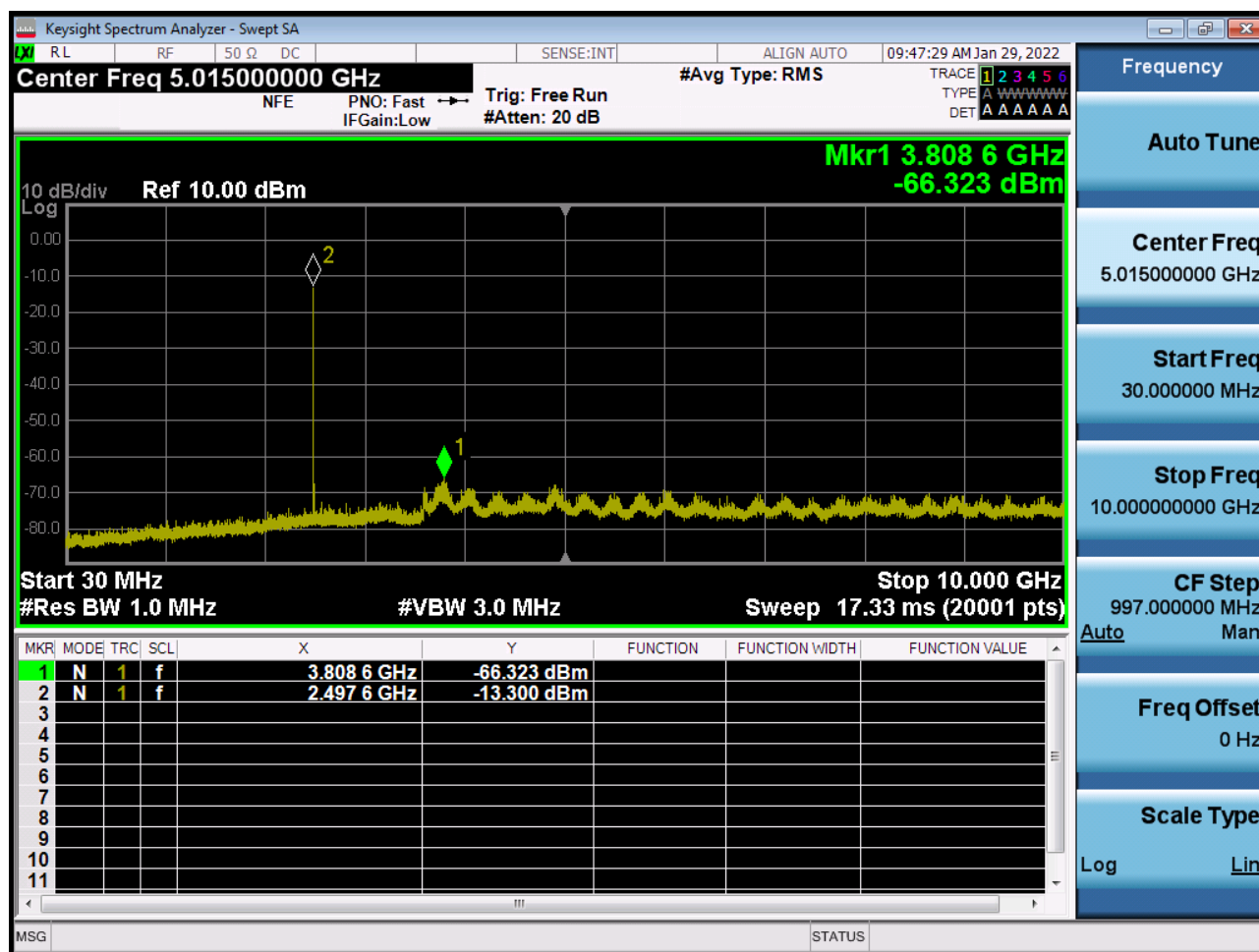
Sub6 n41. Conducted Spurious Plot 1 (30 MHz Ch.502200 BPSK RB 1)
