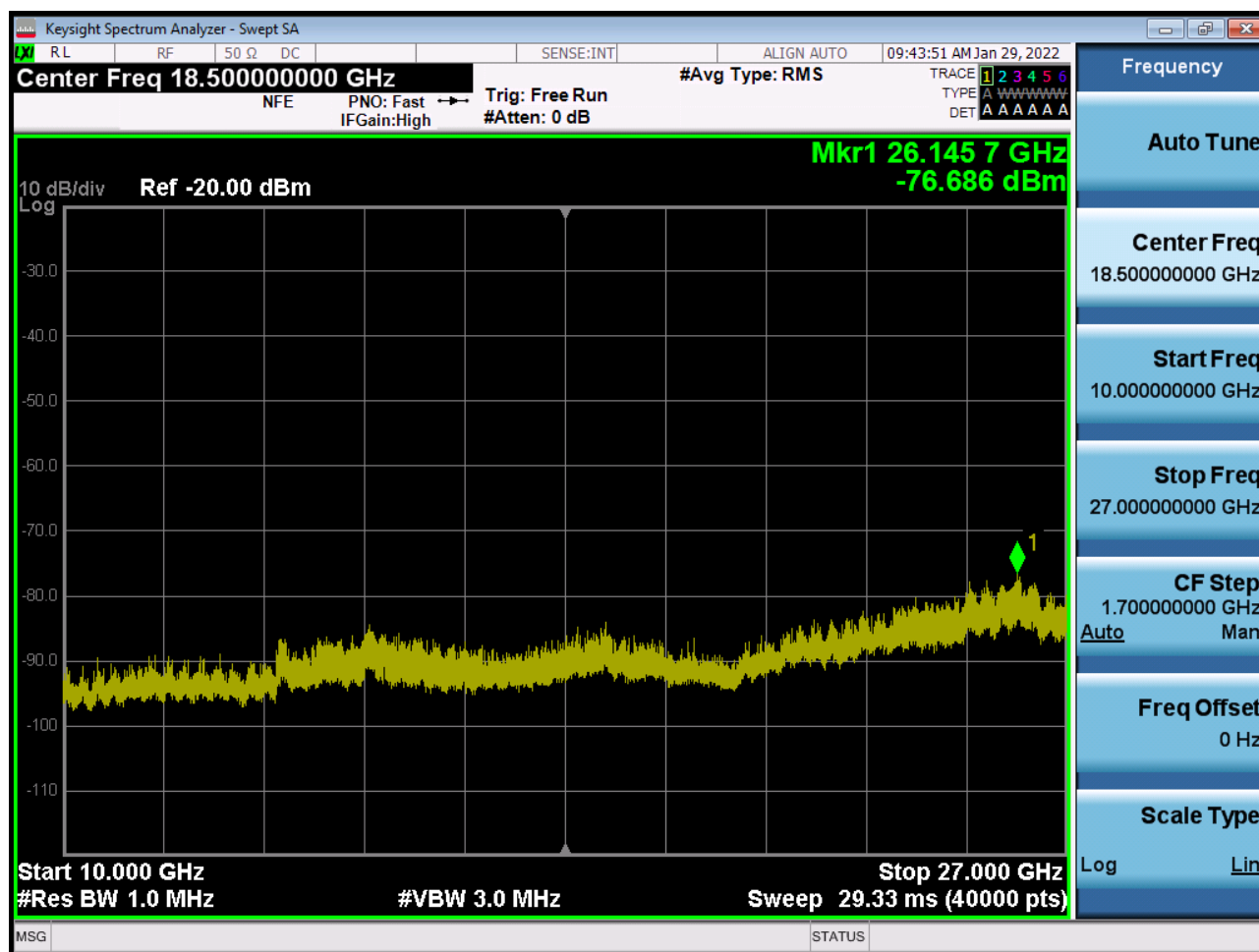
Sub6 n41. Conducted Spurious Plot 2 (20 MHz Ch.535998 BPSK RB 1)
