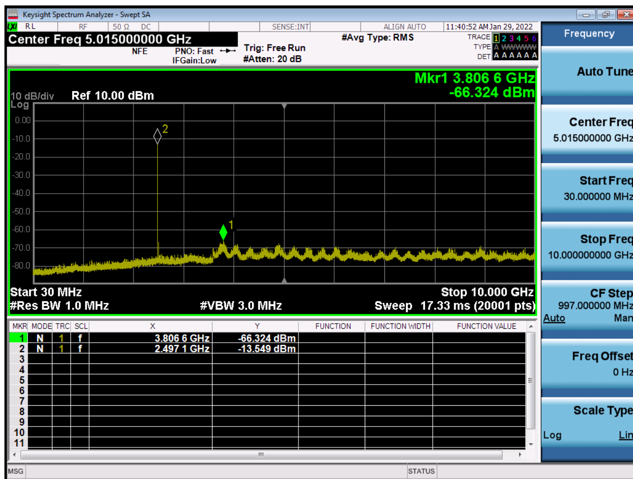
Sub6 n41. Conducted Spurious Plot 1 (60 MHz Ch.505200 BPSK RB 1)
