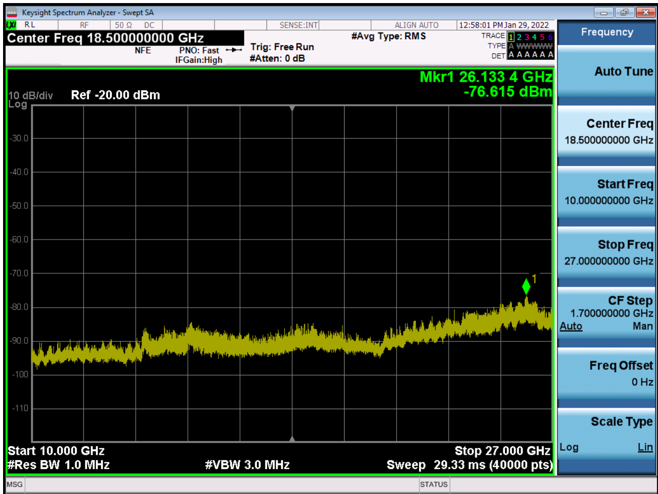
Sub6 n41. Conducted Spurious Plot 2 (90 MHz Ch. 518598 BPSK RB 1)
