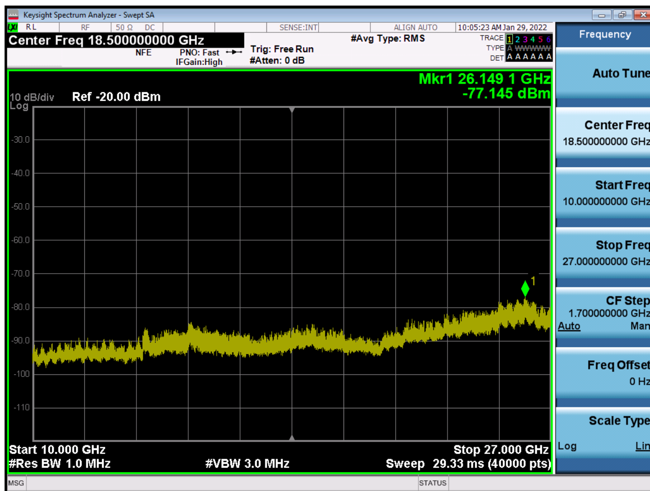
Sub6 n41. Conducted Spurious Plot 2 (40 MHz Ch.534000 BPSK RB 1)
