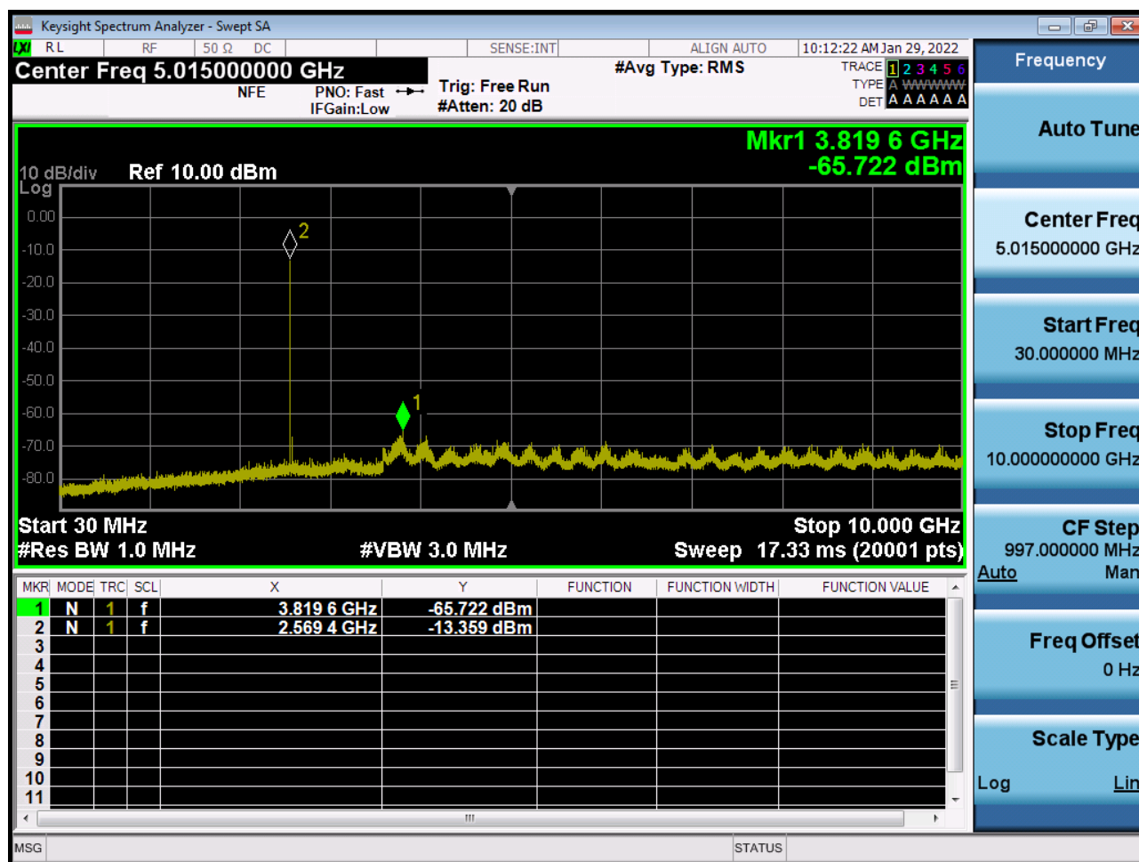
Sub6 n41. Conducted Spurious Plot 1 (50 MHz Ch.518598 BPSK RB 1)
