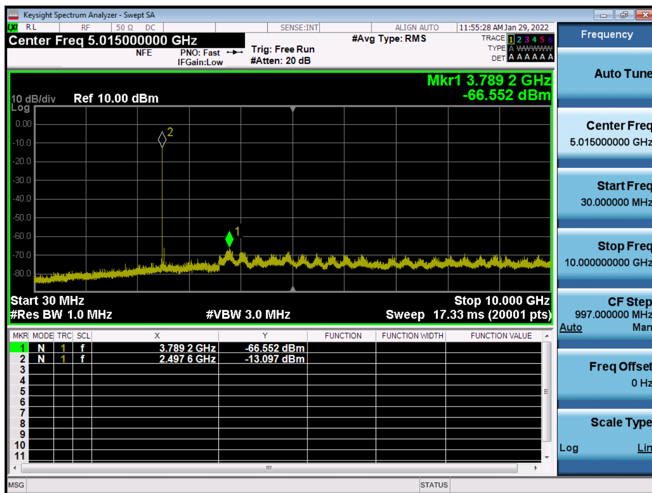
Sub6 n41. Conducted Spurious Plot 1 (80 MHz Ch.507204 BPSK RB 1)
