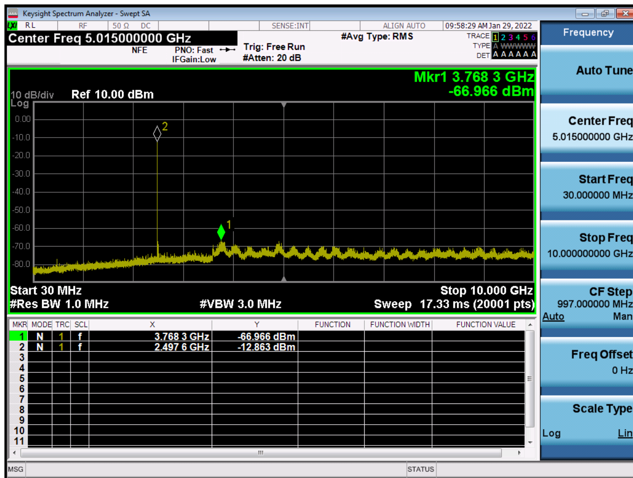
Sub6 n41. Conducted Spurious Plot 1 (40 MHz Ch.503202 BPSK RB 1)
