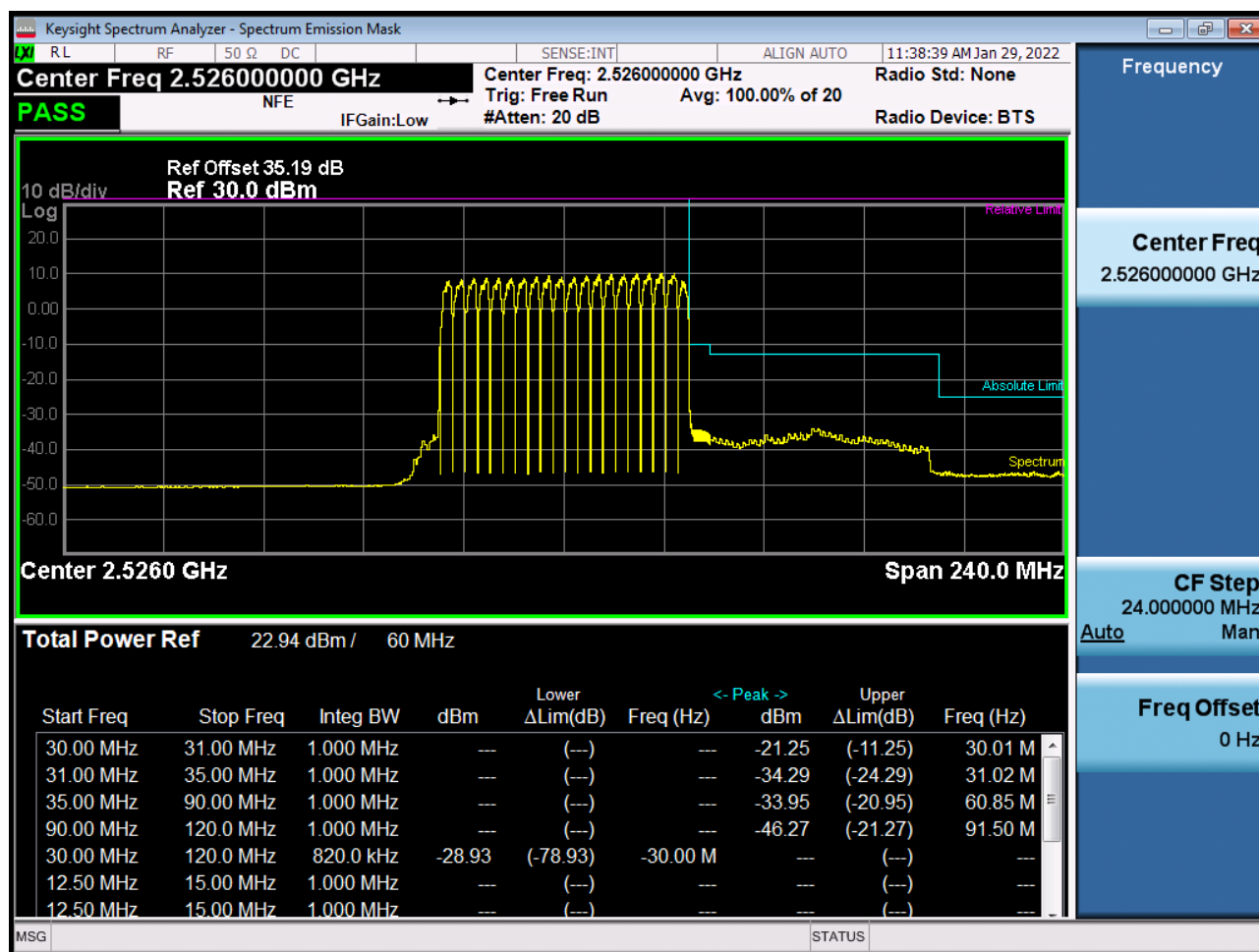
Sub6 n41. Low Channel Edge Plot (60 MHz Ch.505200 BPSK)-2
