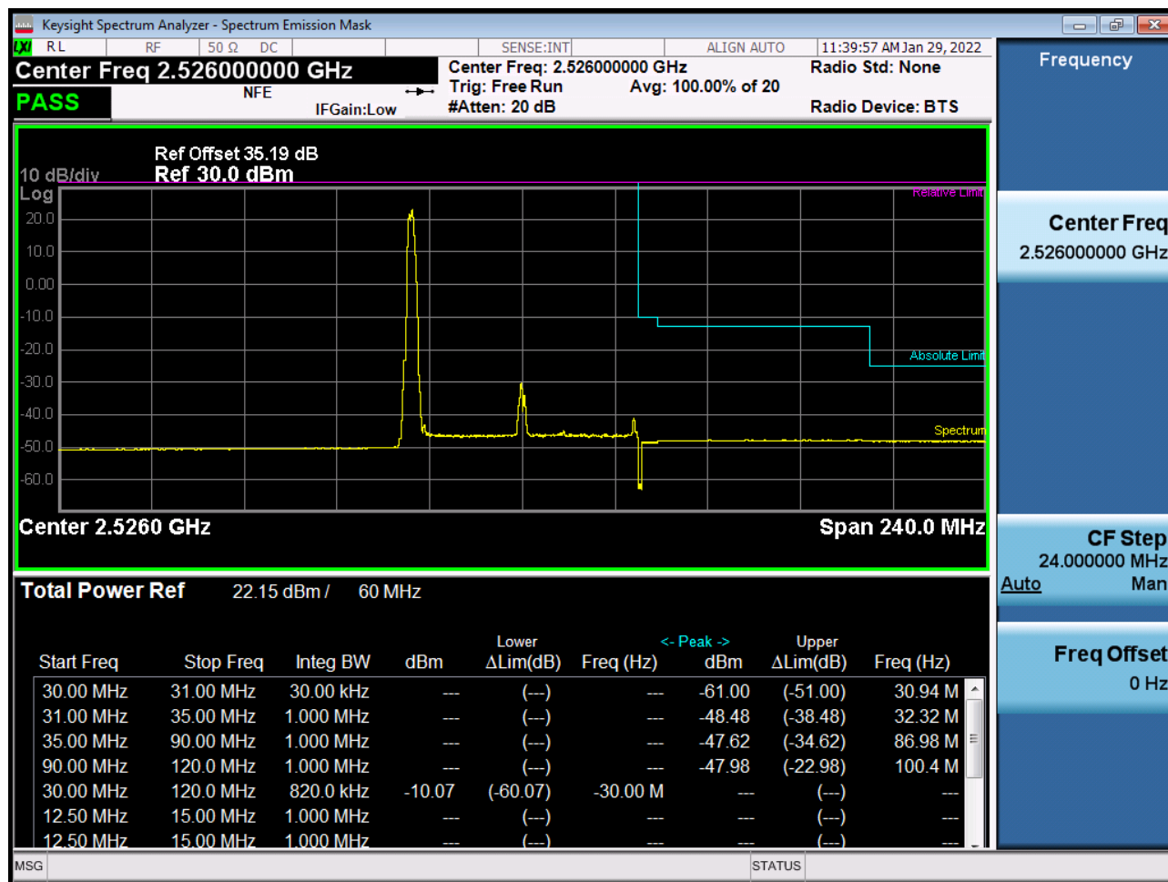
Sub6 n41. Low Channel Edge Plot (60 MHz Ch.505200 BPSK_RB1)-2
