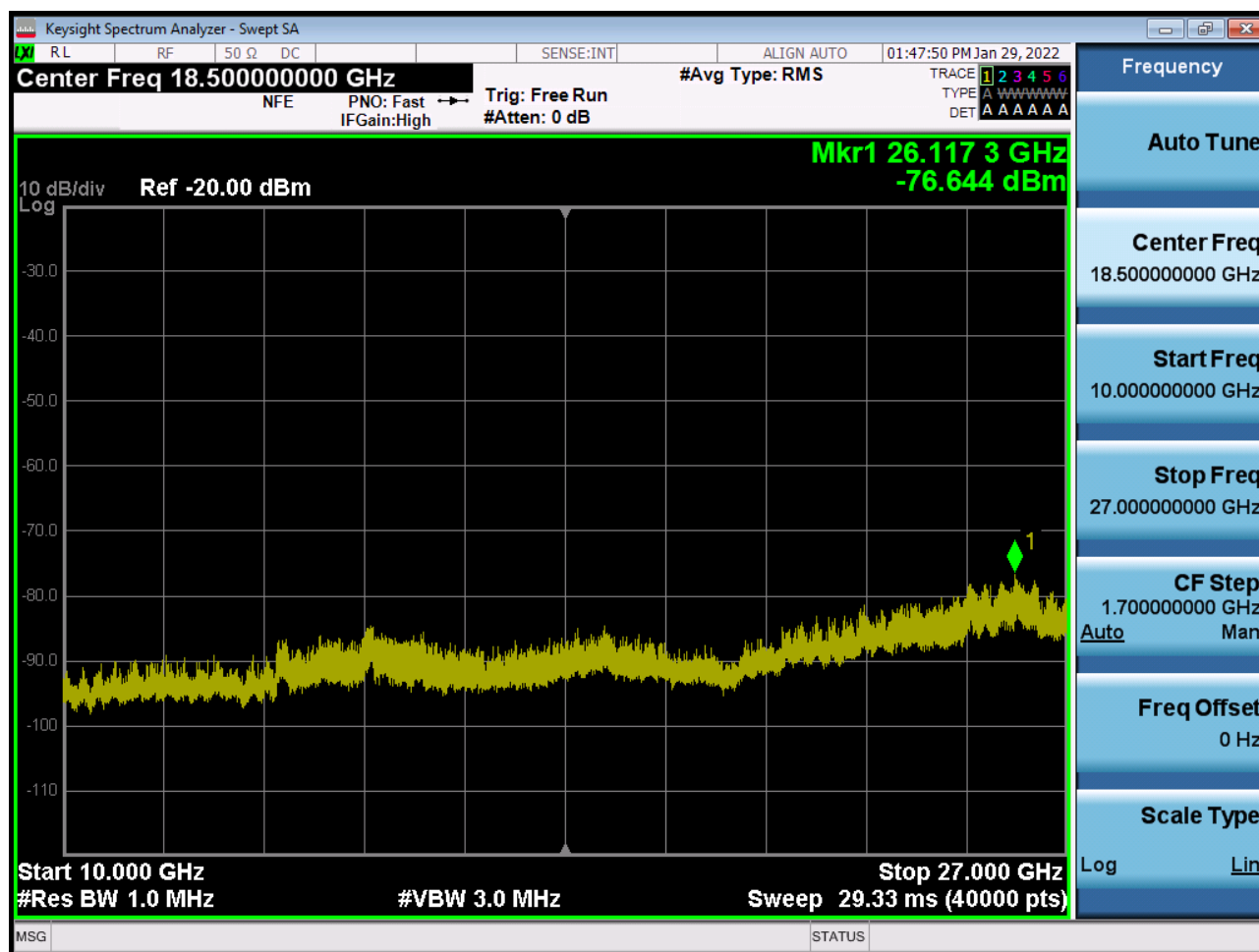
Sub6 n41. Conducted Spurious Plot 2 (80 MHz Ch.529998 BPSK RB 1)
