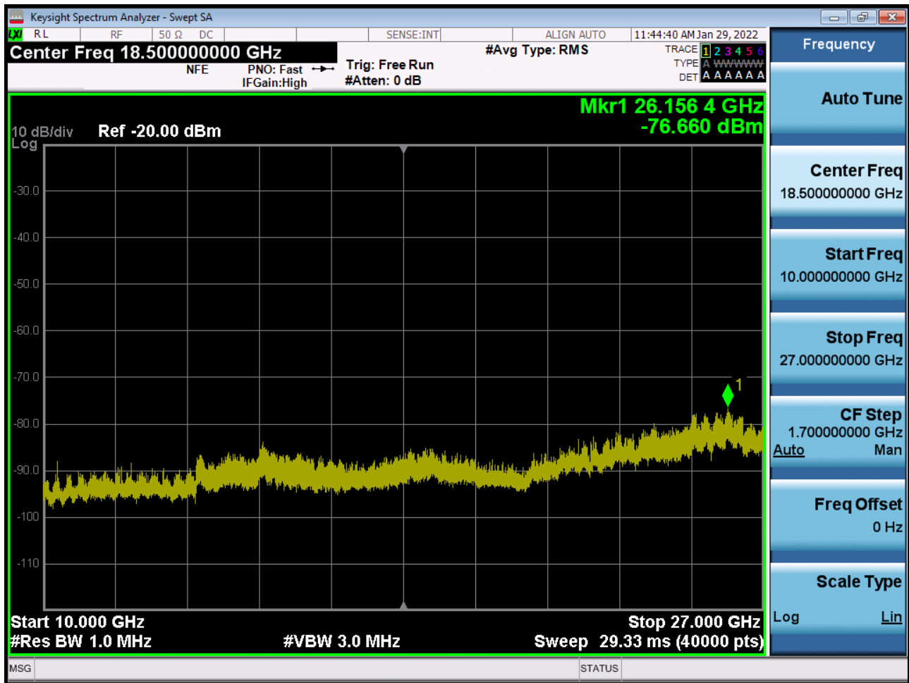
Sub6 n41. Conducted Spurious Plot 2 (60 MHz Ch. 518598 BPSK RB 1)
