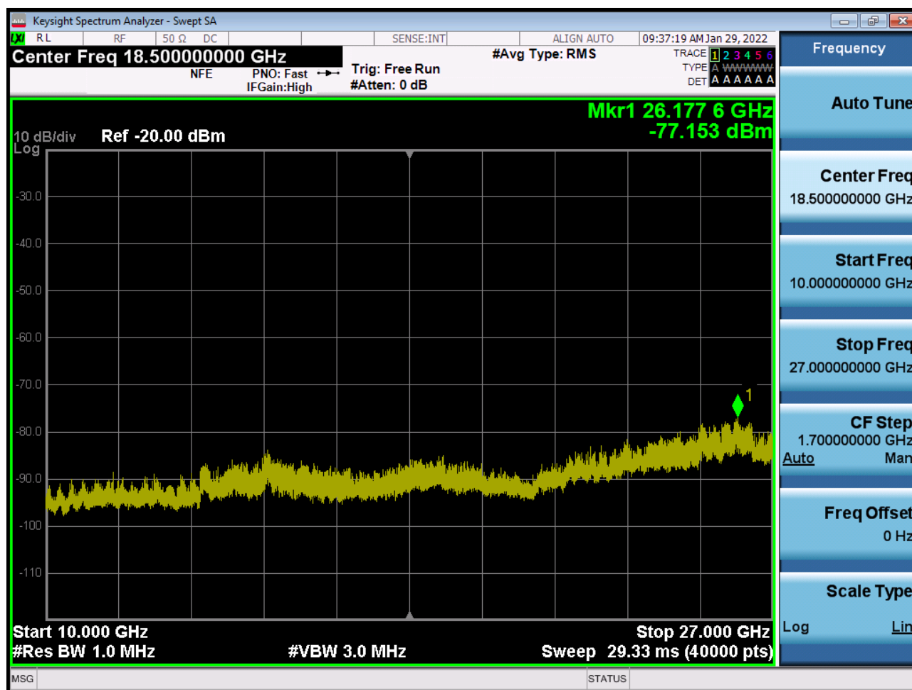
Sub6 n41. Conducted Spurious Plot 2 (20 MHz Ch.501204 BPSK RB 1)
