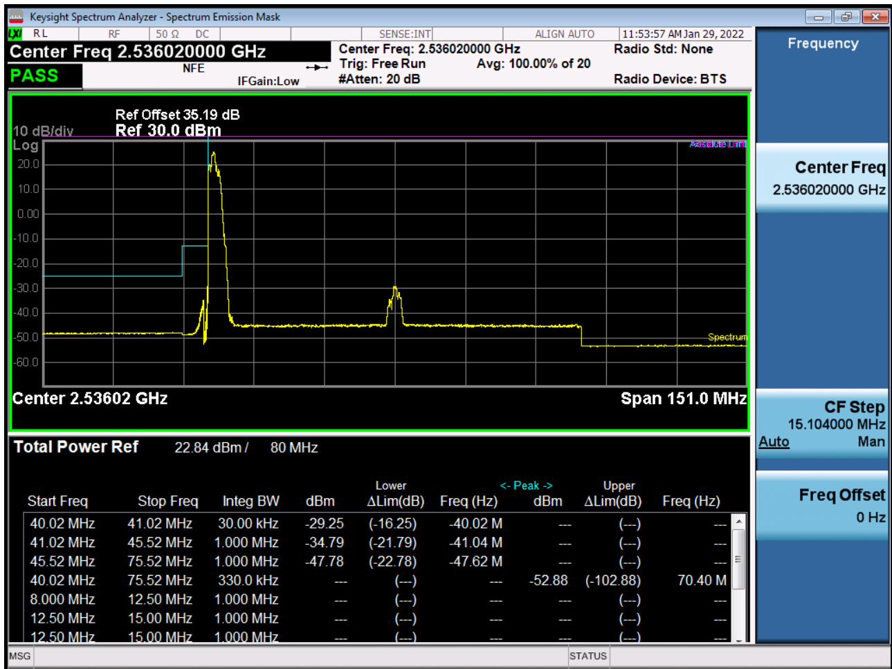
Sub6 n41. Low Channel Edge Plot (80 MHz Ch.507204 BPSK RB 1)-1
