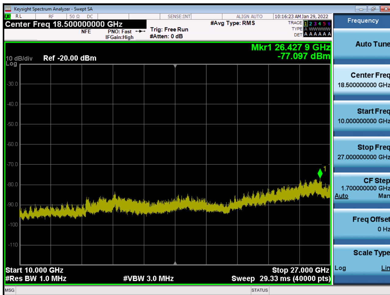
Sub6 n41. Conducted Spurious Plot 2 (50 MHz Ch.532998 BPSK RB 1)
