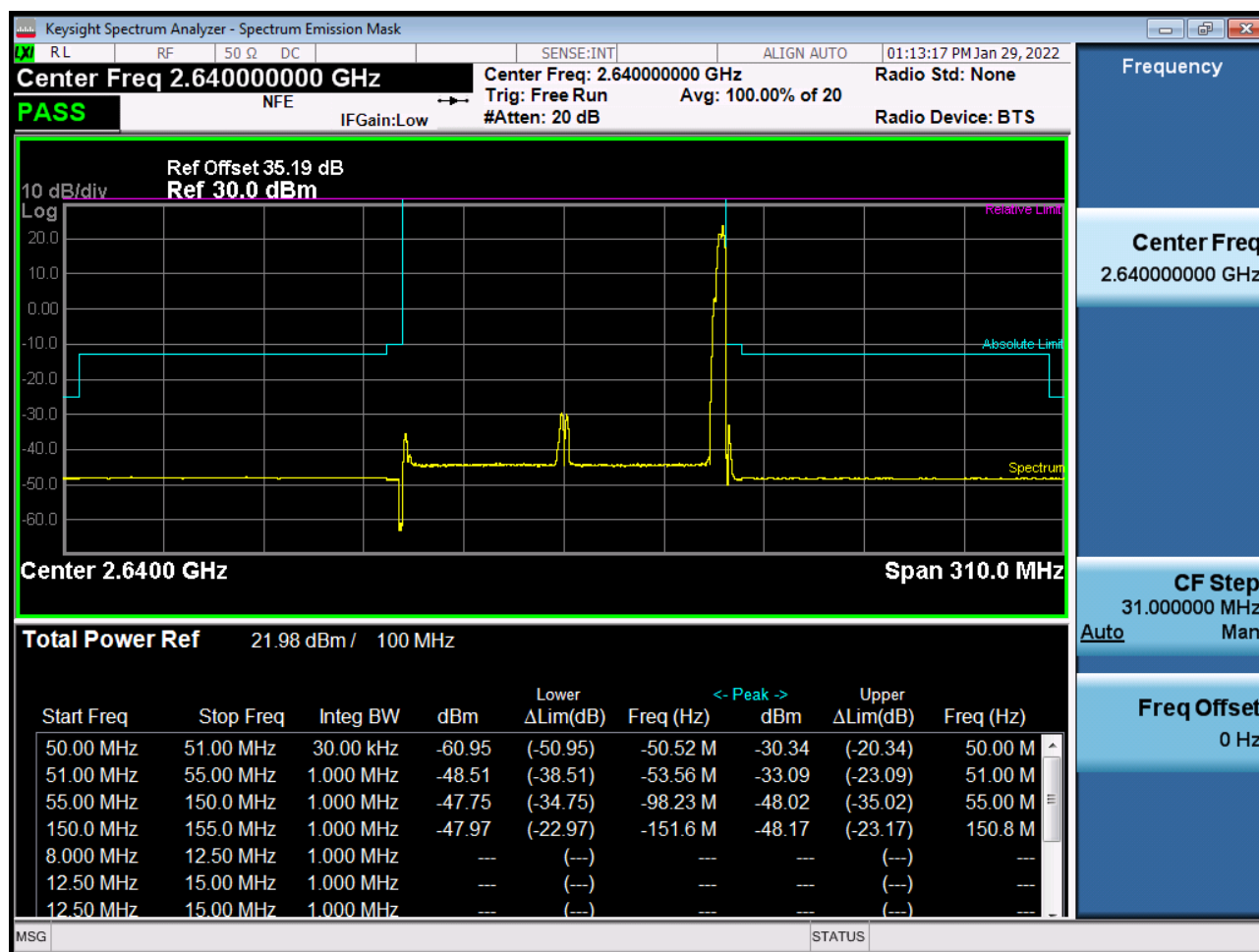
Sub6 n41. High Channel Edge Plot (100 MHz Ch.528000 BPSK RB 1)
