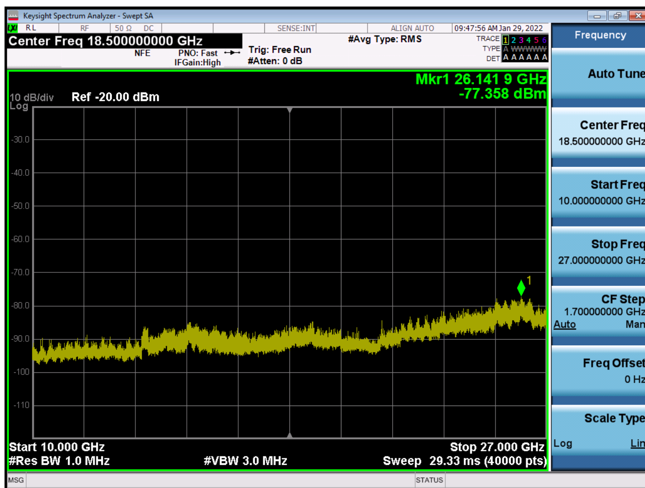
Sub6 n41. Conducted Spurious Plot 2 (30 MHz Ch.502200 BPSK RB 1)
