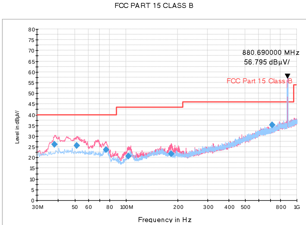
Figure 1: [EUT+TA] LTE B5+5G NR n5 Middle ch Idle
