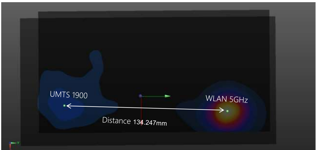
Plot #2 UMTS 1900+ WLAN 5GHz (Hotspot Mode)
