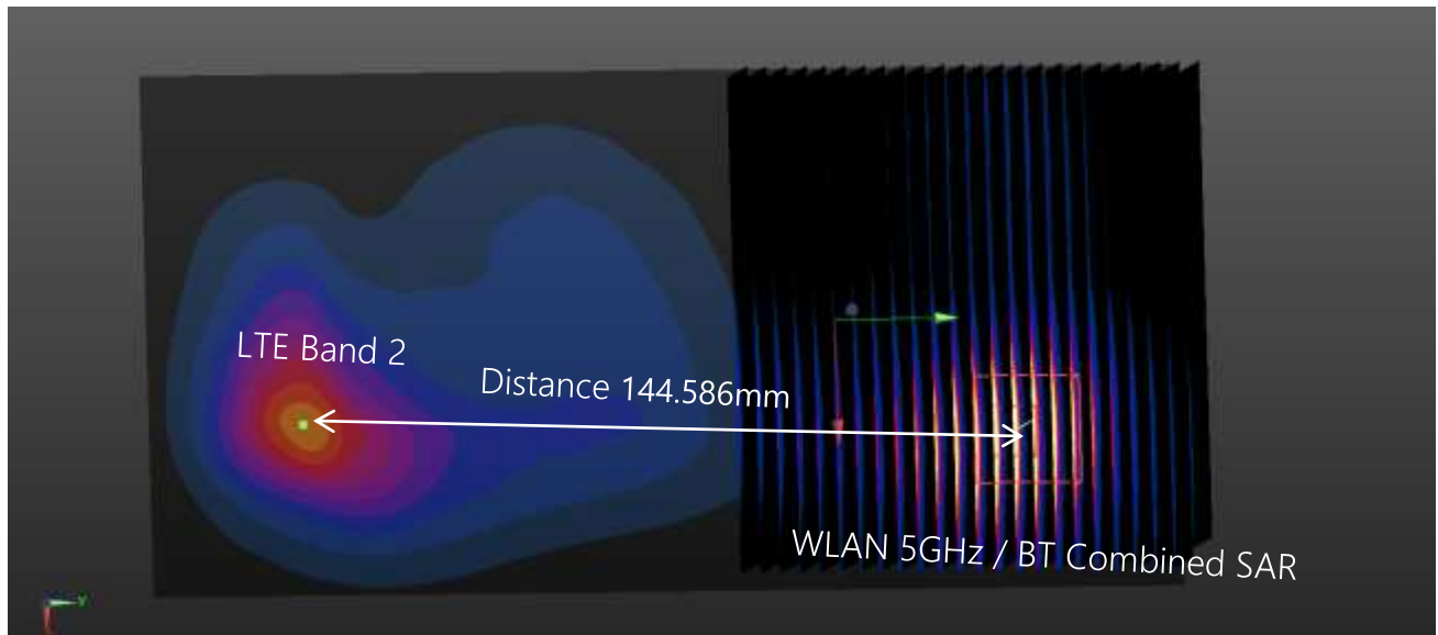
Plot #13 LTE Band 2 + WLAN 5GHz / Bluetooth Combined SAR (Hotspot Mode)
