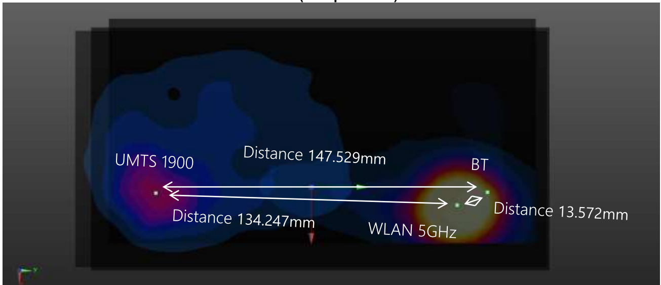
Plot #6 UMTS 1900 + WLAN 5GHz + Bluetooth (Hotspot Mode)
