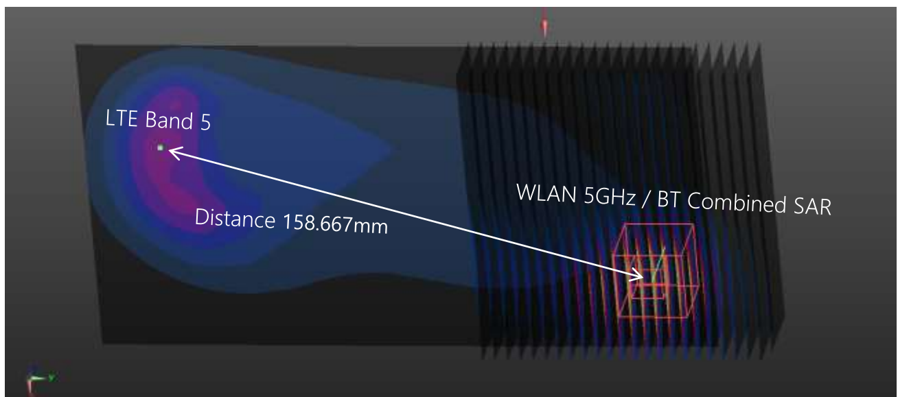
Plot #14 LTE Band 5 + WLAN 5GHz / Bluetooth Combined SAR (Hotspot Mode)
