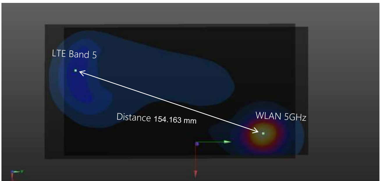
Plot #4 LTE Band 5 + WLAN 5GHz (Hotspot Mode)
