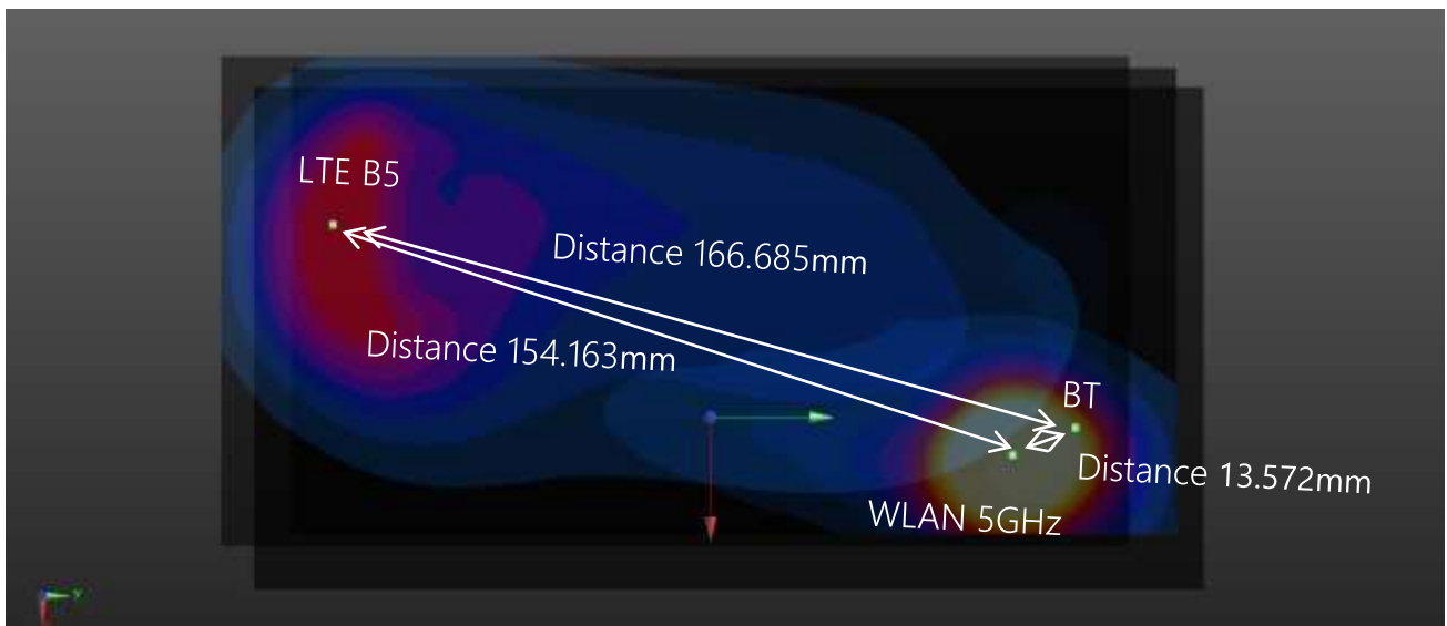
Plot #8 LTE Band 5 + WLAN 5GHz + Bluetooth (Hotspot Mode)
