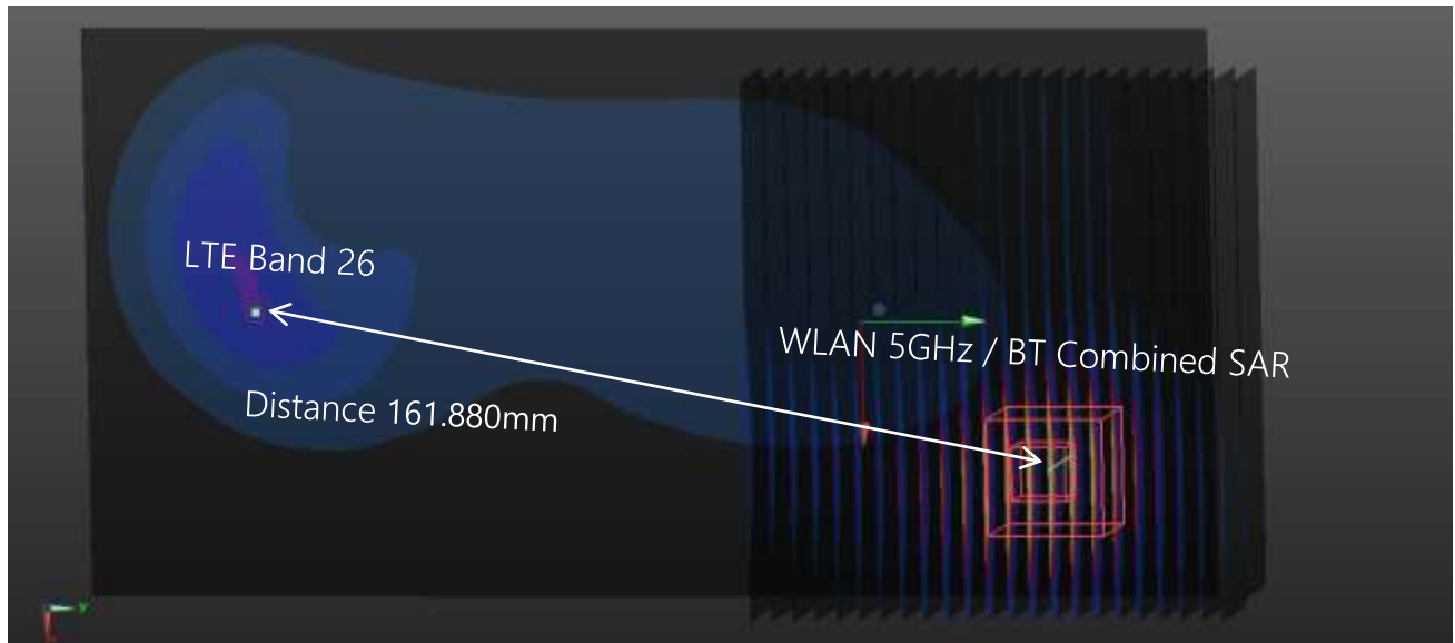
Plot #15 LTE Band 26 + WLAN 5GHz / Bluetooth Combined SAR (Hotspot Mode)
