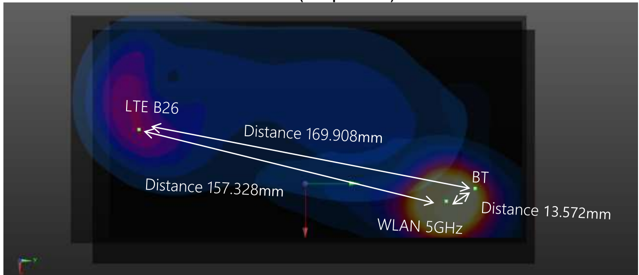
Plot #9 LTE Band 26 + WLAN 5GHz + Bluetooth (Hotspot Mode)
