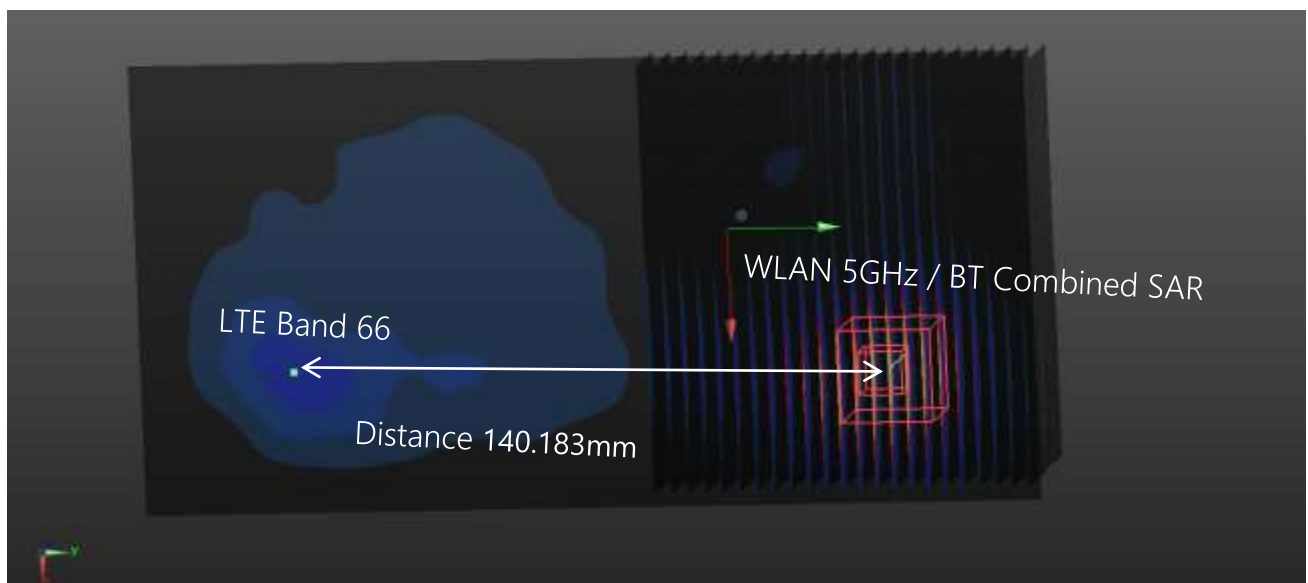
Plot #16 LTE Band 66 + WLAN 5GHz / Bluetooth Combined SAR (Hotspot Mode)
