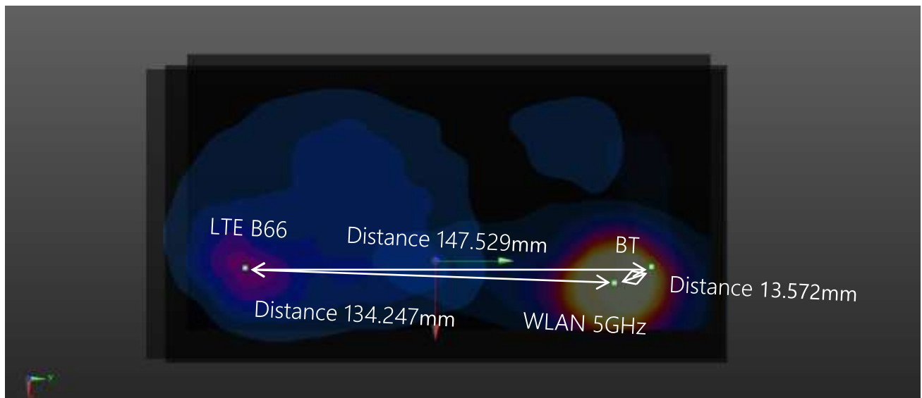
Plot #10 LTE Band 66 + WLAN 5GHz + Bluetooth (Hotspot Mode)
