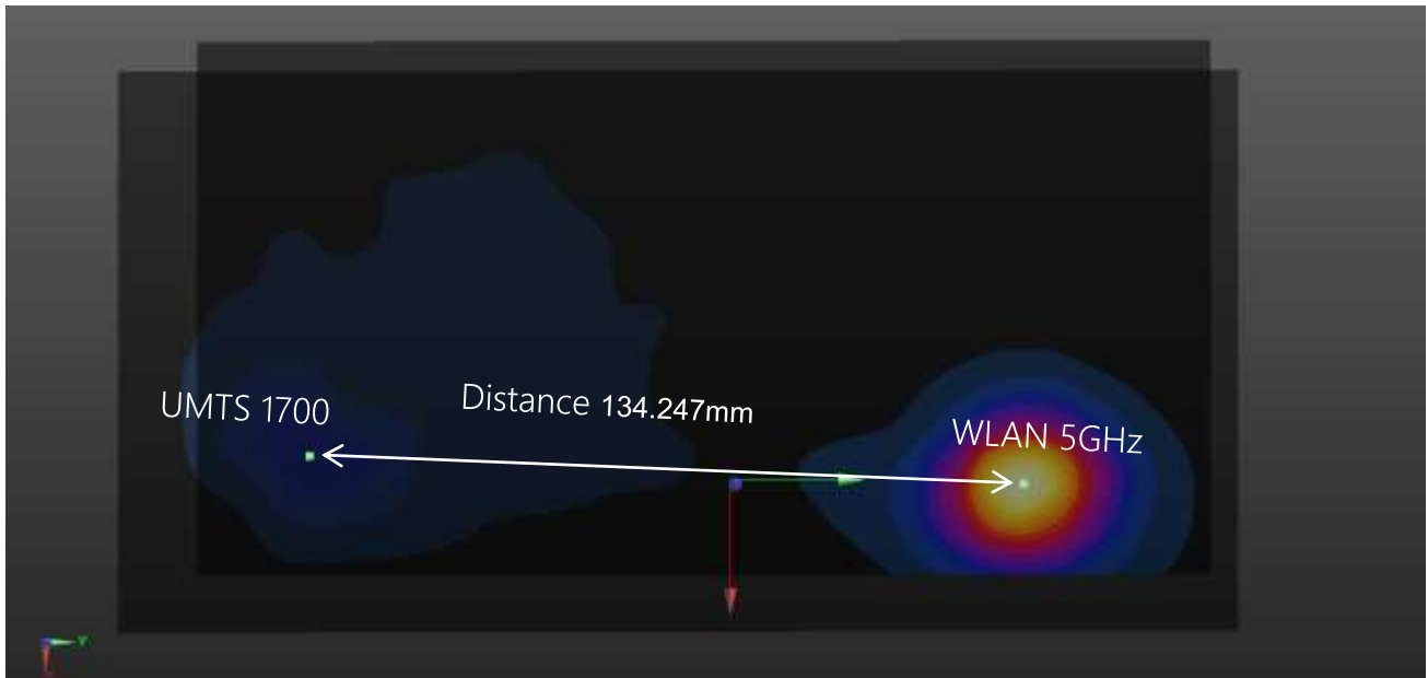
Plot #1 UMTS 1700+ WLAN 5GHz (Hotspot Mode)
