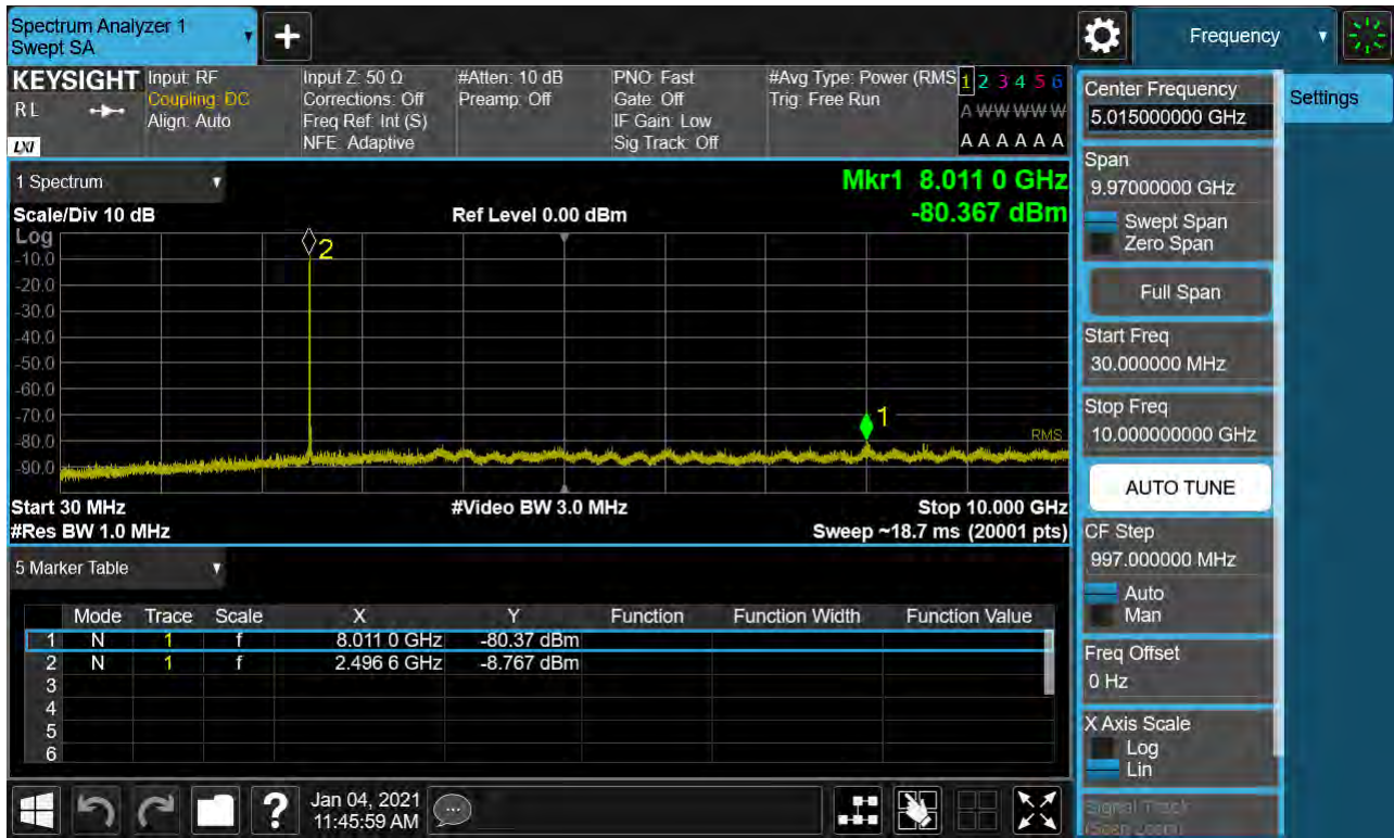
BAND 41. Conducted Spurious Plot 1 (10 MHz Ch.39700 QPSK RB 1, Offset 0)
