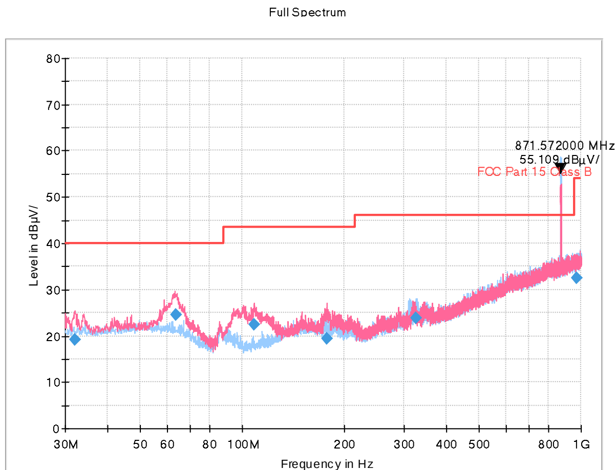
Figure 1: Radiated Emission (30 to 1 000) MHz, [EUT+TA] LTE B5+5G NR n5 Low ch Idle
