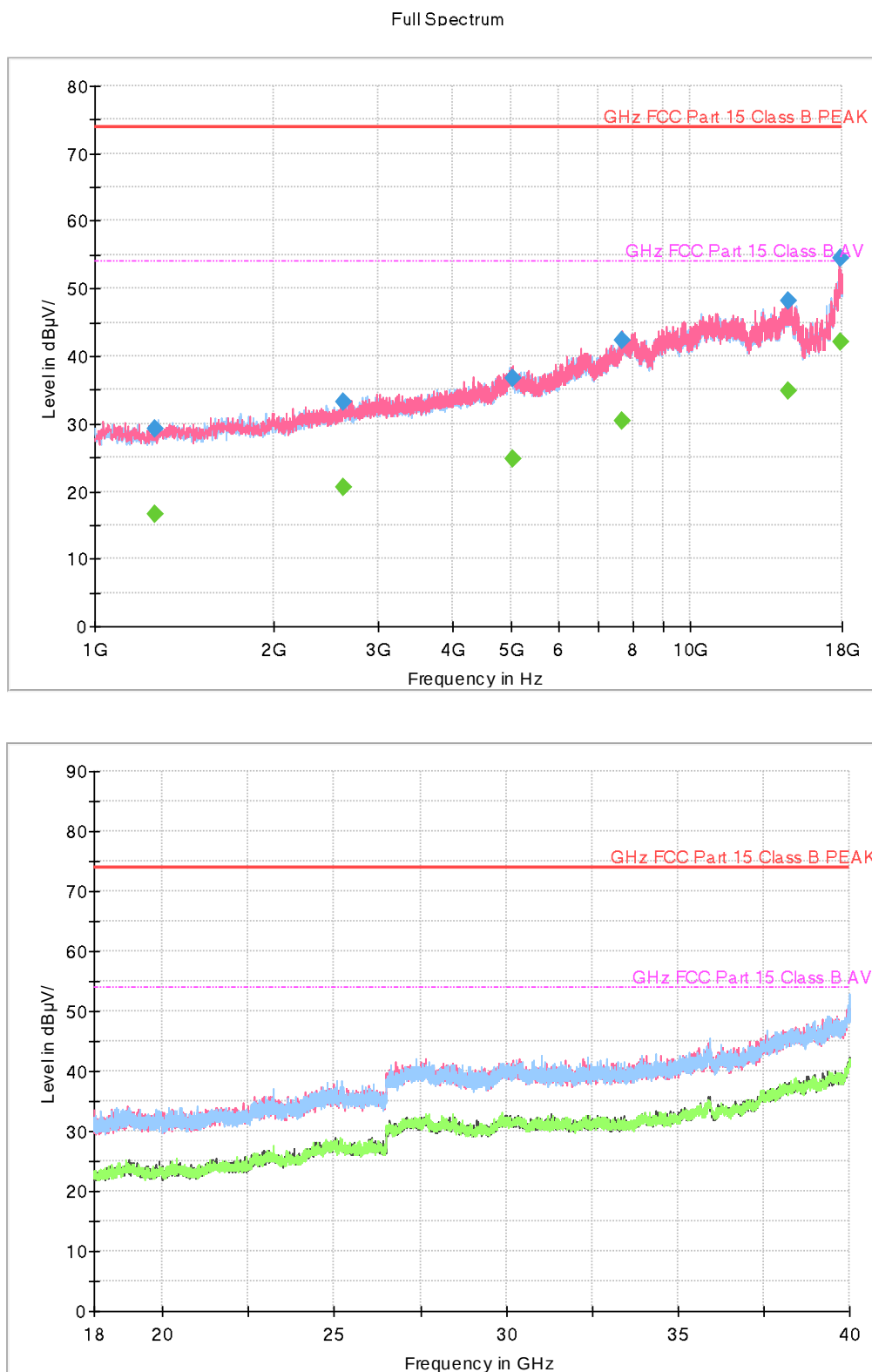
Figure 6: Radiated Emission (1 to 40) GHz, [EUT+Earphone] LTE B5+5G NR n5 Low ch Idle
