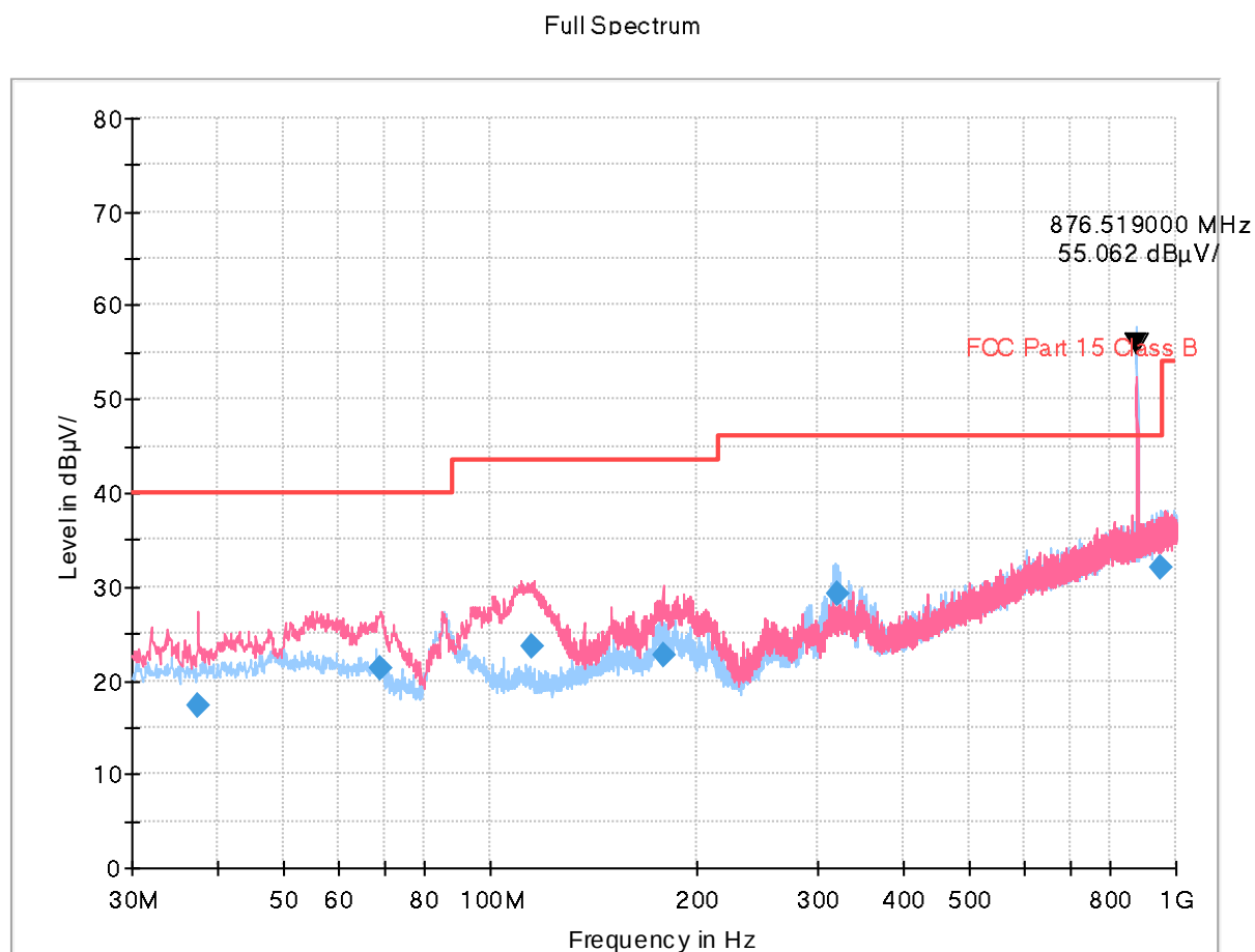
Figure 3: Radiated Emission (30 to 1 000) MHz, [EUT+TA] LTE B26 Middle ch Idle
