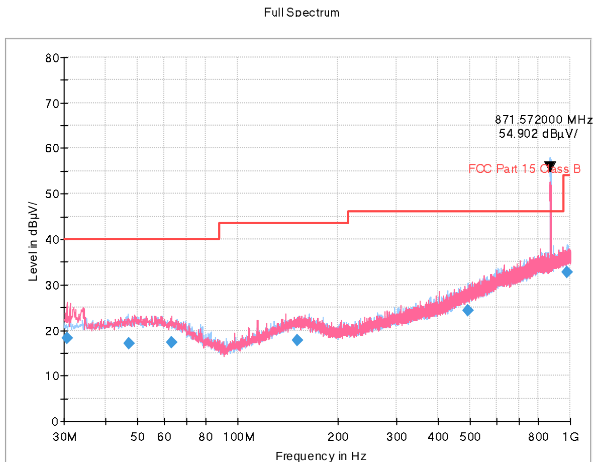
Figure 4: Radiated Emission (30 to 1 000) MHz, [EUT+Earphone] LTE B5+5G NR n5 Low ch Idle
