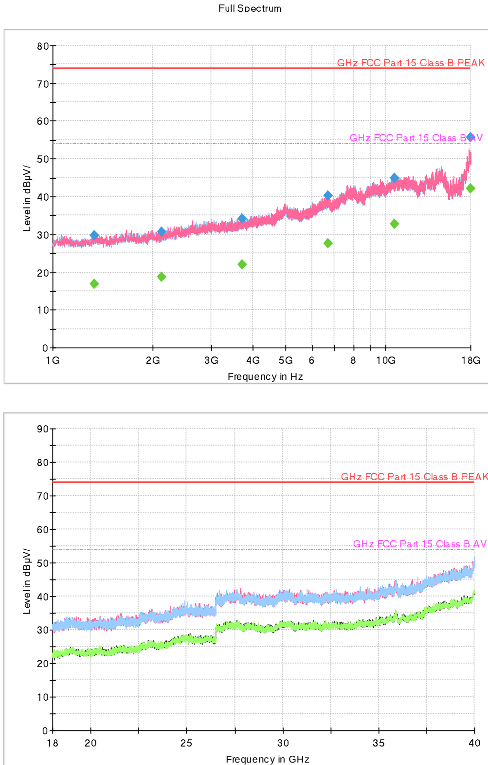
Figure 5: Radiated Emission (1 to 40) GHz, [EUT+TA] LTE B5+5G NR n5 Low ch Idle
