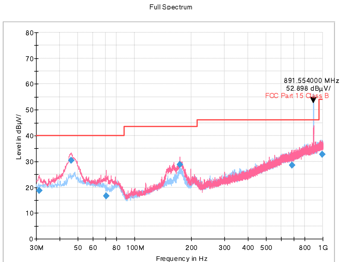
Figure 3: Radiated Emission (30 to 1 000) MHz, [EUT+TA] LTE B26 High ch Idle
