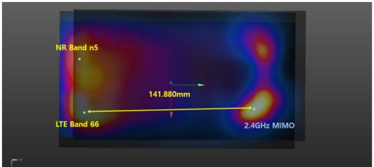
Plot #12 NR Band n5+ LTE Band 66+ 2.4 GHz WLAN MIMO
