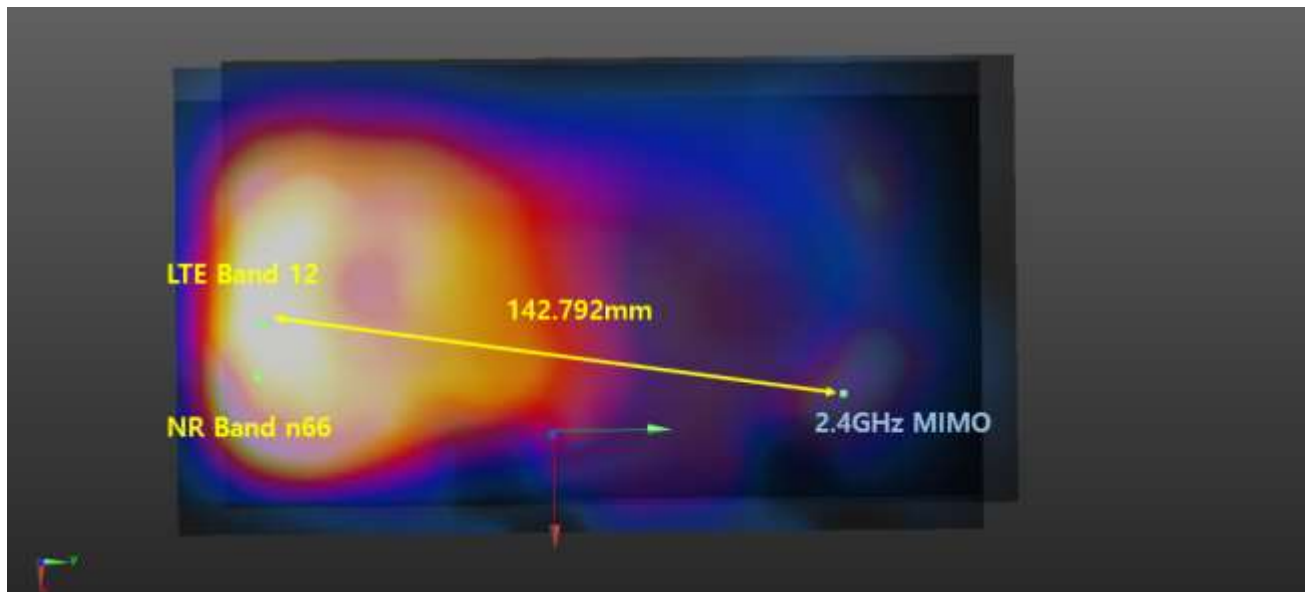
Plot #8 NR Band n66+ LTE Band 12+ 2.4 GHz WLAN MIMO
