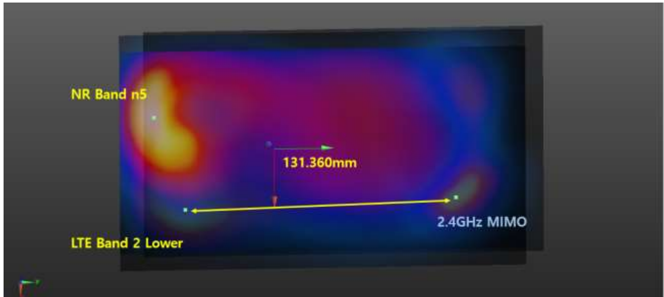
Plot #11 NR Band n5+ LTE Band 2 Lower+ 2.4 GHz WLAN MIMO
