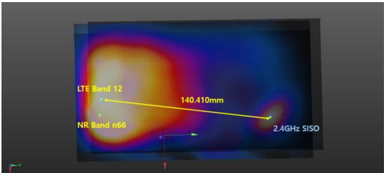
Plot #2 NR Band n66+ LTE Band 12+ 2.4 GHz WLAN SISO
