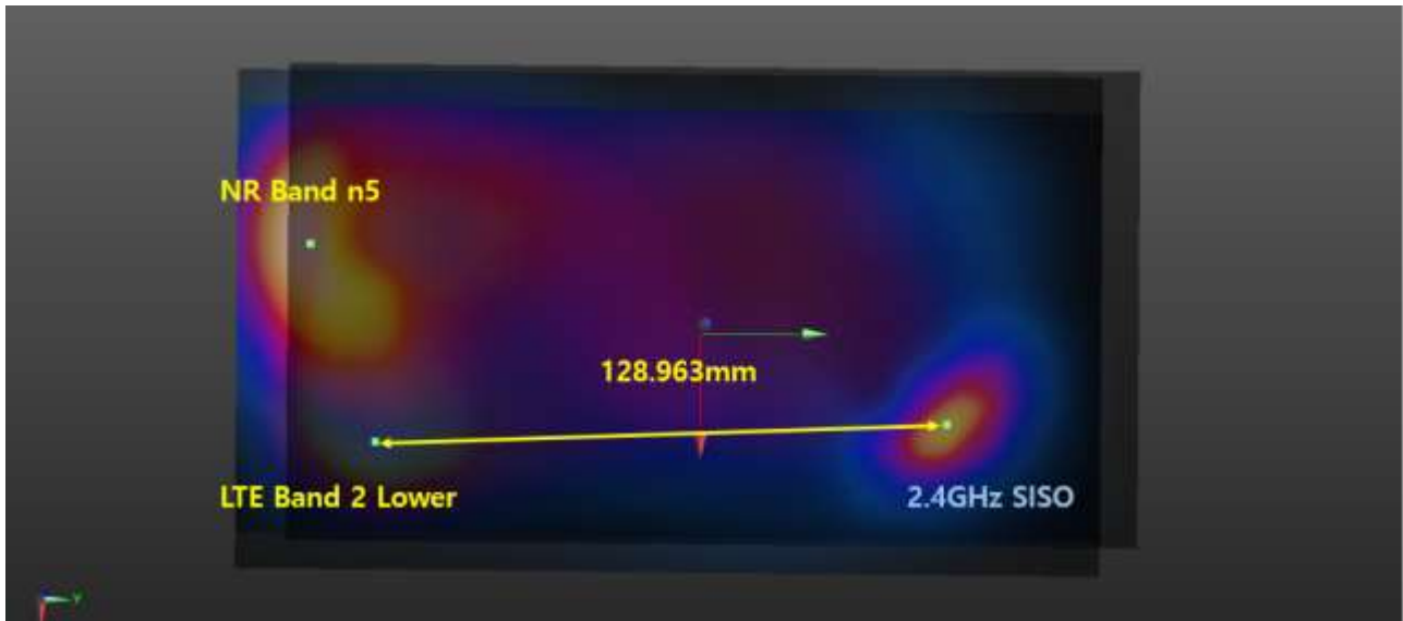
Plot #5 NR Band n5+ LTE Band 2 Lower+ 2.4 GHz WLAN SISO
