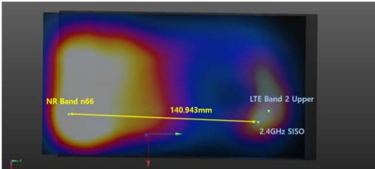
Plot #1 NR Band n66+ LTE Band 2 Sub Ant2 + 2.4 GHz WLAN SISO
