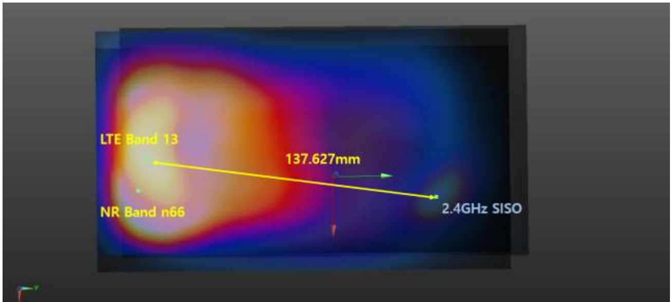
Plot #3 NR Band n66+ LTE Band 13+ 2.4 GHz WLAN SISO
