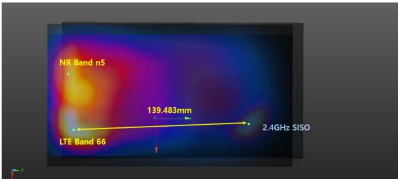
Plot #6 NR Band n5+ LTE Band 66+ 2.4 GHz WLAN SISO
