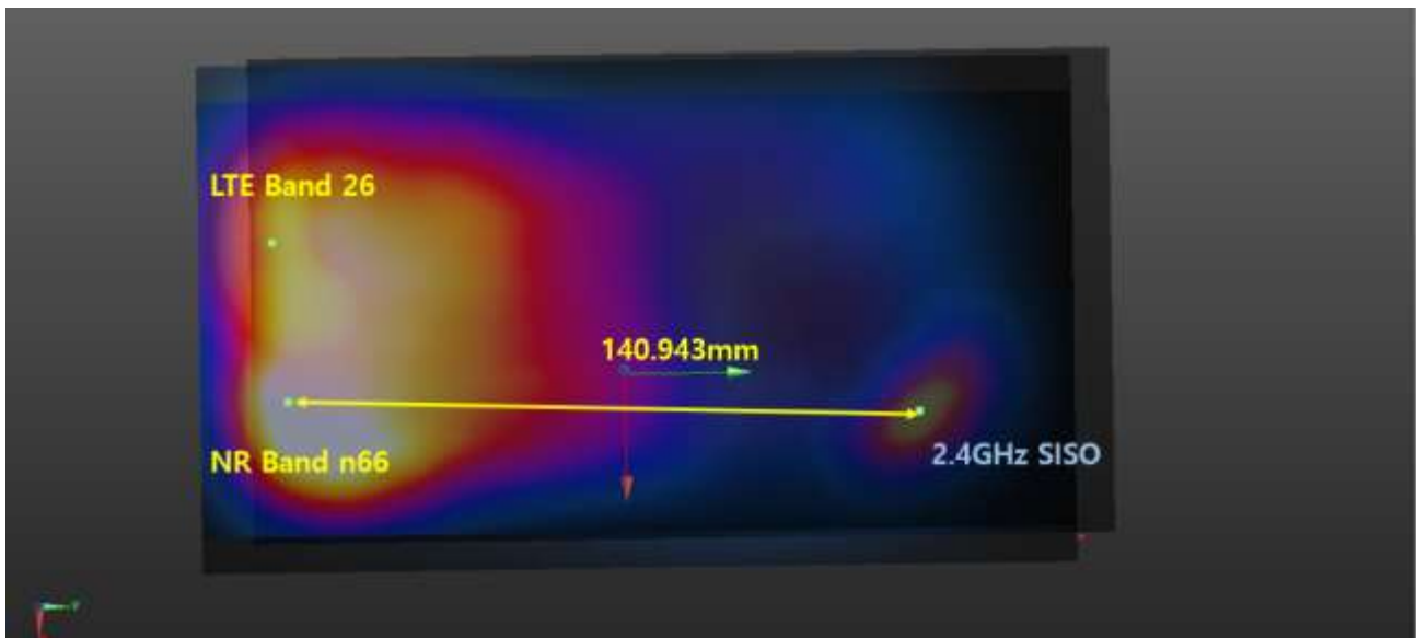
Plot #4 NR Band n66+ LTE Band 26+ 2.4 GHz WLAN SISO
