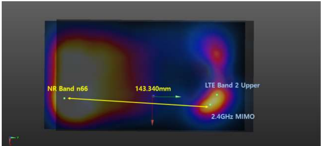
Plot #7 NR Band n66+ LTE Band 2 Sub Ant2 + 2.4 GHz WLAN MIMO
