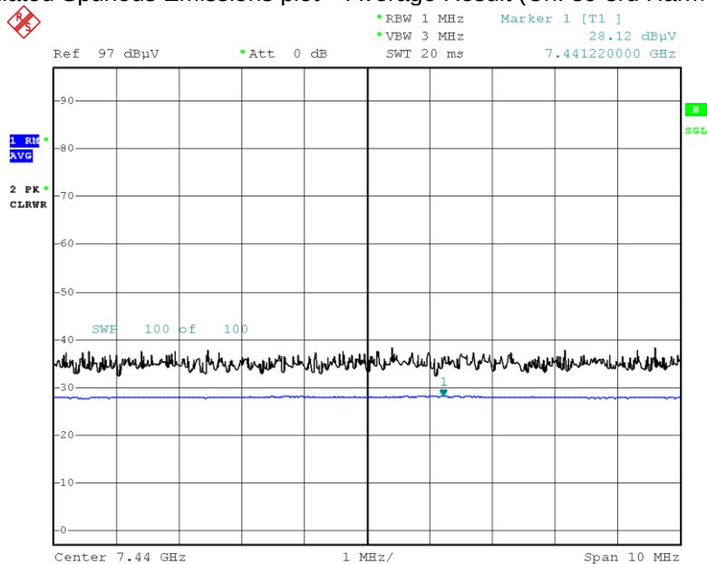
Radiated Spurious Emissions plot – Average Result (Ch. 39 3rd Harmonic)
