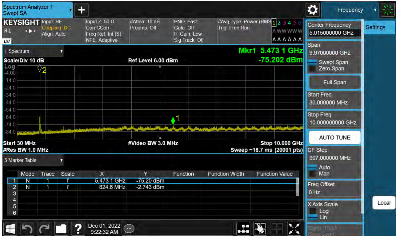
Sub6 n5. Conducted Spurious Plot (165300ch_5 MHz_BPSK_RB 1_1)
