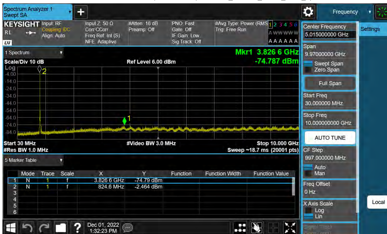
Sub6 n5. Conducted Spurious Plot (166300ch_15 MHz_BPSK_RB 1_1)
