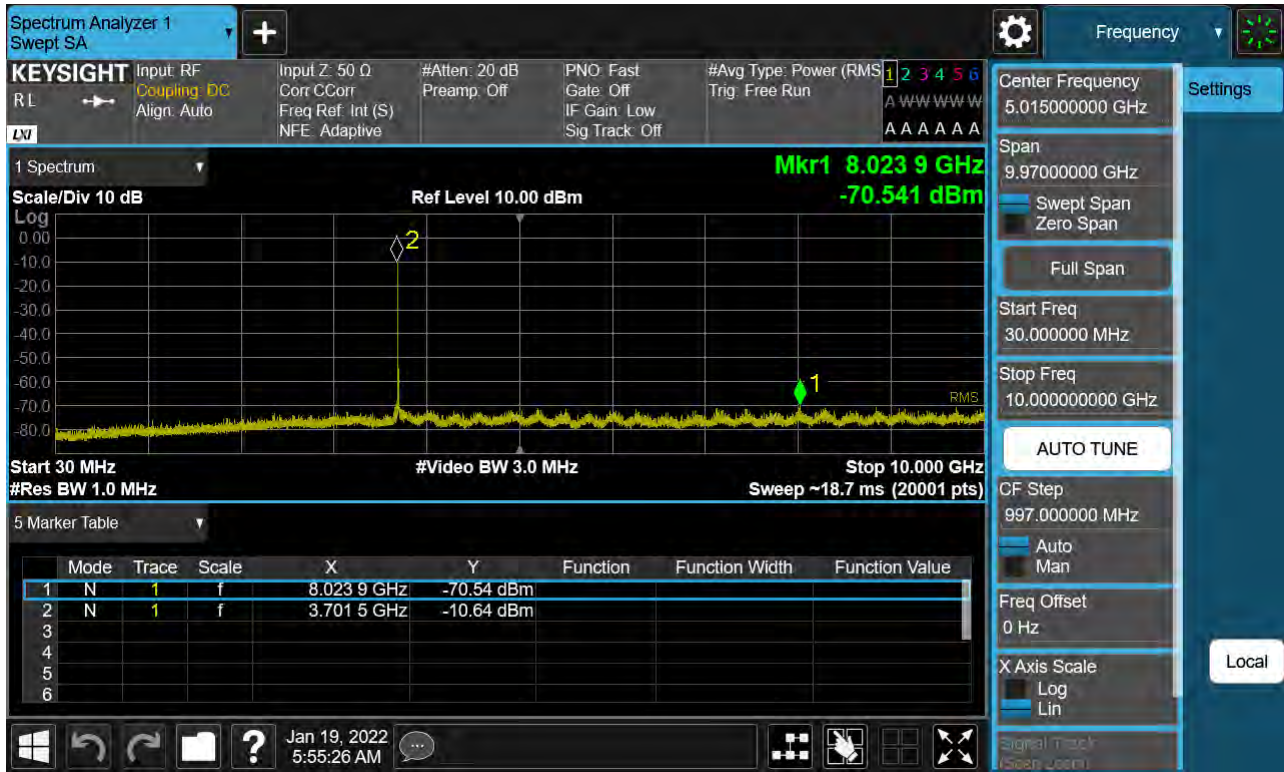
Sub6 n77. Conducted Spurious Plot_1 (647334ch_20 MHz_BPSK)
