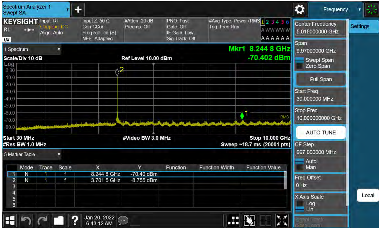
Sub6 n77. Conducted Spurious Plot_1 (647500ch_25 MHz_BPSK)
