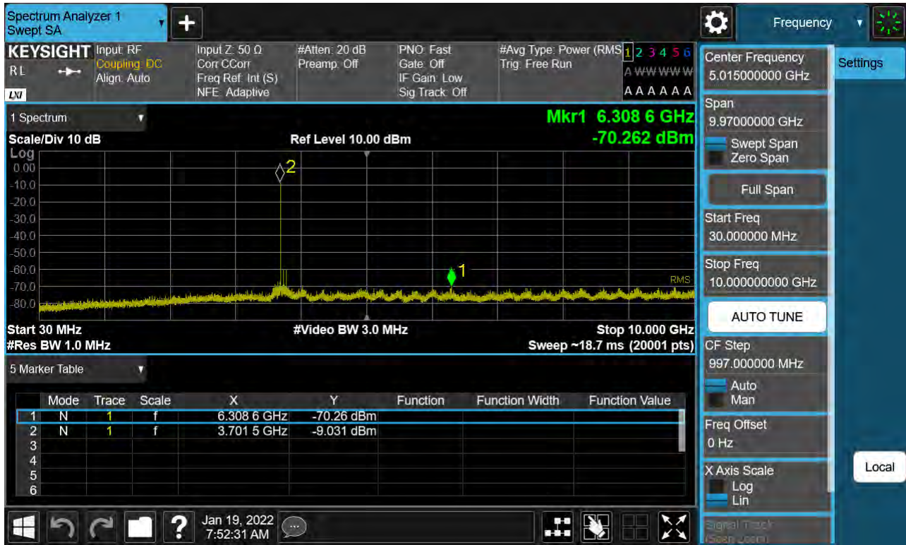
Sub6 n77. Conducted Spurious Plot_1 (649668ch_90 MHz_BPSK)
