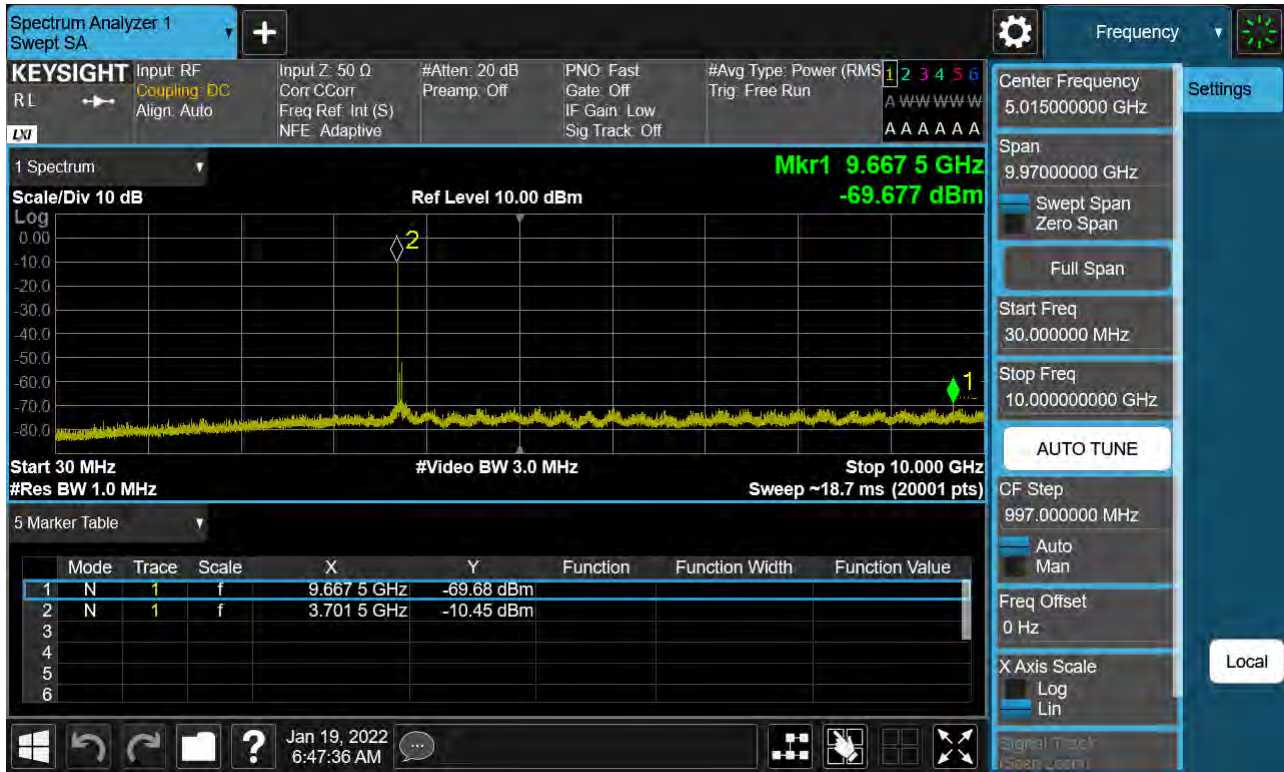
Sub6 n77. Conducted Spurious Plot_1 (648334ch_50 MHz_BPSK)
