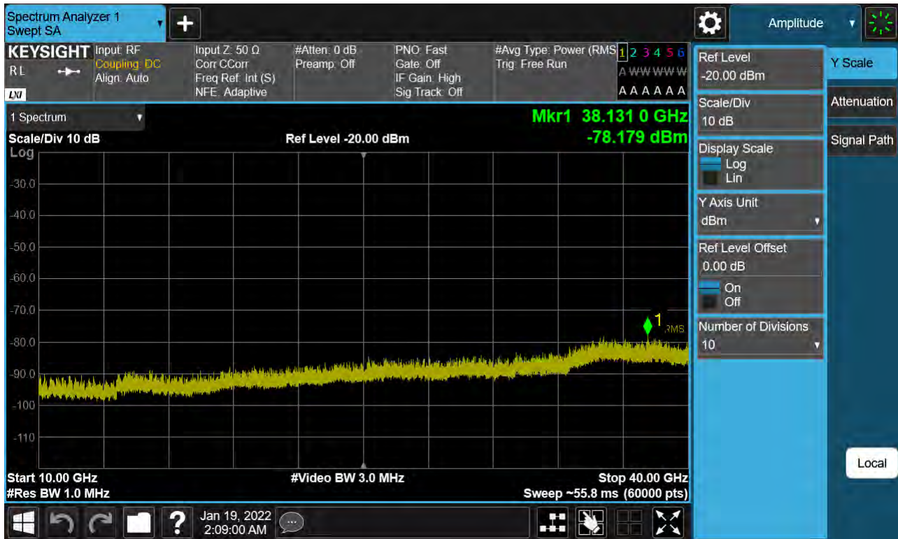
Sub6 n77. Conducted Spurious Plot_2 (636166ch_15 MHz_BPSK)
