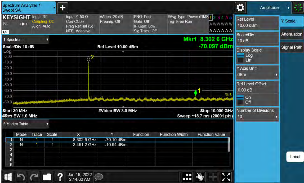
Sub6 n77. Conducted Spurious Plot_1 (630668ch_20 MHz_BPSK)
