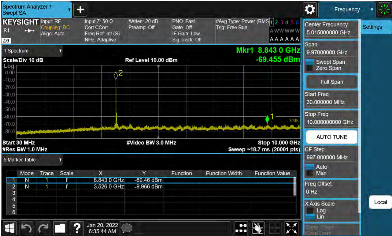
Sub6 n77. Conducted Spurious Plot_1 (635834ch_25 MHz_BPSK)
