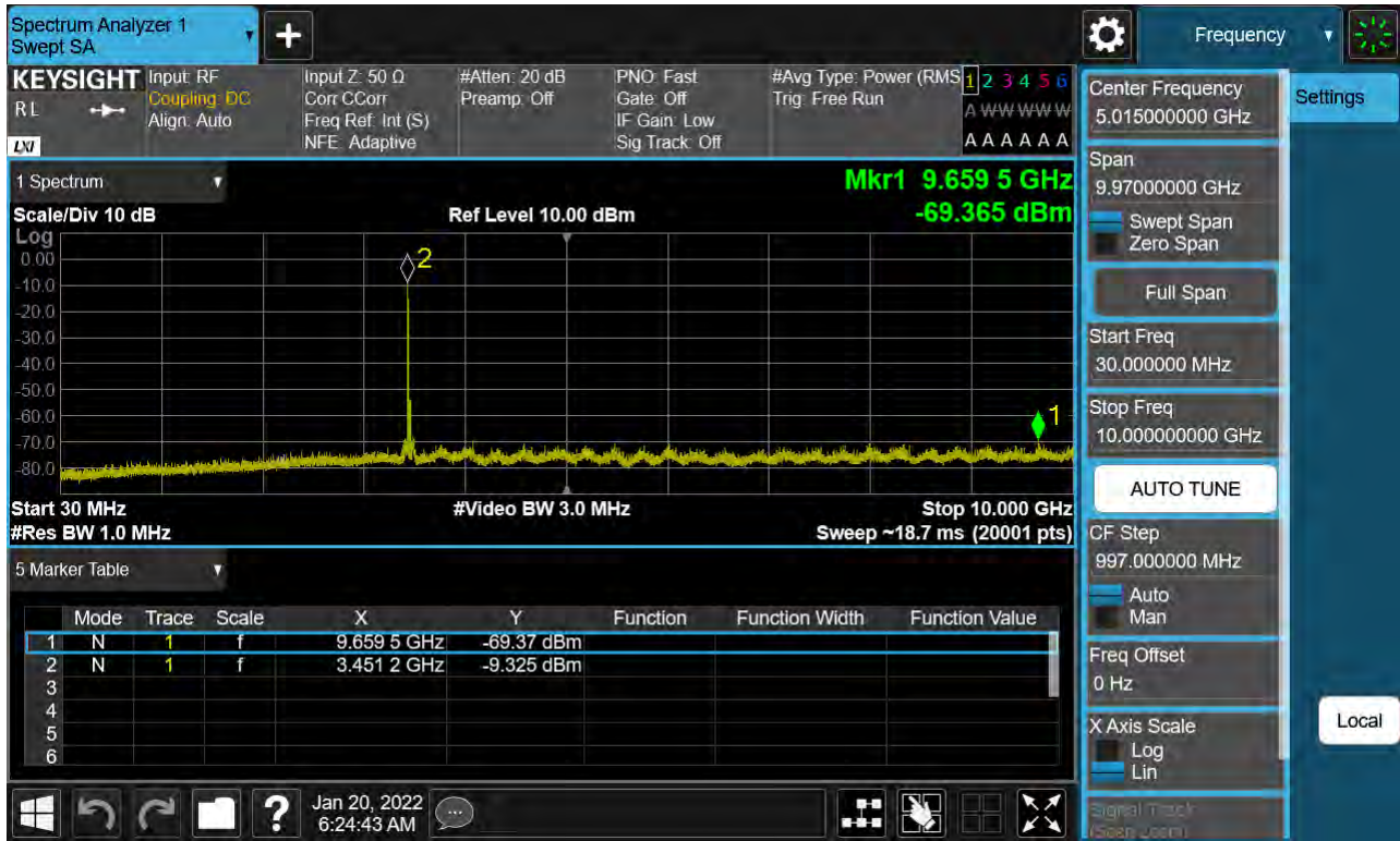
Sub6 n77. Conducted Spurious Plot_1 (630836ch_25 MHz_BPSK)
