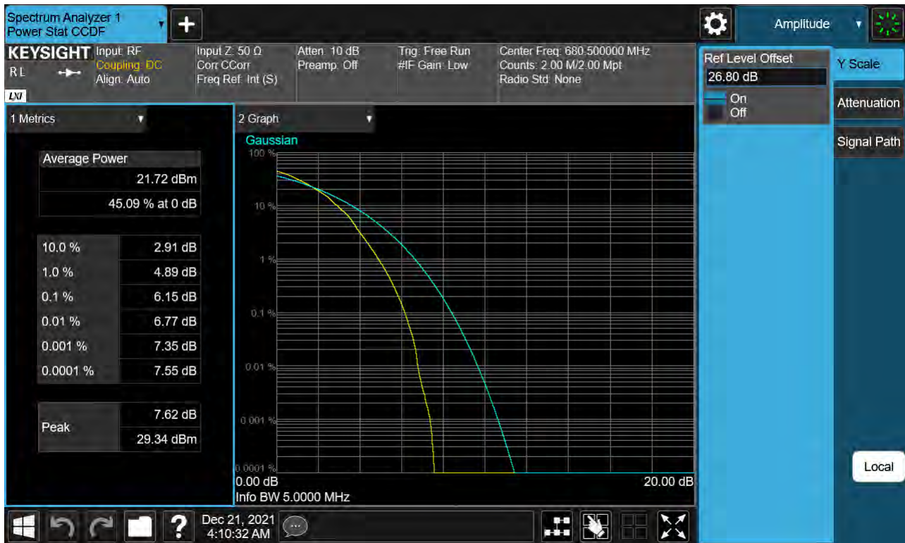
Sub6 n71. PAR Plot (5 M BW_Ch.349000_64QAM_Full RB)
