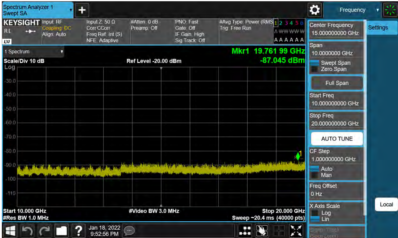
Sub6 n66. Conducted Spurious Plot_2 (349000ch_15 MHz_BPSK_ RB 1_1)
