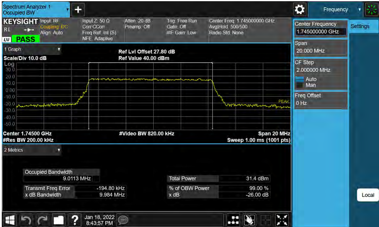
Sub6 n66. Occupied Bandwidth Plot (10 M BW Ch.349000 QPSK Full RB)
