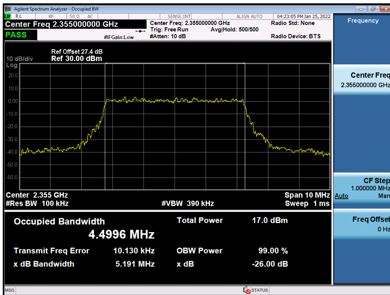
BAND 40. Occupied Bandwidth Plot (5 MHz 2355 MHz_64QAM_FullRB)
