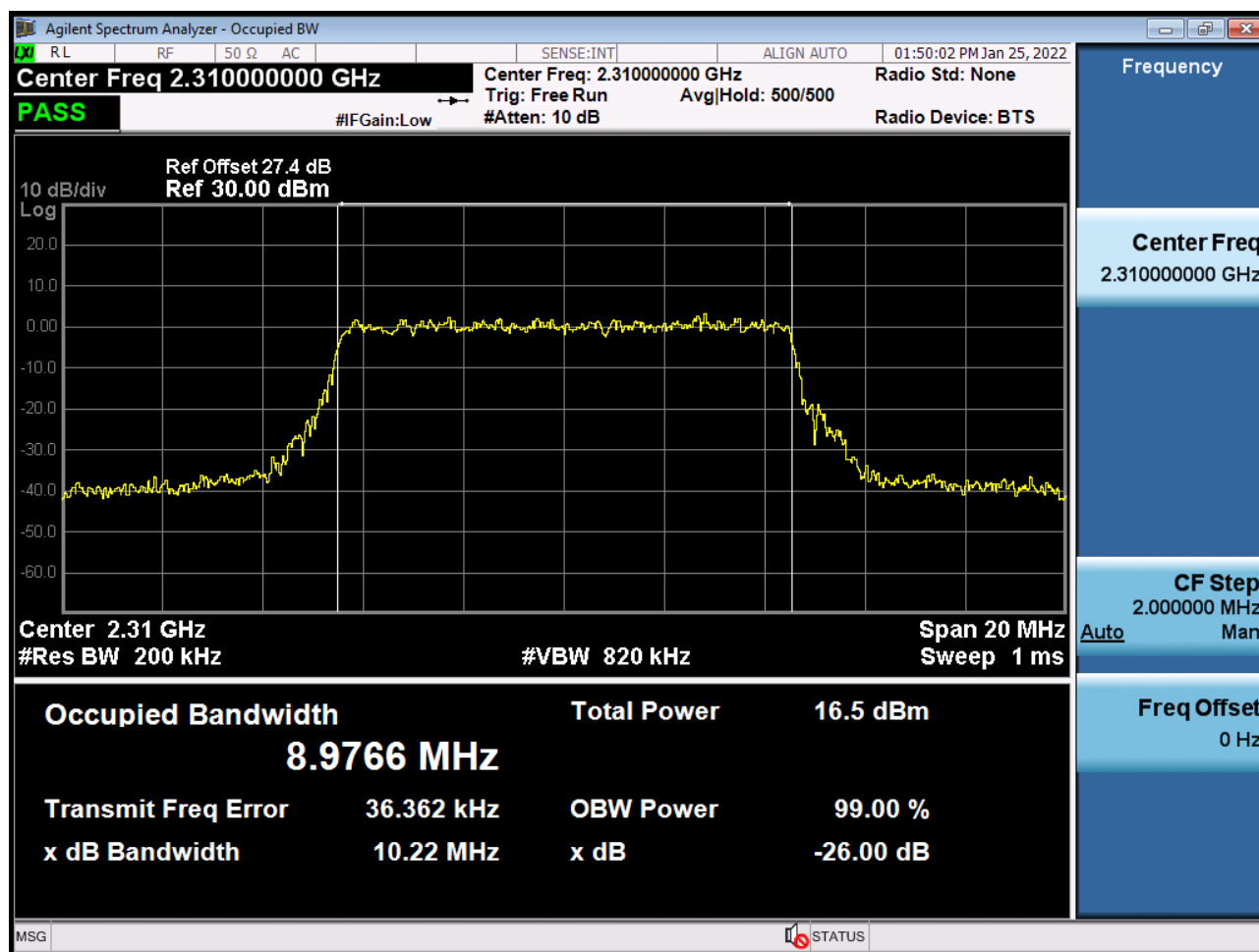
BAND 40. Occupied Bandwidth Plot (10 MHz 2310 MHz 16QAM FullRB)
