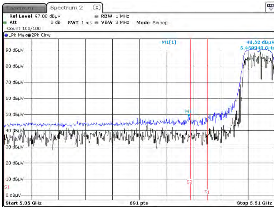
Peak Result (802.11 ac_VHT20_ MCS0, Ch.100)
