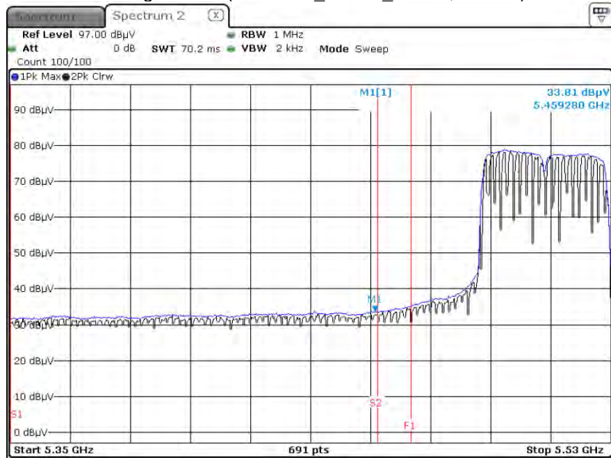
Average Result (802.11 ac_VHT40_ MCS0, Ch.102)
