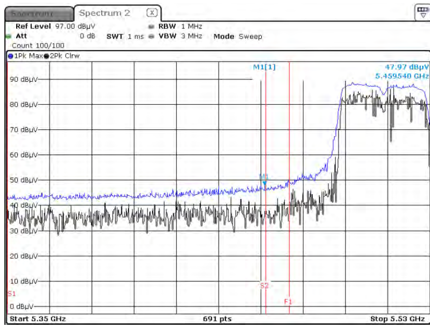
Peak Result (802.11 ac_VHT40_ MCS0, Ch.102)
