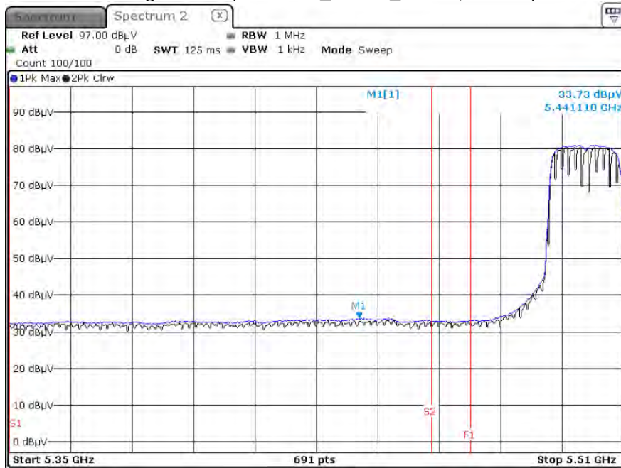
Average Result (802.11 ac_VHT20_ MCS0, Ch.100)
