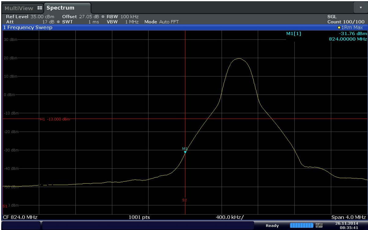
Plot 6-49. Lower Band Edge Plot (Band 5 – 10.0MHz – QPSK – RB Size 1)
