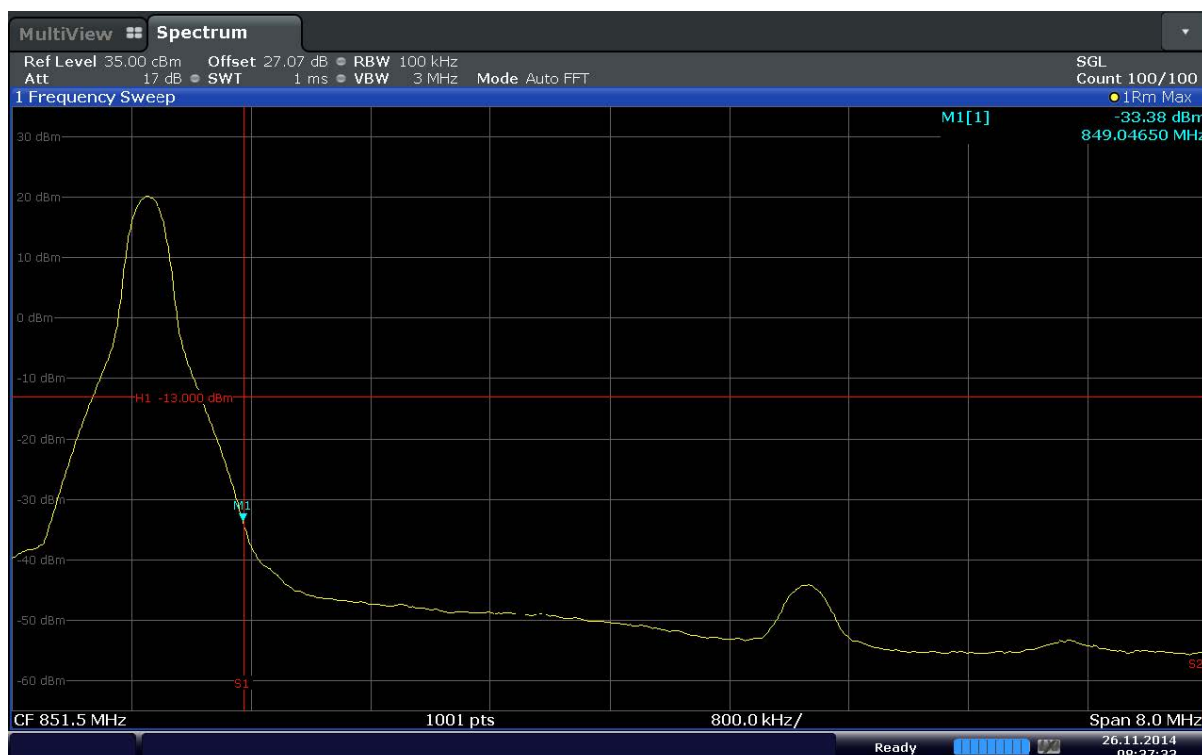
Plot 6-51. Upper Band Edge Plot (Band 5 – 10.0MHz – QPSK – RB Size 1)
