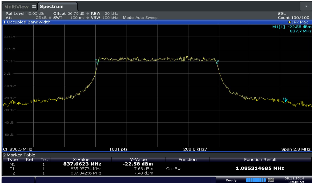
Plot 6-2. Occupied Bandwidth Plot (Band 5 – 1.4MHz 16QAM - RB Size 6)
