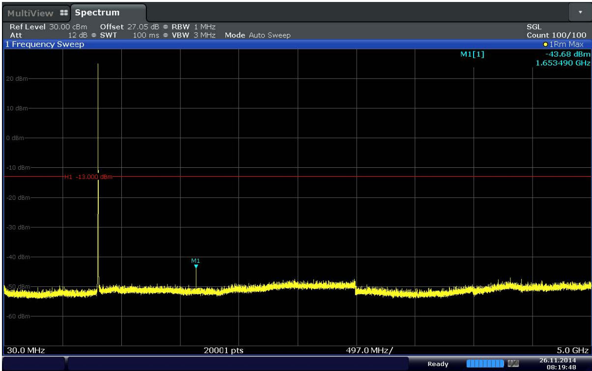
Plot 6-15. Conducted Spurious Plot (Band 5–3.0MHz–QPSK–RB Size 1–RB Offset 14– Ch.20415)
