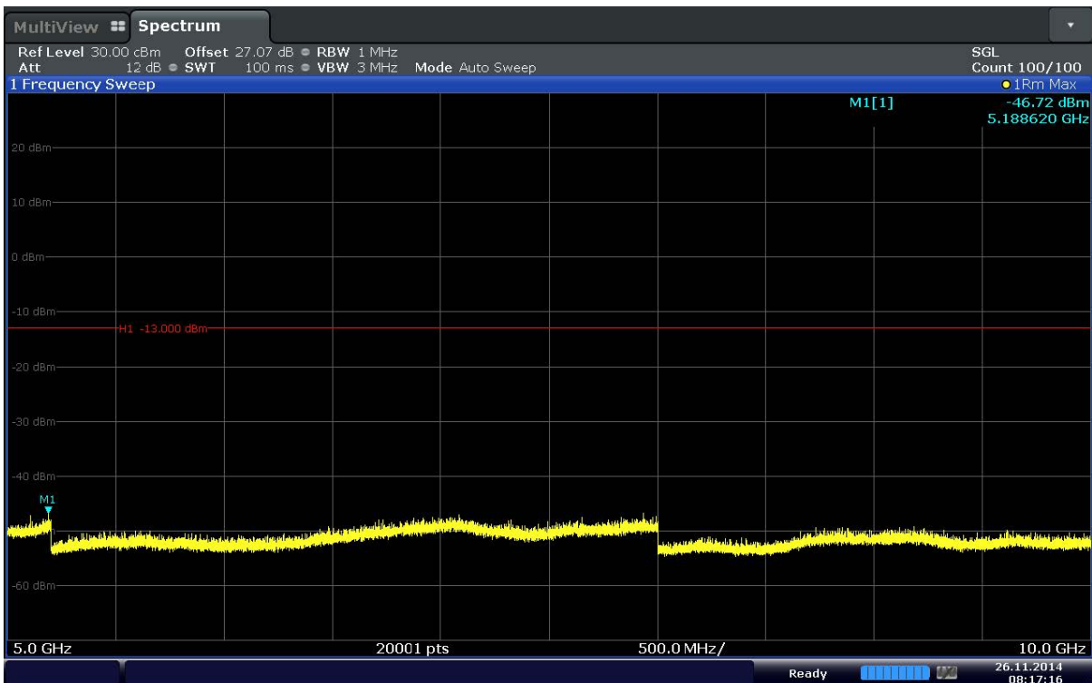
Plot 6-11. Conducted Spurious Plot (Band 5-1.4MHz-QPSK-RB Size 1-RB Offset 2-Ch.20525)
