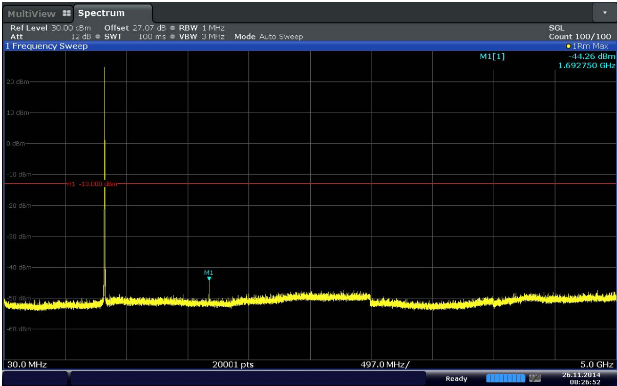
Plot 6-25. Conducted Spurious Plot (Band 5–5.0MHz–16QAM–RB Size 1–RB Offset 12– Ch.20625)
