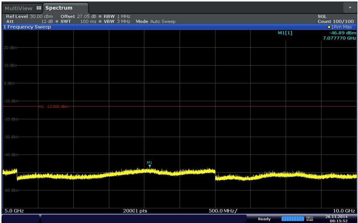
Plot 6-10. Conducted Spurious Plot (Band 5-1.4MHz-QPSK-RB Size 3-RB Offset 0-Ch.20407)
