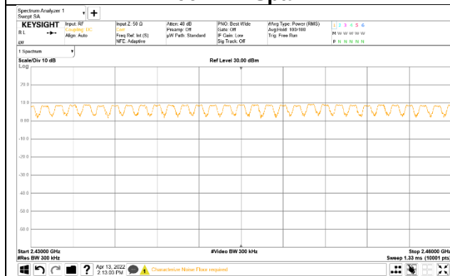
30MHz SPAN, SEGMENT 2 OF 3
