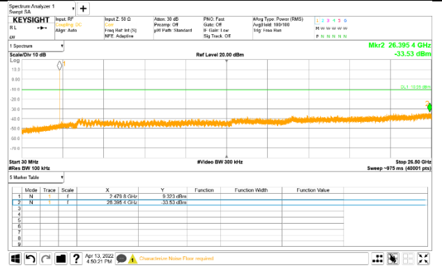
OUT-OF-BAND 78 CHANNEL
