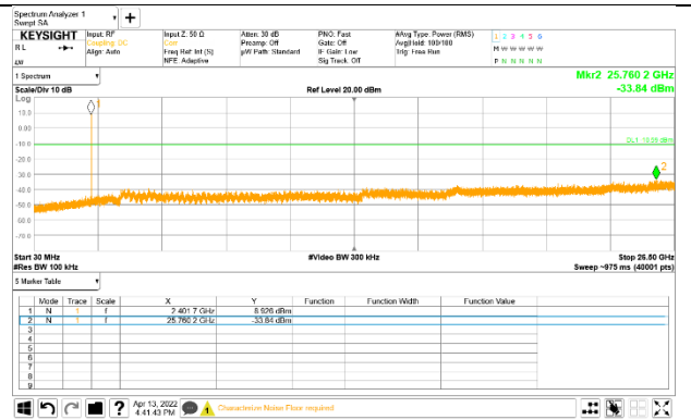
OUT-OF-BAND 0 CHANNEL
