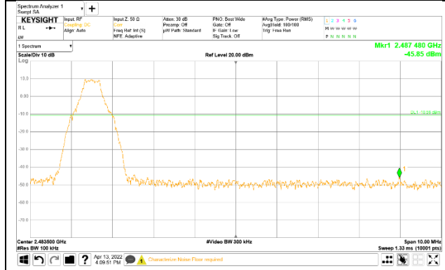
78 CHANNEL BANDEDGE
