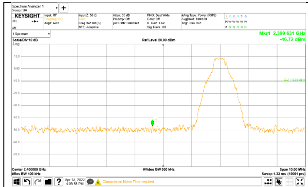
0 CHANNEL BANDEDGE
