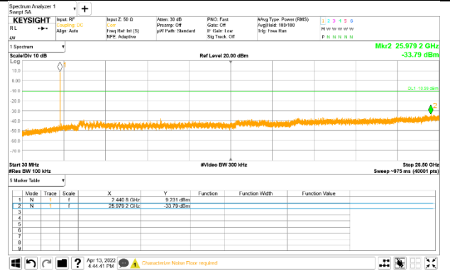
OUT-OF-BAND 39 CHANNEL
