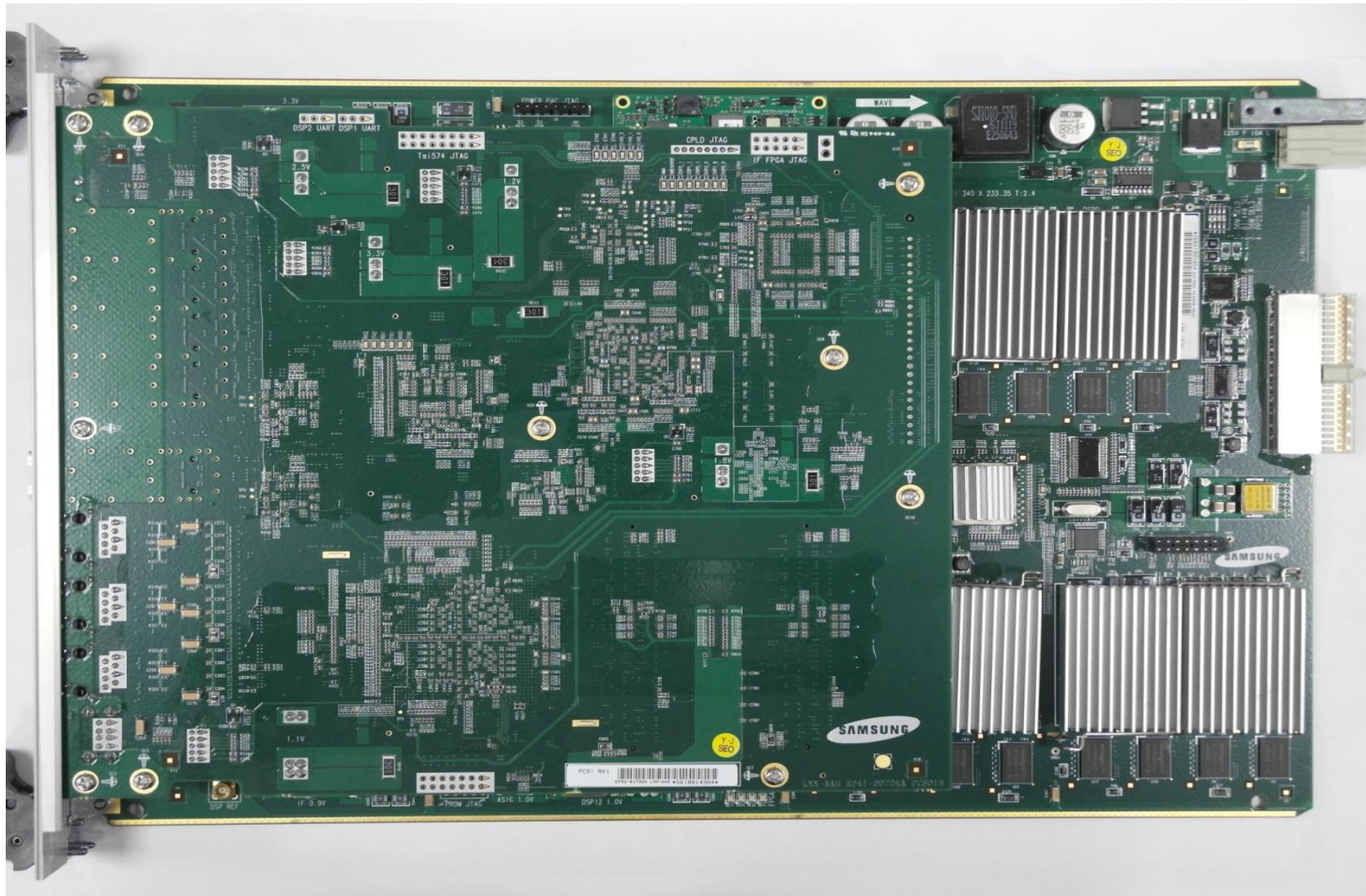
[MRA-L with the LMM-AAS daughter board equipped on the top of the MRA-L]
