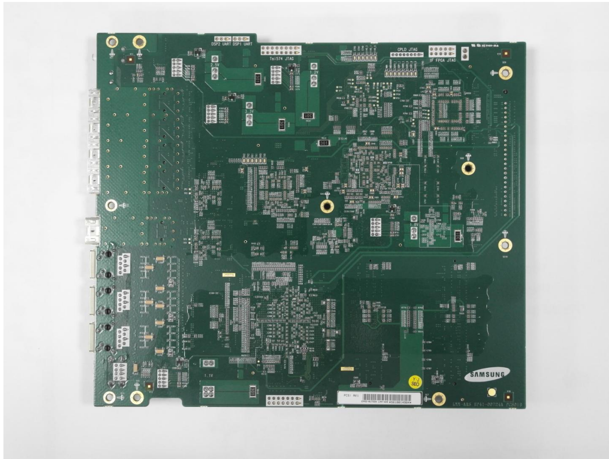
[LMM-AAS Daughter board Bottom]
