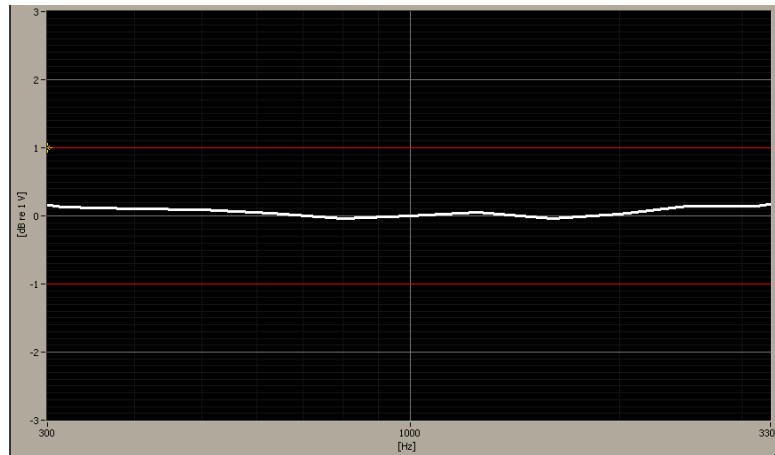
Figure 6-3 Helmholtz Coil Validation for Frequency Response
