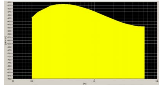
Figure 5-4 P.50 Artificial Voice Signal
