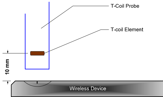
Figure 5-11 Measurement Distance
