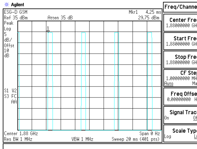
Figure 8-4 GSM Signal
